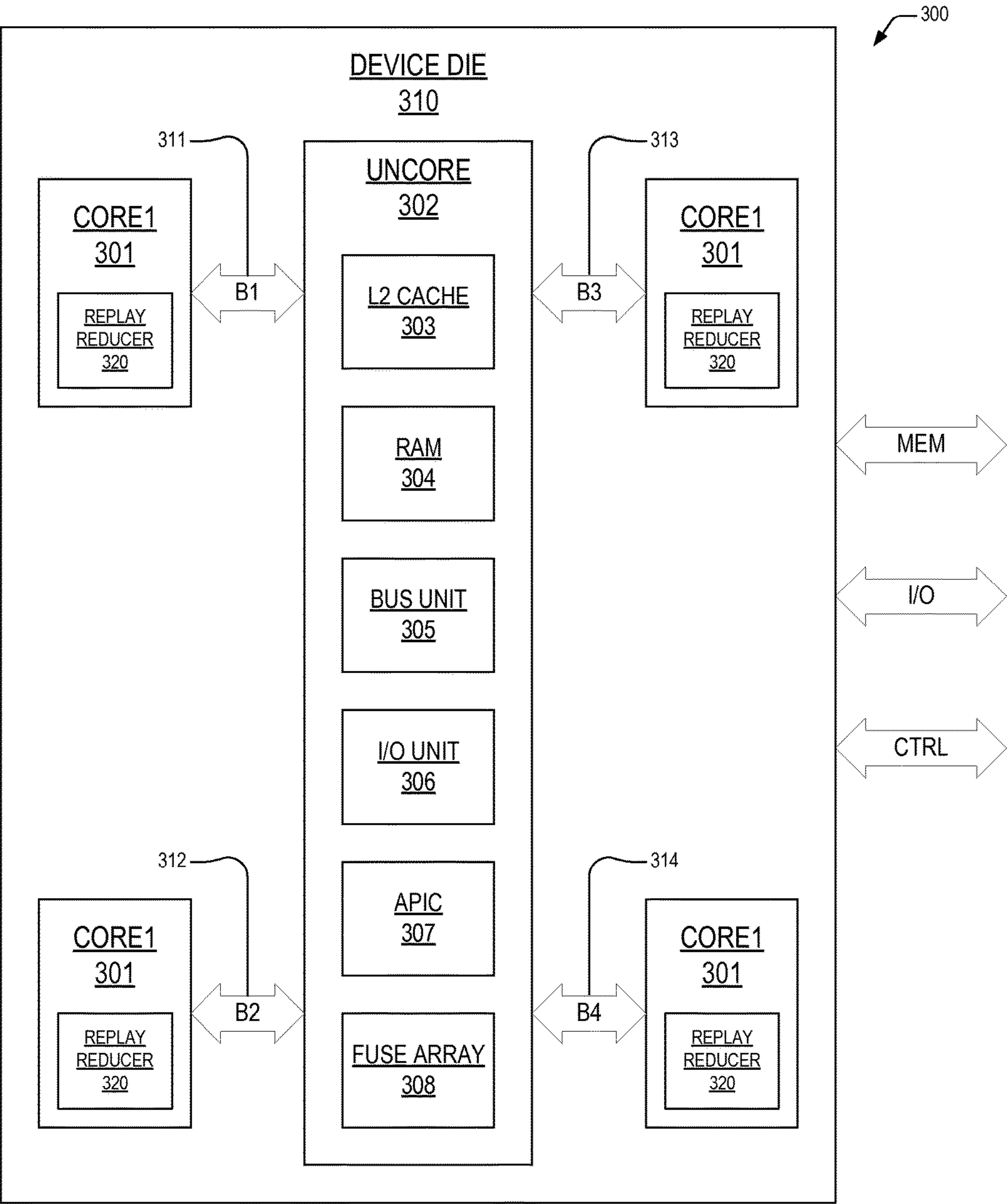
FIG. 3 POWER SAVING MECHANISM FOR LOADS FROM NON-CORE RESOURCES
