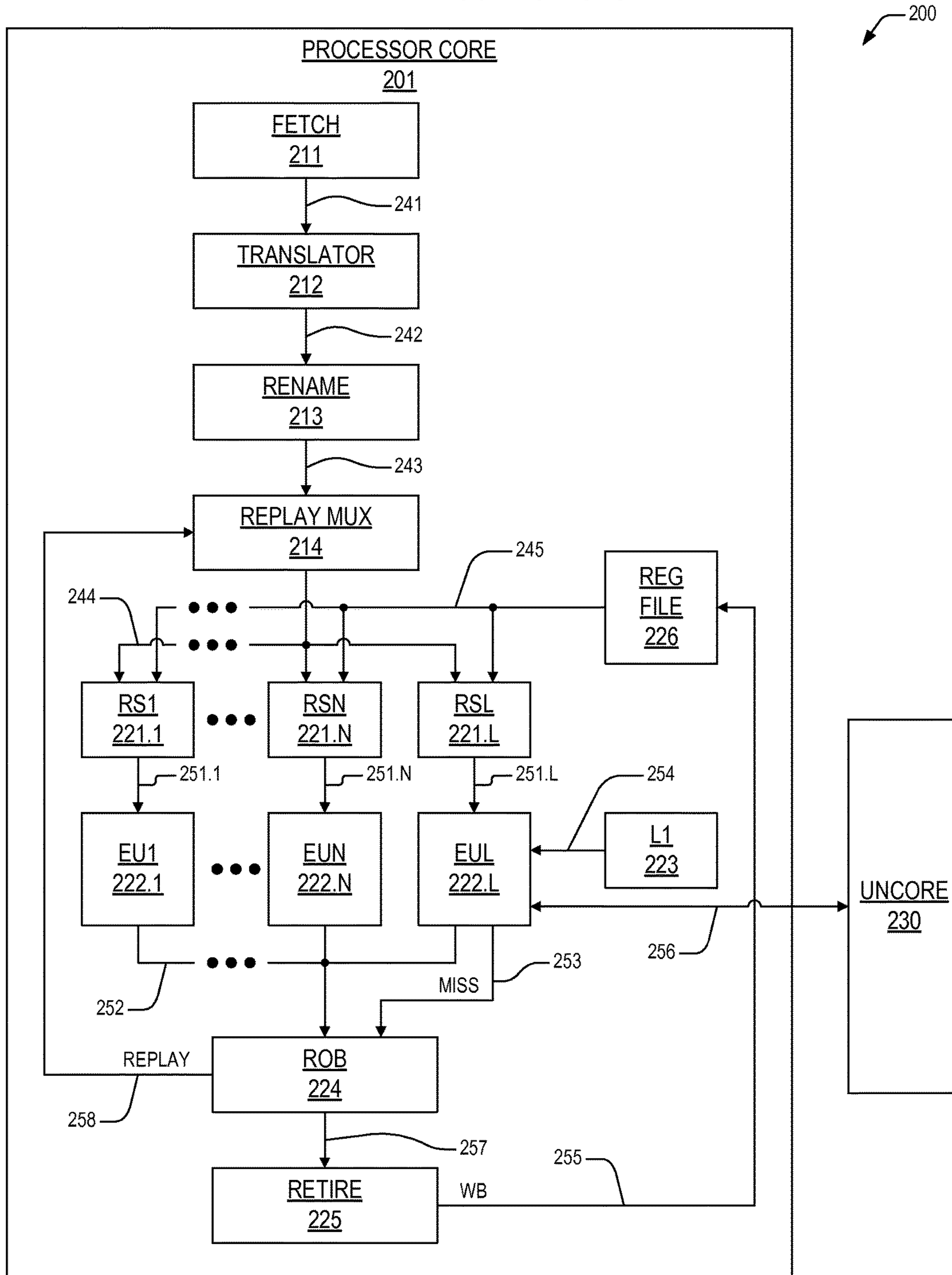
FIG. 2 (Prior Art)
