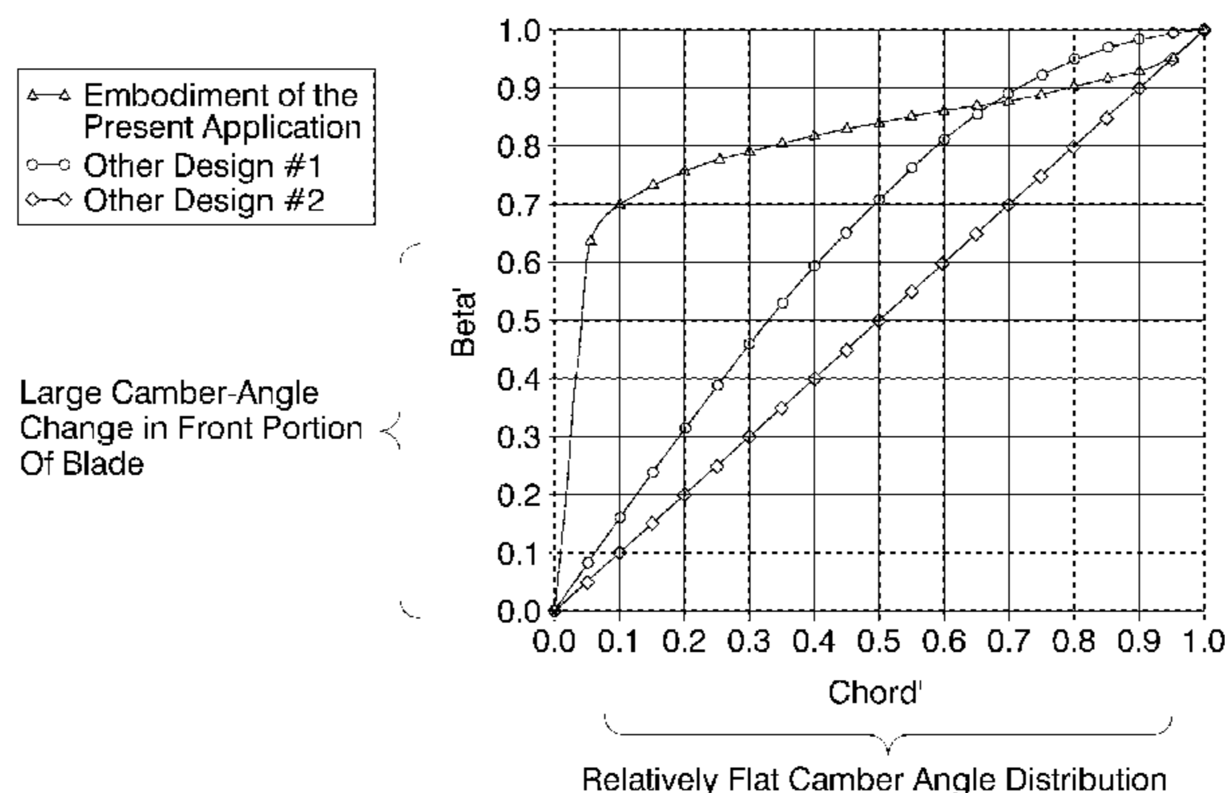
Normalized Beta Distributions vs. Normalized Chord
