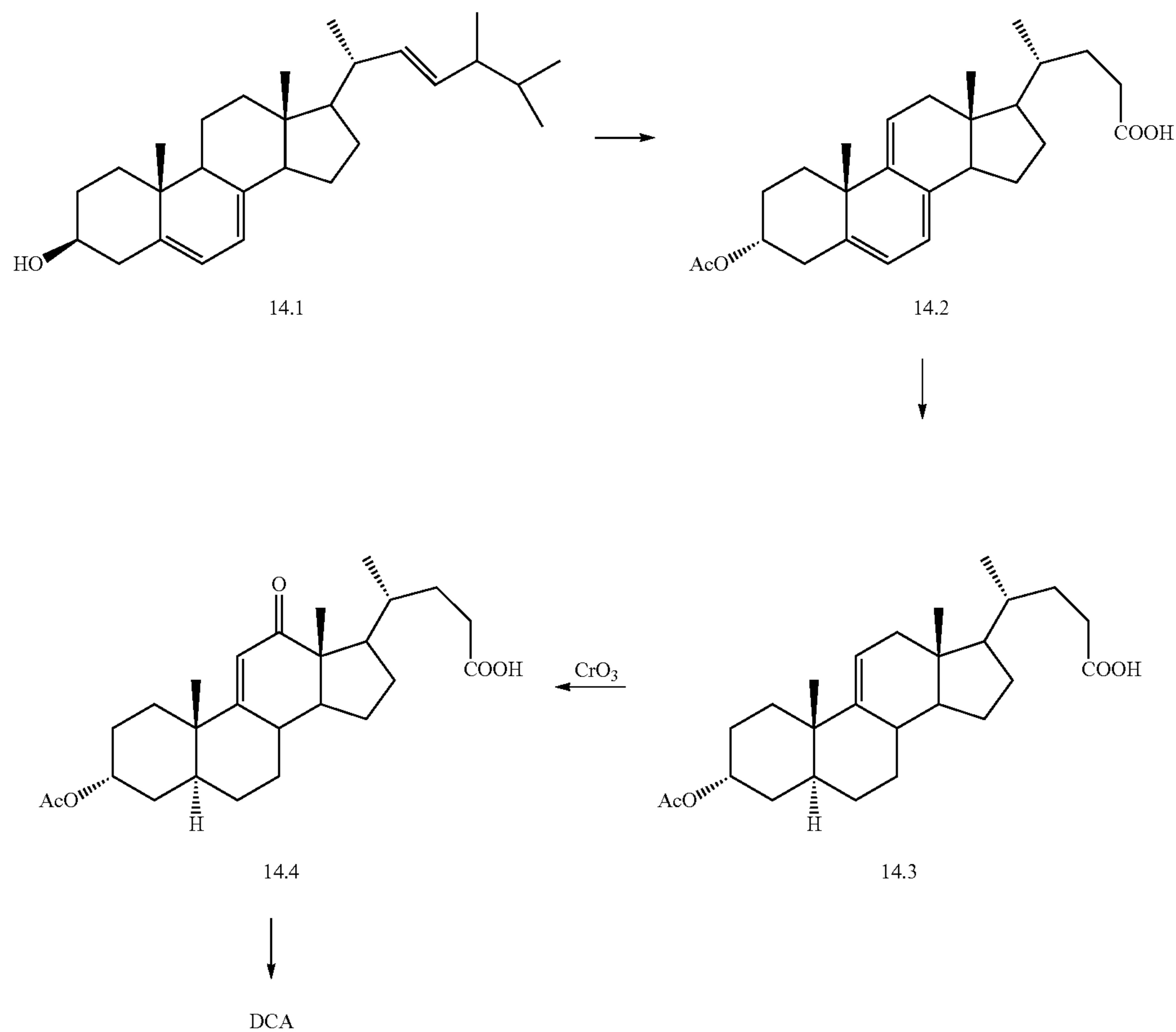
Scheme 14. Triene formation from Ergosterol
