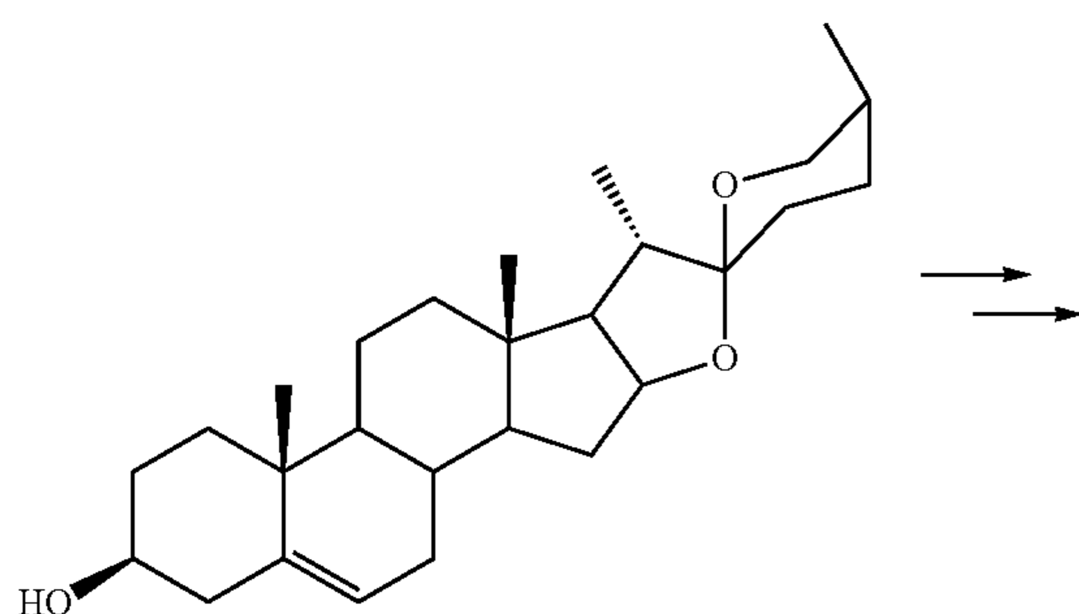
General Sapogenin formula
