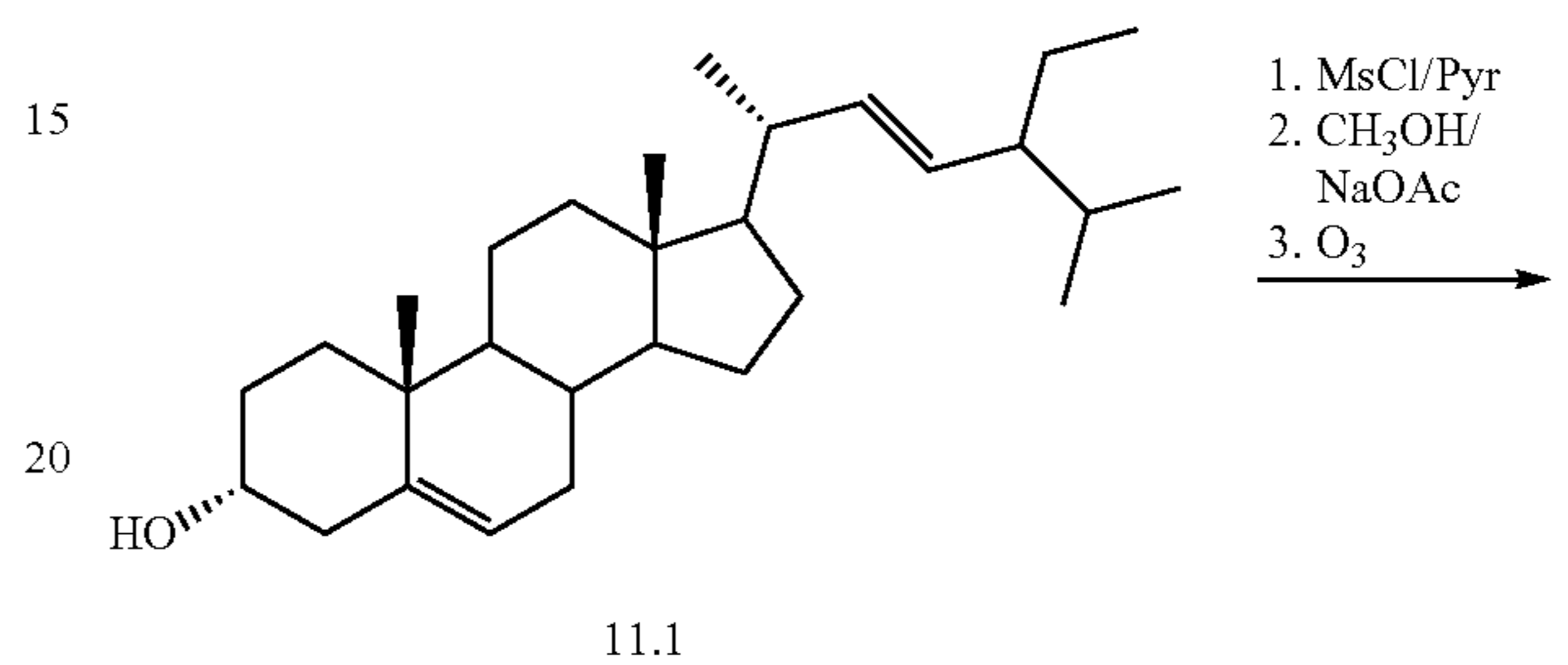
Scheme 11. Ozonolysis of i-steroid and side chain reduction
