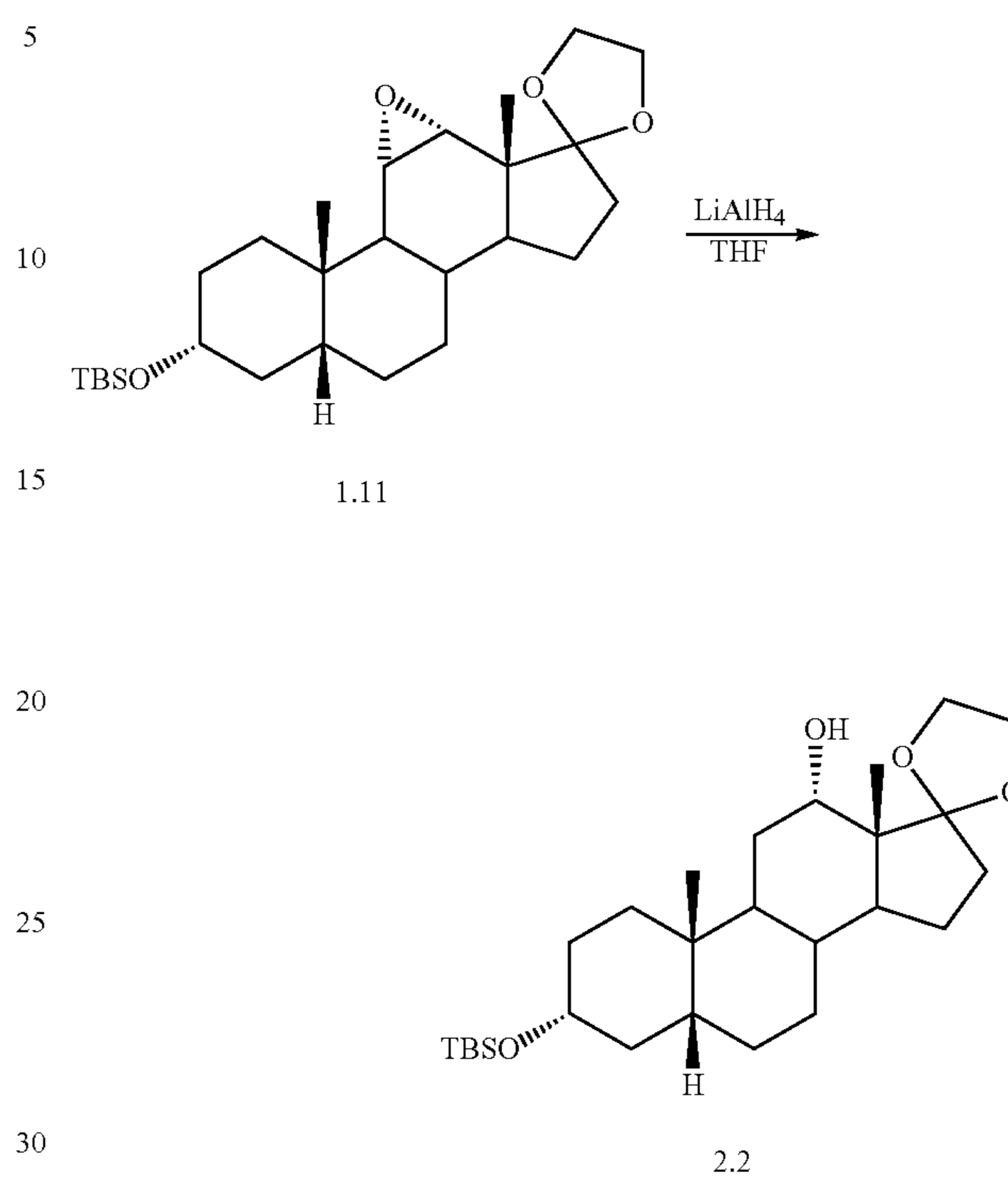
Scheme 3. Stereoselective Reduction of C 11 -C 12 epoxide.
