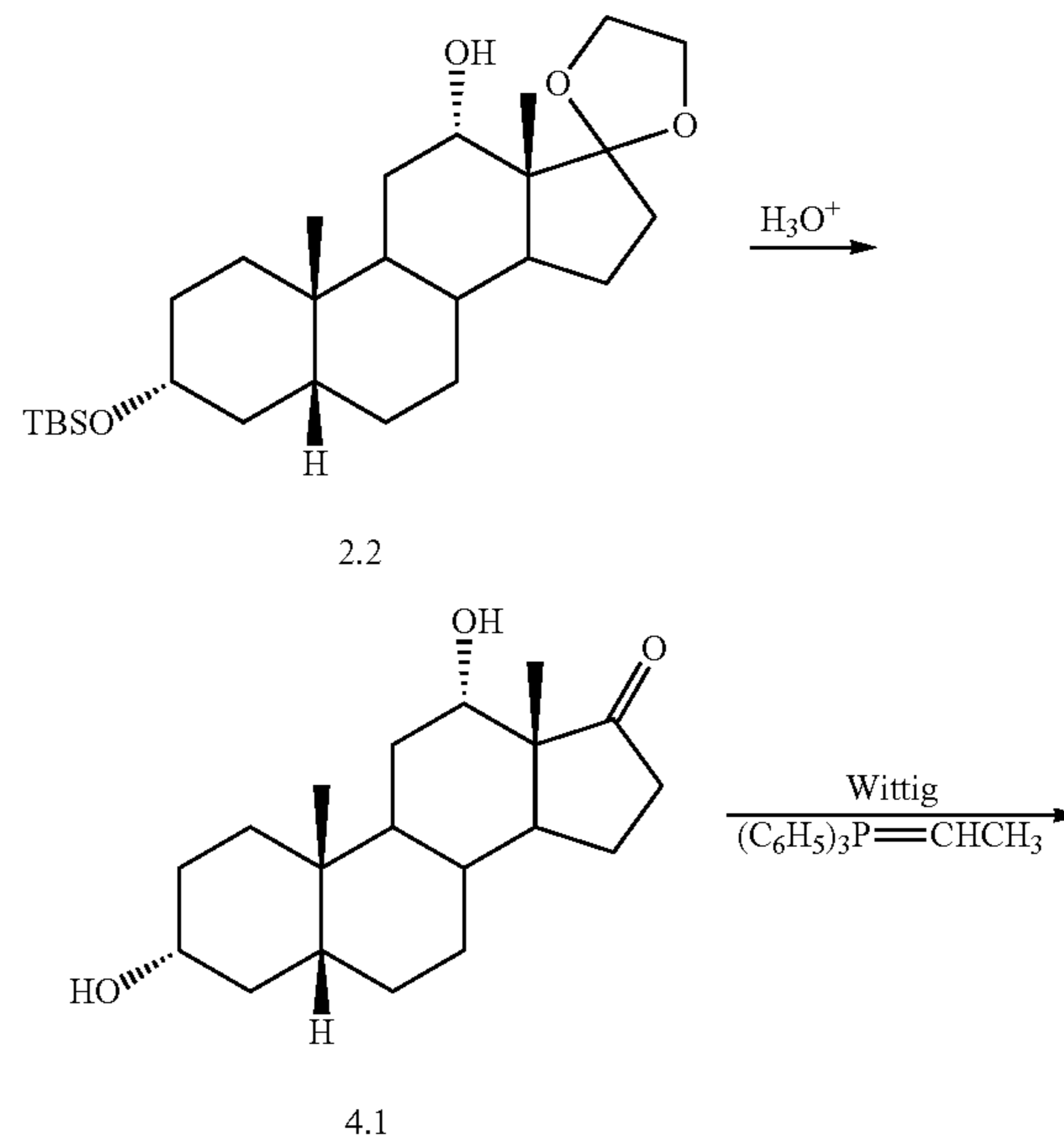
Scheme 4. Deprotection and Wittig Reaction
