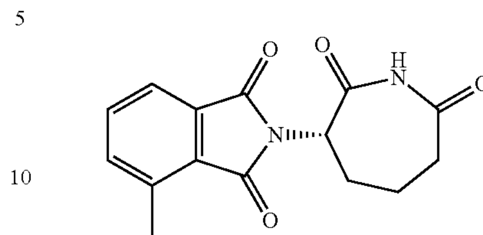
4-Amino-2-[(3R)-2,7-dioxoazepan-3-yl]isoindoline-1,3-dione (Compound 20)
