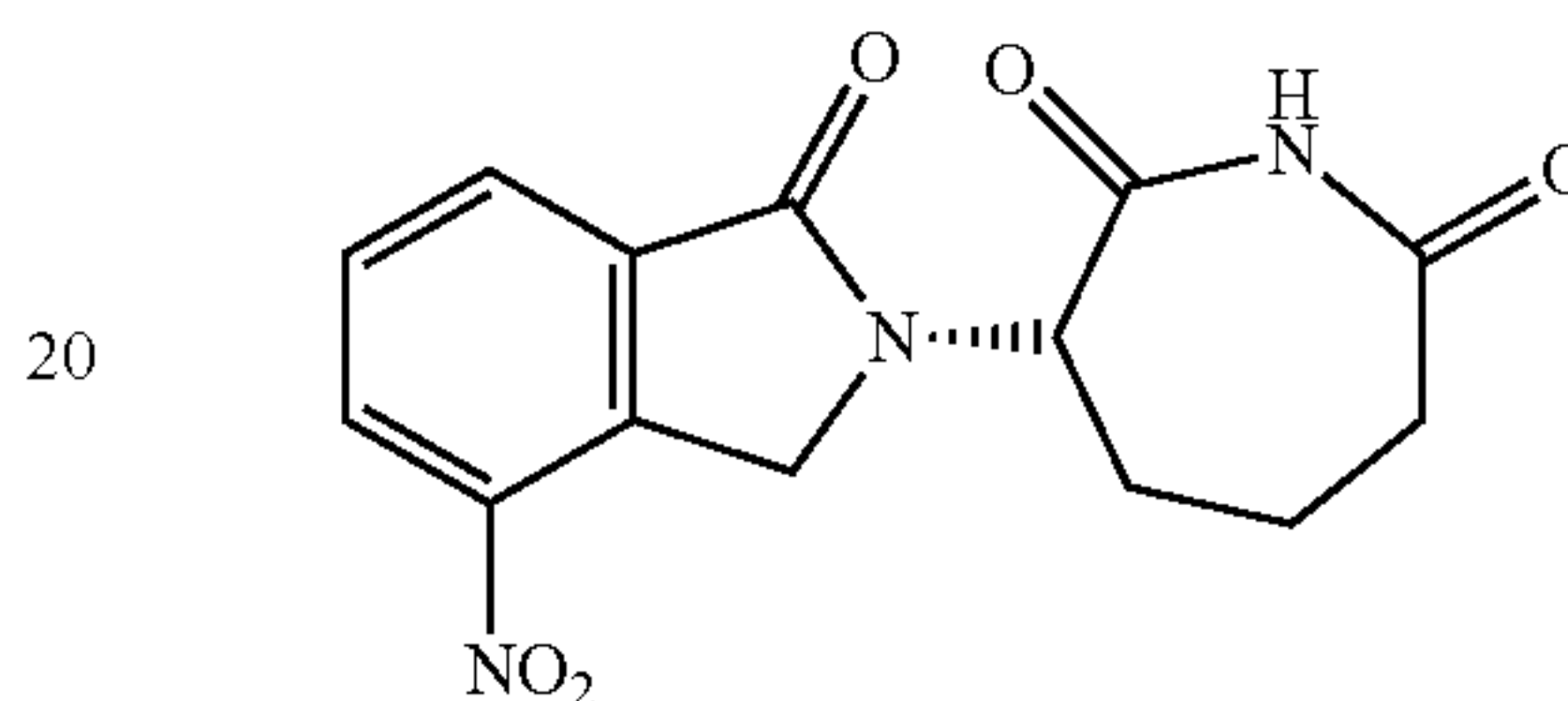
(3S)-3-[(2S)-5-Methyl-2-isoindolinoyl]-2,7-azepinedione (Compound 35)
