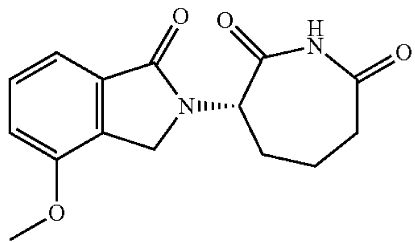
(3S)-3-[(2S)-4-Methoxy-2-isoindolinoyl]-2,7-azepinedione (Compound 34)
