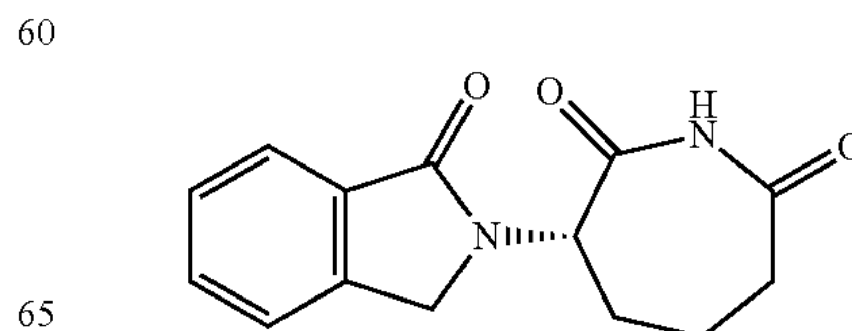
(3S)-3-[(2S)-2-Isoindolinoyl]-2,7-azepinedione (Compound 26)
