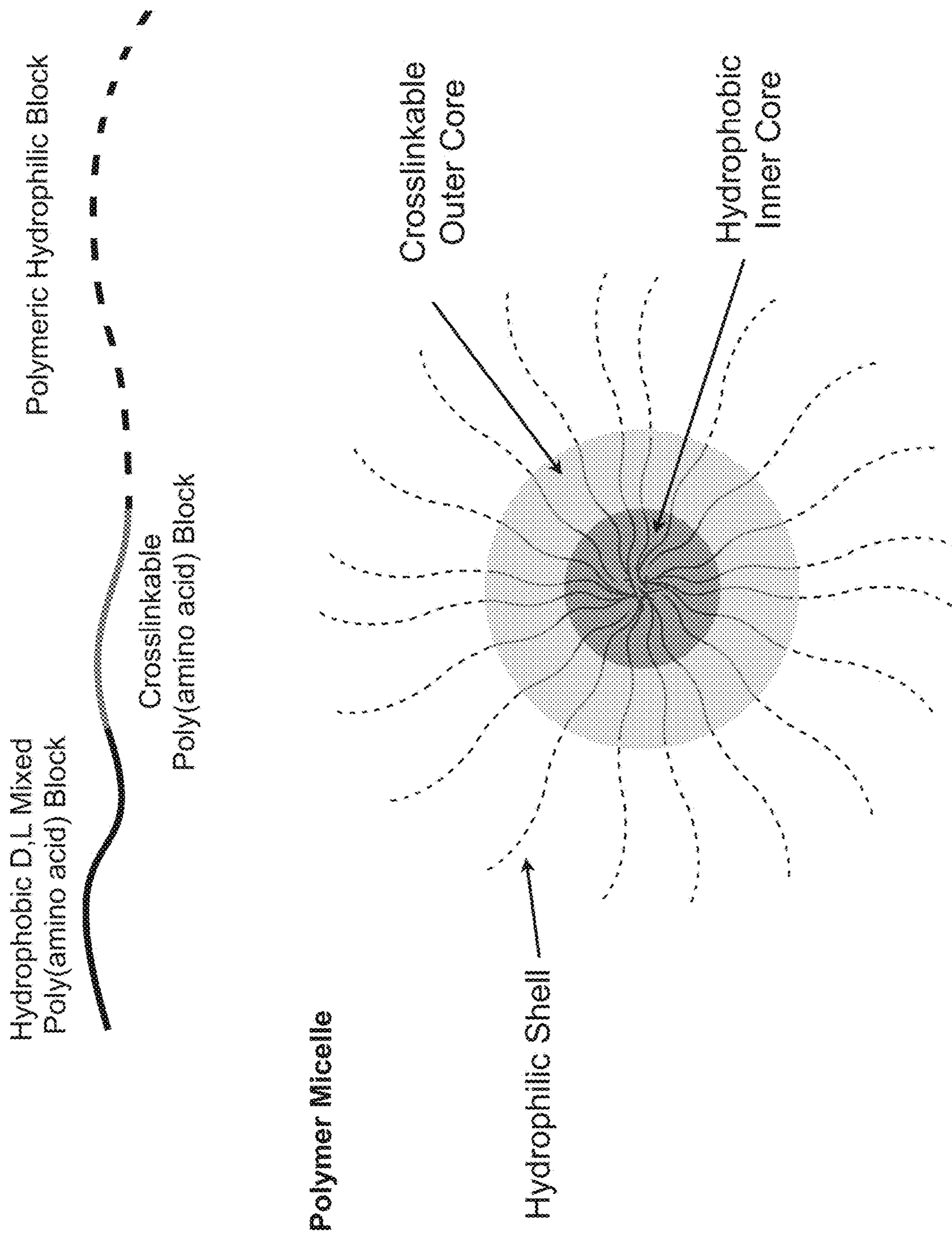
Figure 1. Triblock Copolymer
