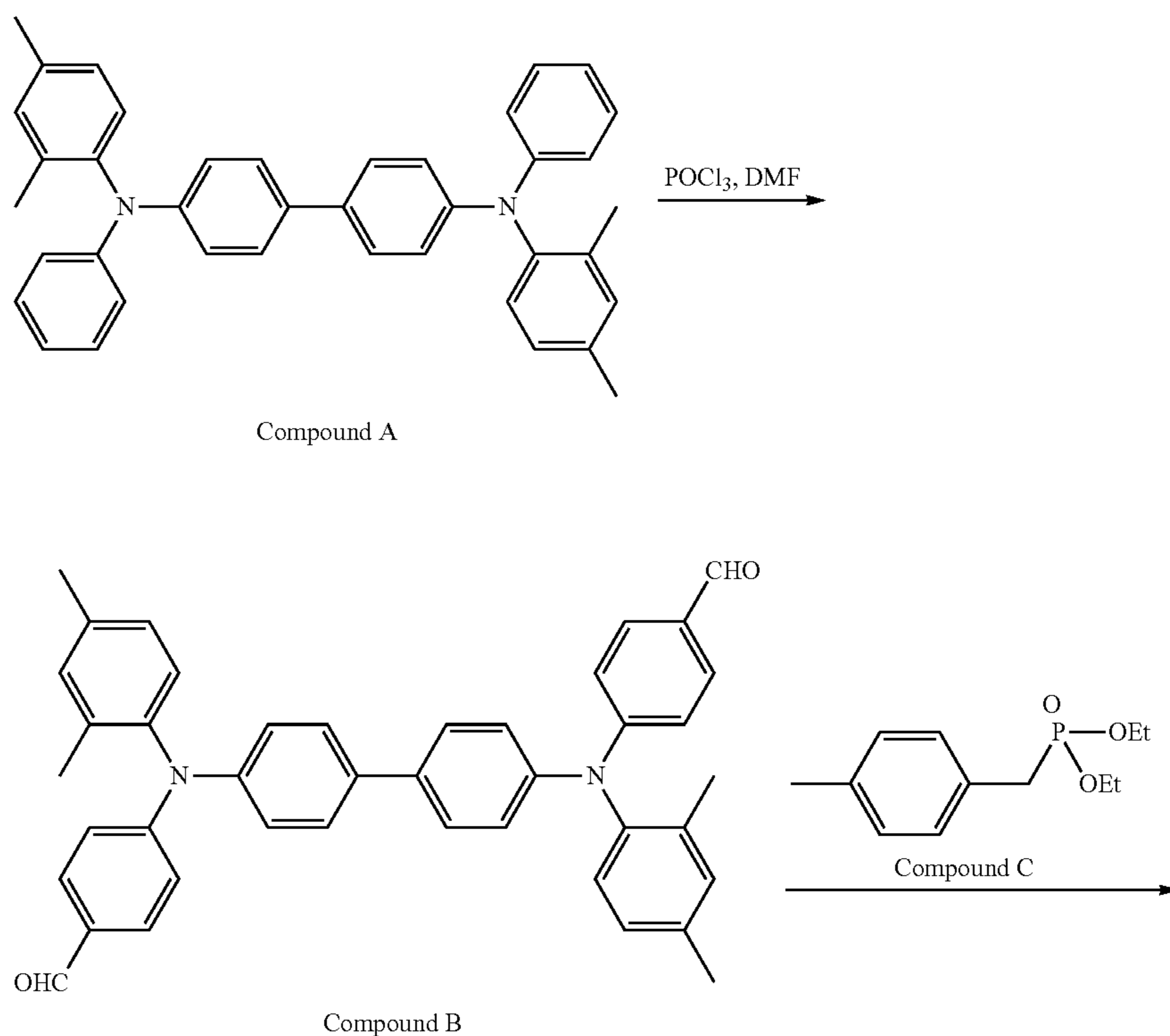
(Scheme 1)
