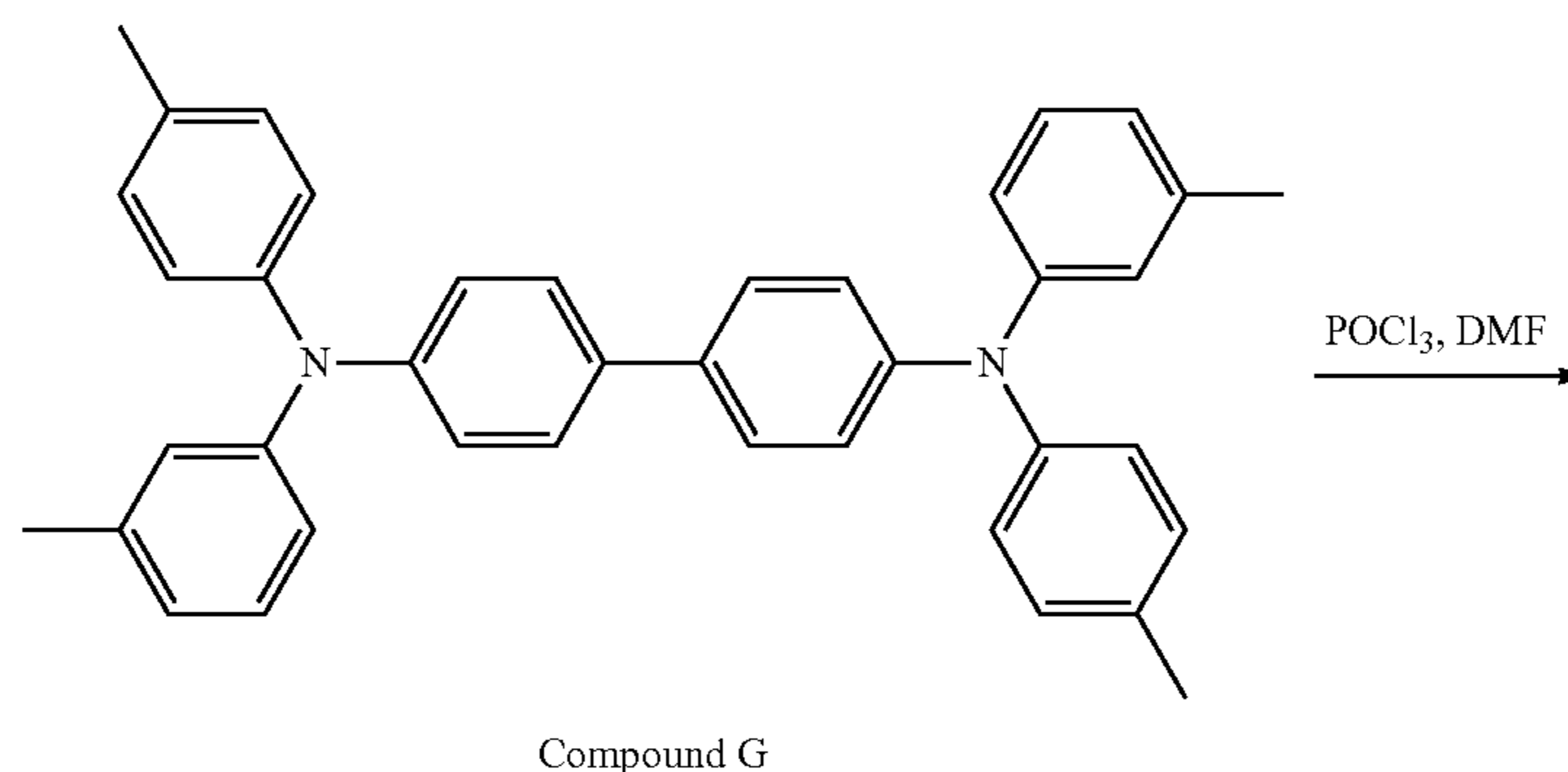
(Scheme 3)
