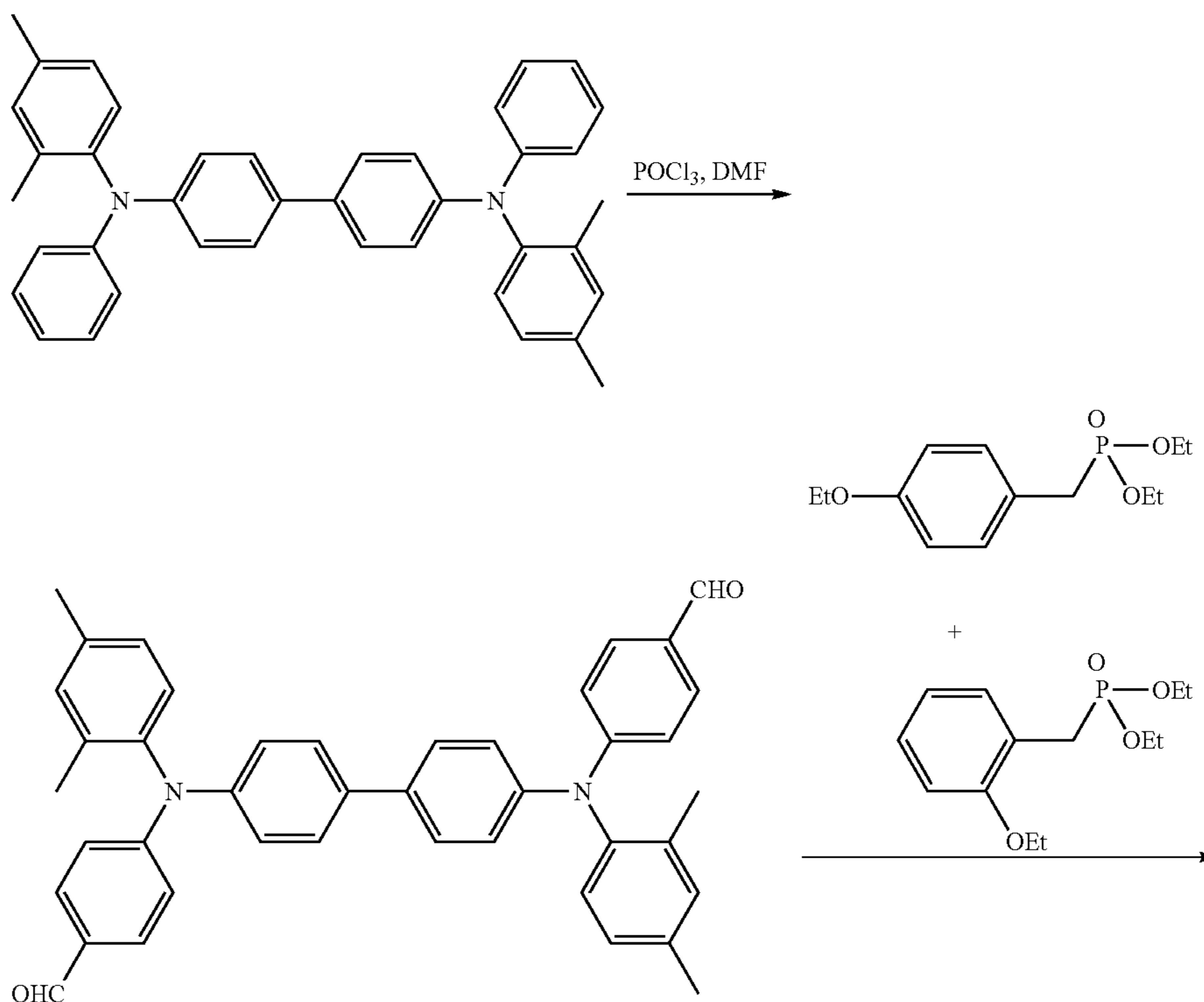
(Scheme 3)
