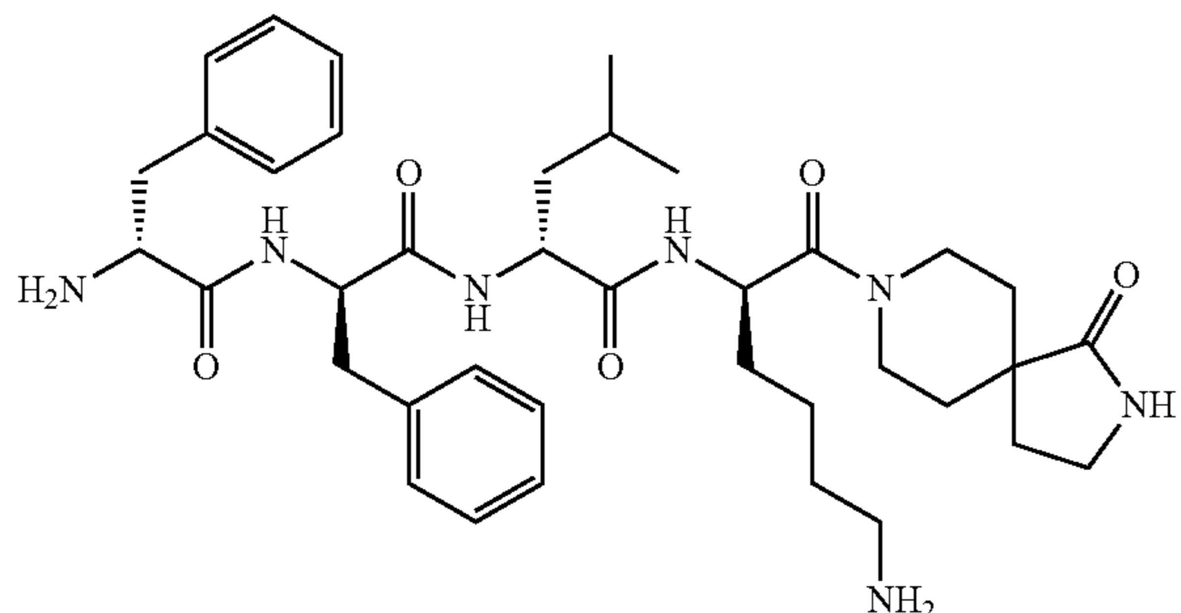
Compound (26): D-Phe-D-Phe-D-Leu-D-Lys-[2-methyl-2,8-diazaspiro[4,5]decan-1-one amide] (SEQ ID NO: 2):
