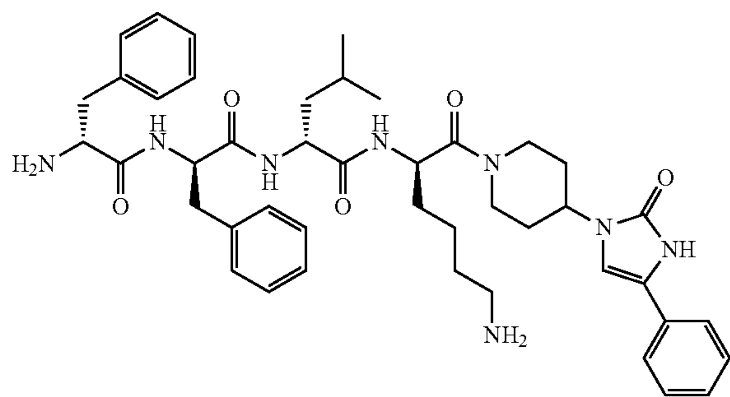
Compound (31): D-Phe-D-Phe-D-Leu-D-Lys-[4-(3,5-dimethyl-4H-1,2,4-triazol-4-yl)piperidine amide] (SEQ ID NO: 2):
