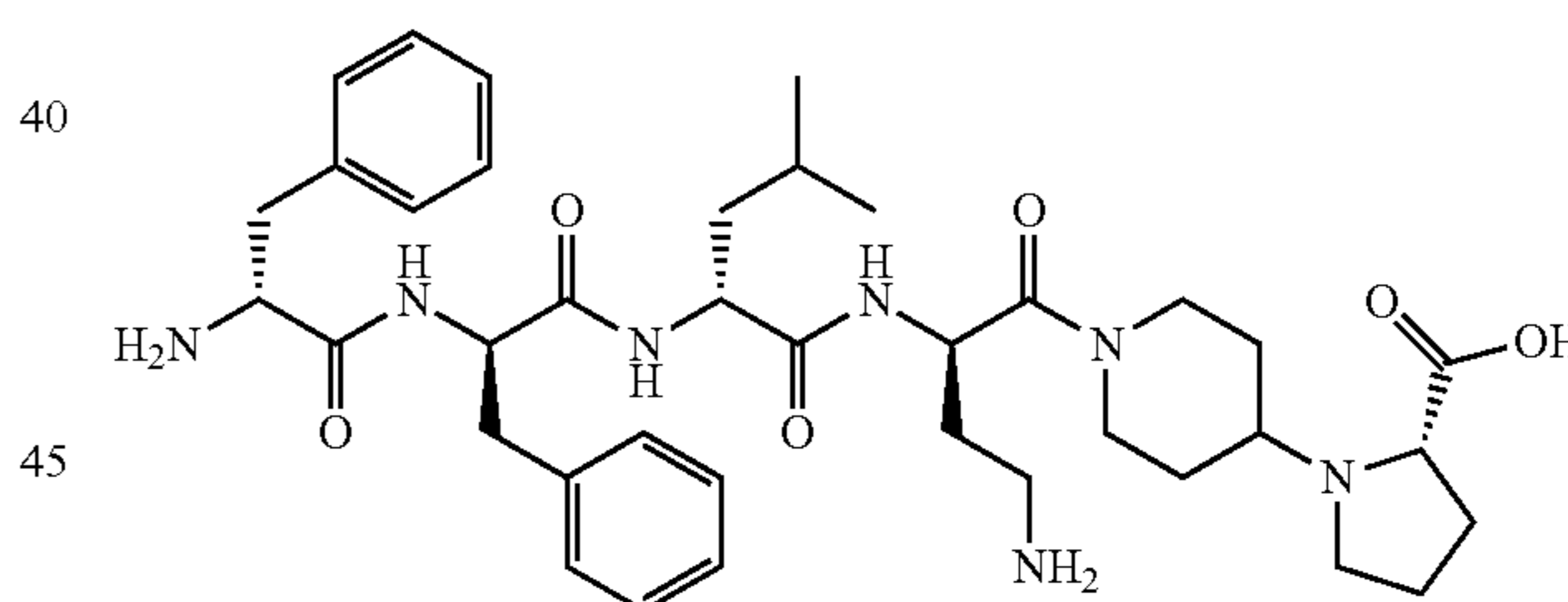
Compound (13): D-Phe-D-Phe-D-Leu-D-Nar-[N-(4-piperidiny)l-L-proline]-OH (SEQ ID NO: 7):
