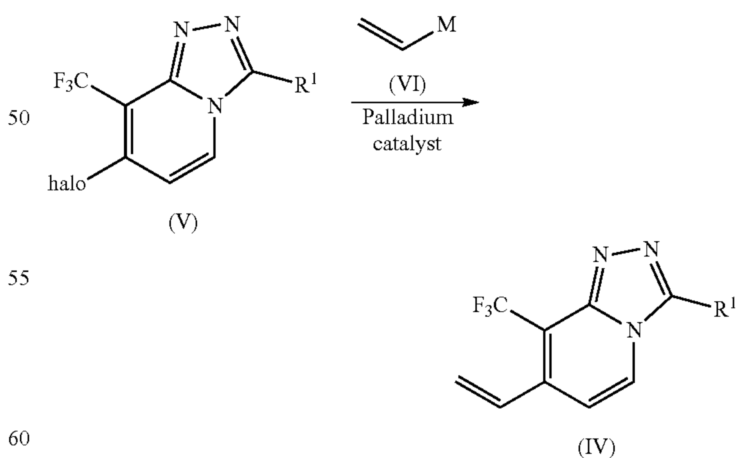
Reaction Scheme 4
