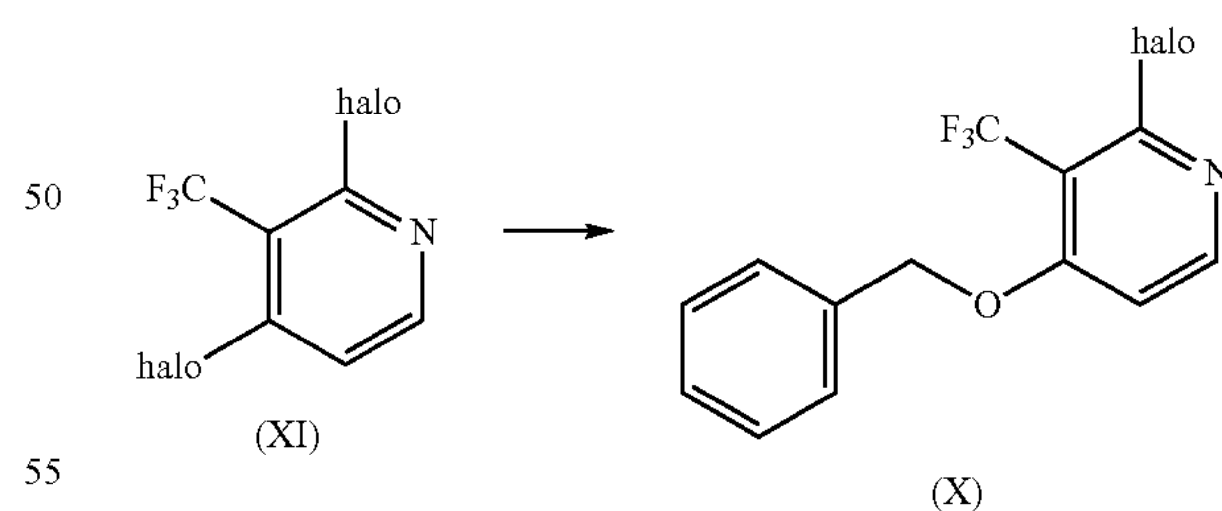
Reaction Scheme 8
