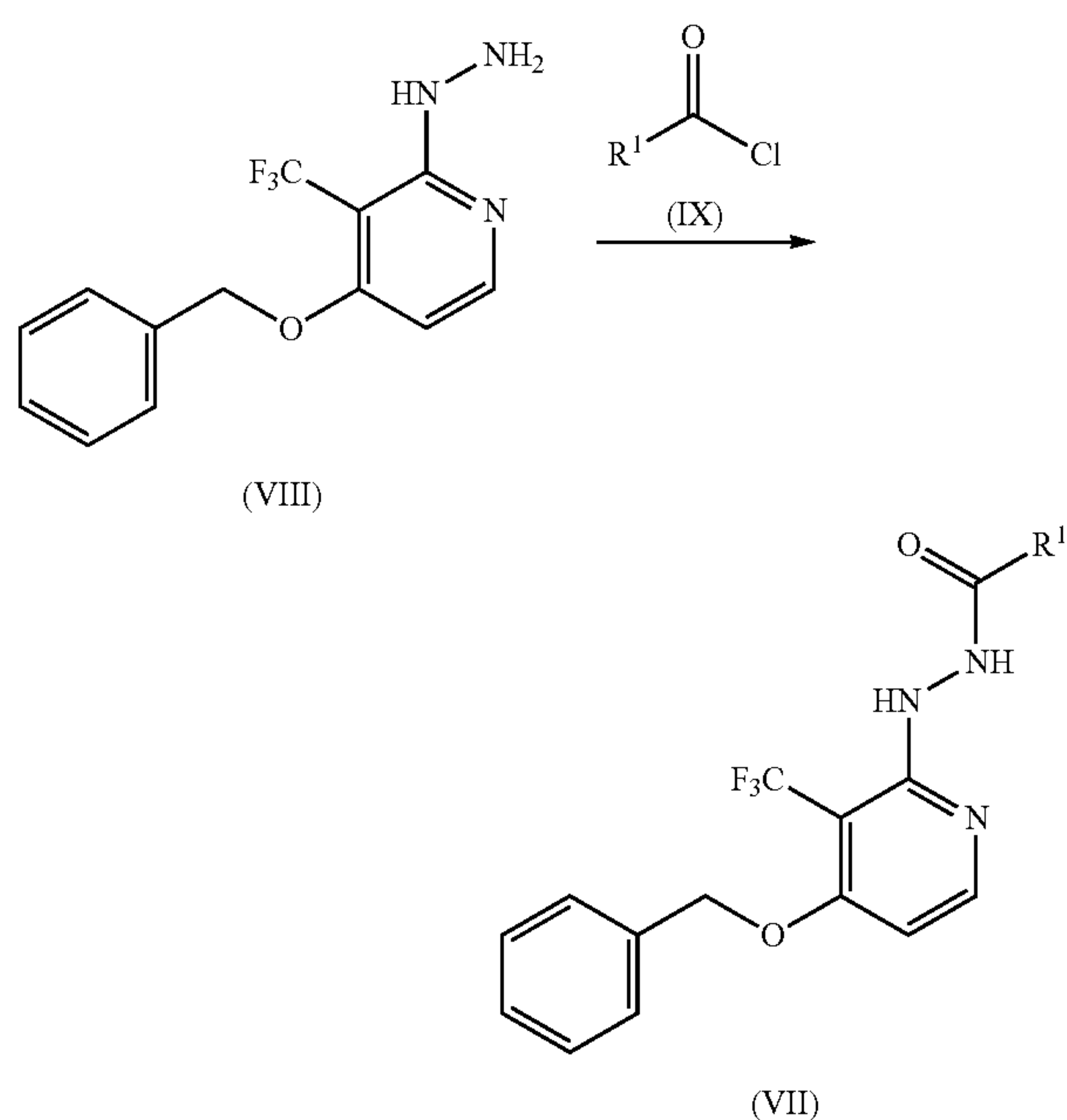
Reaction Scheme 6
