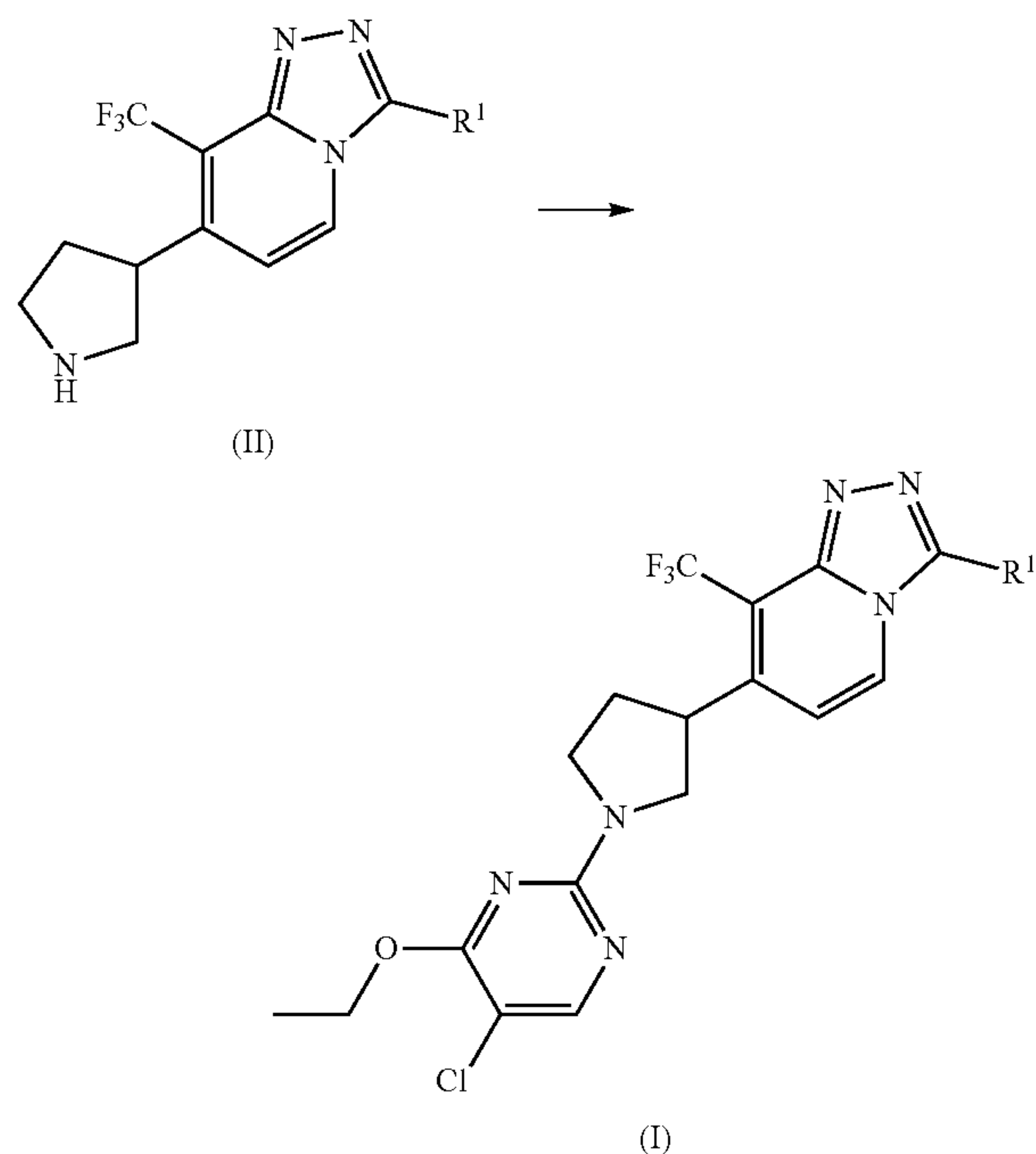
Reaction Scheme 1
