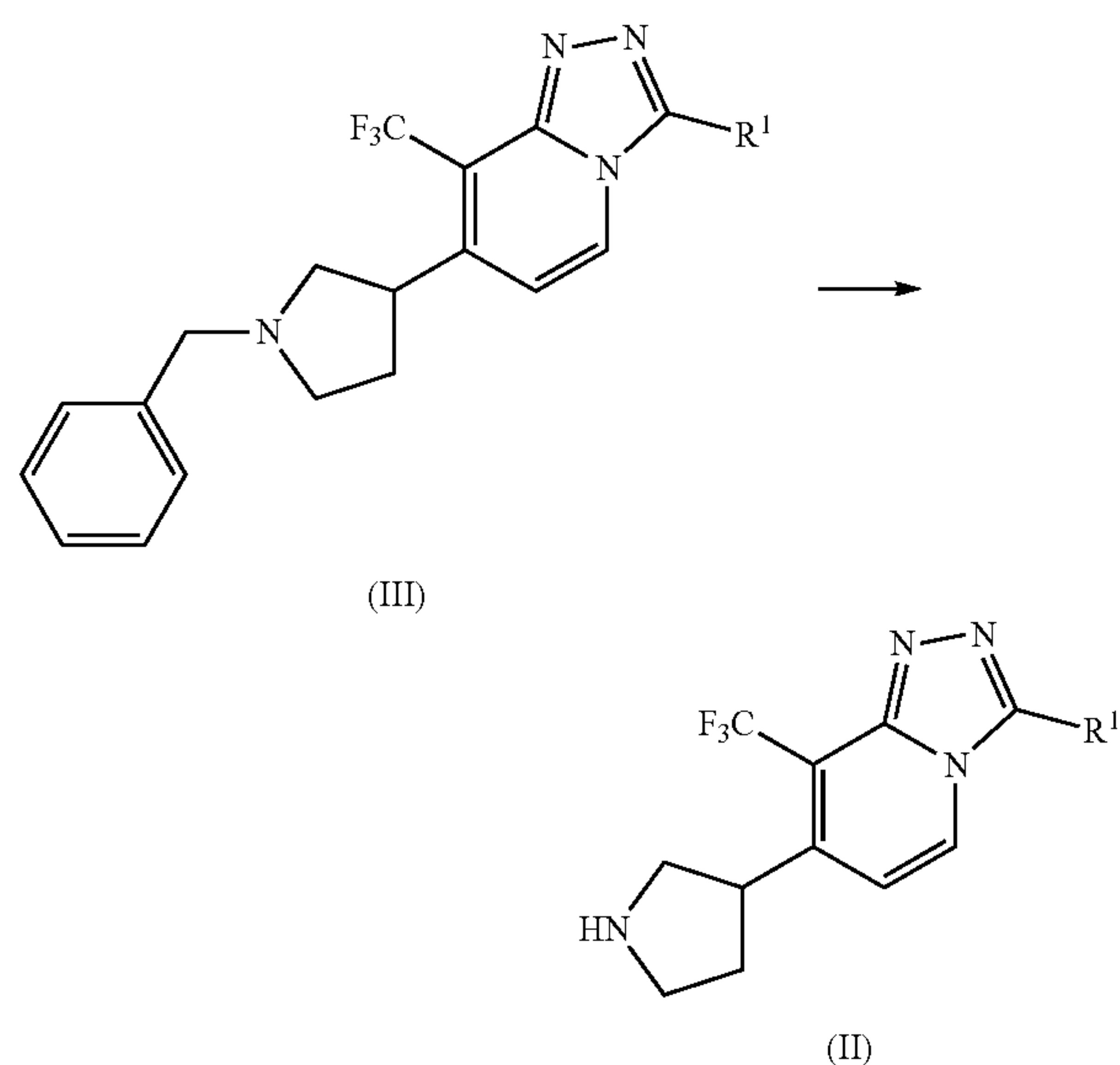
Reaction Scheme 2
