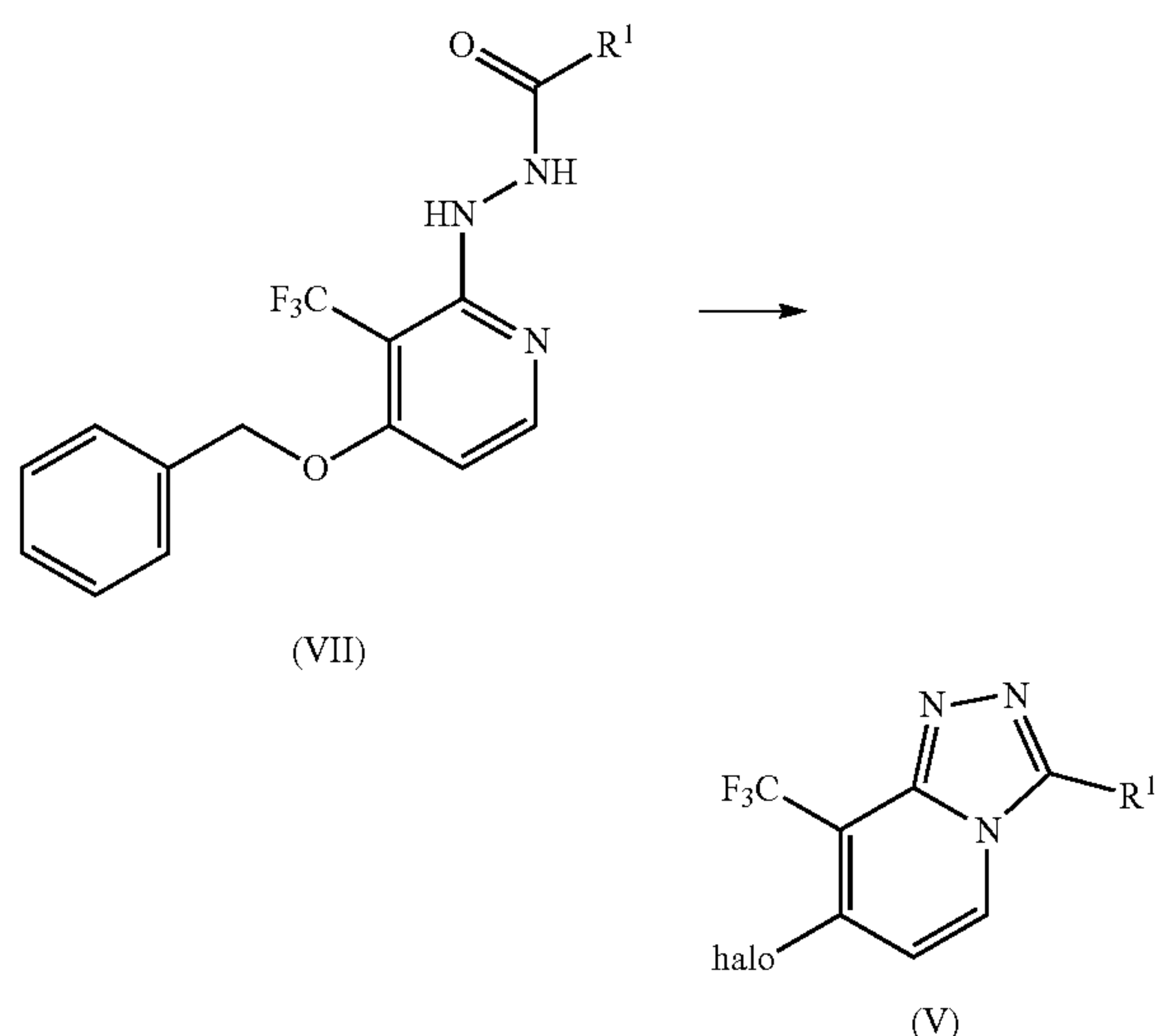
Reaction Scheme 5
