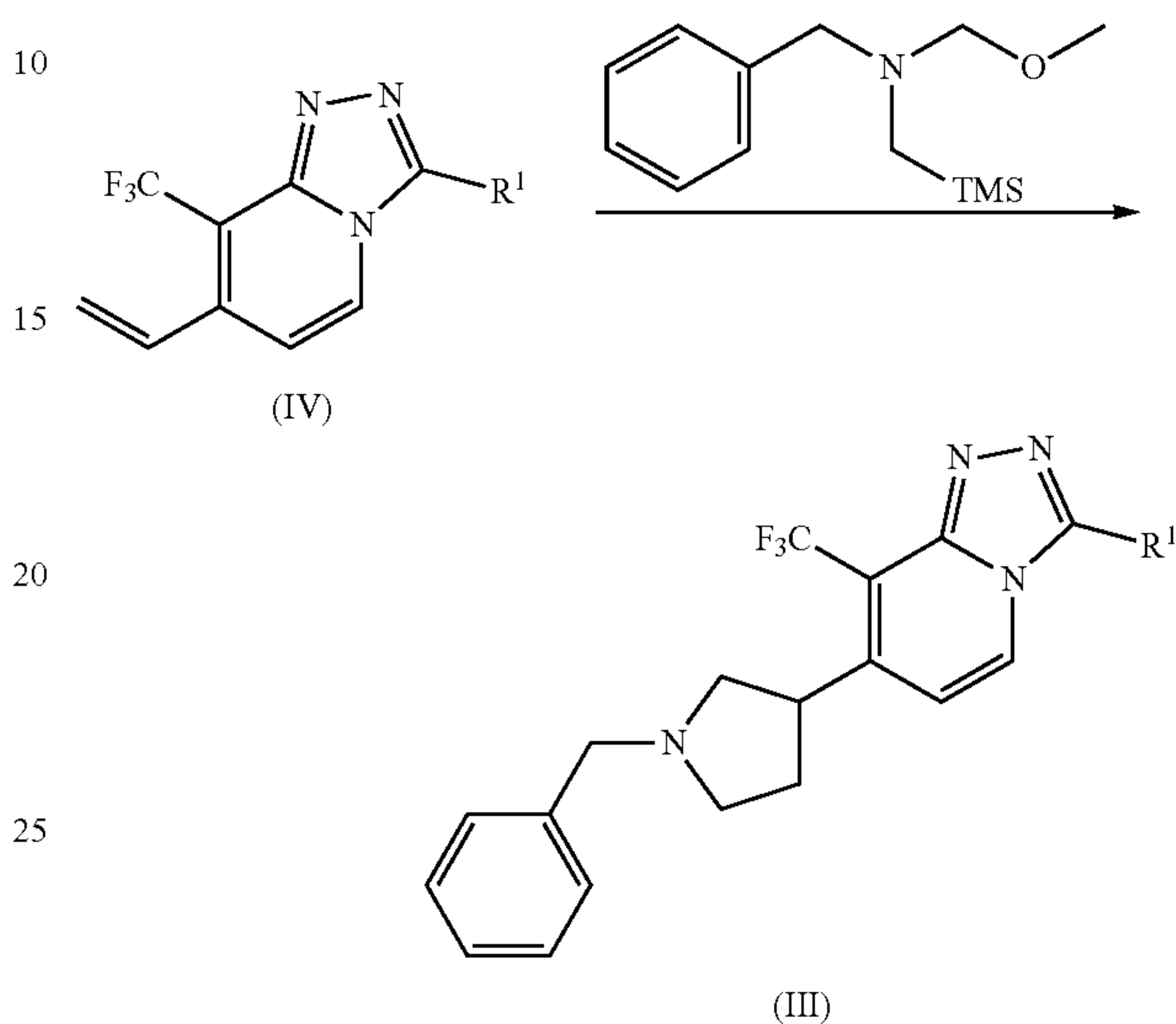
Reaction Scheme 3
