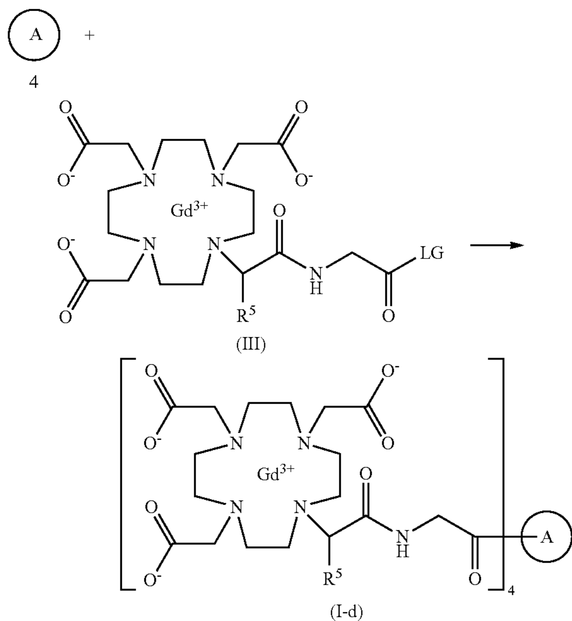
Scheme 4
