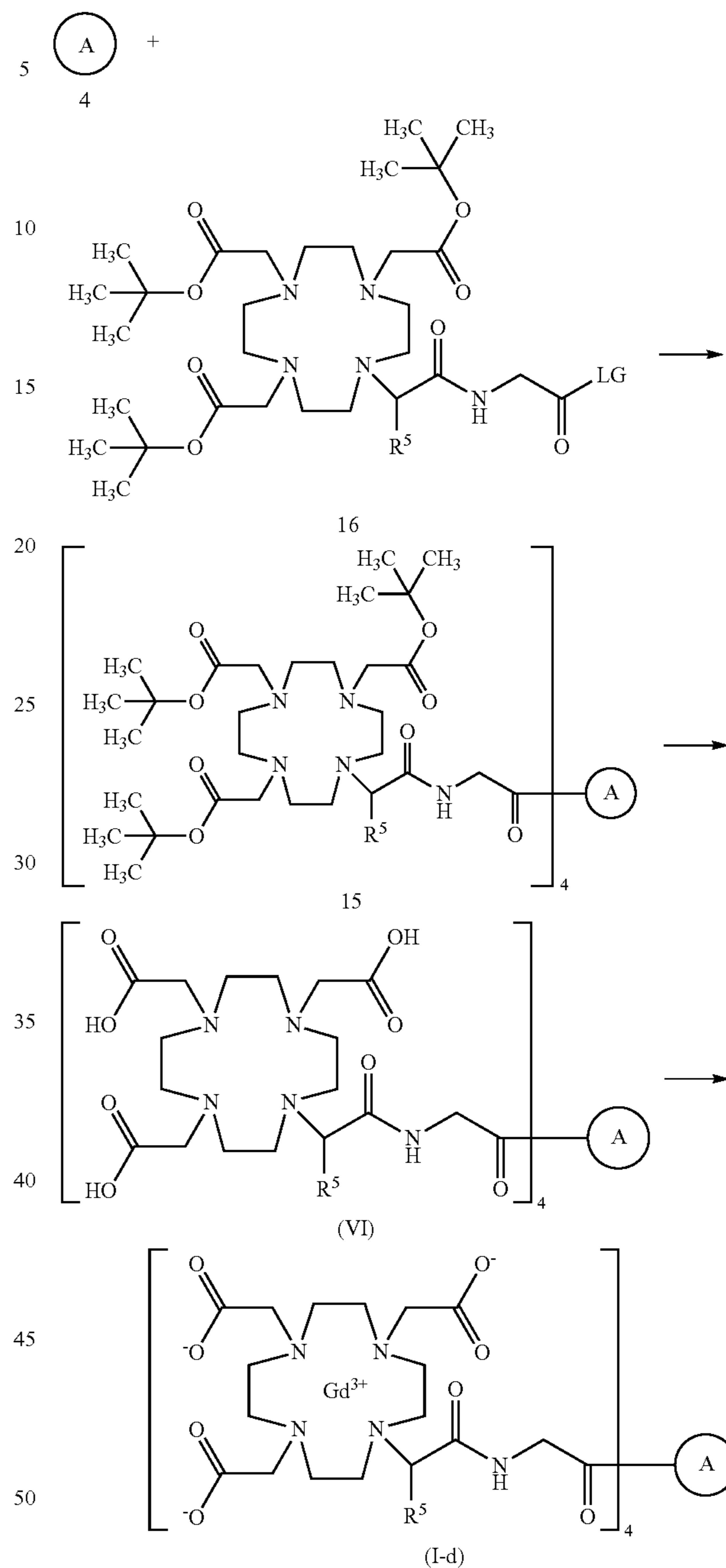
Scheme 12
