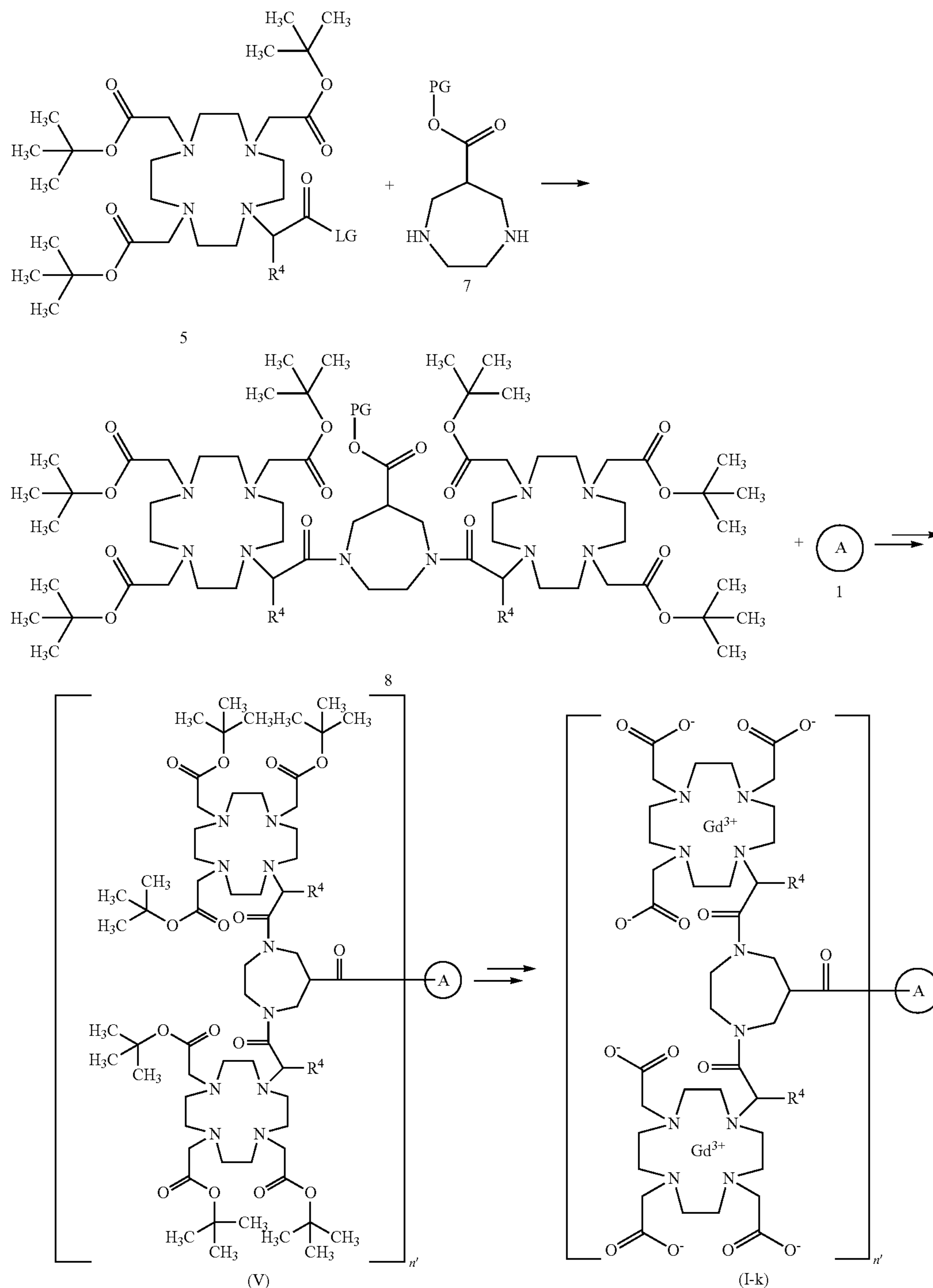
Scheme 9
