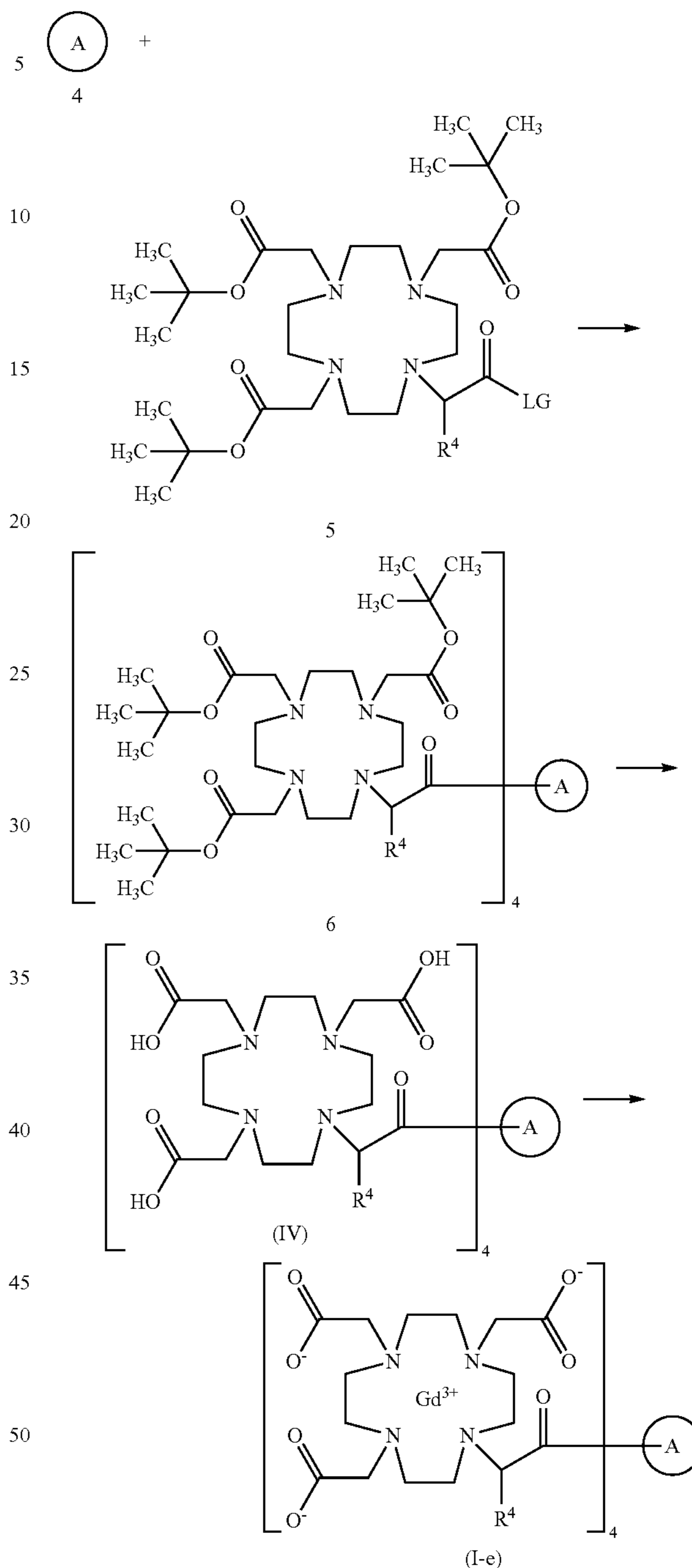
Scheme 5
