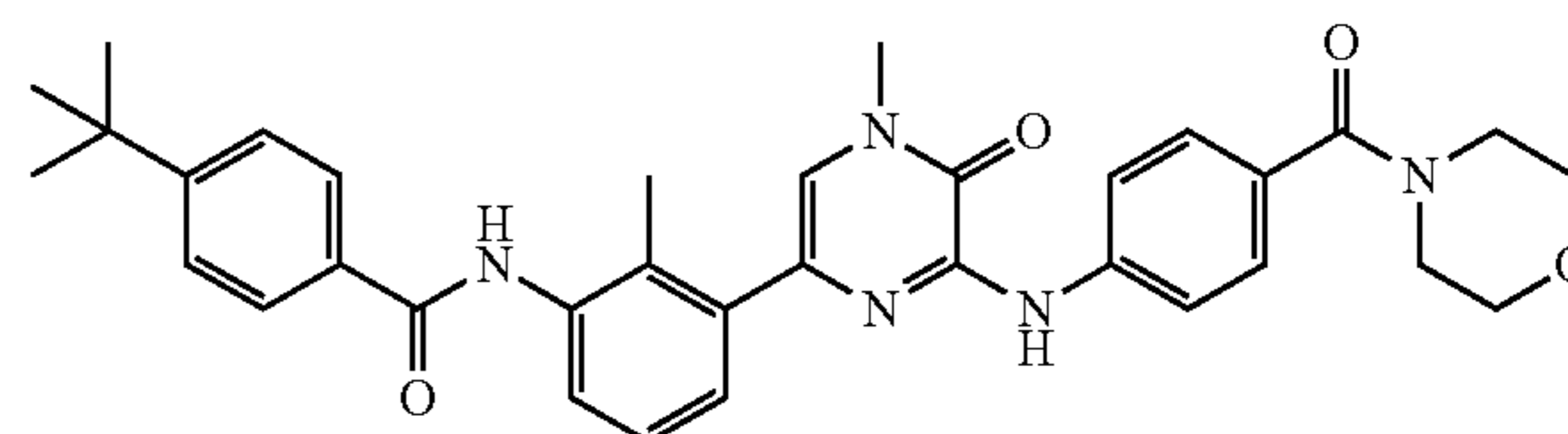
CGI-1746
