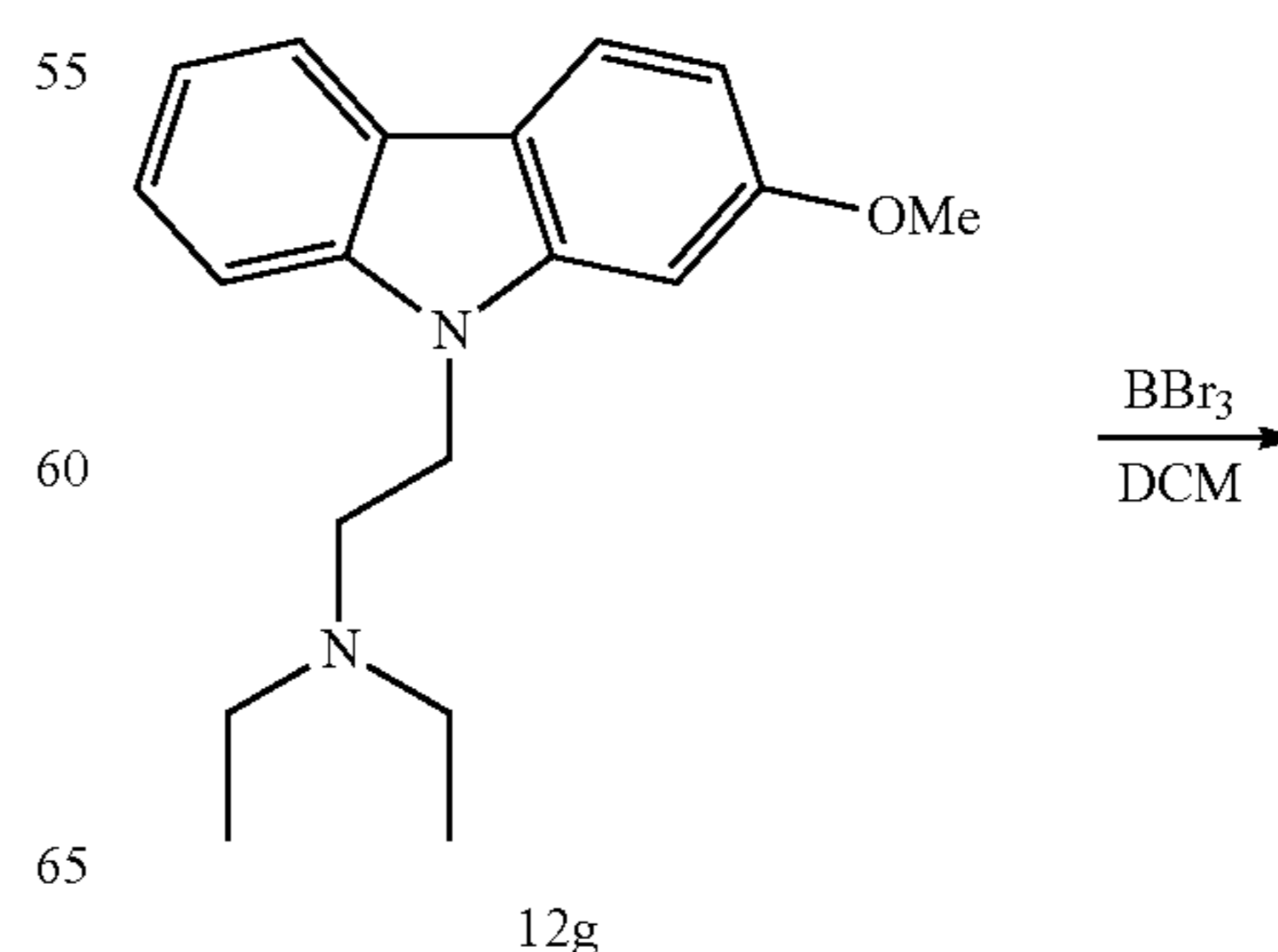
Scheme 9
