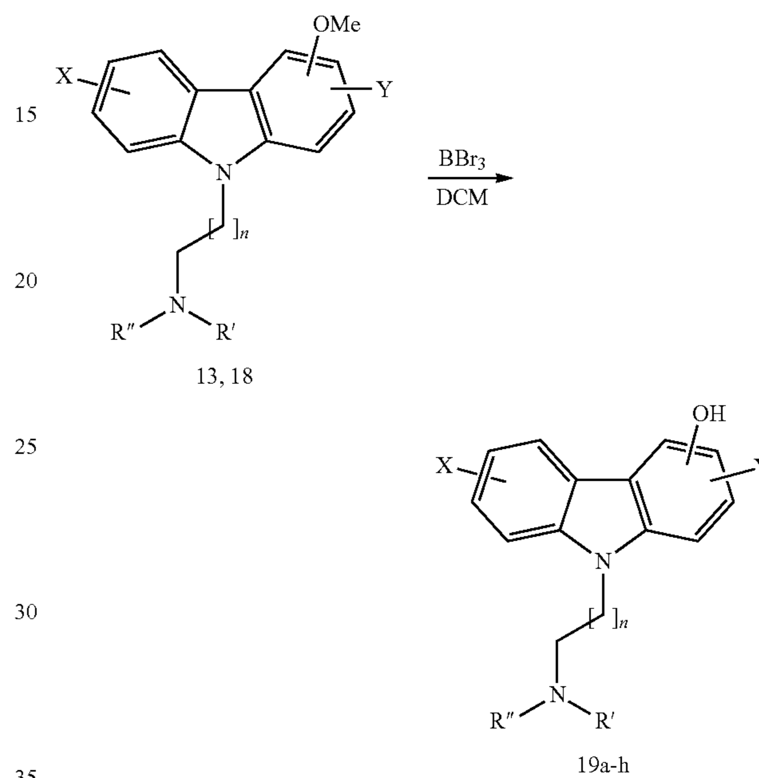
Scheme 8
