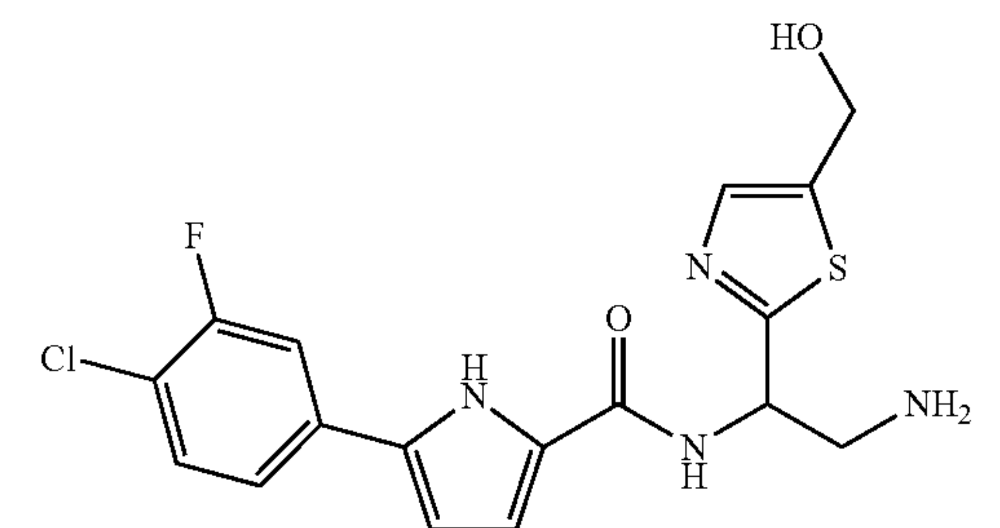
Compound 94 (Stereoisomer 1)
