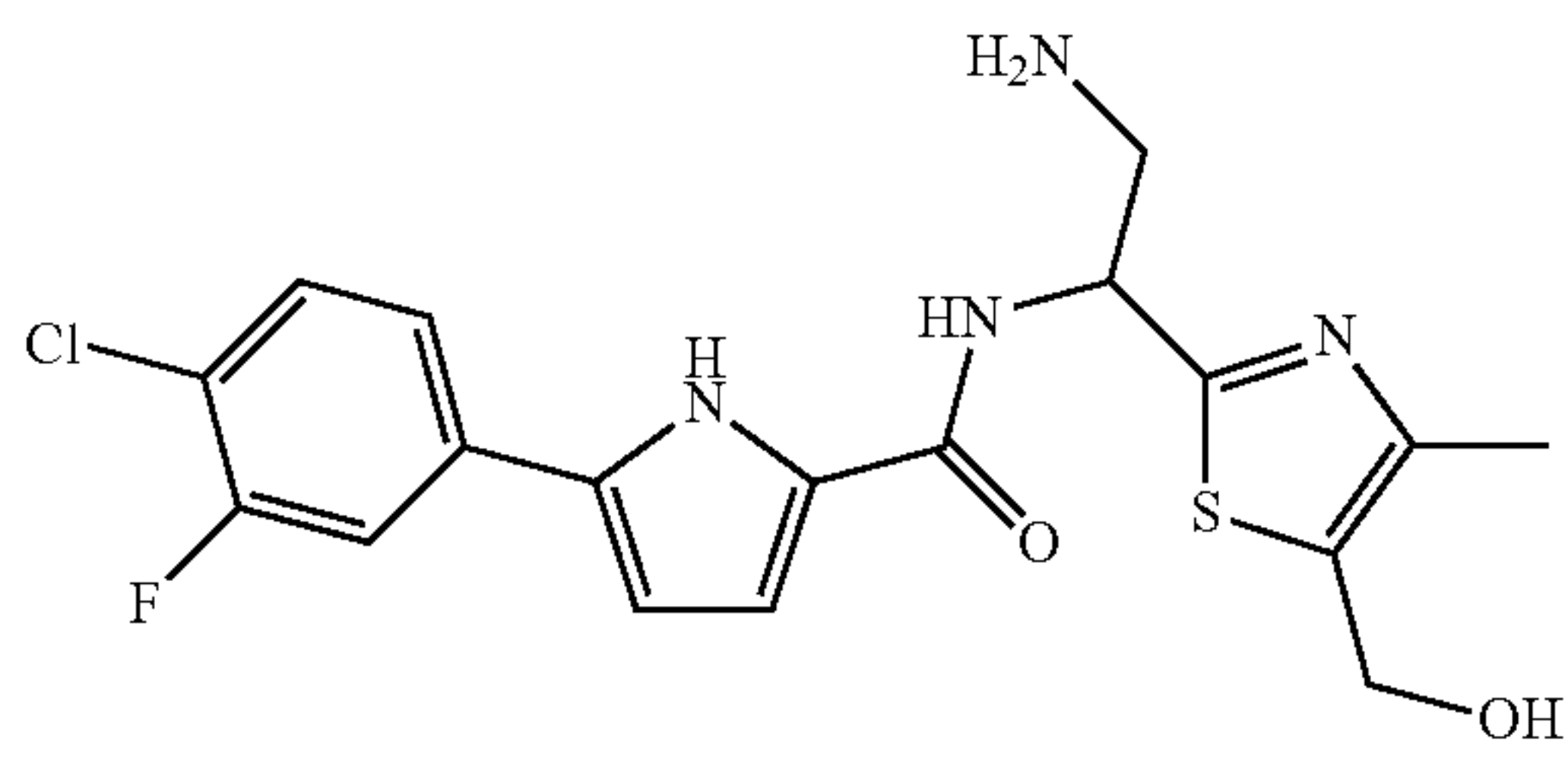
Compound 94 (Stereoisomer 1)
