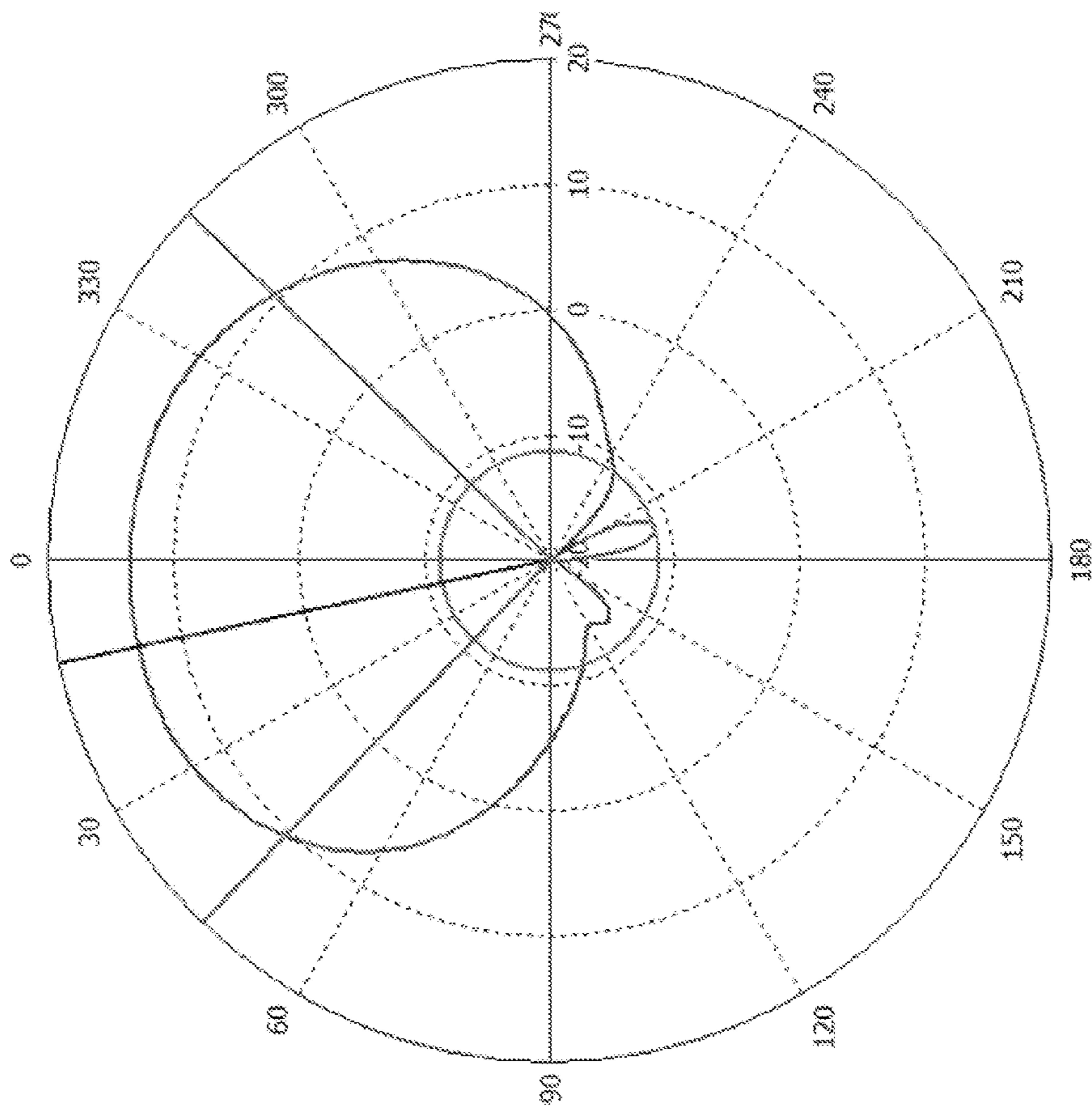
Farfield Directivity Copolar (Theta=90)
