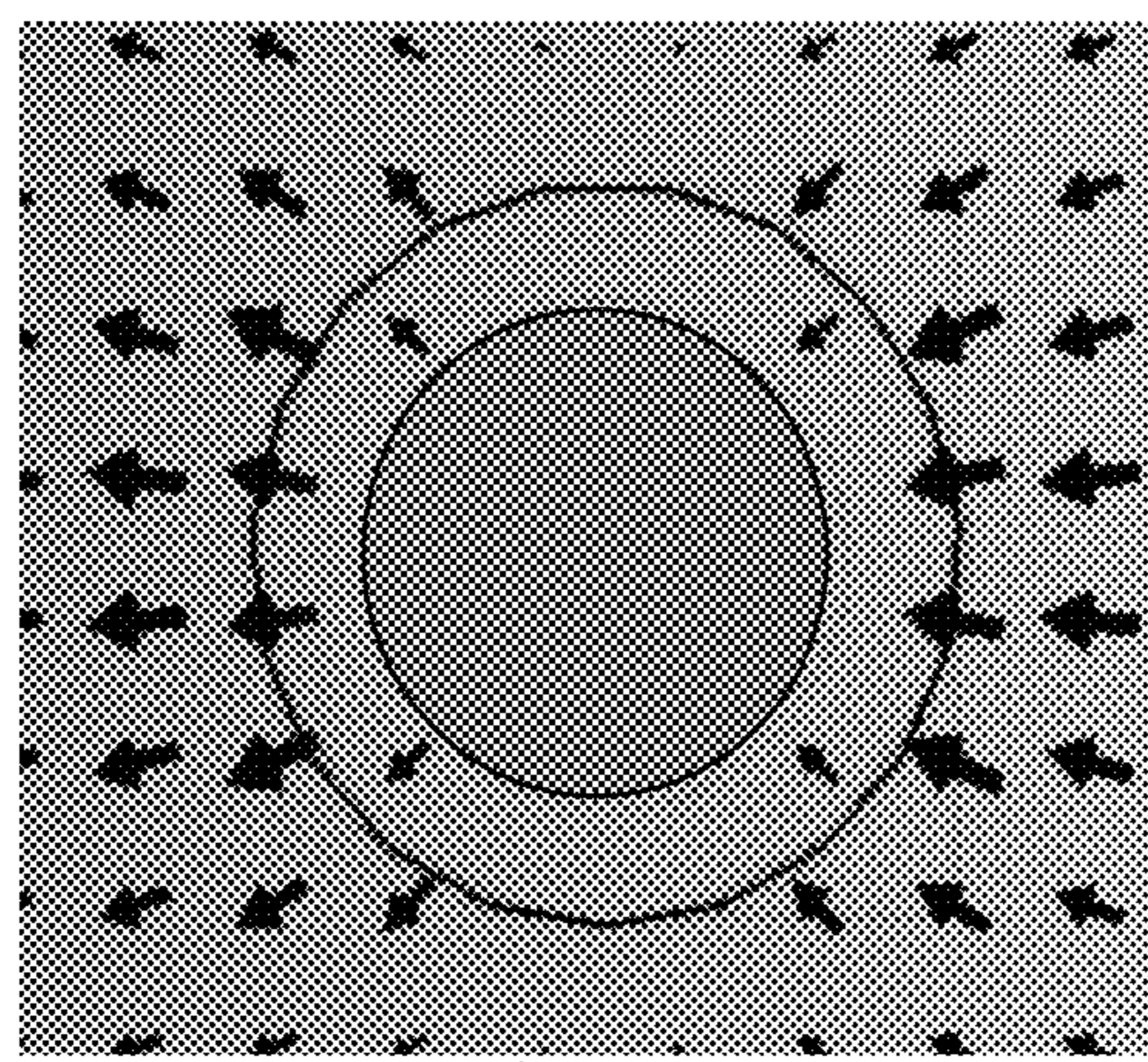
Hybrid mode (HE11) 2057
