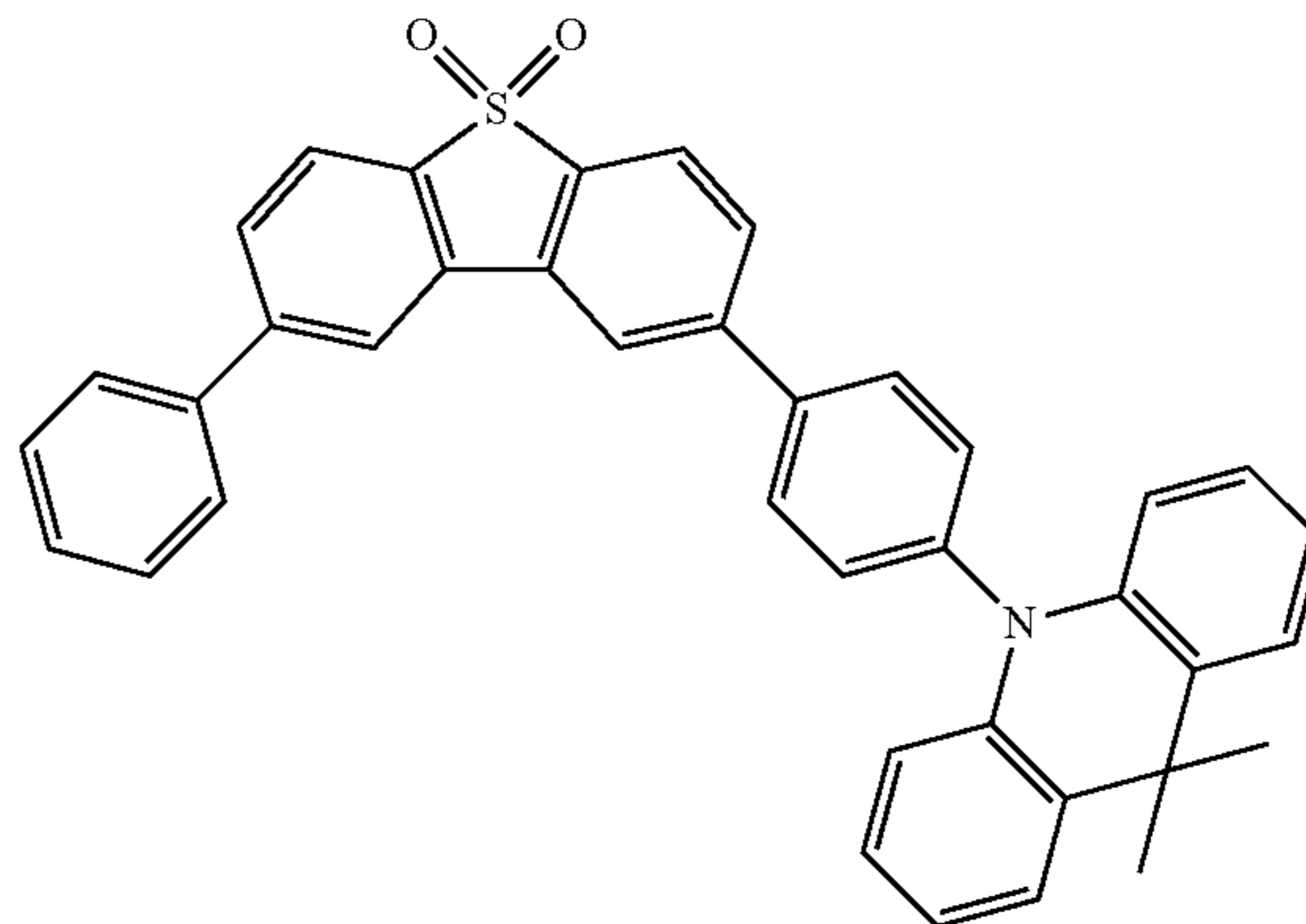
compound 3
