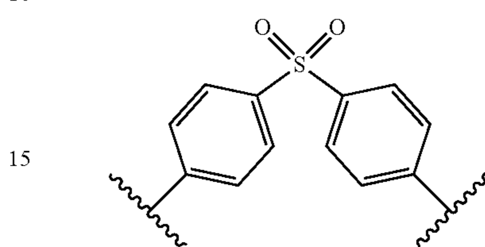
[Formula 2]
