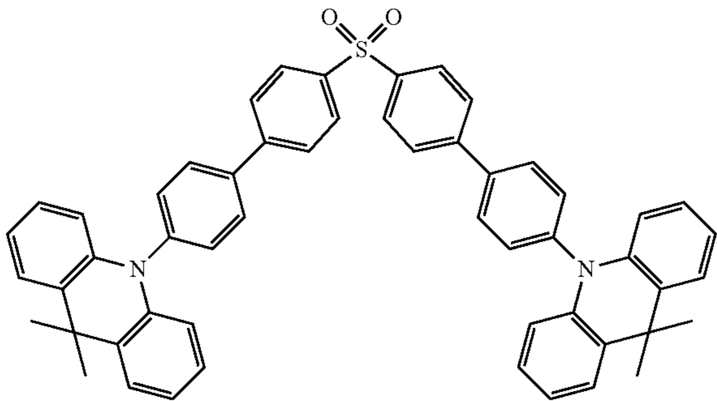
compound 14
