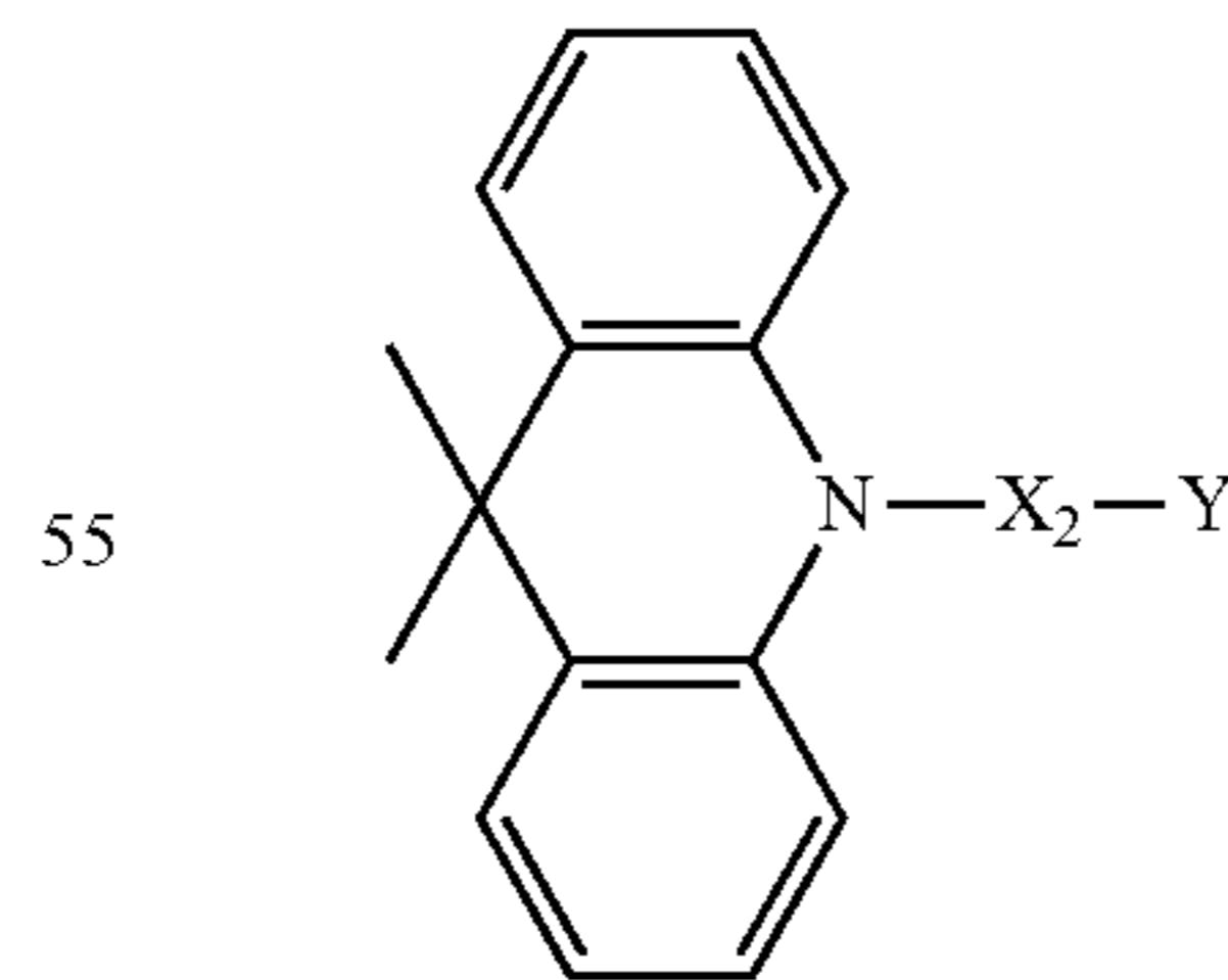
[Formula 1-2]
