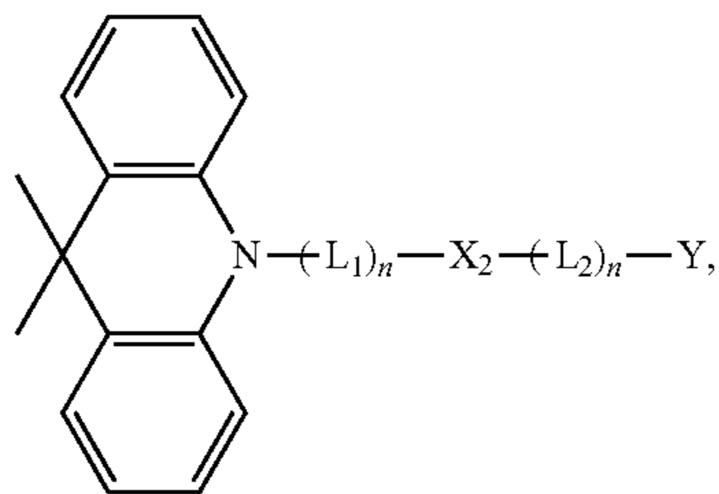
[Formula 2]
