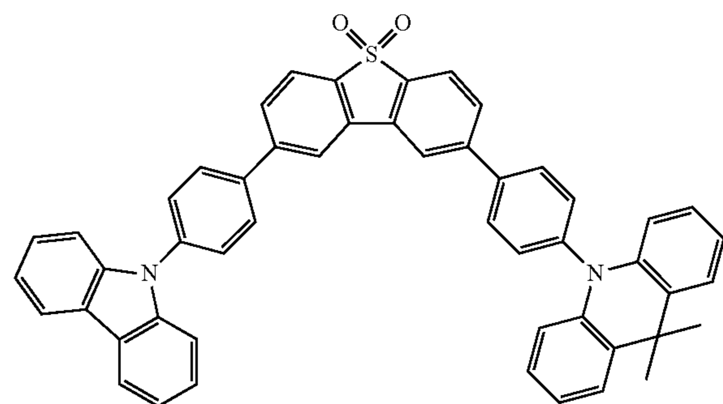
compound 12
