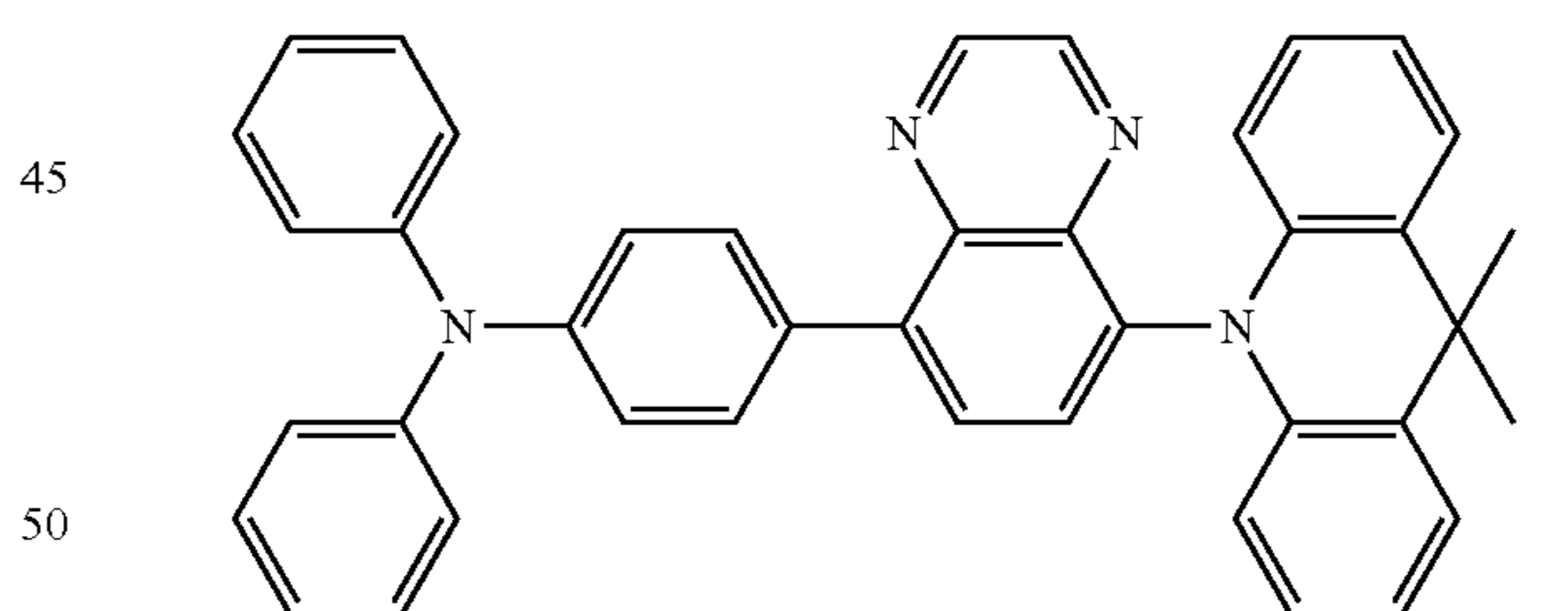
compound 30
