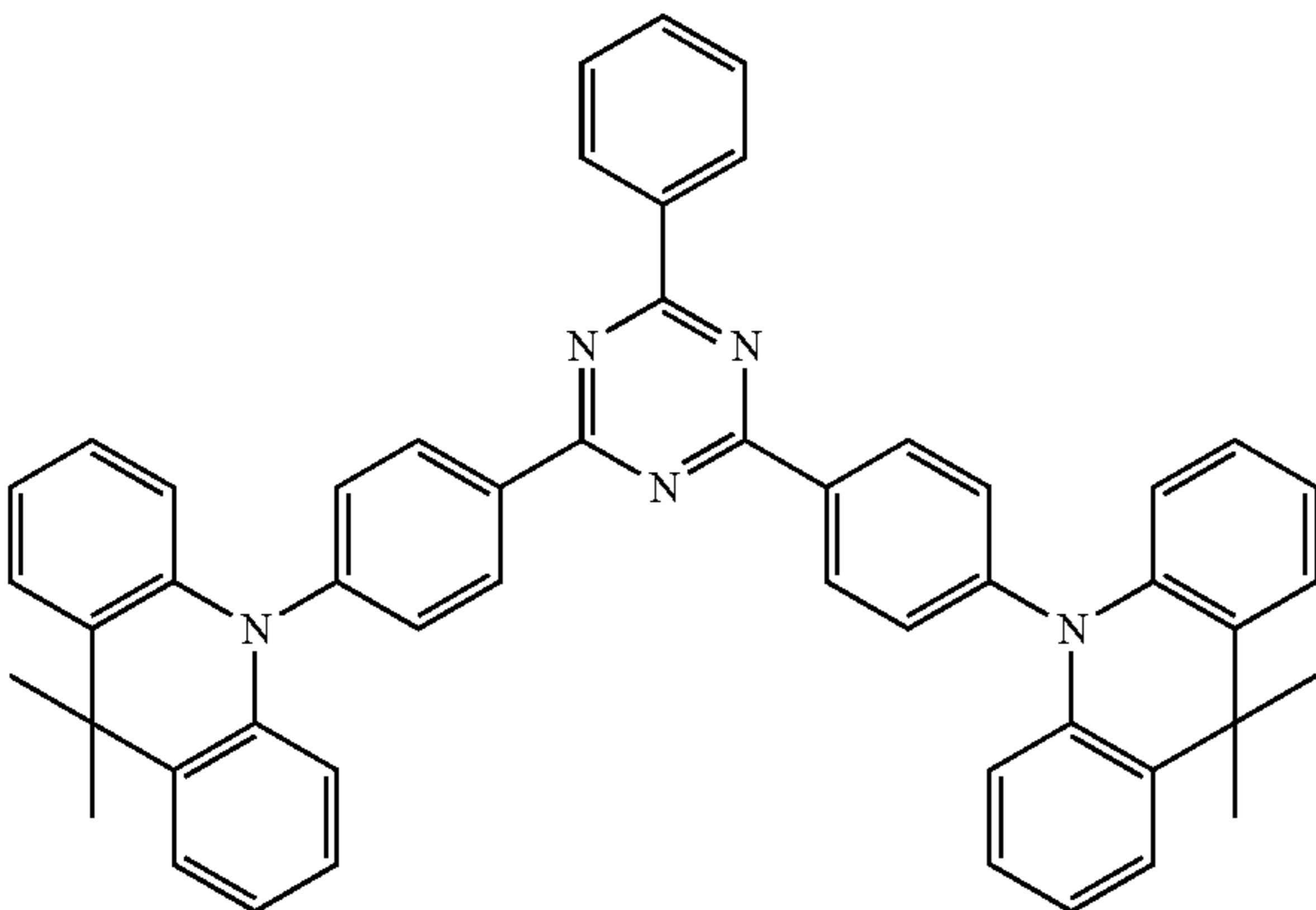
compound 15
