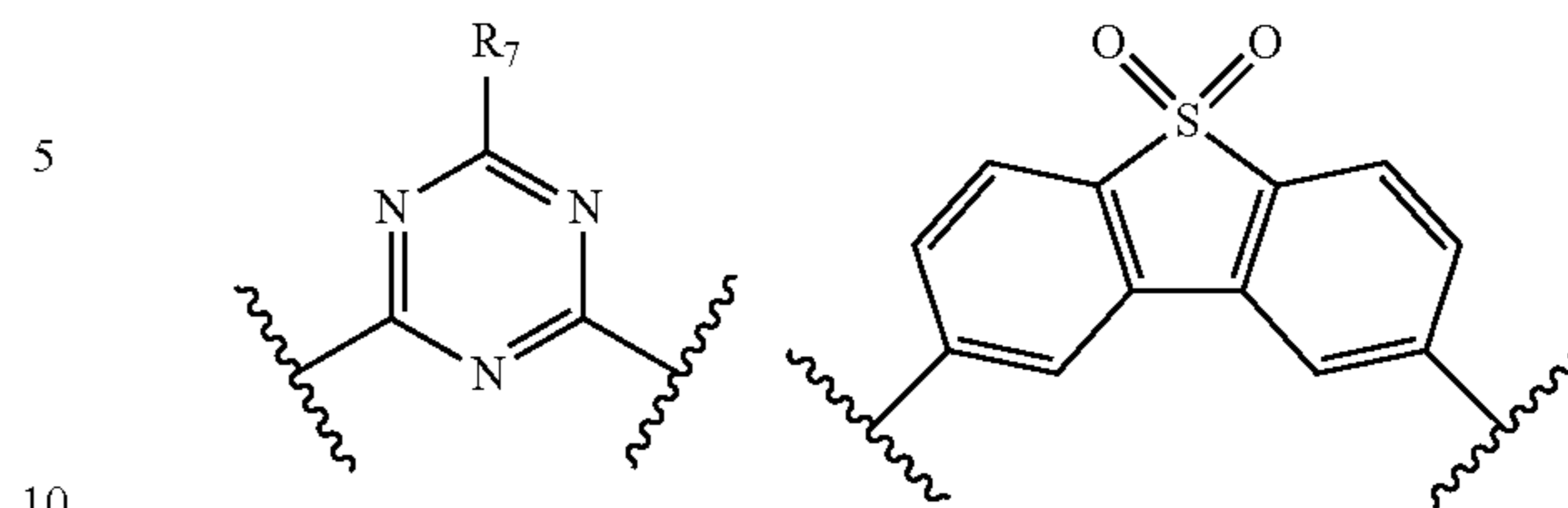
[Formula 1]
