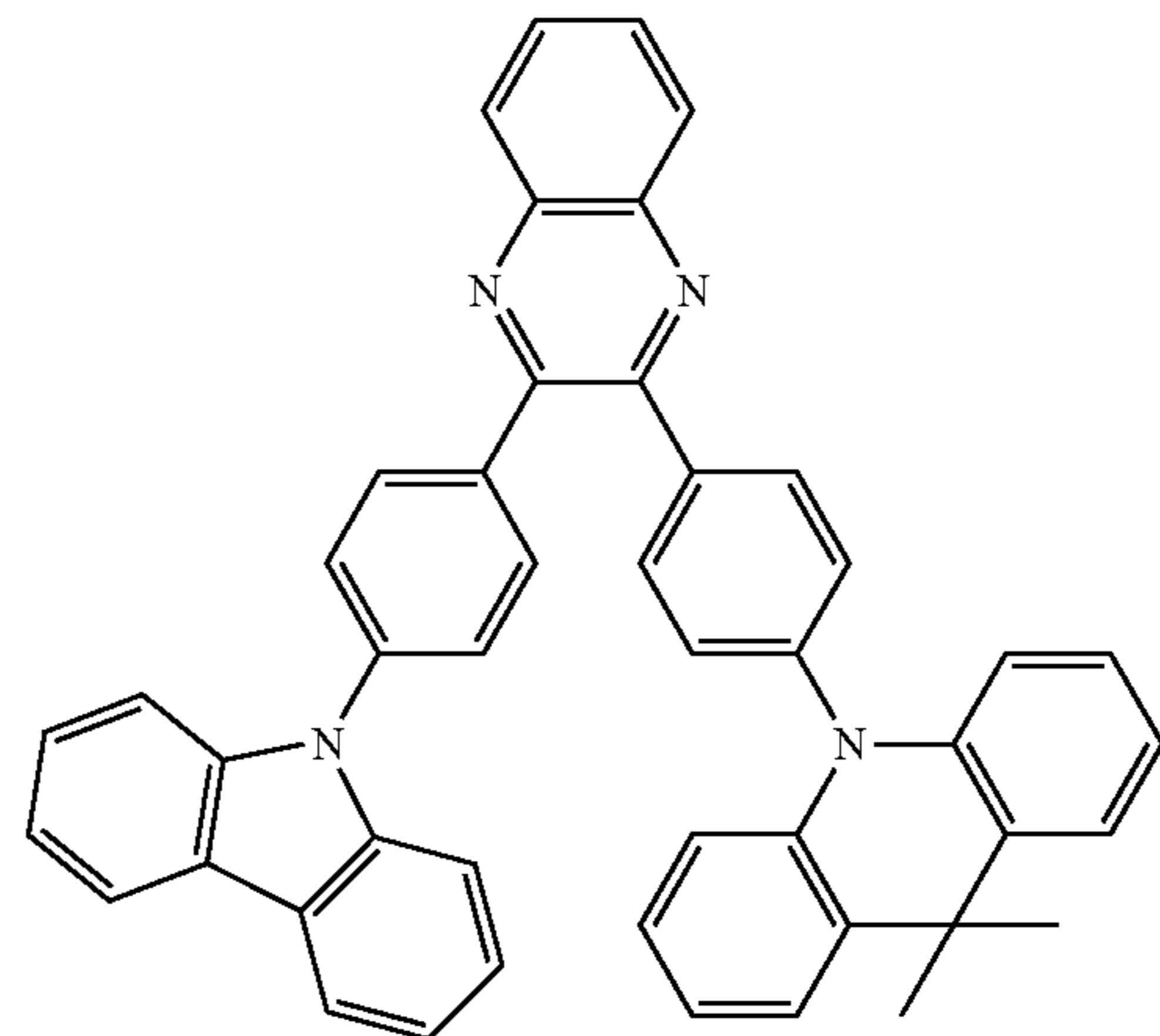
compound 19
