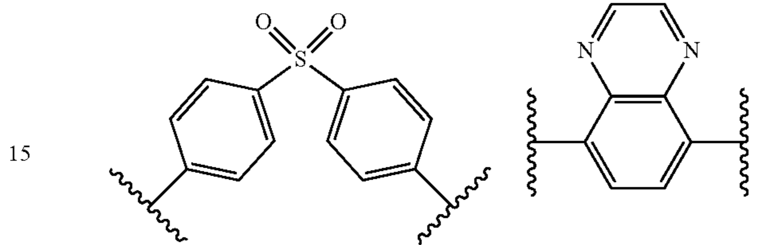
[Formula 2]
