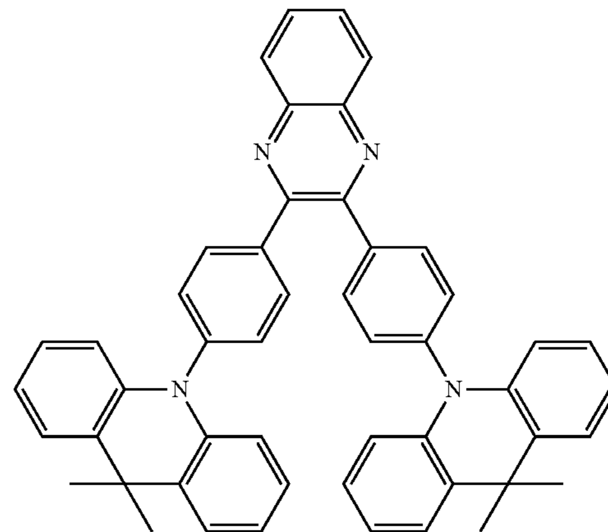
compound 18
