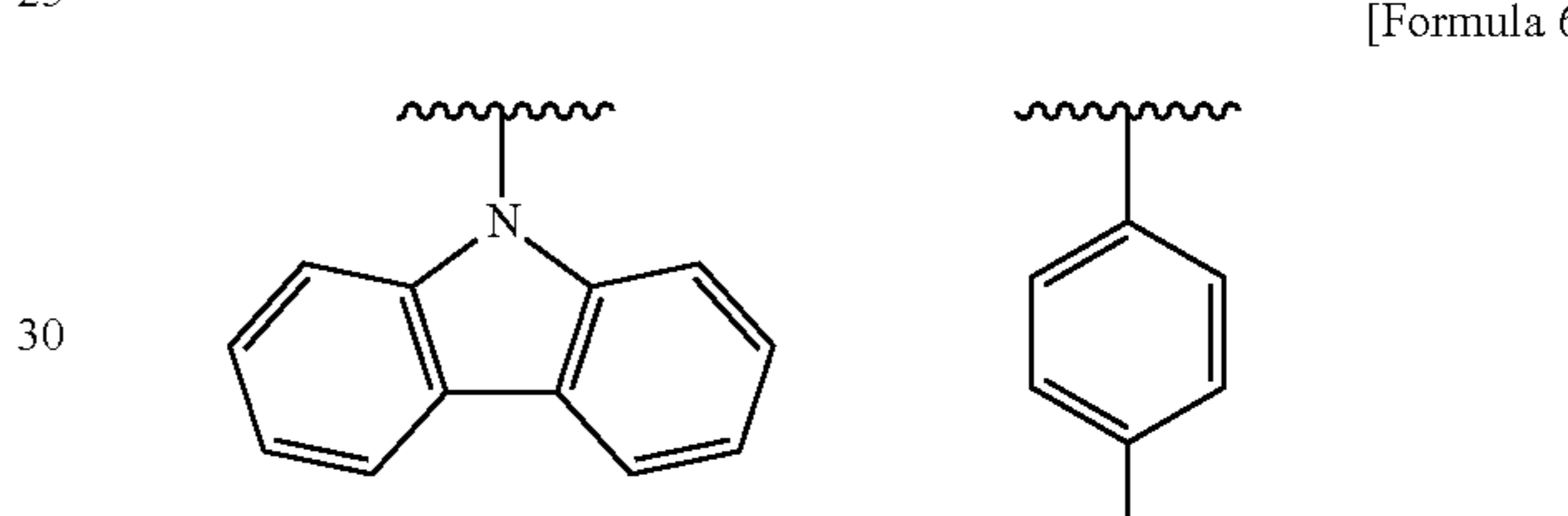
[Formula 6]
