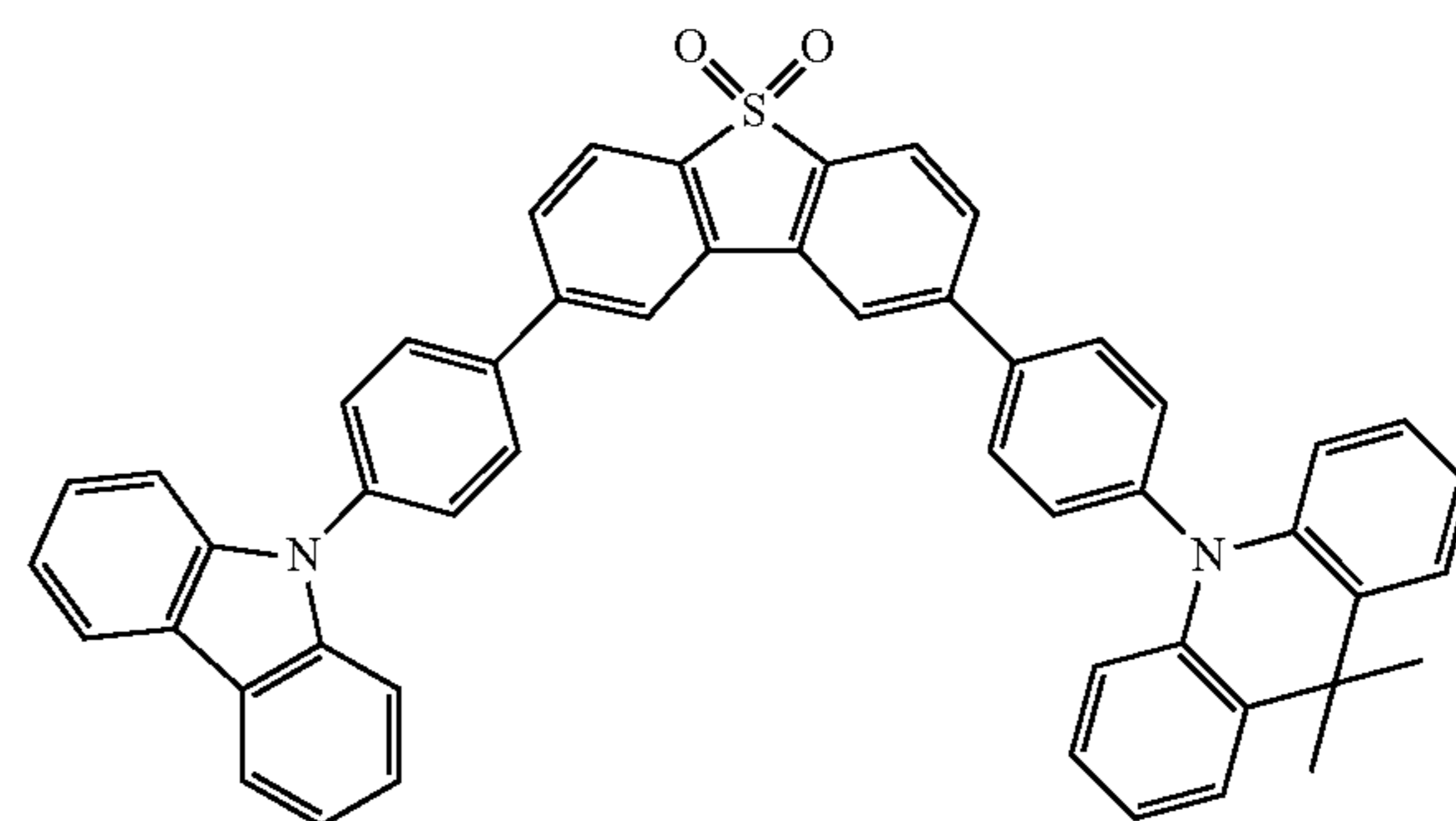
compound 12
