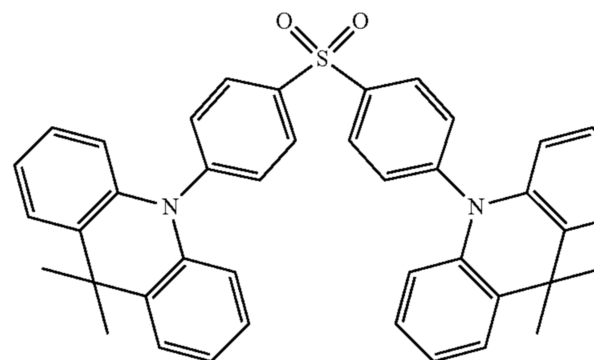
compound 20
