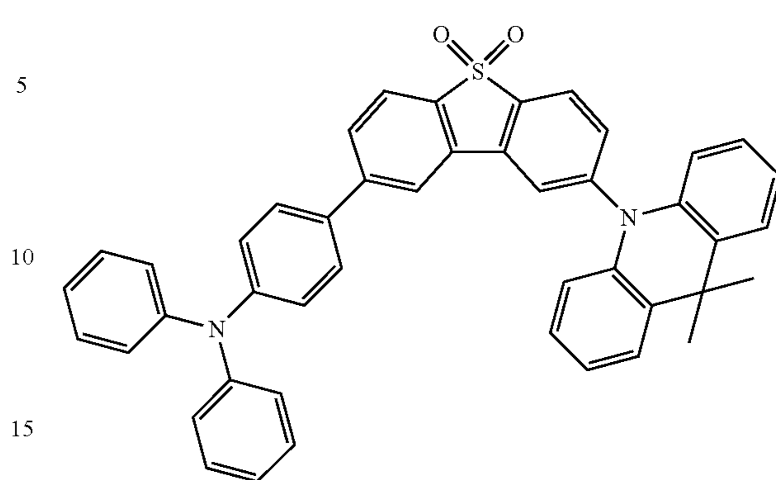
compound 27
