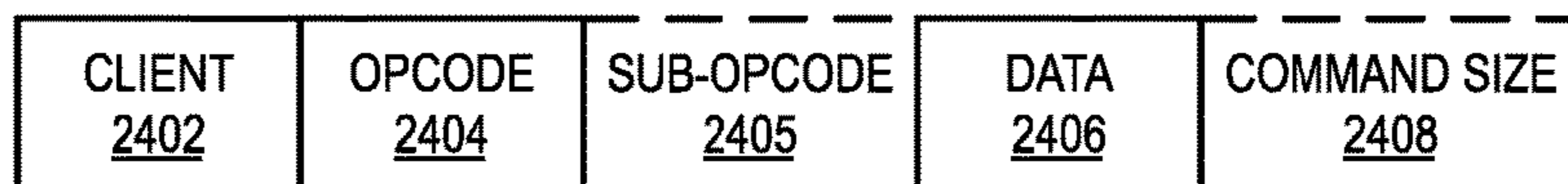
FIG. 24A GRAPHICS PROCESSOR COMMAND FORMAT 2400
