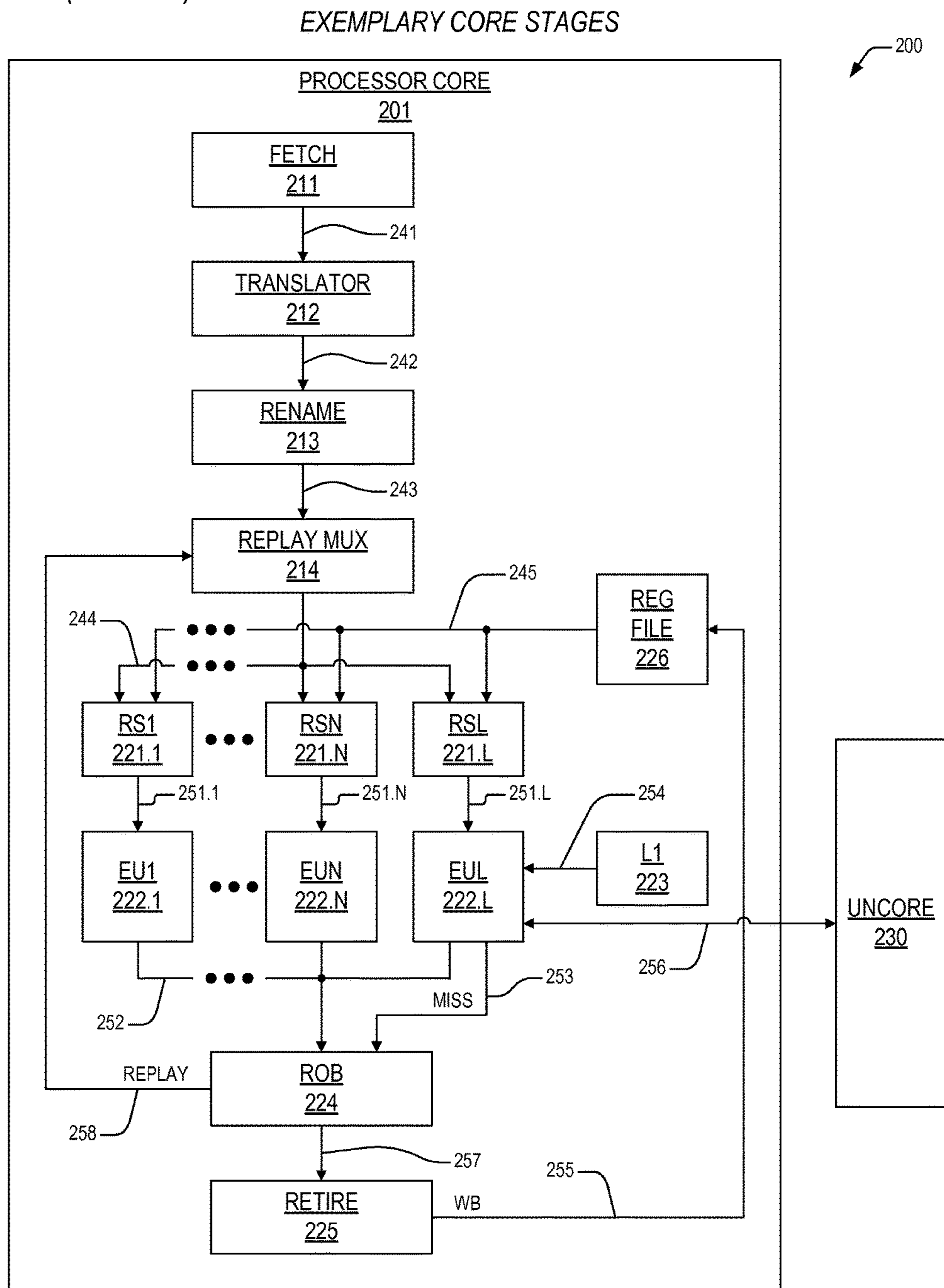
FIG. 2 (Prior Art)
