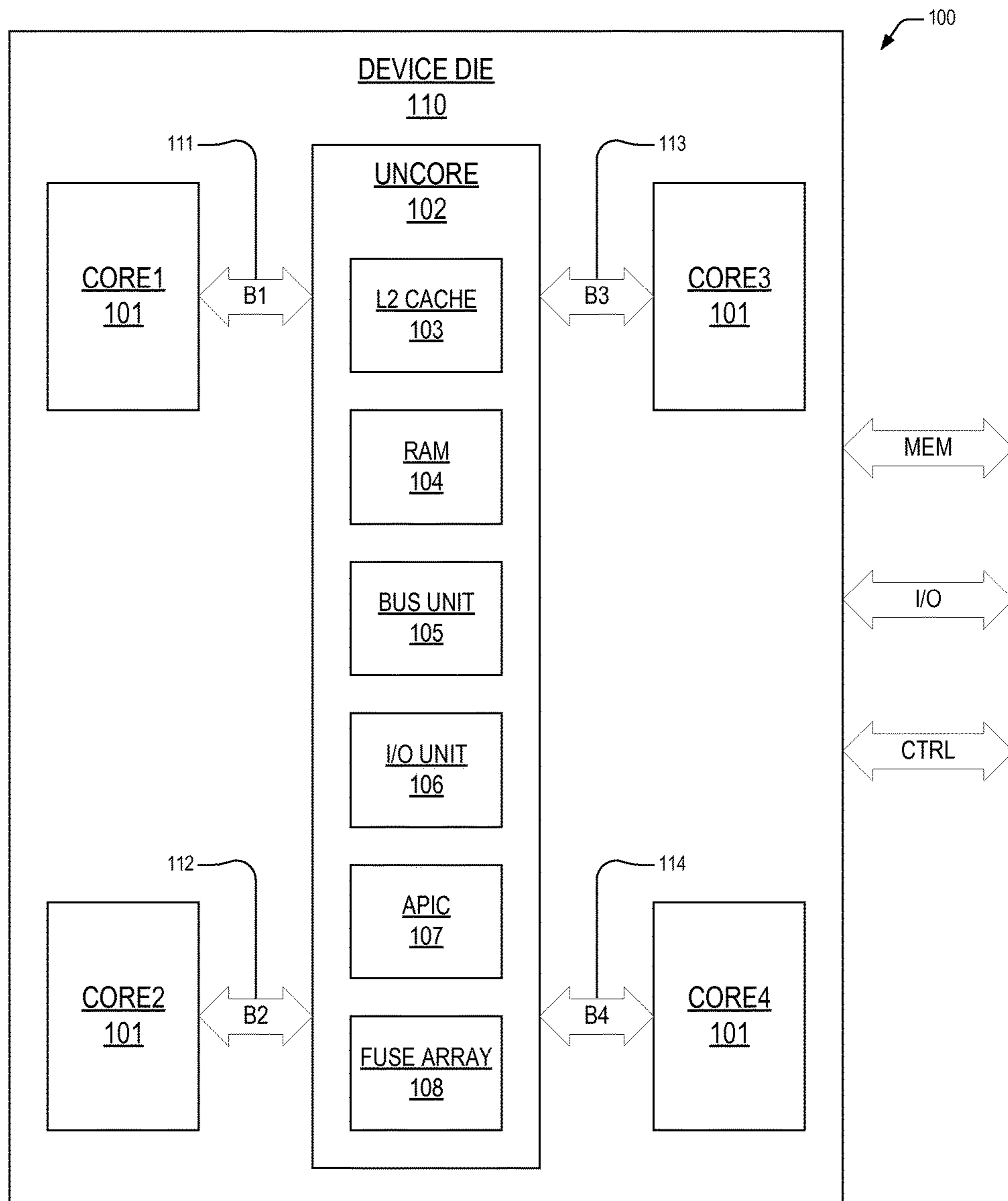
MULTI-CORE PROCESSOR WITH NON-CORE COMMON RESOURCES
