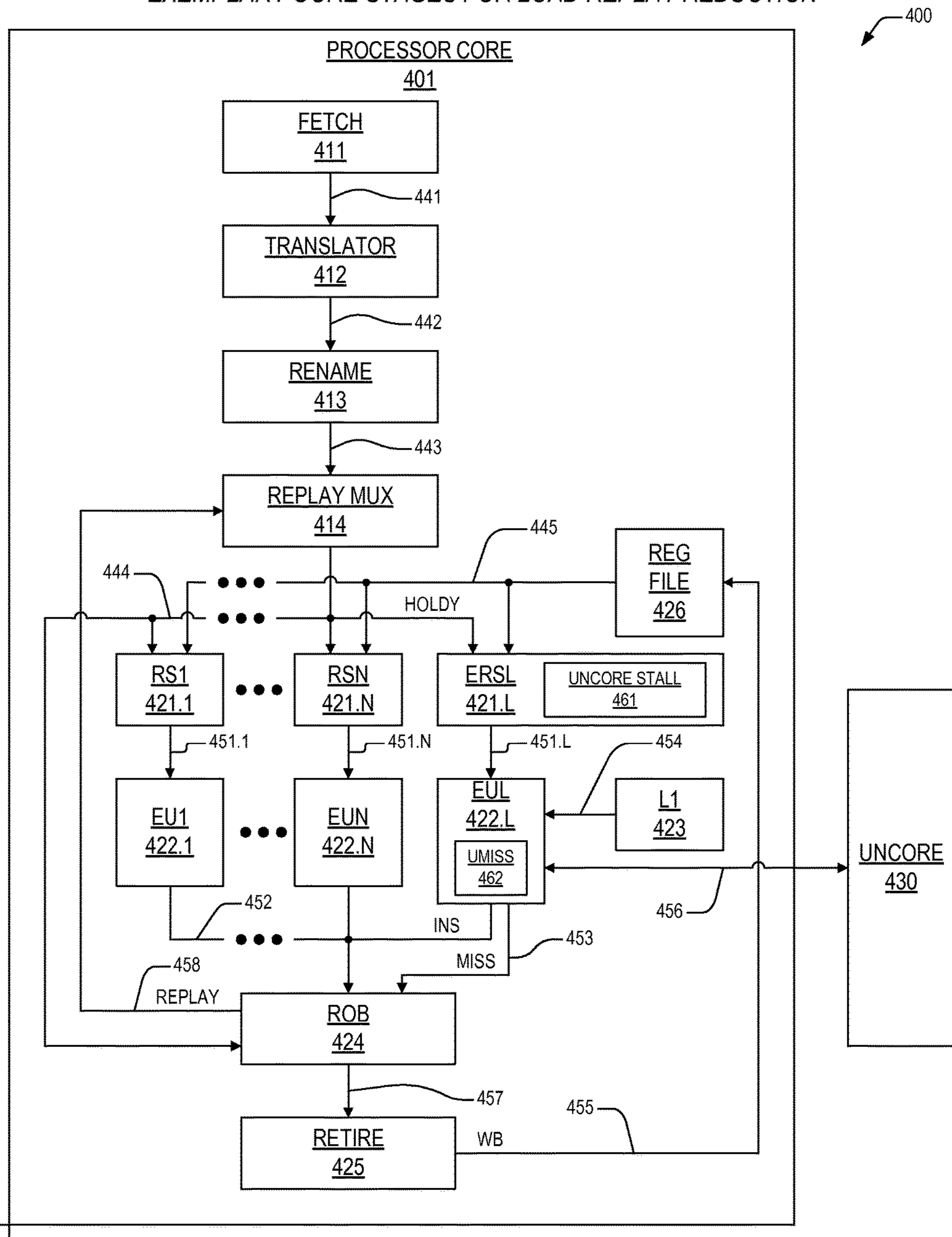
EXEMPLARY CORE STAGES FOR LOAD REPLAY REDUCTION
