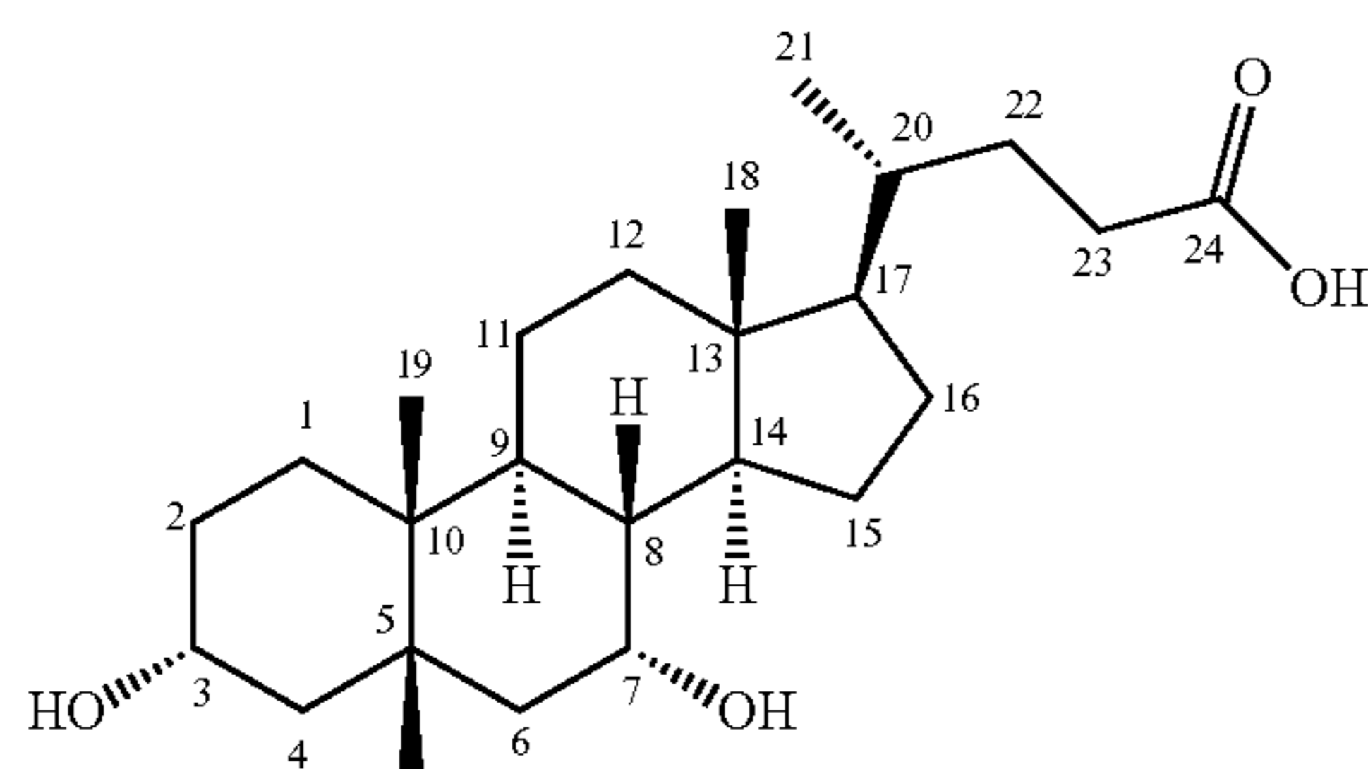
CDCA numbering
