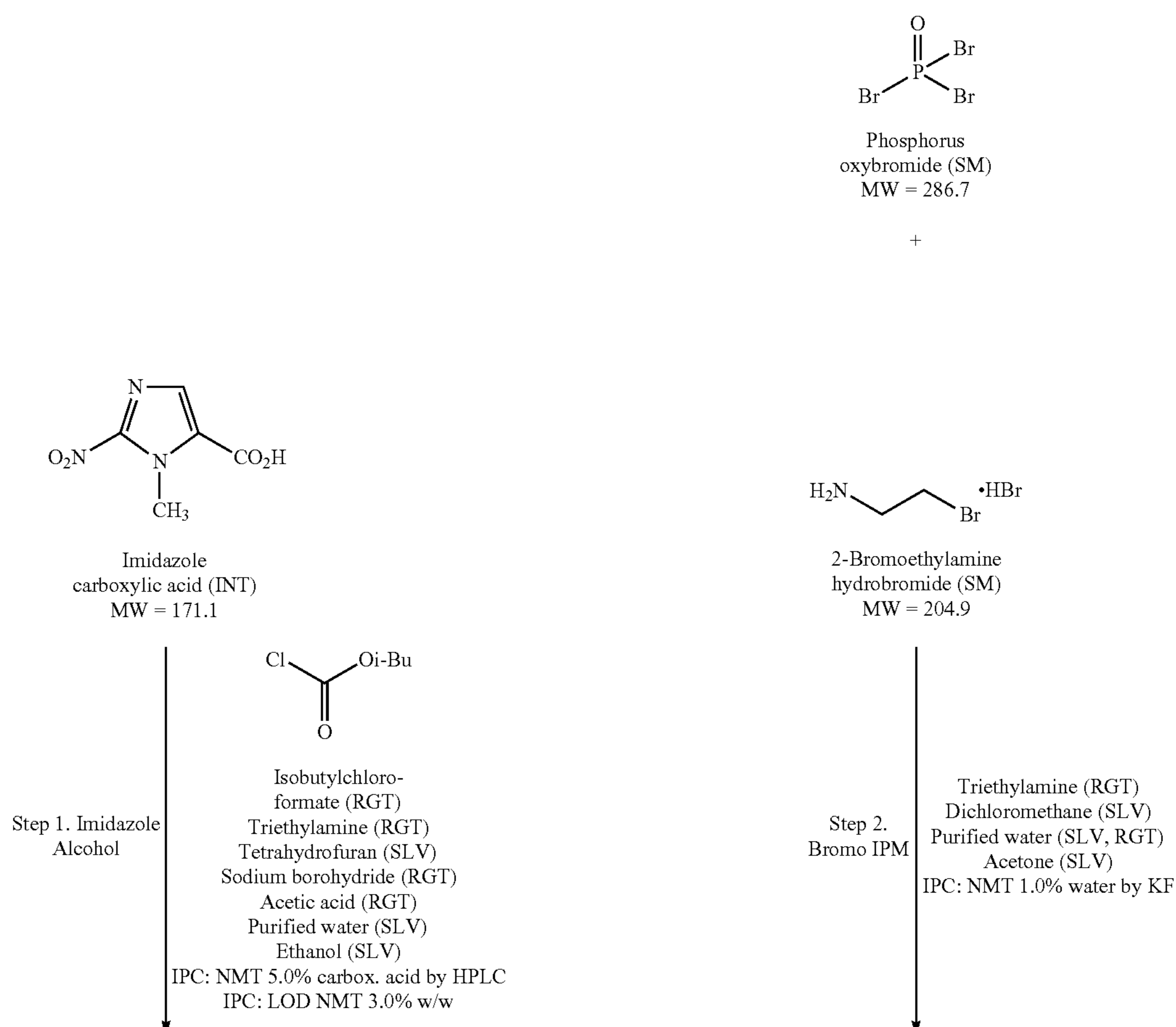
Scheme 2: Process for the Preparation of TH-302
