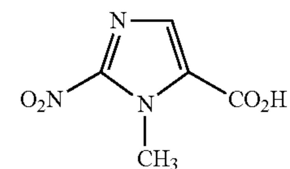
Imidazole carboxylic acid (INT) MW = 171.1
