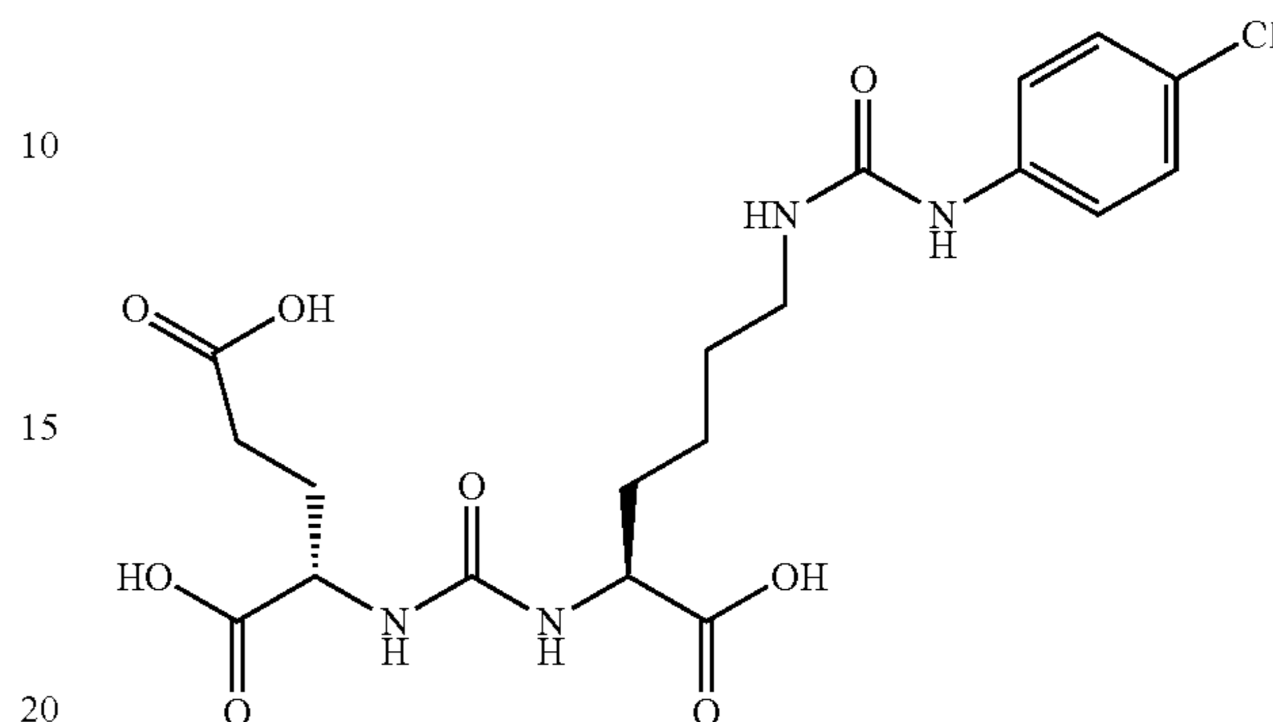
2-(3-{1-Carboxy-5-[3-(4-bromo-phenyl)-ureido]-pentyl}-ureido)-pentanedioic acid (12) (MIP 1129)
