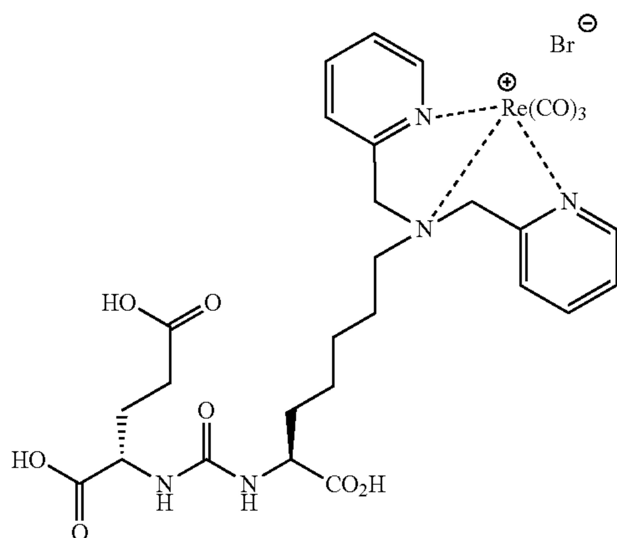
2-{3-[1-Carboxy-5-(carboxymethyl-pyridin-2-ylmethyl-amino)-pentyl]ureido}-pentanedioic acid (26)
