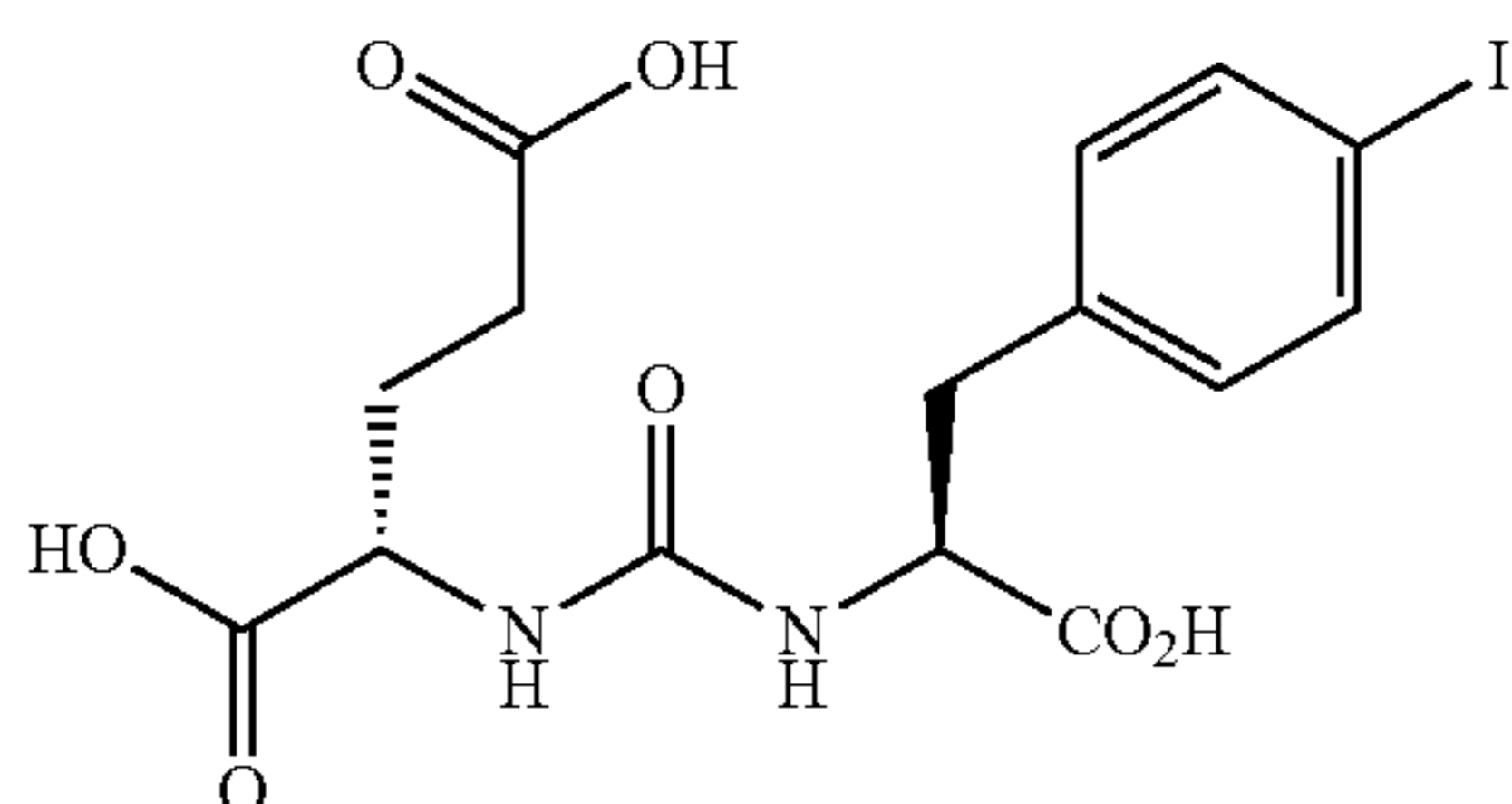
(S,S)-2-{3-[1-Carboxy-5-(2-iodo-benzylamino)-pentyl]-ureido}-pentanedioic acid (12) (MIP 1035)
