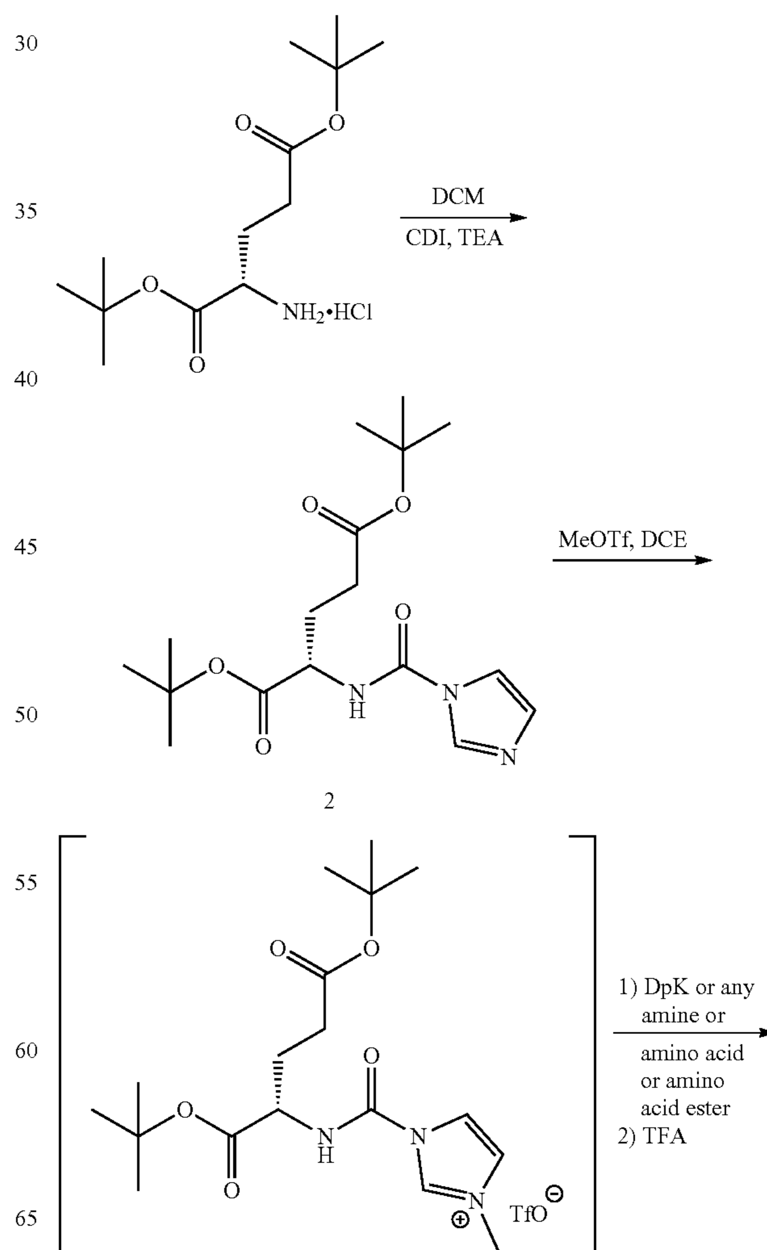
Scheme 1. General pathway for the synthesis of PSMA compounds.
