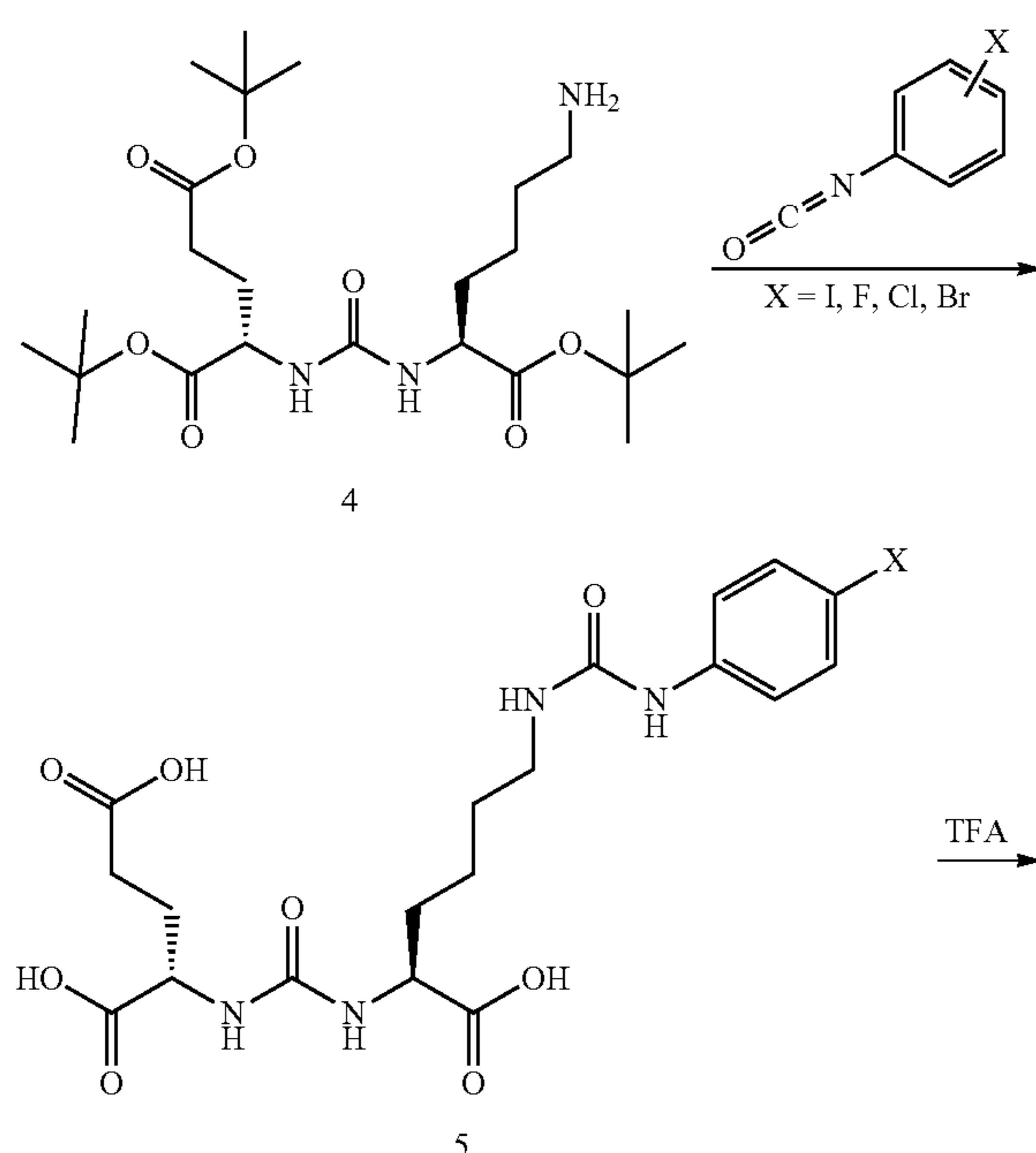
Scheme B. General pathway for the synthesis of halogenated Glu-Urea-Ureido(Phenyl-X) analogs.
