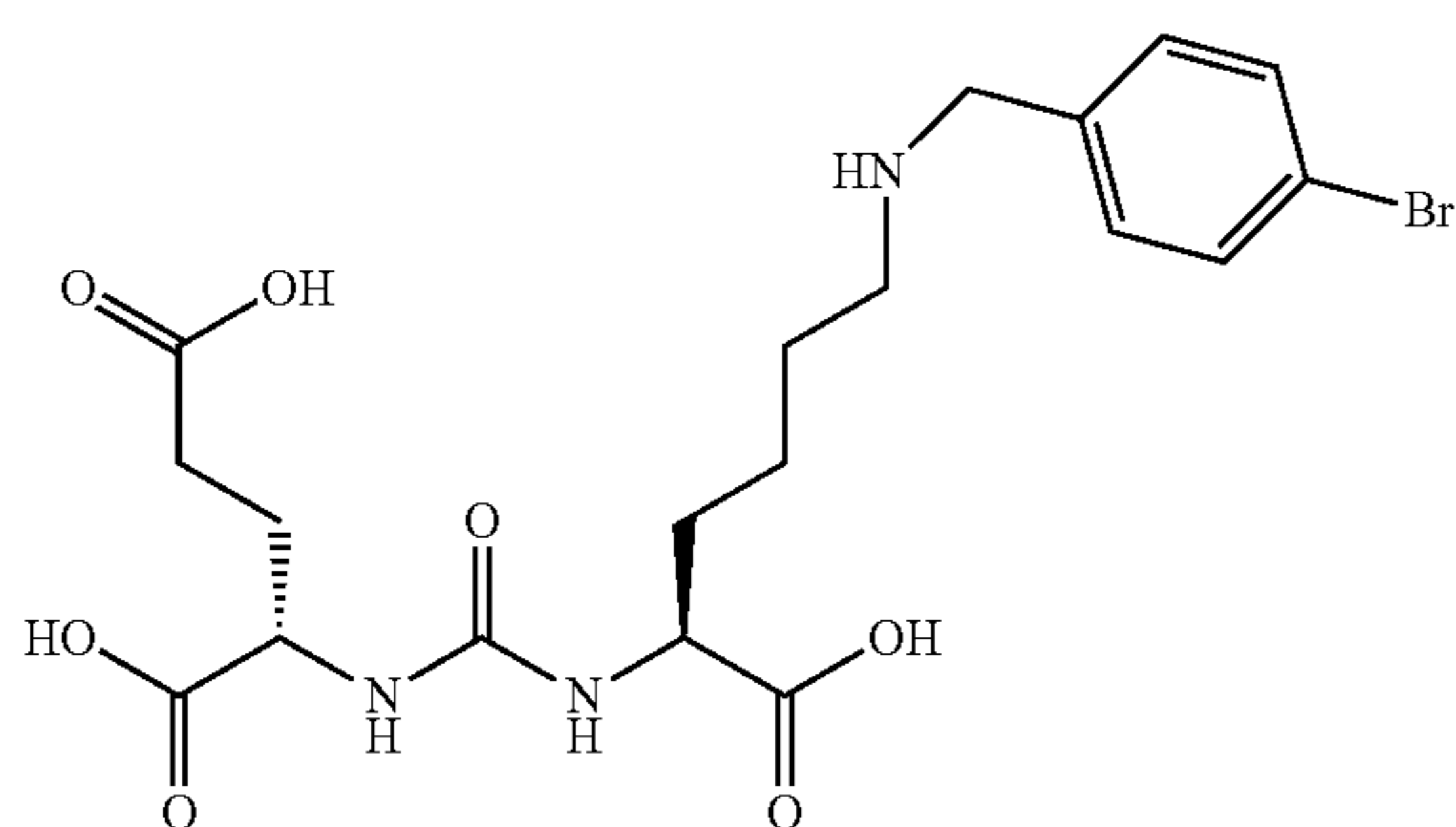
(S,S)-2-{3-[1-Carboxy-5-(4-iodo-benzoylamino)-pentyl]-ureido}-pentanedioic acid (17) (MIP 1044)
