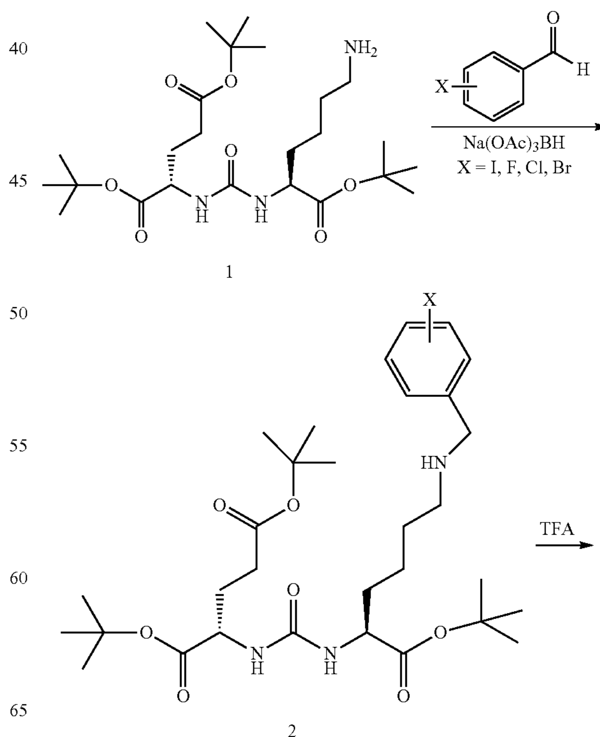
Scheme A. General pathway for the synthesis of halogenated Glu-Urea-Lys(N-benzyl-X) analogs (3).
