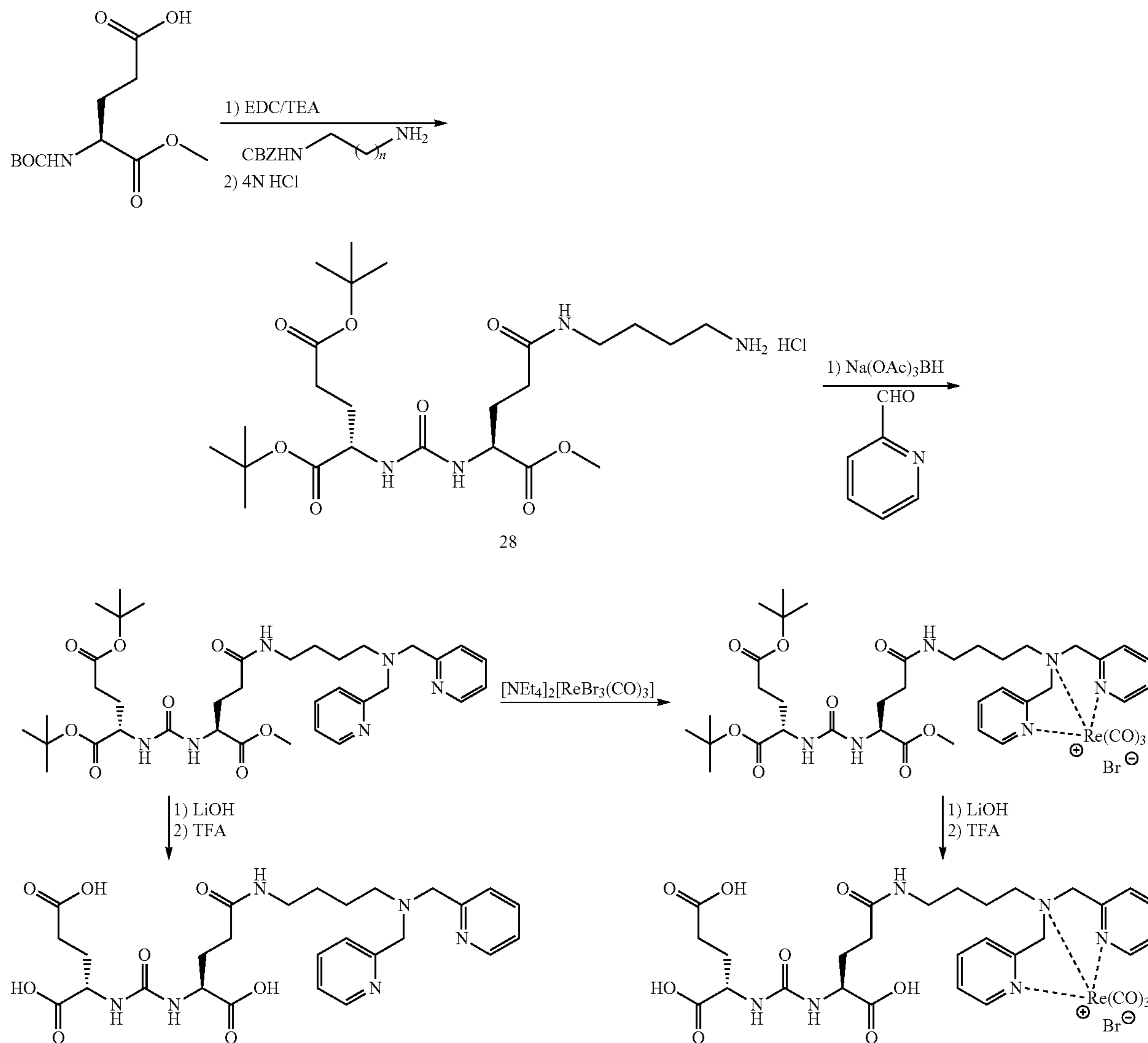
Scheme 4.
