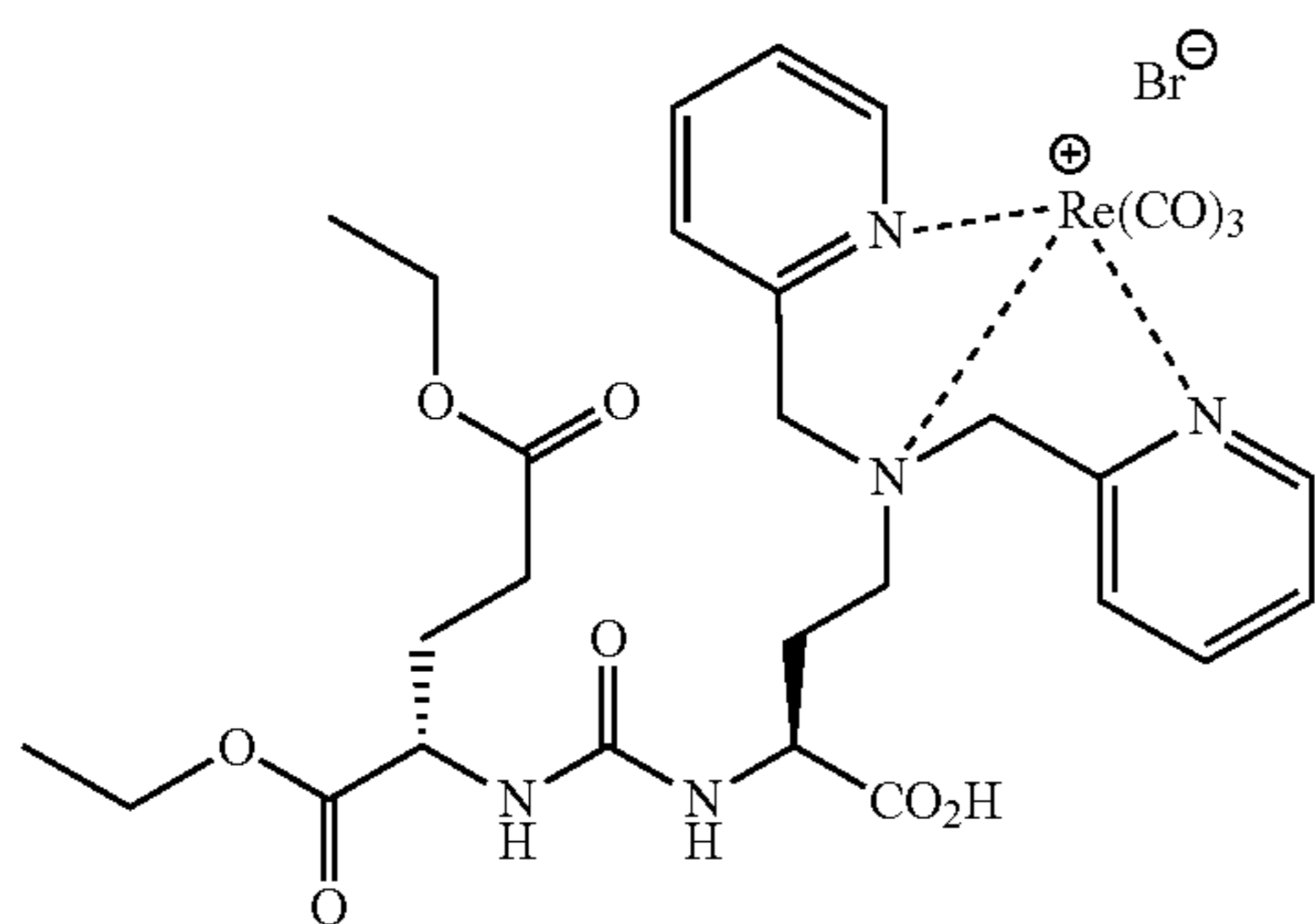
[Re(CO) 3 (2-{3-[5-(Bis-pyridin-2-ylmethyl-amino)-1-carboxy-pentyl]-ureido}-pentanedioic acid)][Br] (25) (MIP 1029)
