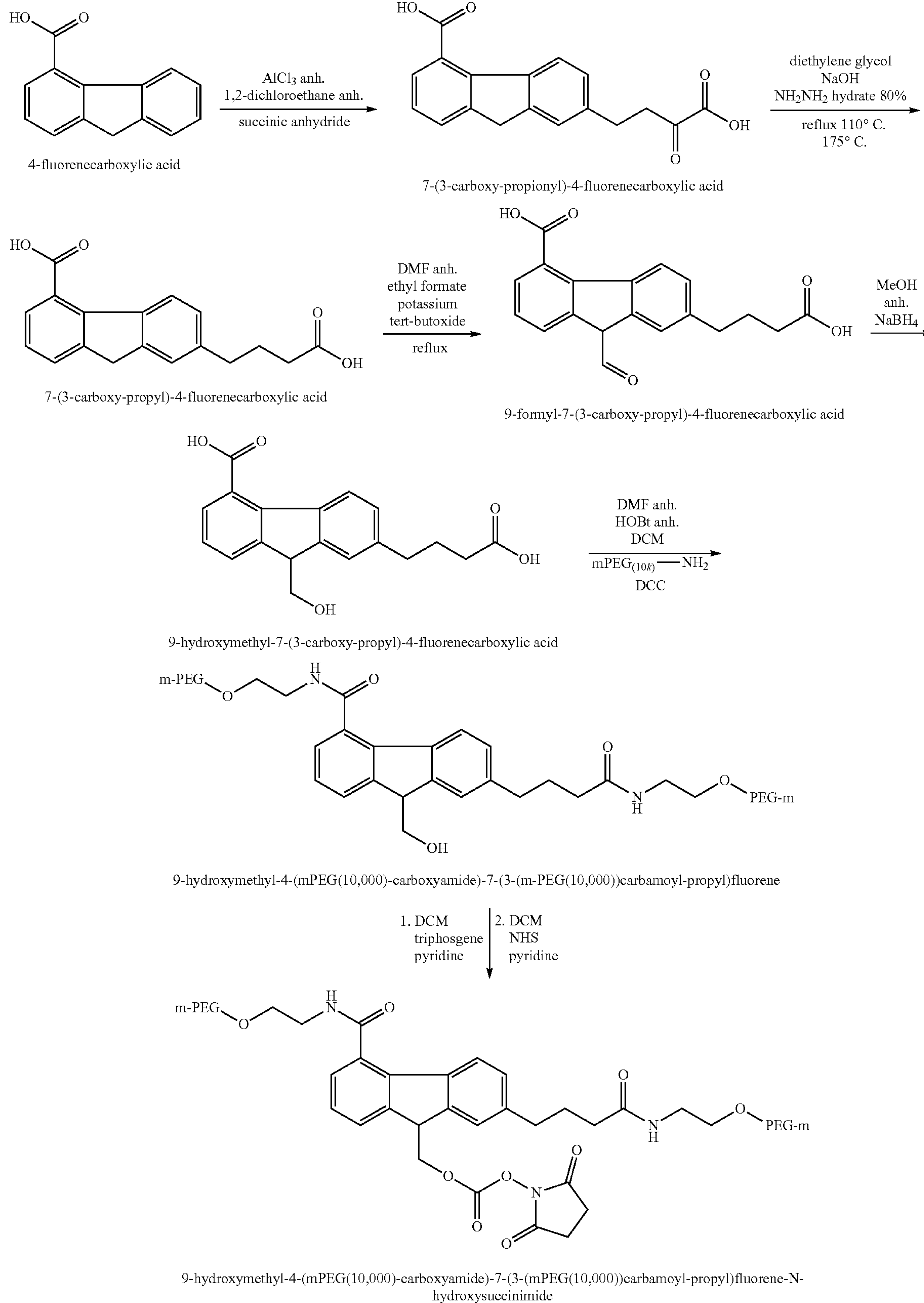
Scheme 4.
