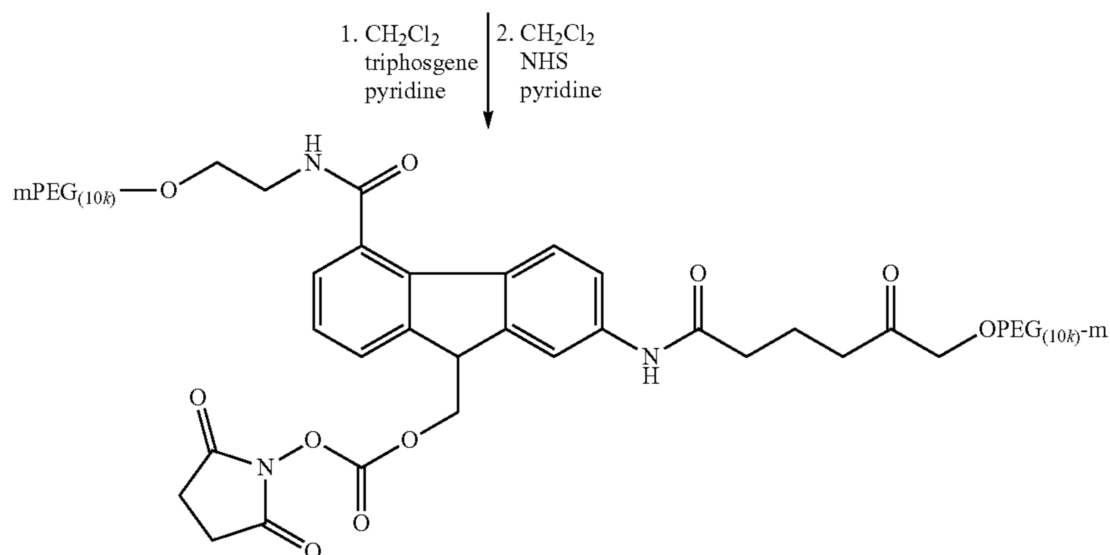
9-hydroxymethyl-4-(mPEG(10,000)-carboxyamide)-7-(m-PEG(10,000)-amidoglutamic acid)fluorene-N-hydroxysuccinimide
