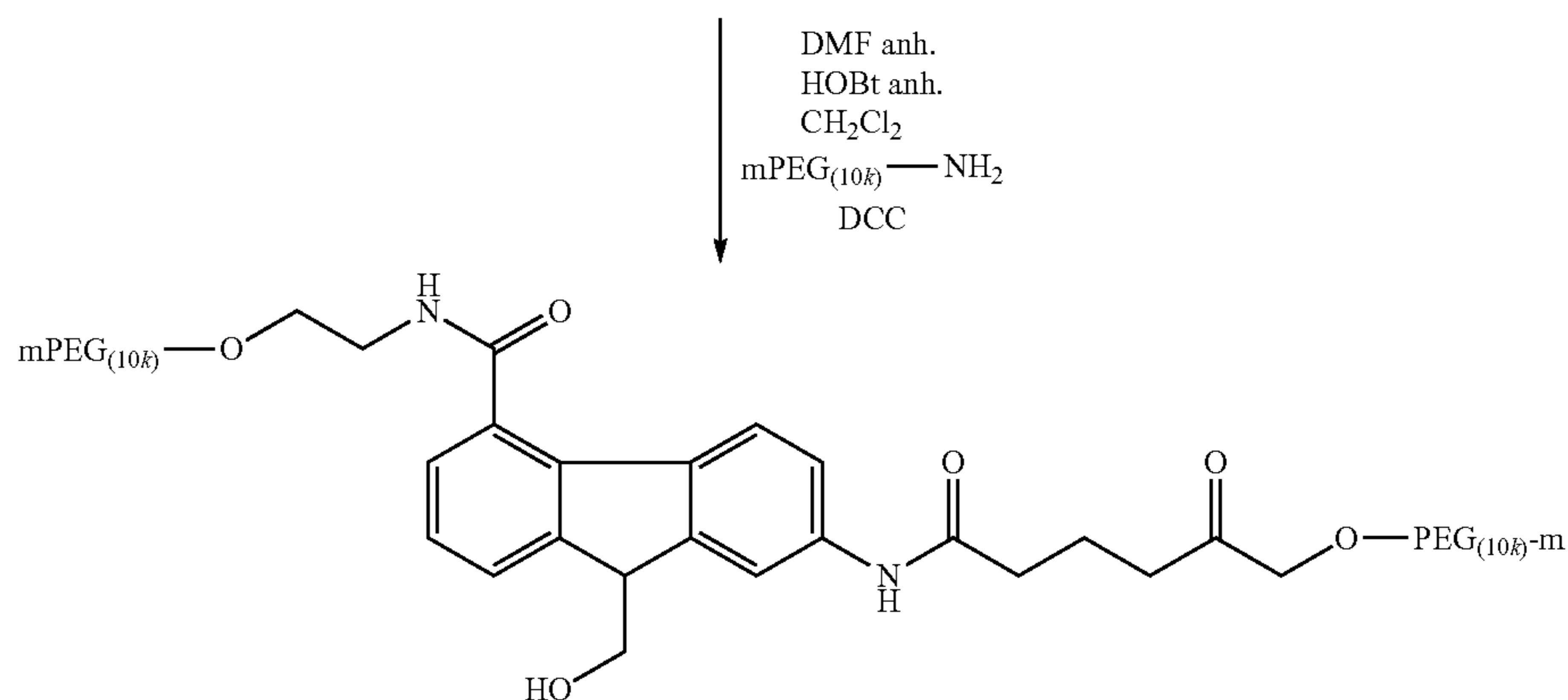
9-hydroxymethyl-4-(mPEG(10,000)-carboxyamide)-7-(m-PEG(10,000)-amidoglutamic acid)fluorene
