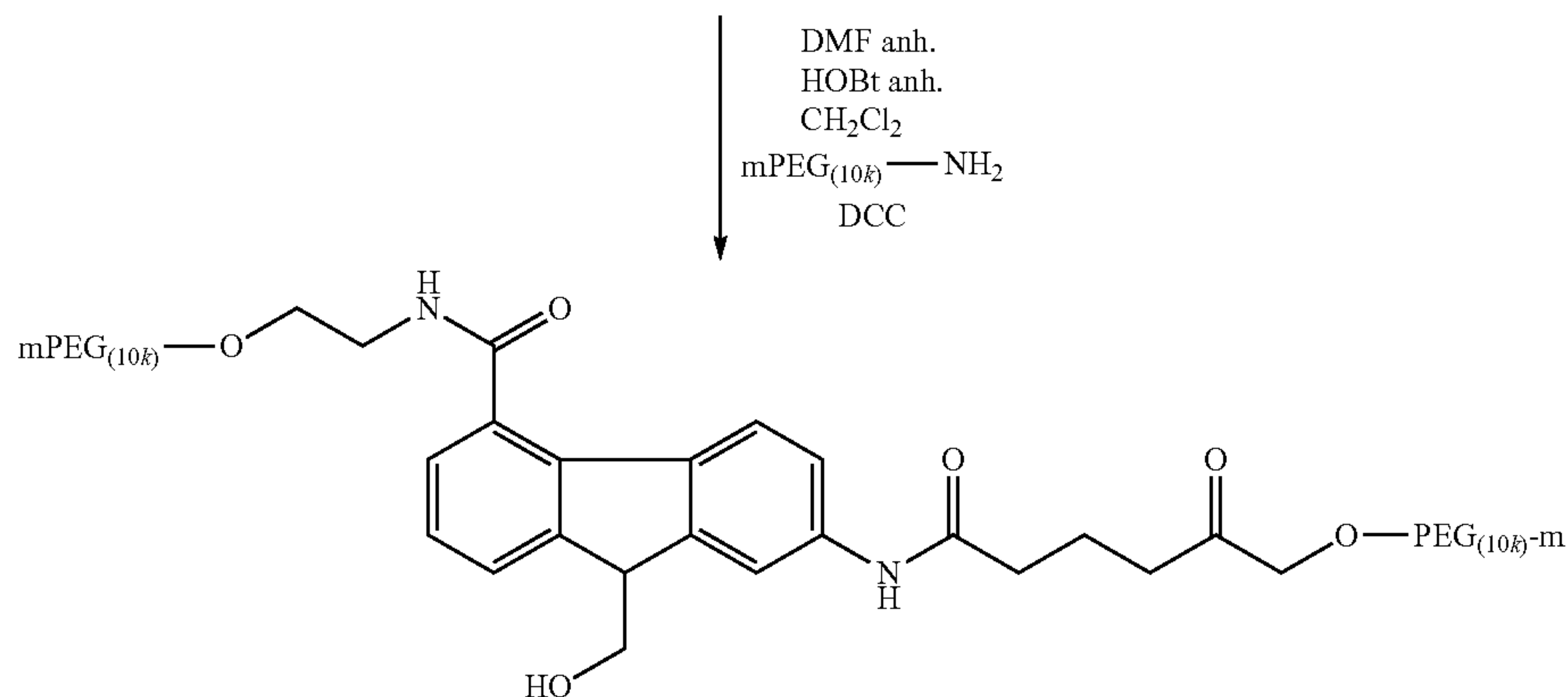
9-hydroxymethyl-4-(mPEG(10,000)-carboxyamide)-7-(m-PEG(10,000)-amidoglutaric acid)fluorene
