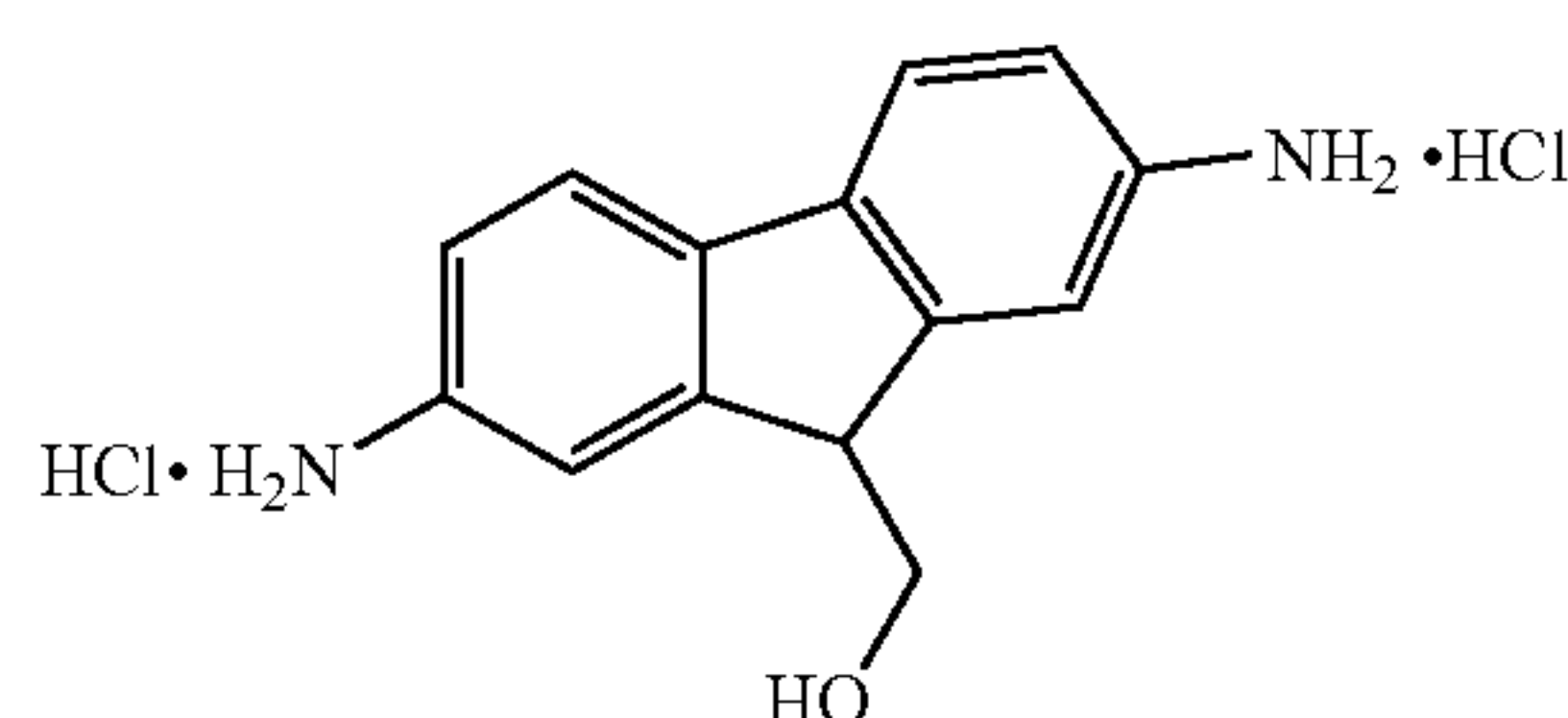
9-hydroxymethyl-2,7-diaminofluorene dihydrochloride
