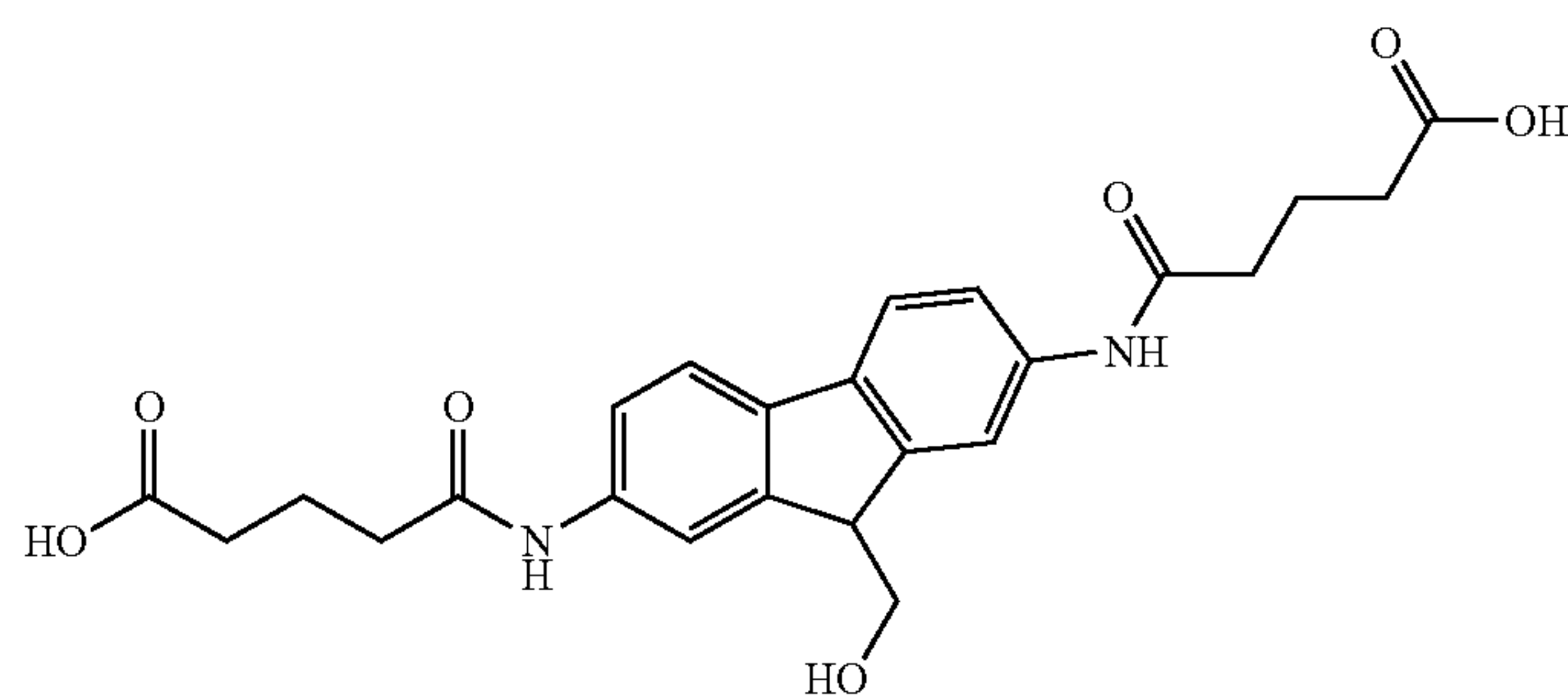
9-hydroxymethyl-2,7-di(amidoglutamic acid)fluorene
