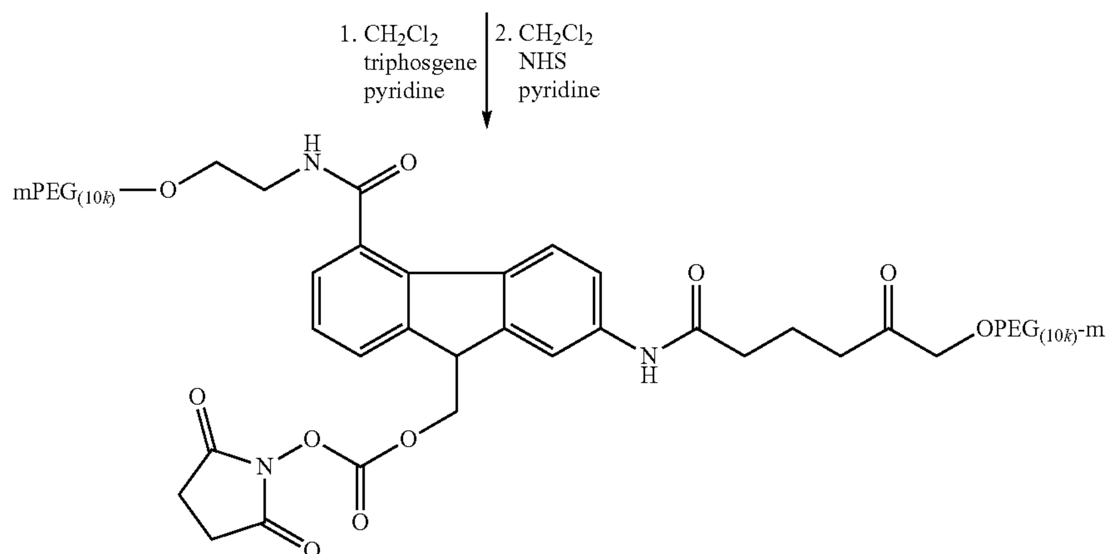
9-hydroxymethyl-4-(mPEG(10,000)-carboxyamide)-7-(m-PEG(10,000)-amidoglutaric acid)fluorene-N-hydroxysuccinimide
