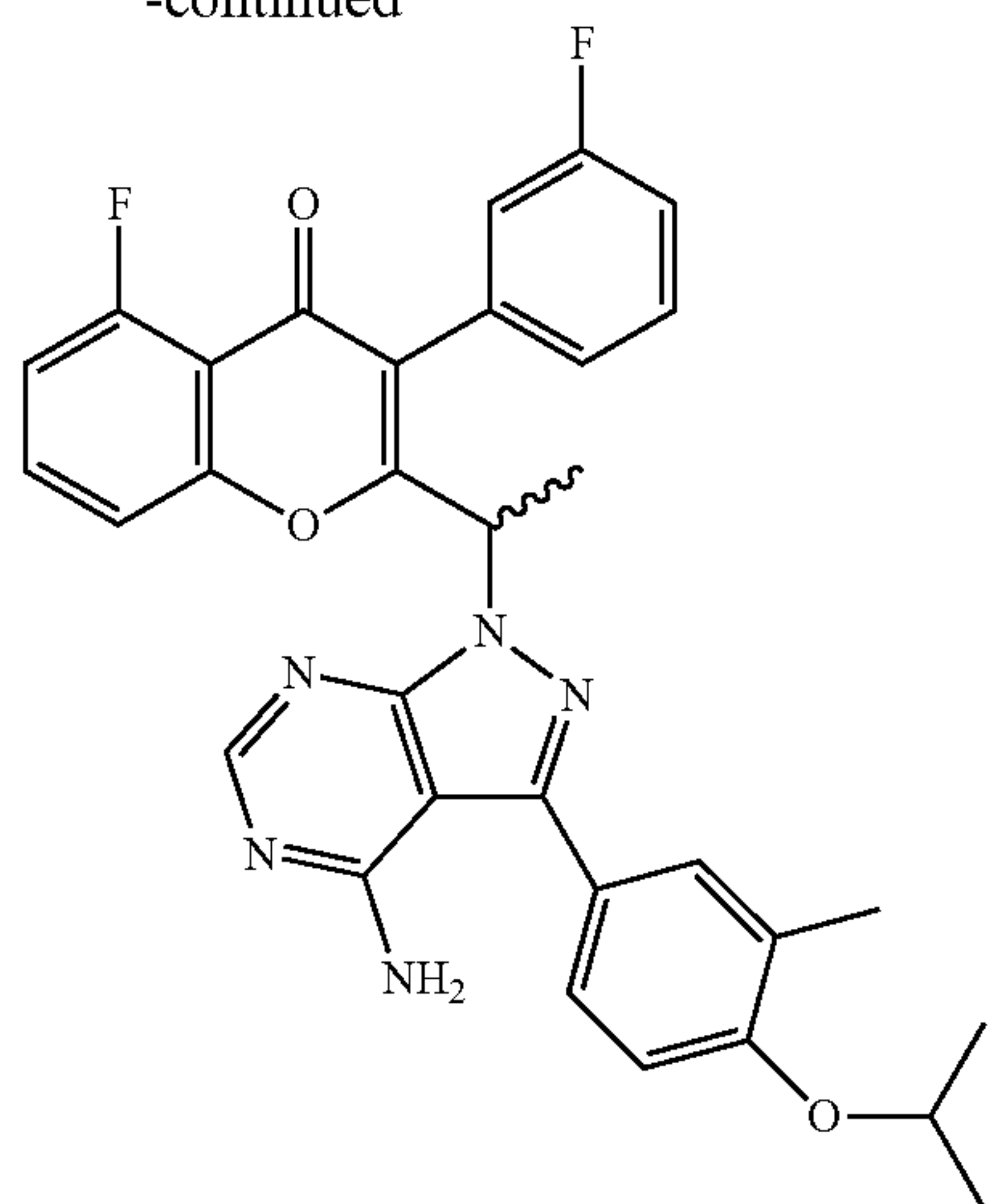
(-)-2-(1-(4-amino-3-(4-isopropoxy-3-methylphenyl)1H-pyrazolo[3,4-d]pyrimidin-1-yl)ethyl)-5-fluoro-3-(3-fluorophenyl)-4H-chromen-4-one
