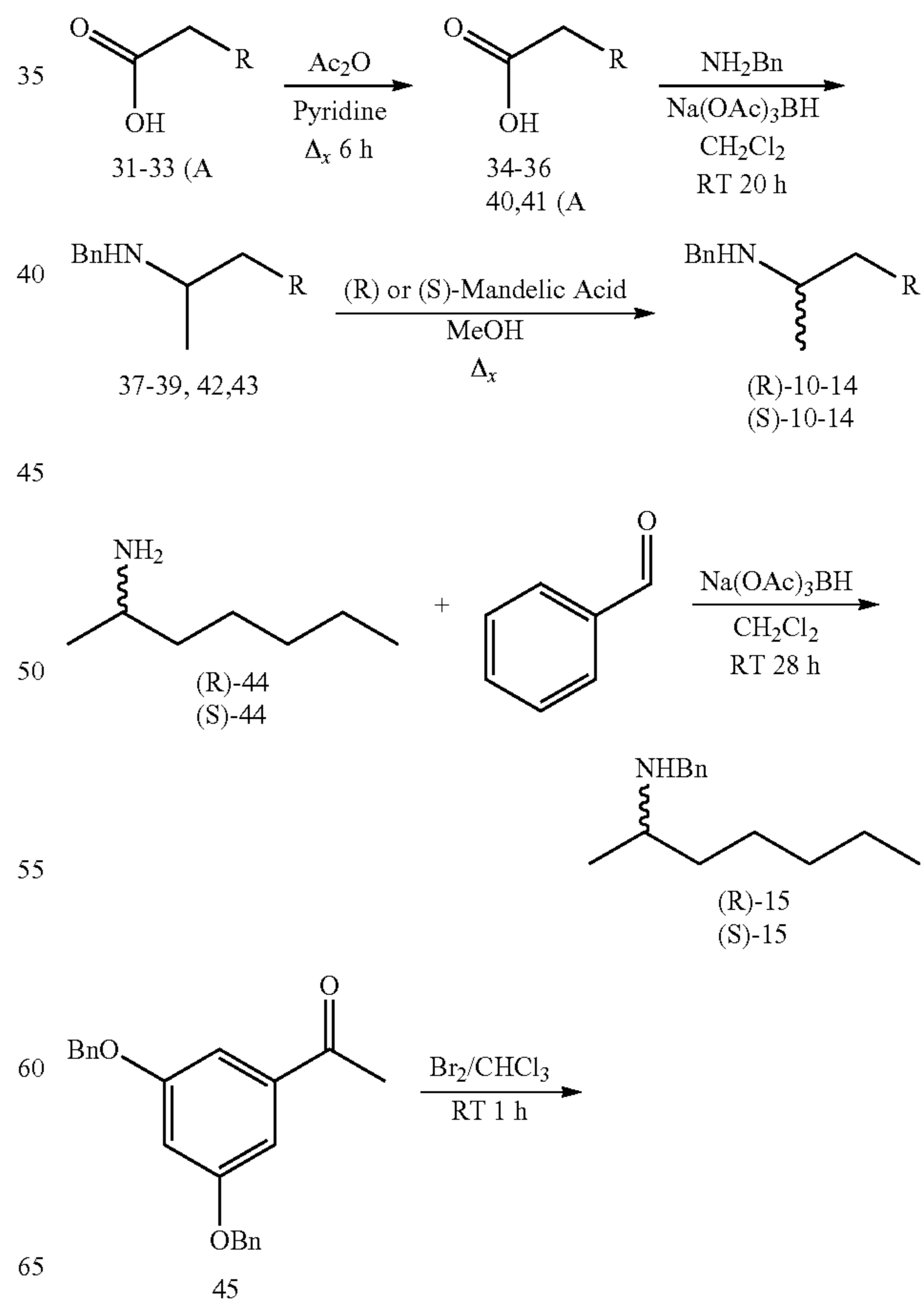
Scheme III describes an exemplary synthesis for the chiral building blocks used in Scheme II. The (R)- and (S)-3',5'-dibenzoyloxyphenyl-bromohydrin enantiomers were obtained by the enantiospecific reduction of 3,5-dibenzoyloxy- \alpha -bromoacetophenone using boron-methyl sulfide complex (BH 3 SCH 3 ) and either (1R,2S)- or (1S,2R)- cis-1-amino-2-indanol. The required (R)- and (S)-2-benzylaminopropanes were prepared by enantioselective crystallization of the rac-2-benzylaminopropanes using either (R)- or (S)-mandelic acid as the counter ion.
