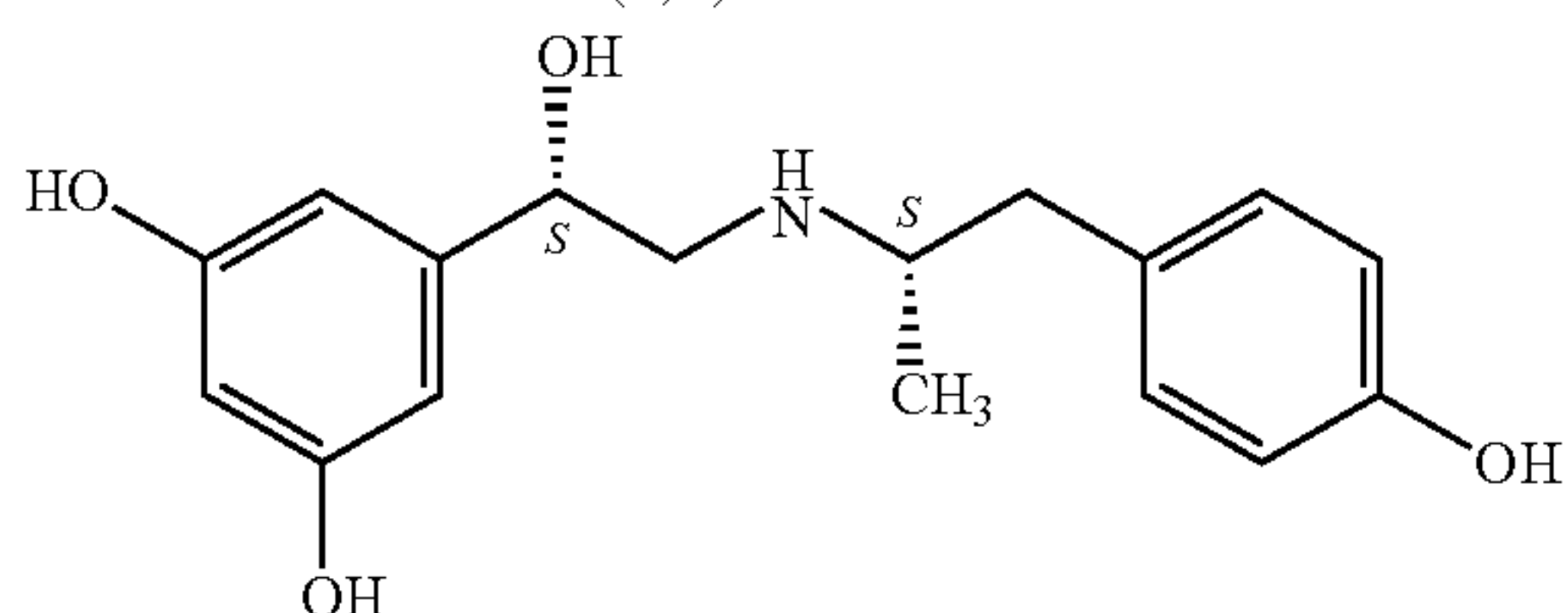
(S,S)-Fenoterol
