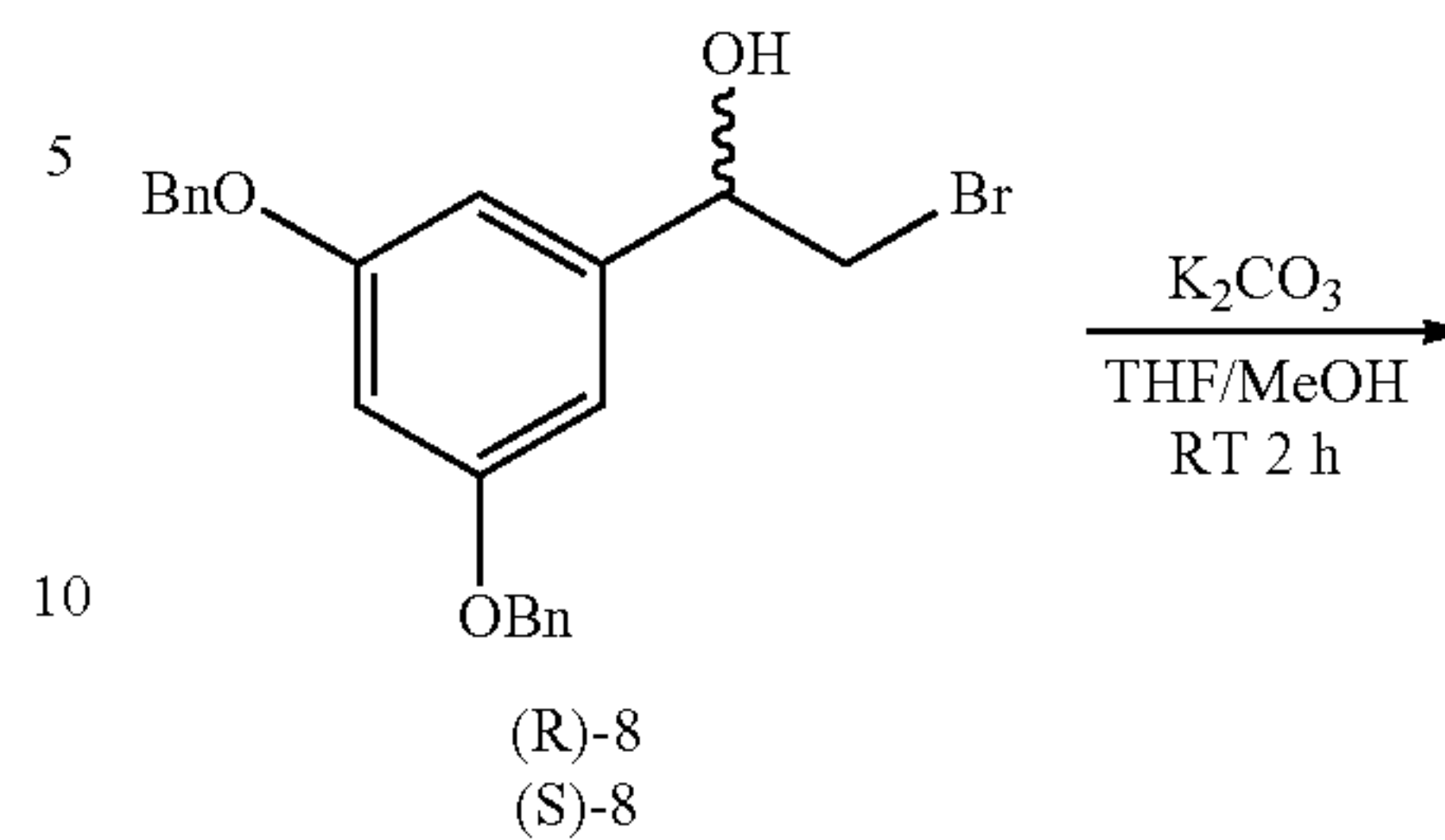
Scheme I
