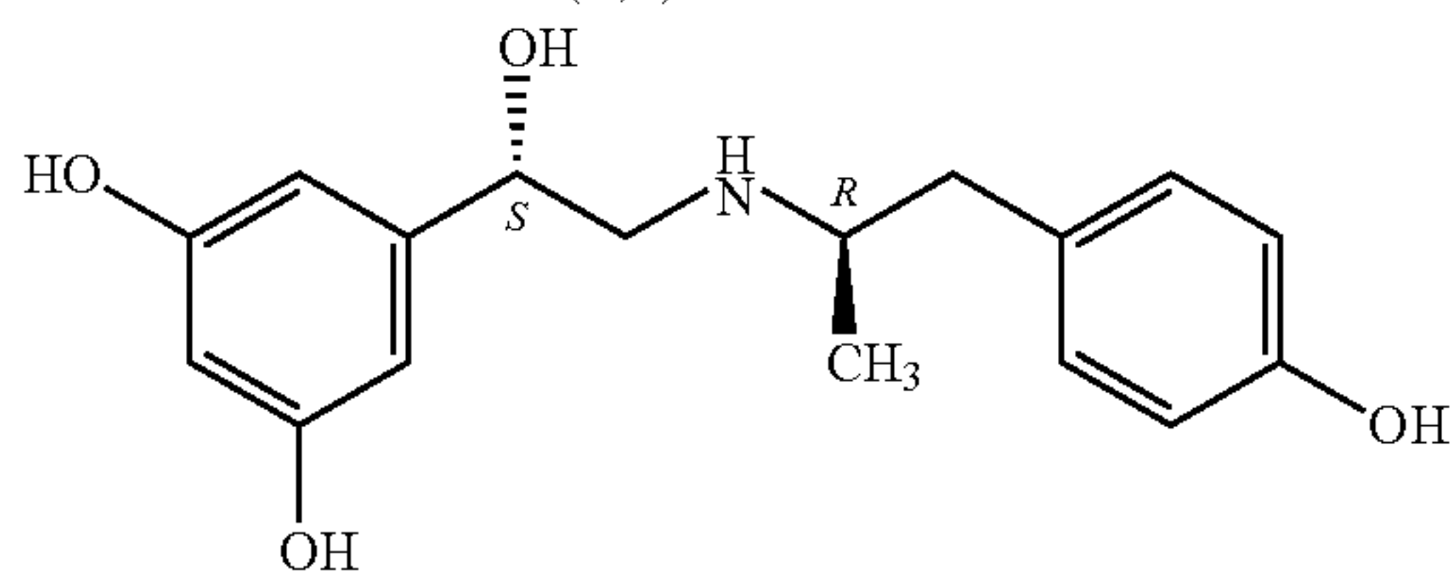
(S,R)-Fenoterol
