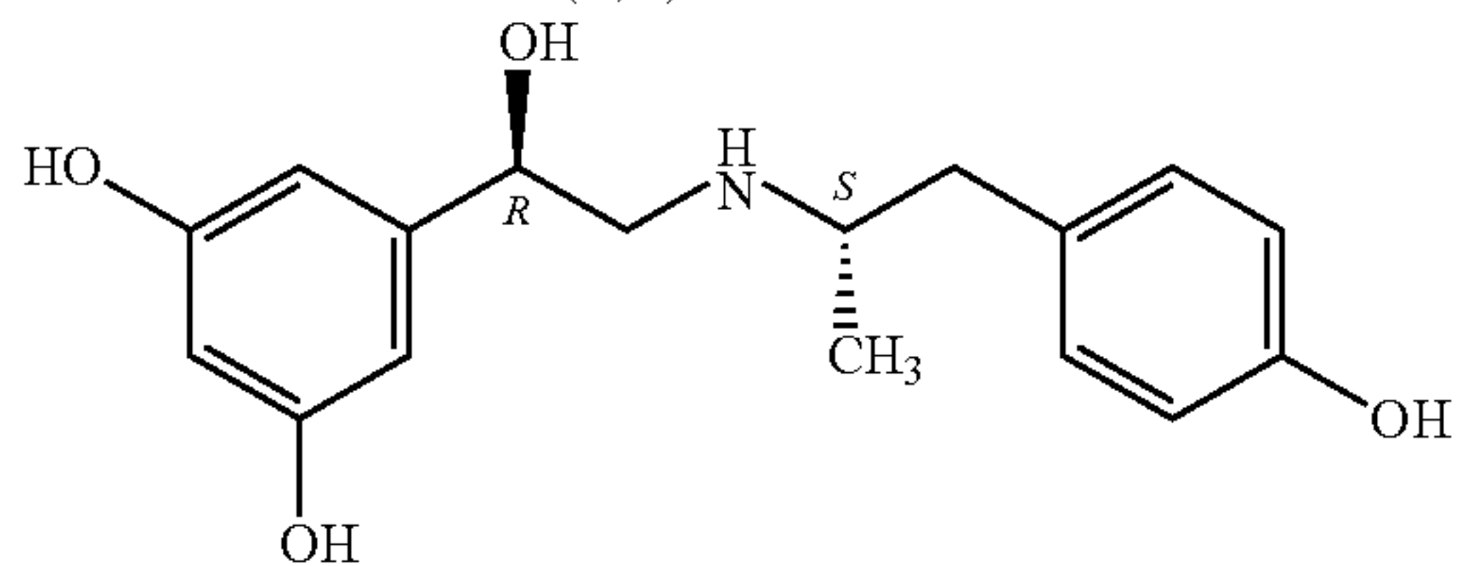
(R,S)-Fenoterol
