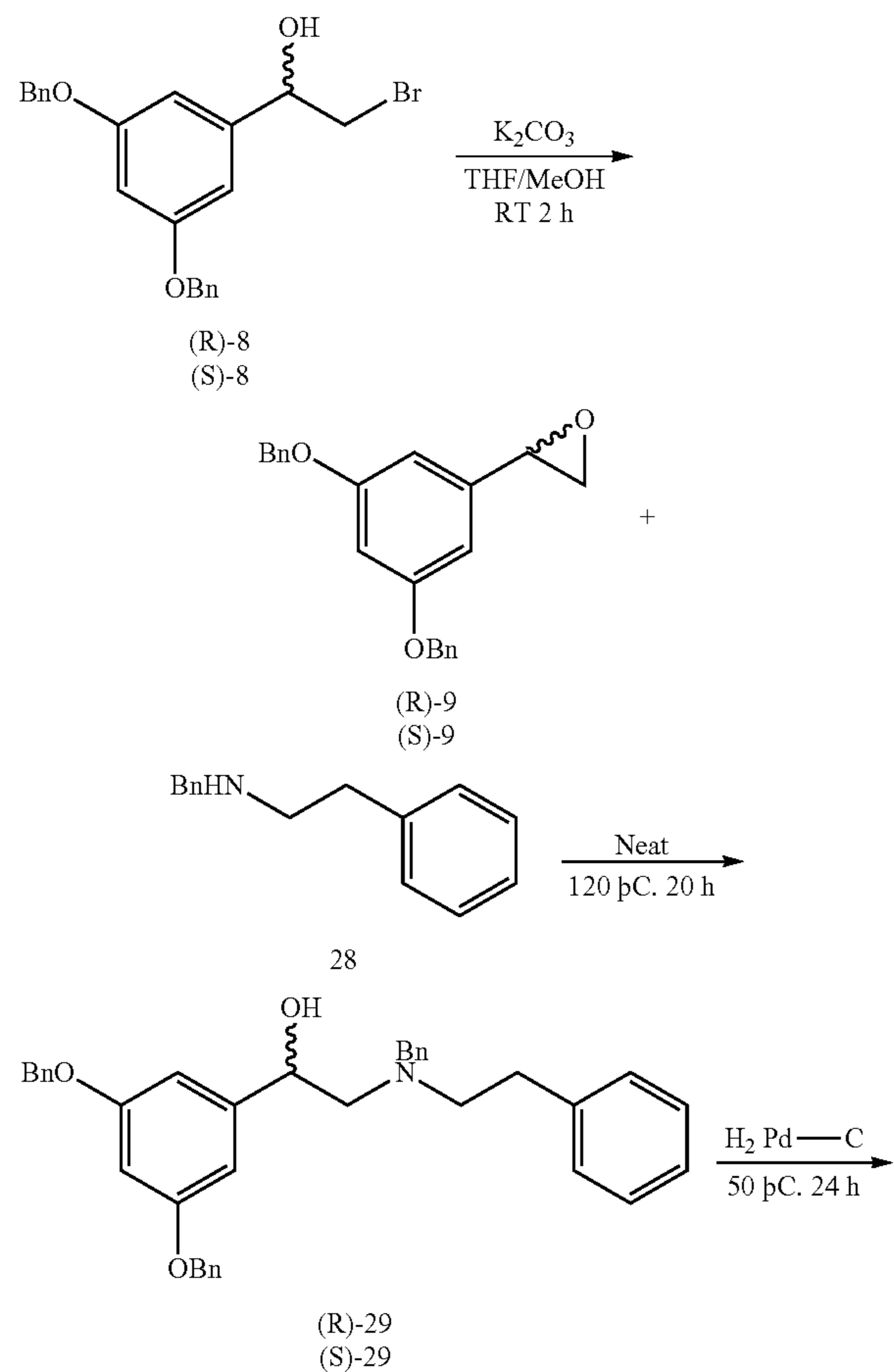
Scheme II: Exemplary synthesis of (R)-7 and (S)-7 using 2-phenethylamine. The resulting compounds may be deprotected by hydrogenation over Pd/C and purified as the fumarate salts.
