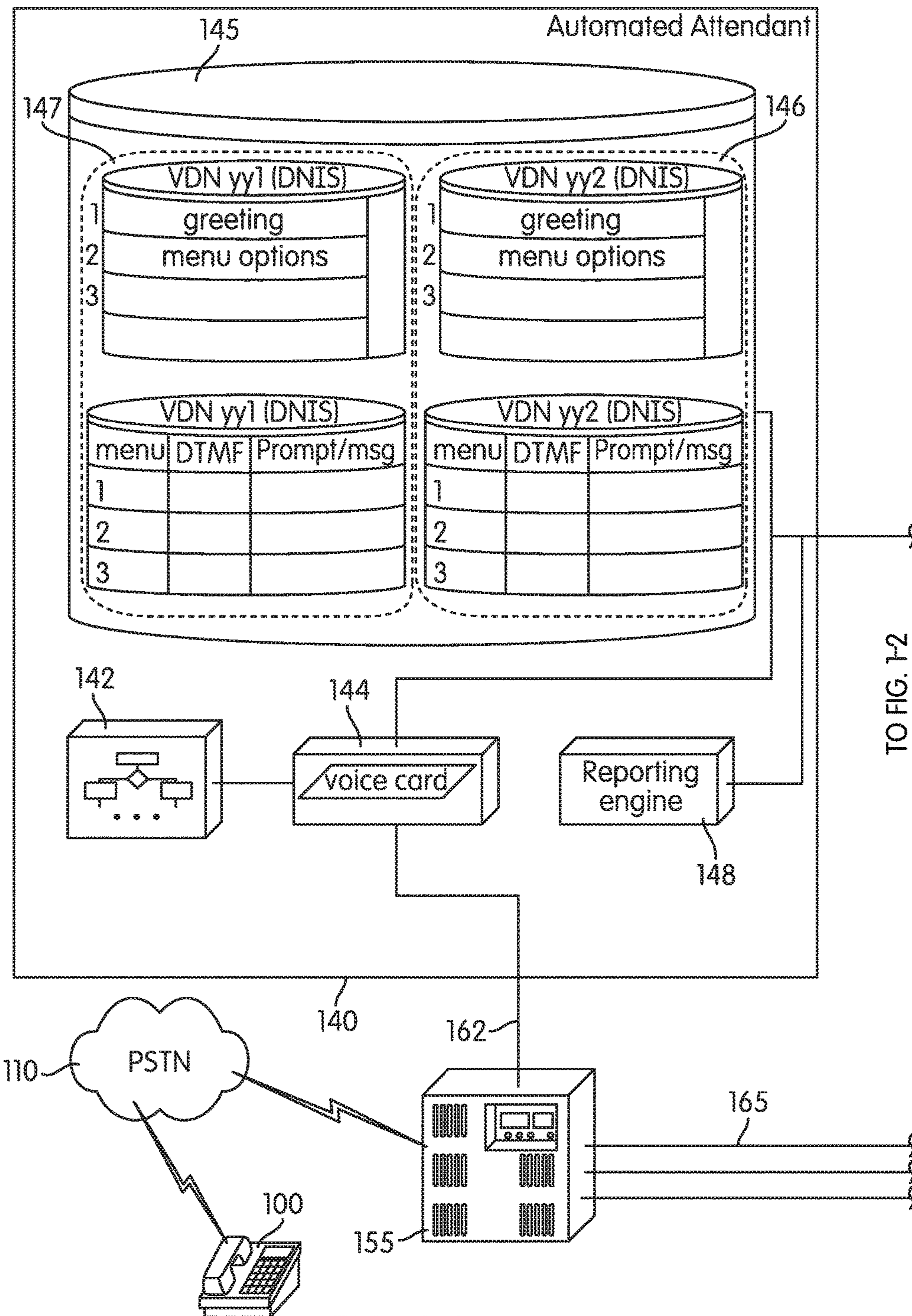
FIG. 1-1 PRIOR ART
