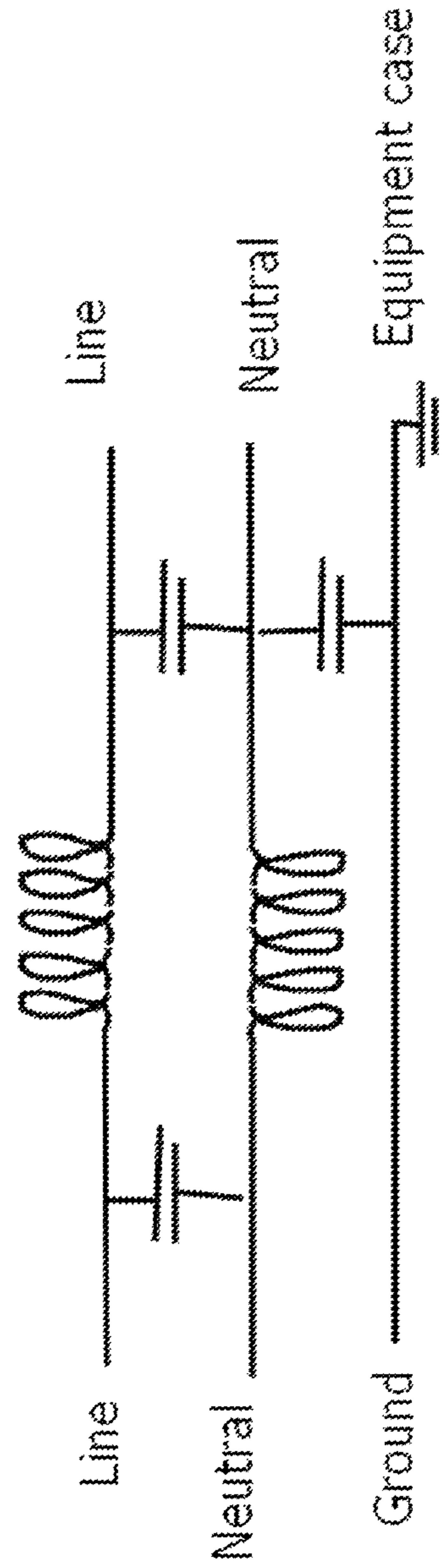
Figure 9B: A safe RFI filter configuration
