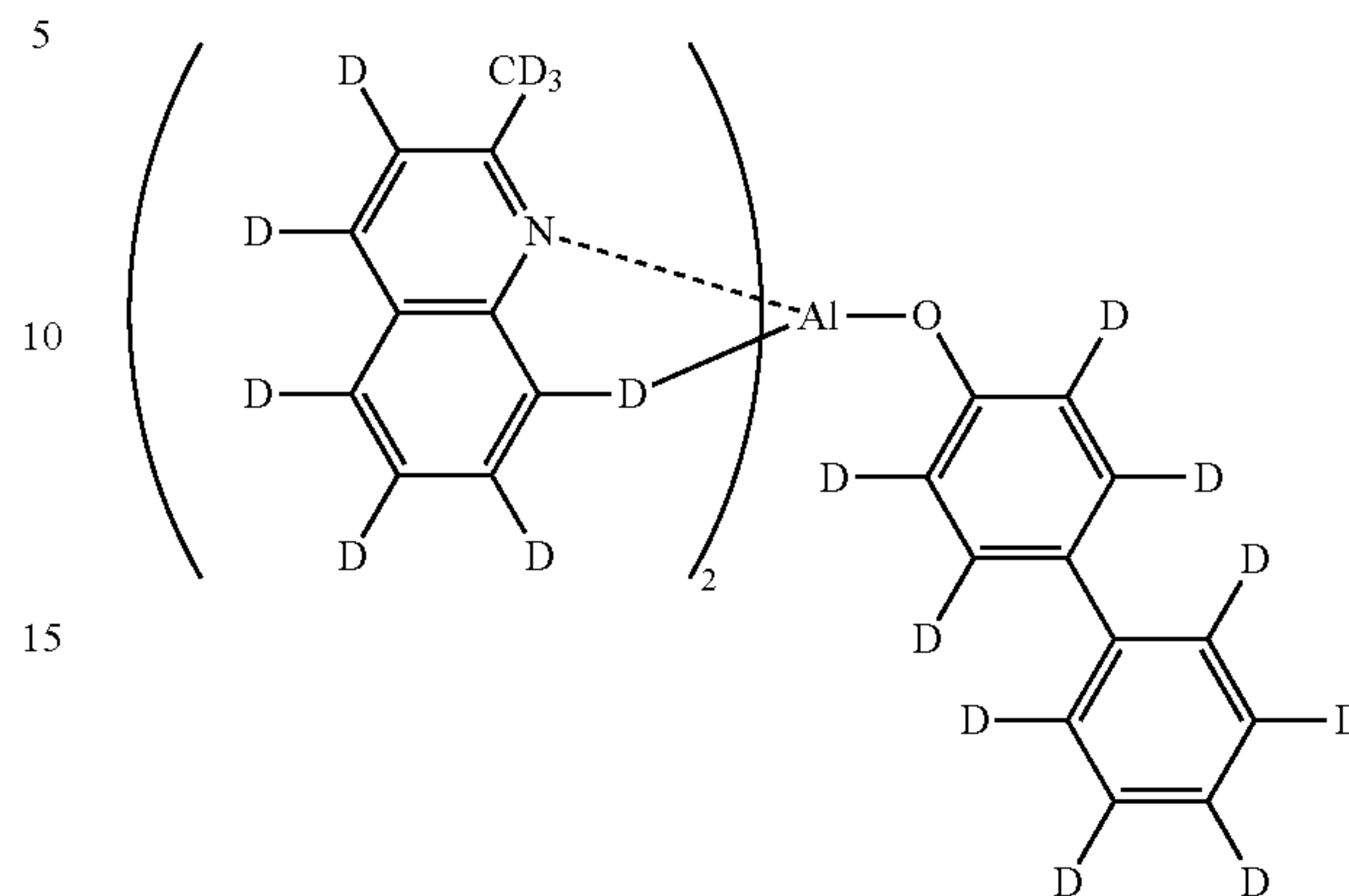
Compound E
