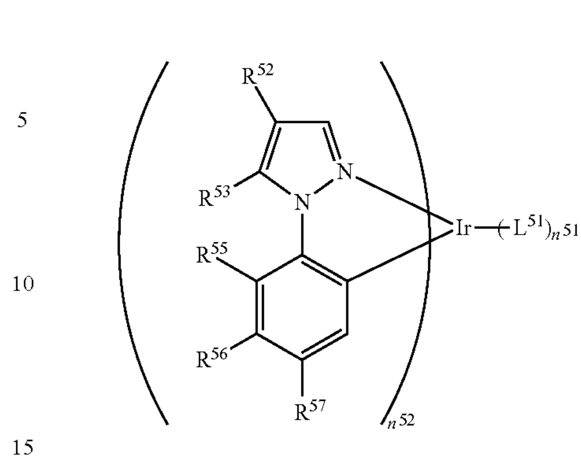
Formula (III)
