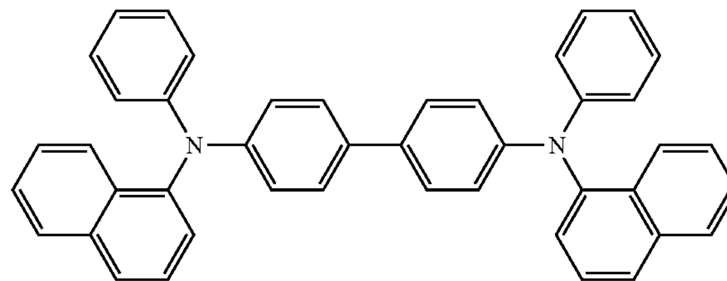
Compound B
