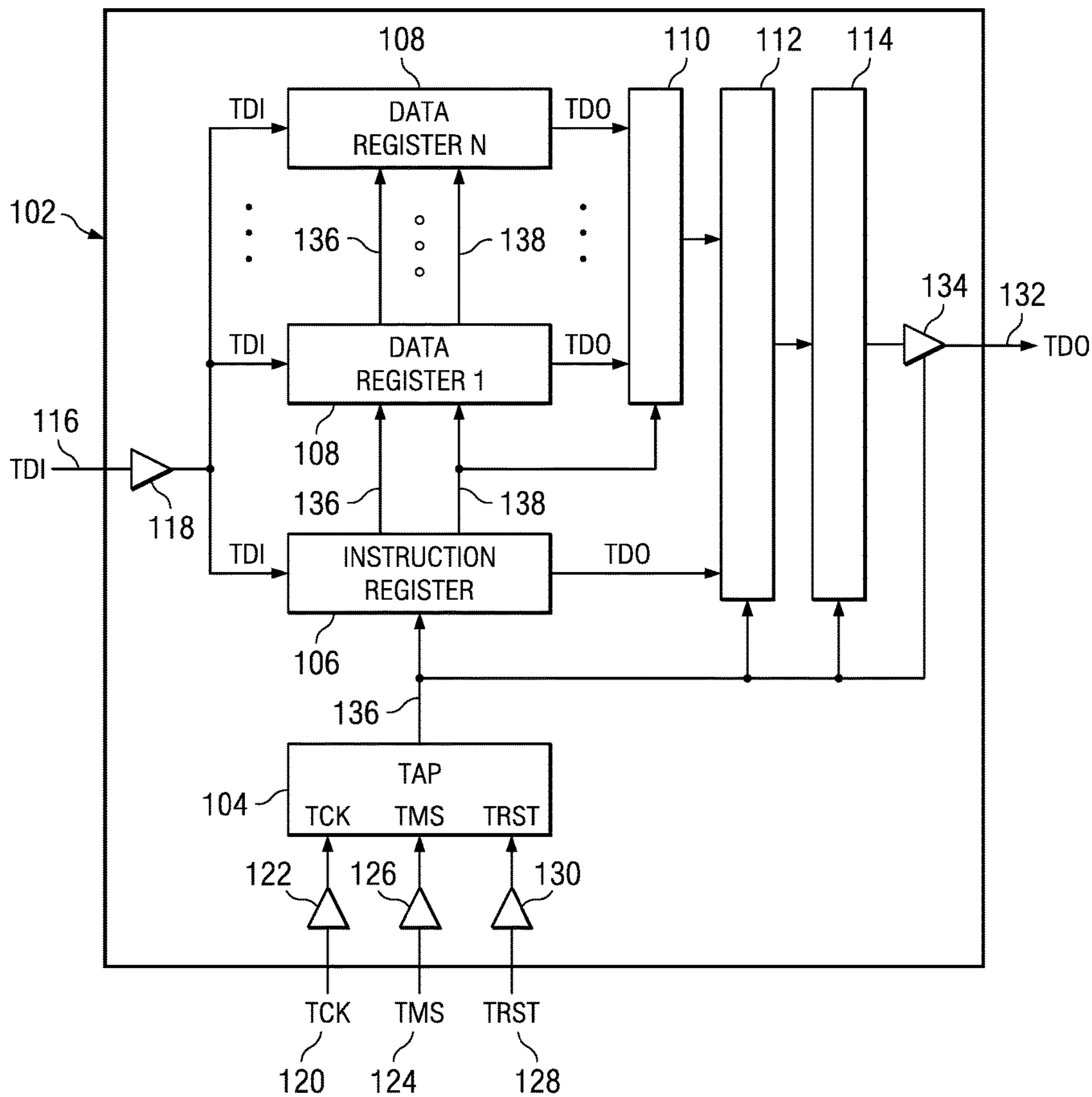
FIG. 1 (PRIOR ART)
