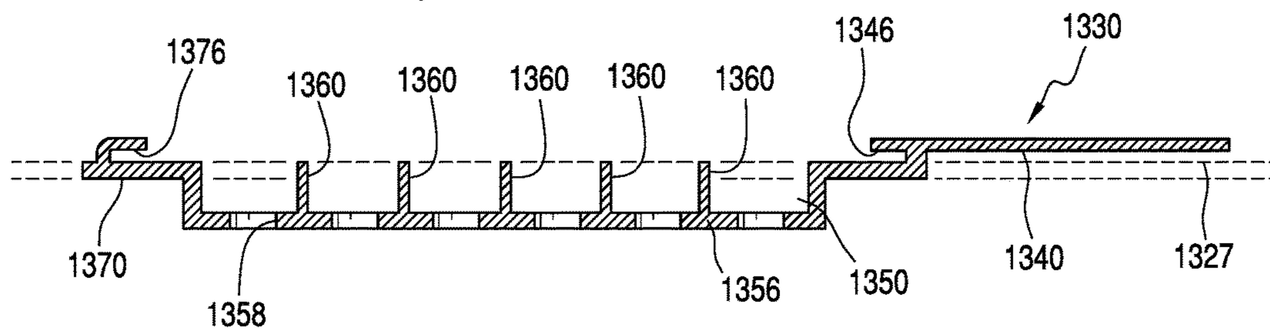
FIG. 2 (PRIOR ART)
