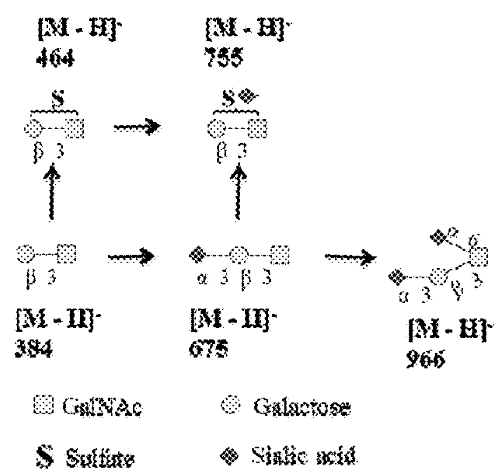
FIG. 6 - glycosylation (recombinant)
