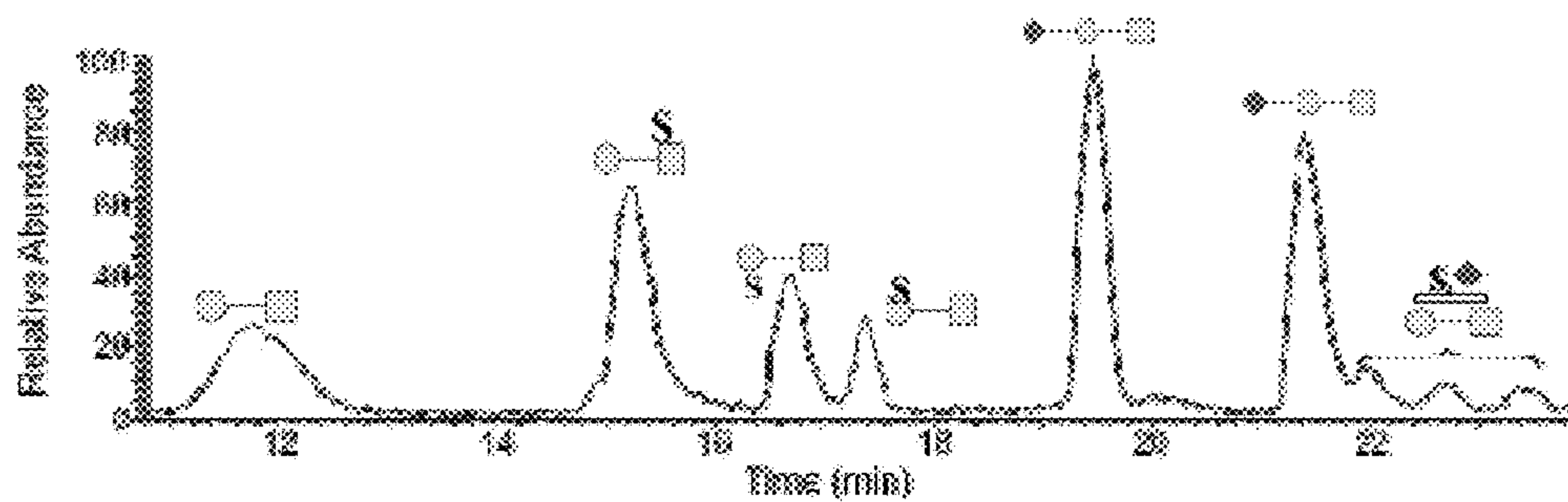
FIG. 7 - glycosylation (recombinant)
