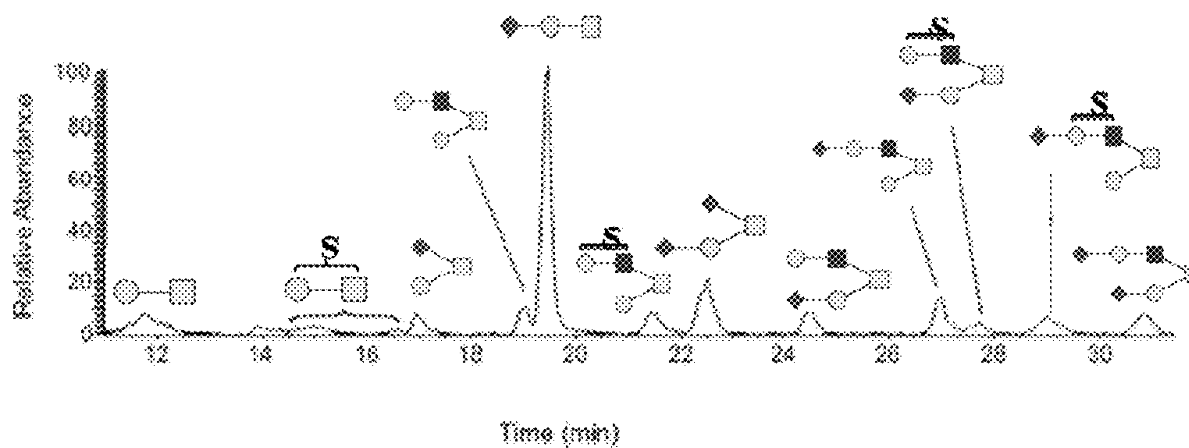
FIG. 9 - glycosylation (native)
