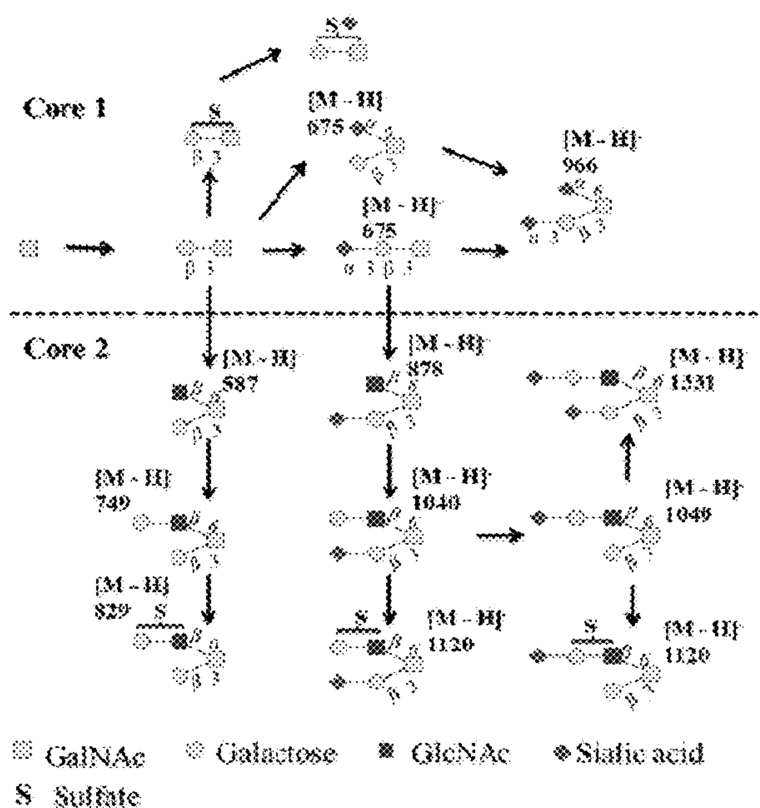
FIG. 8 - glycosylation (native)
