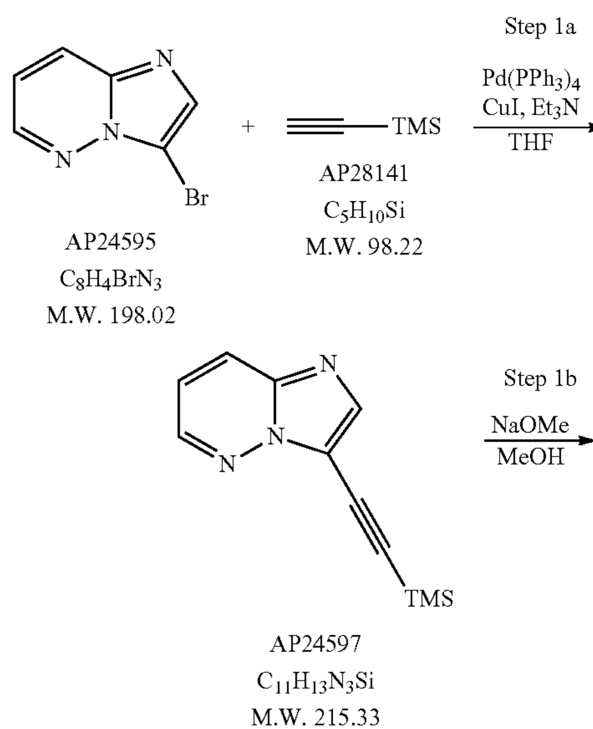
Scheme 2: Step 1-Synthesis of AP25047
