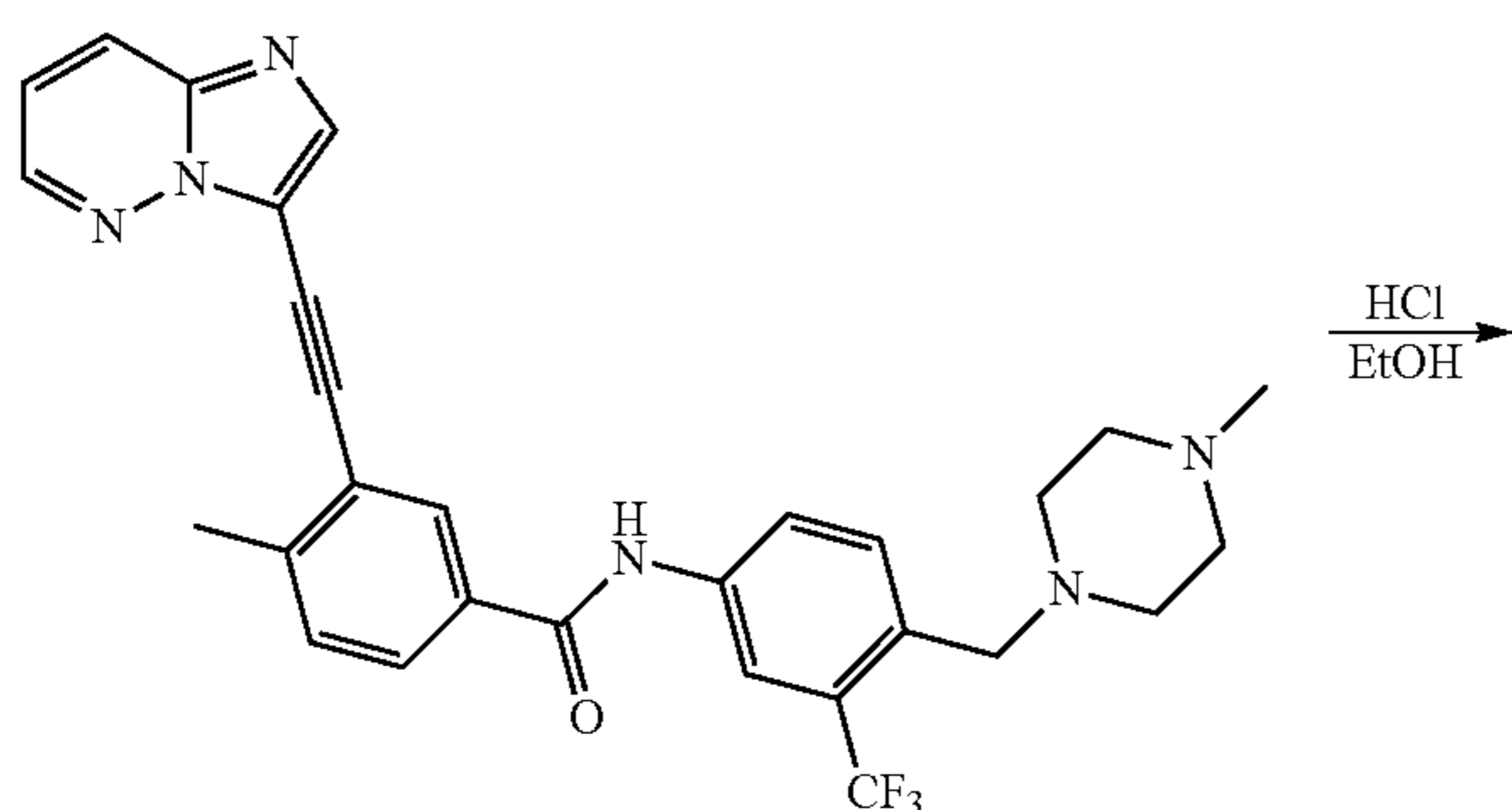
Scheme 5: Step 4-Synthesis of Ponatinib HCl
