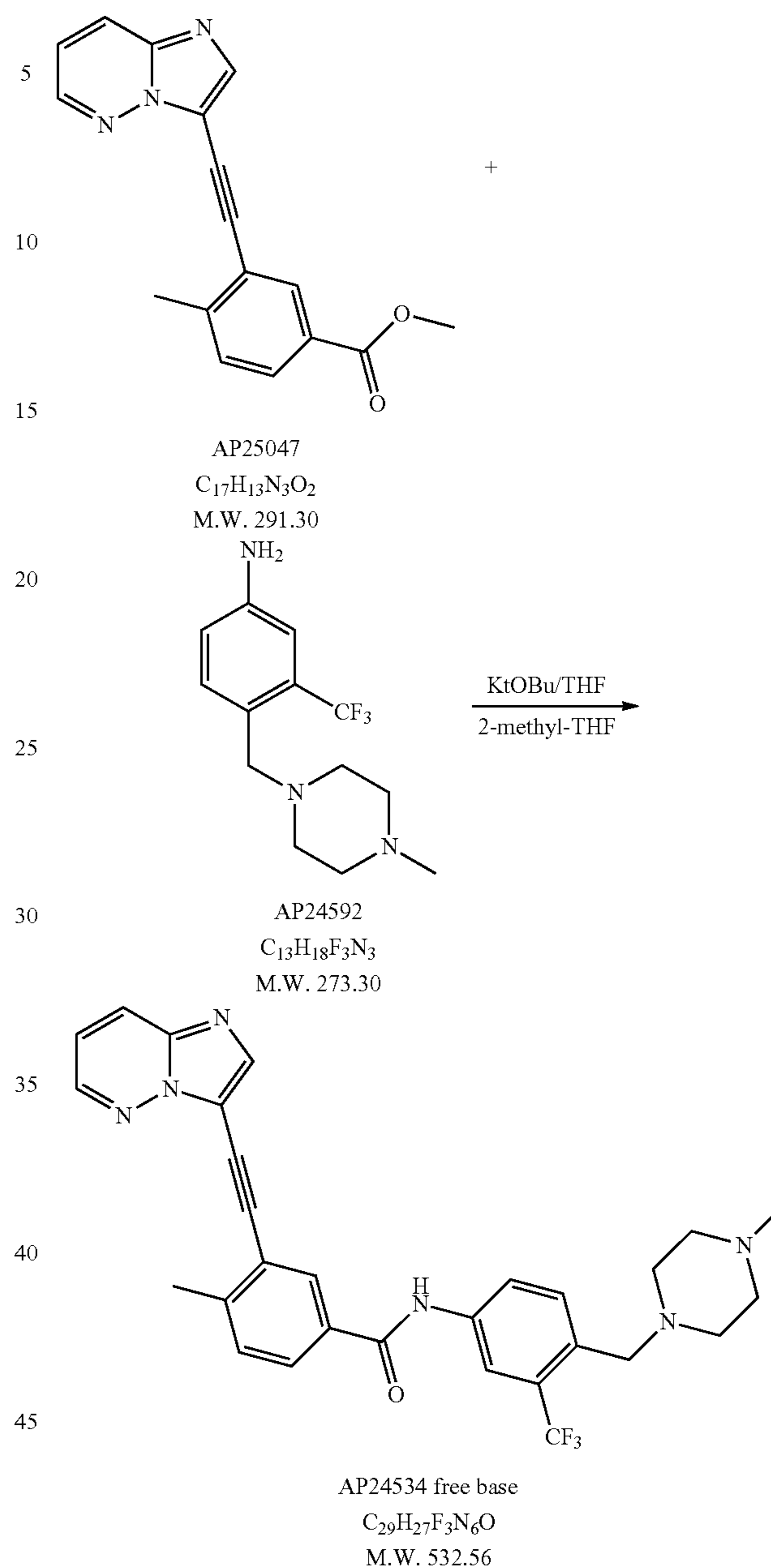
Scheme 4: Step 3-Synthesis of AP24534 Free Base
