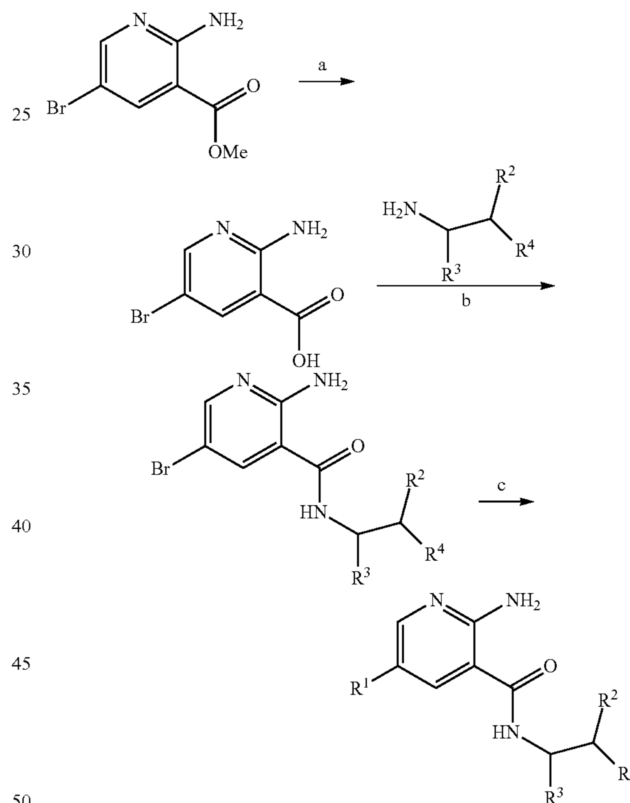
Scheme 2. General Procedure B
