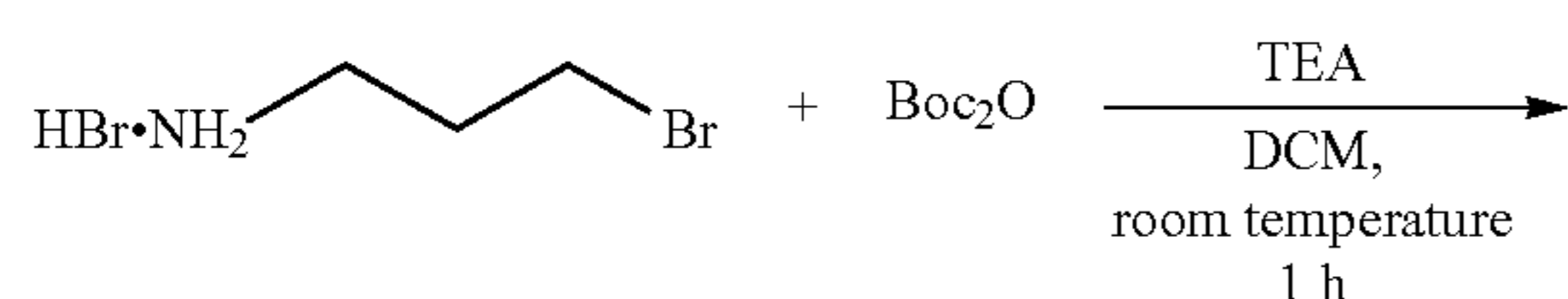
t-Butyl (3-bromopropyl)carbamate (1)
