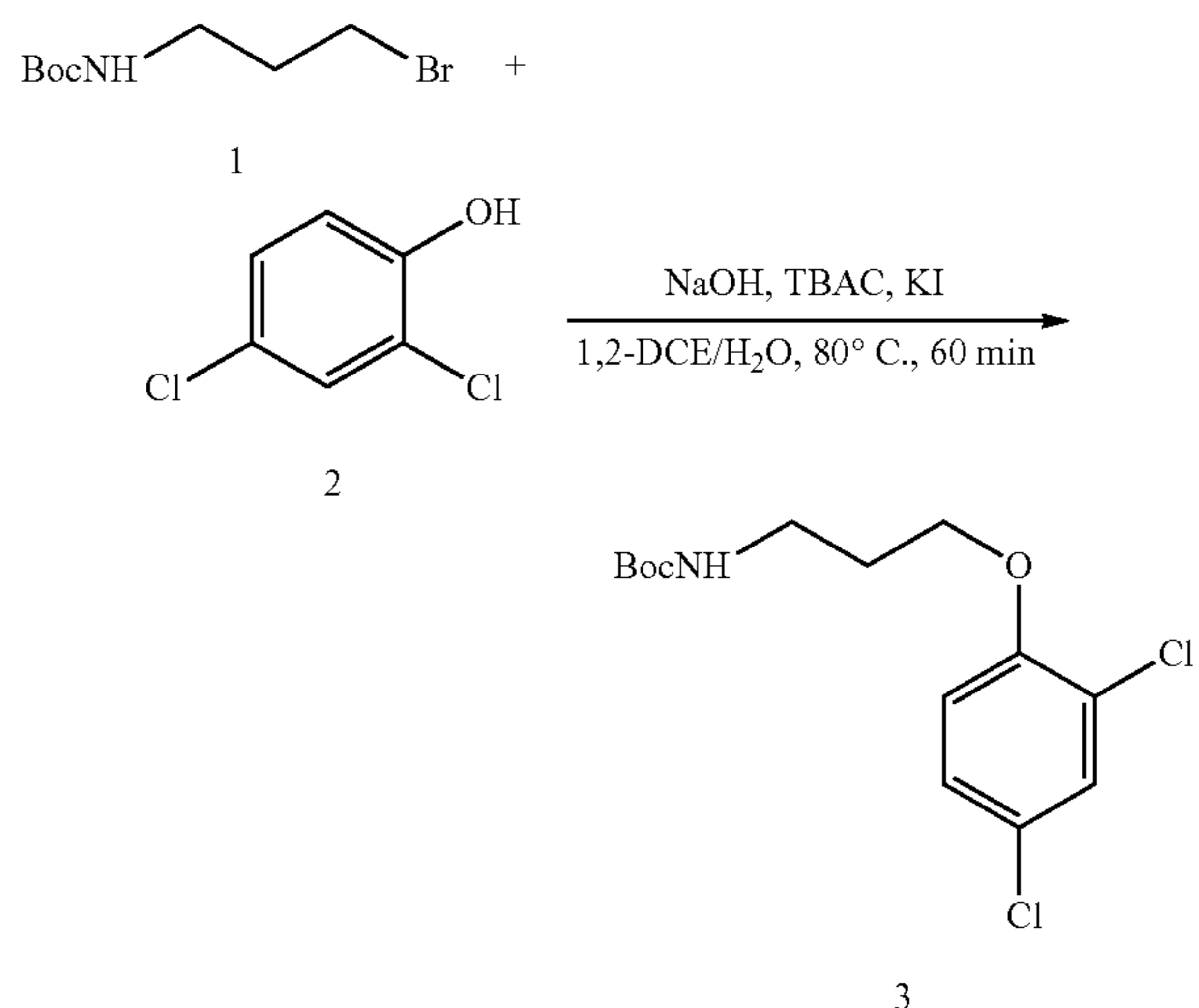
t-Butyl 3-(2,4-dichlorophenoxy)propylcarbamate (3)
