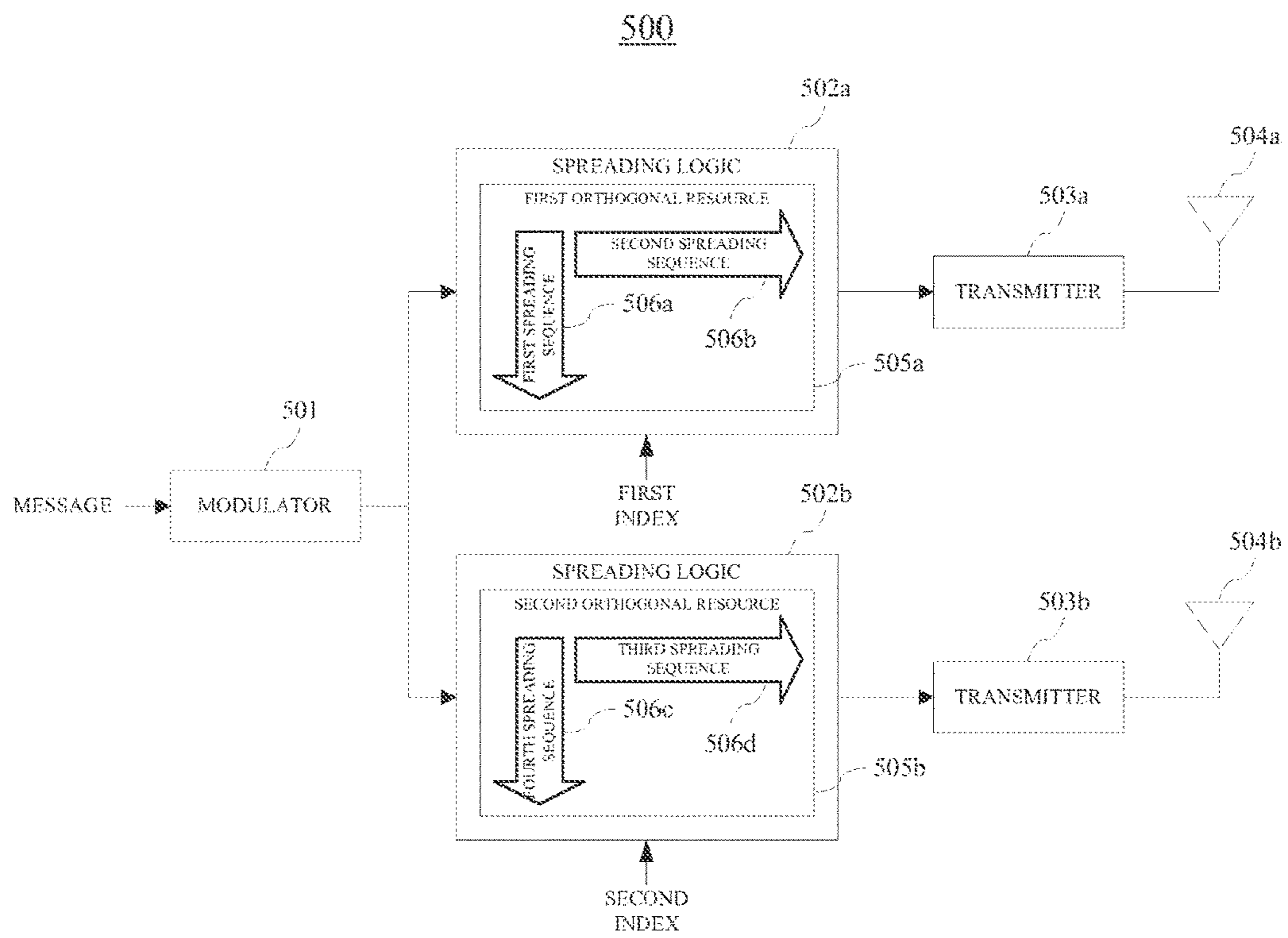
FIG. 5 (PRIOR ART)
