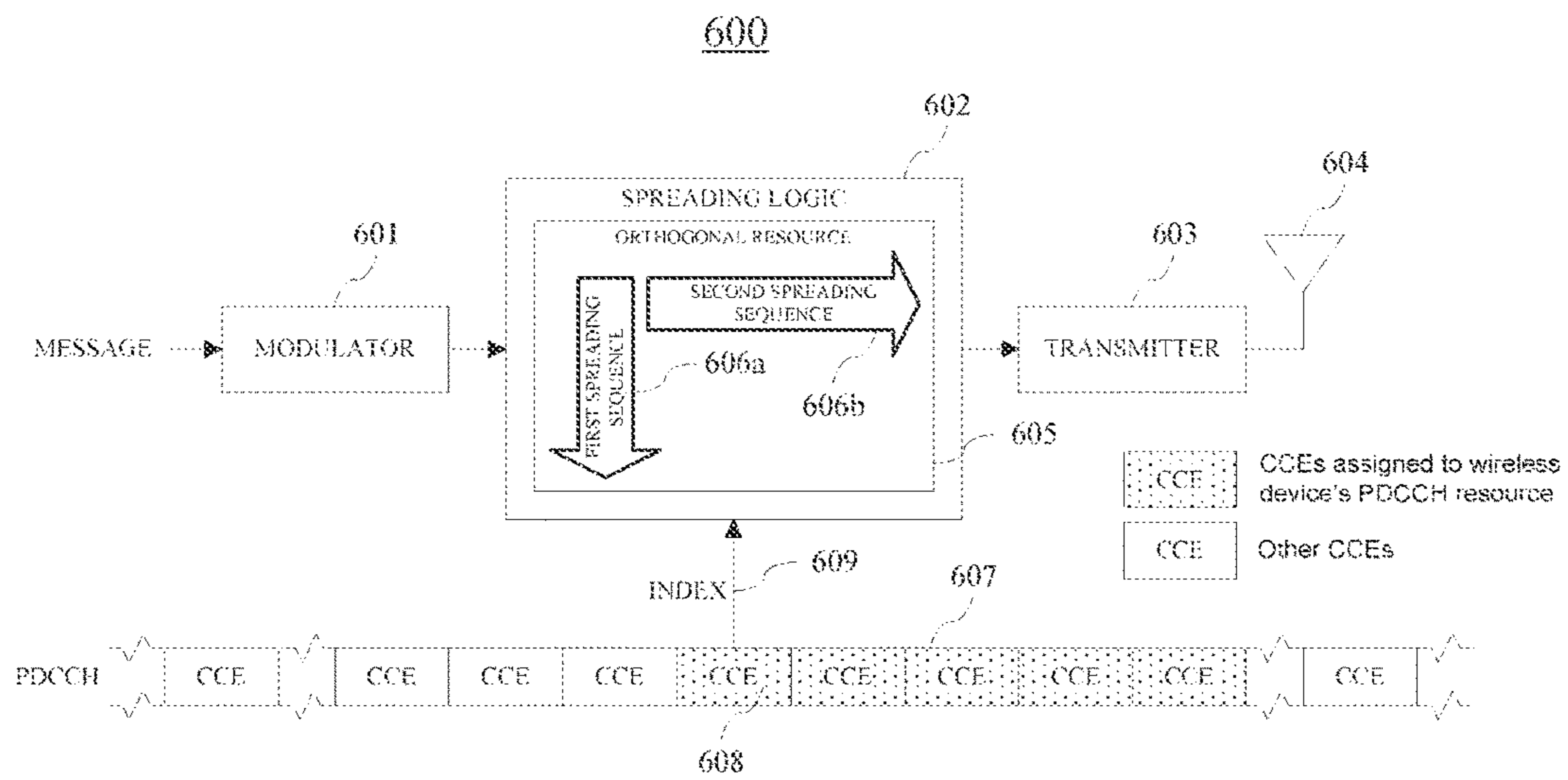
FIG. 6 (PRIOR ART)
