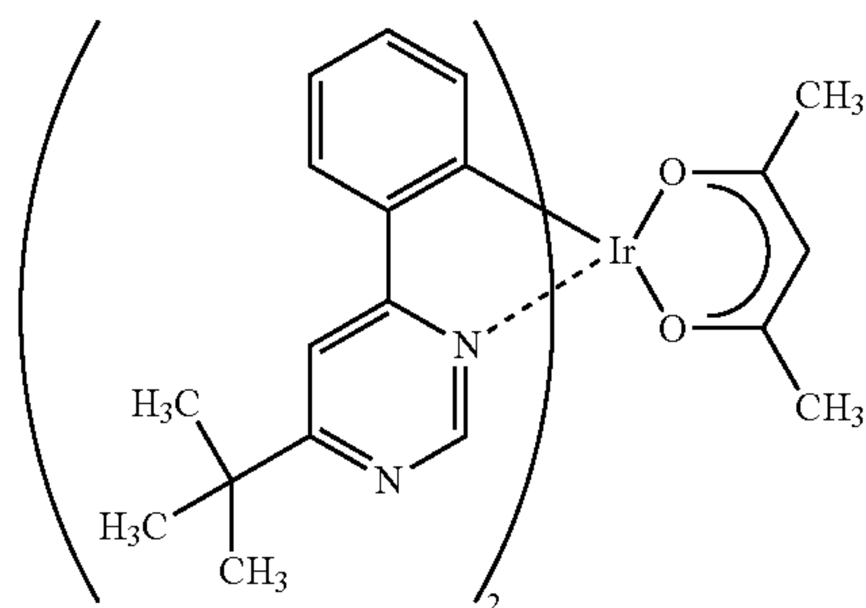
[Ir(tBuppm) 2 (acac)]
