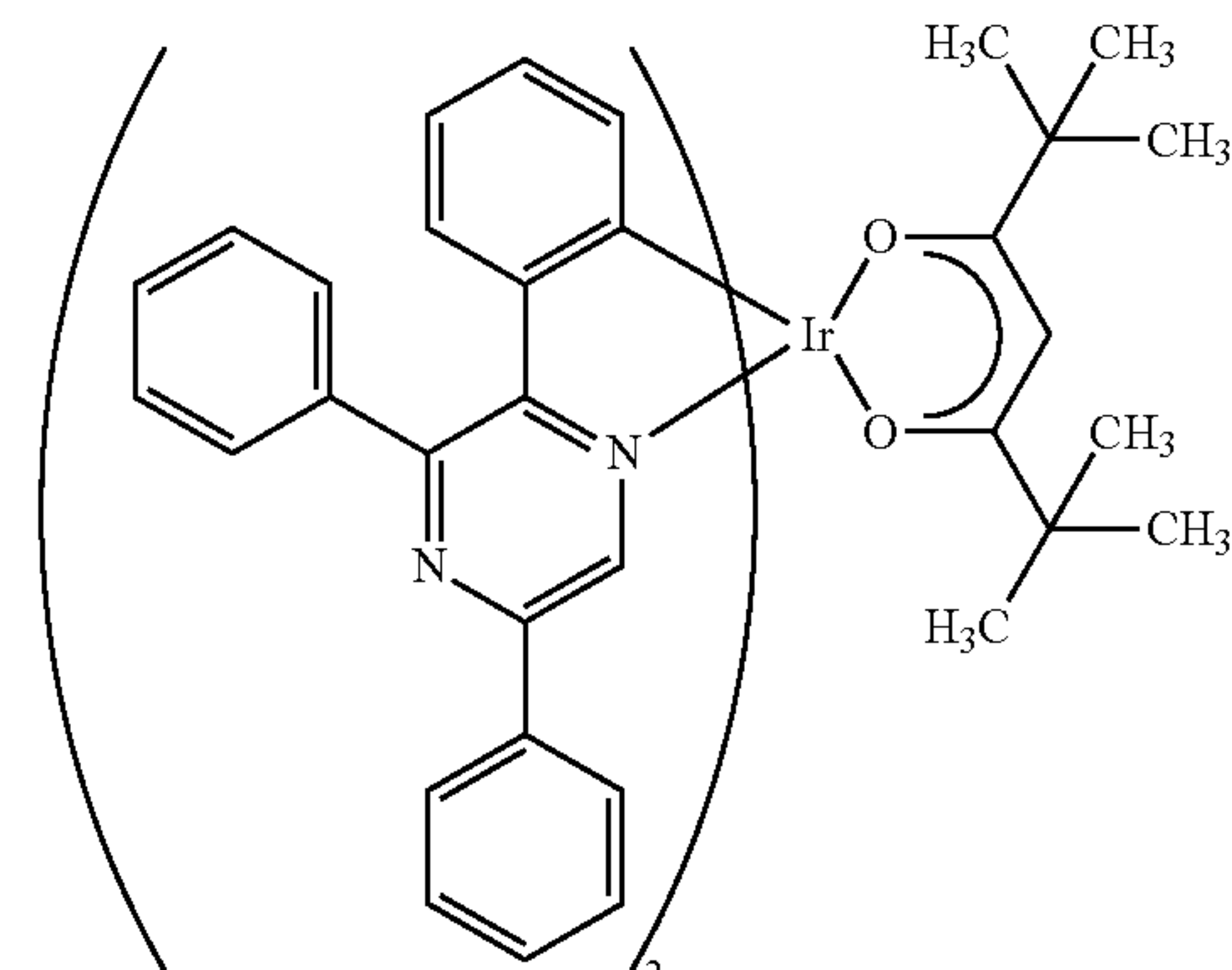
[Ir(tppr) 2 (dpm)]
