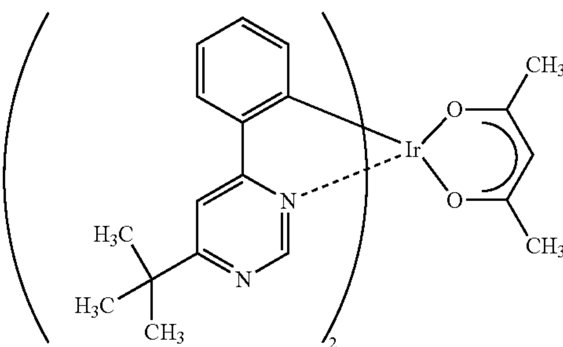
[Ir(tBuppm) 2 (acac)]
