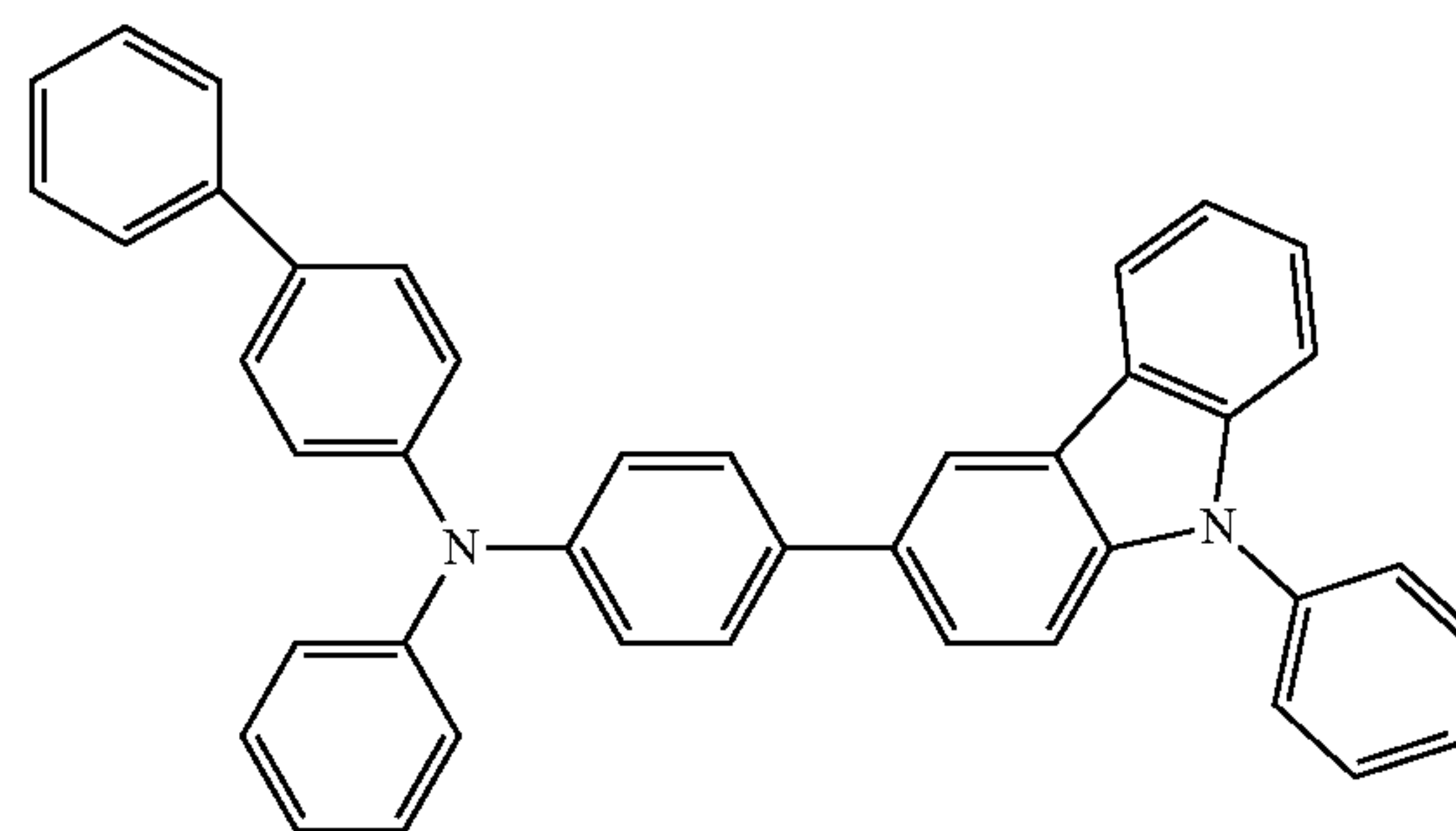
PCBA1BP
