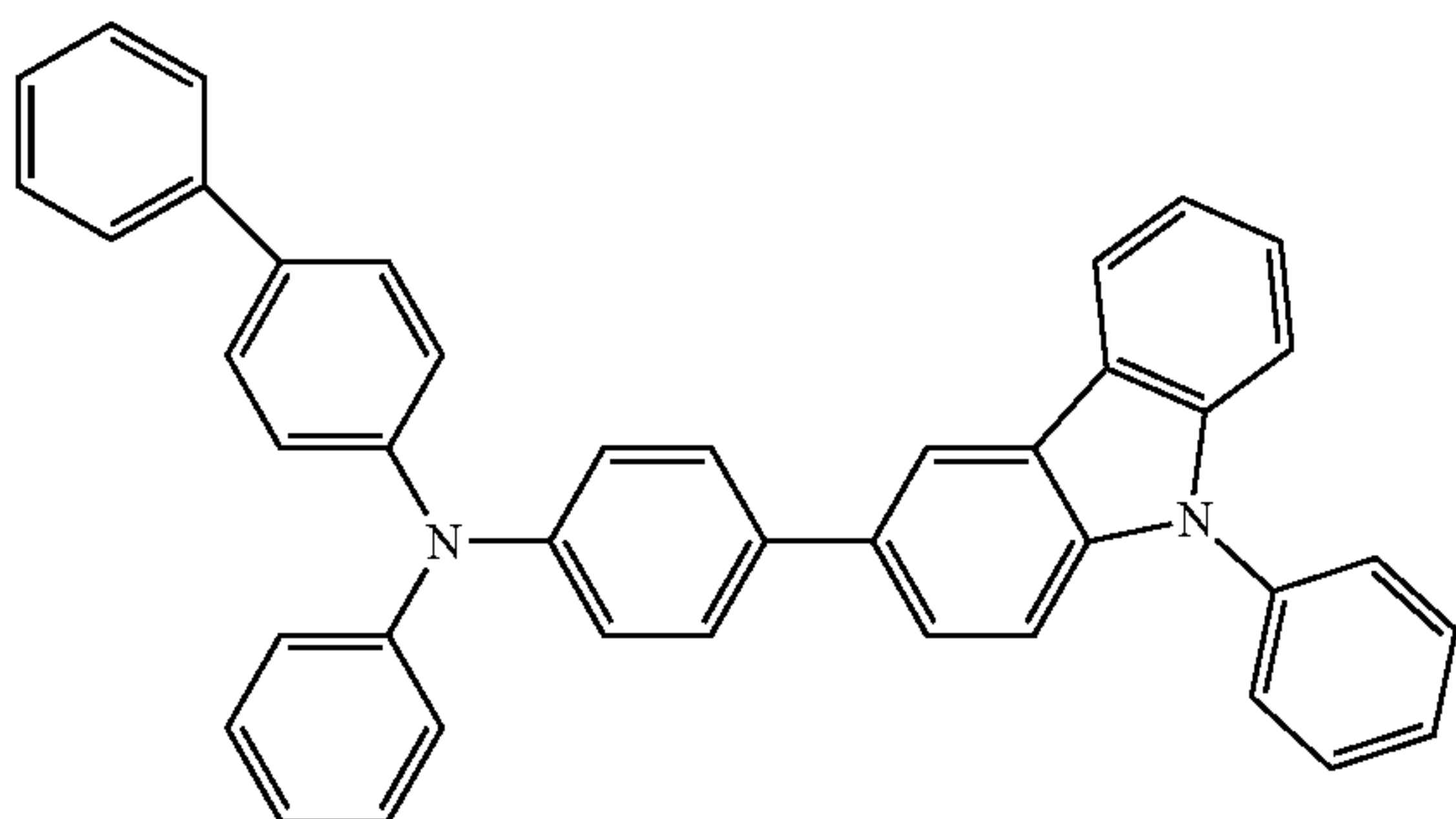
PCBA1BP
