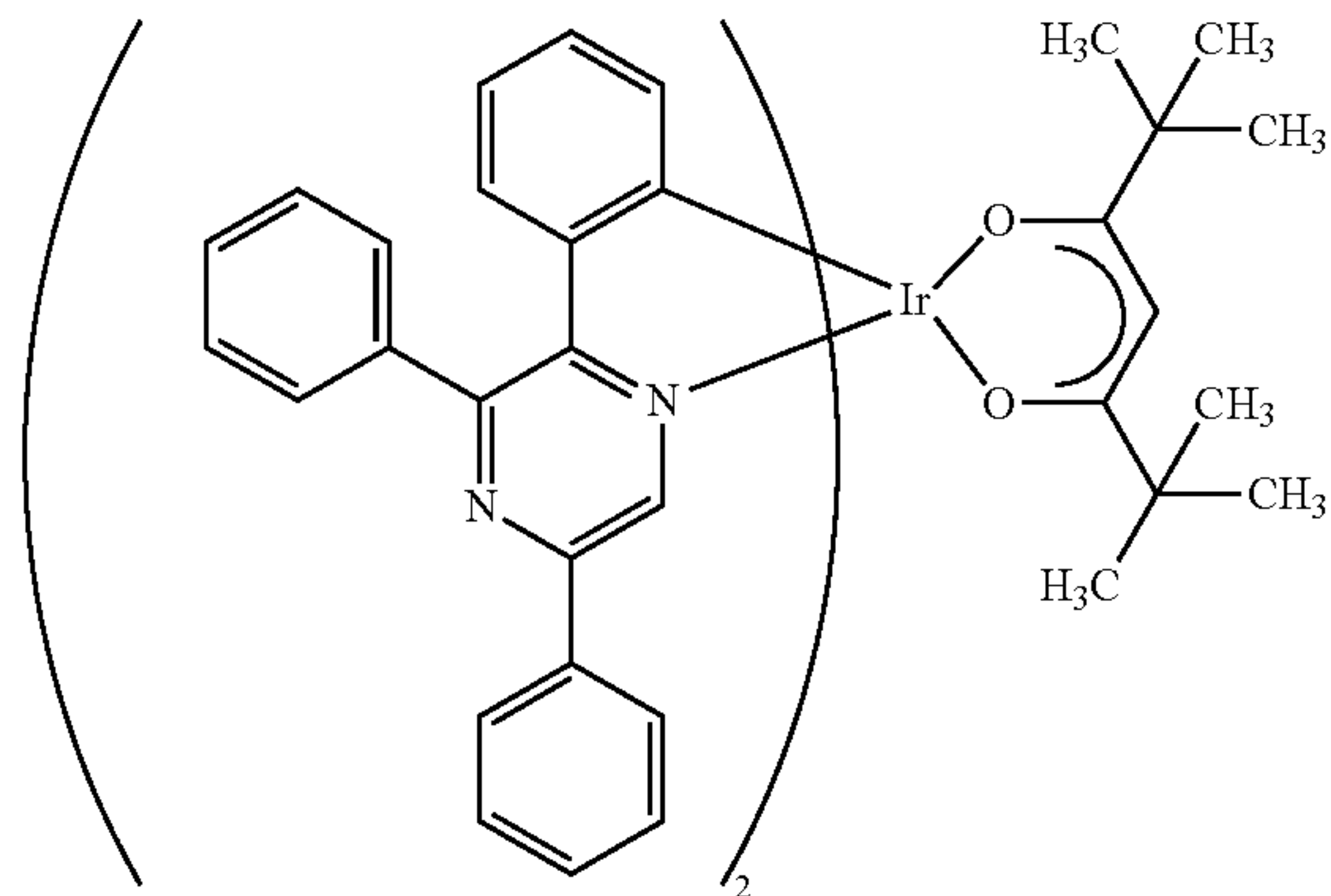
[Ir(tppr) 2 (dpm)]
