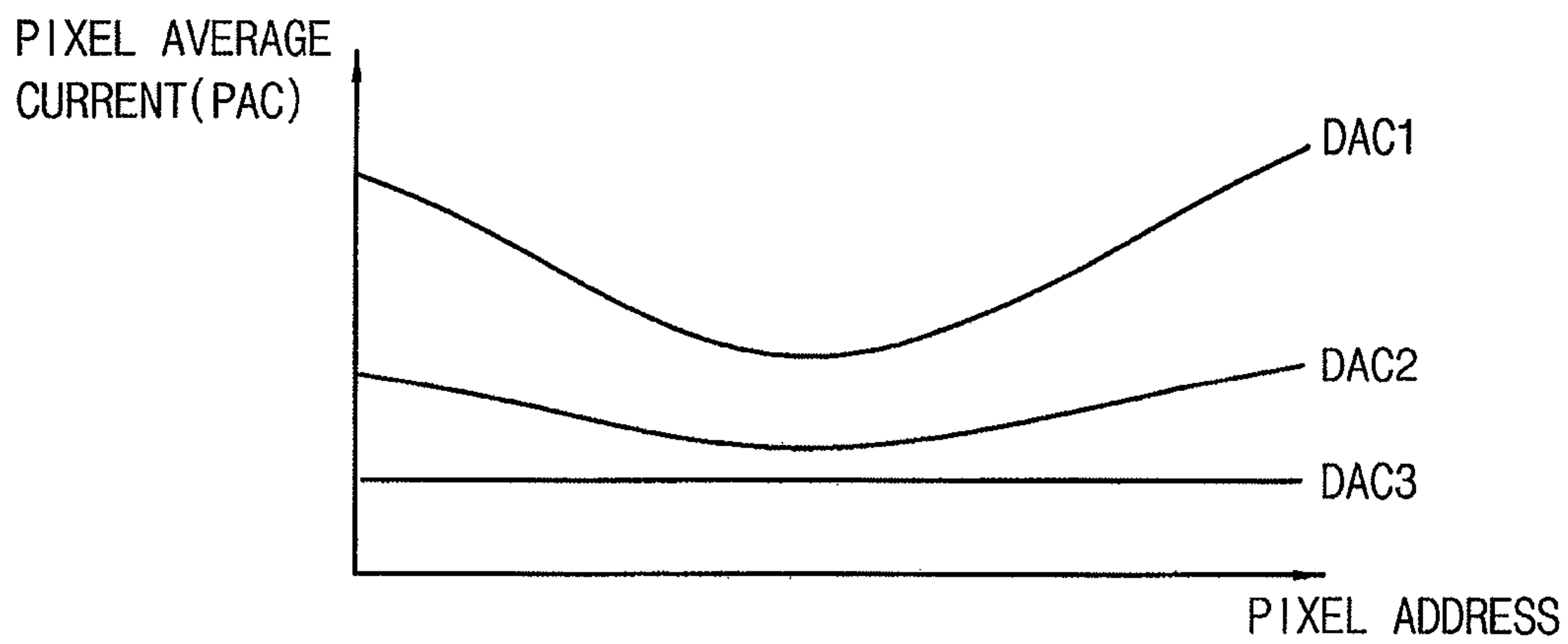
PIXEL AVERAGE CURRENT LUT(PACL T)
