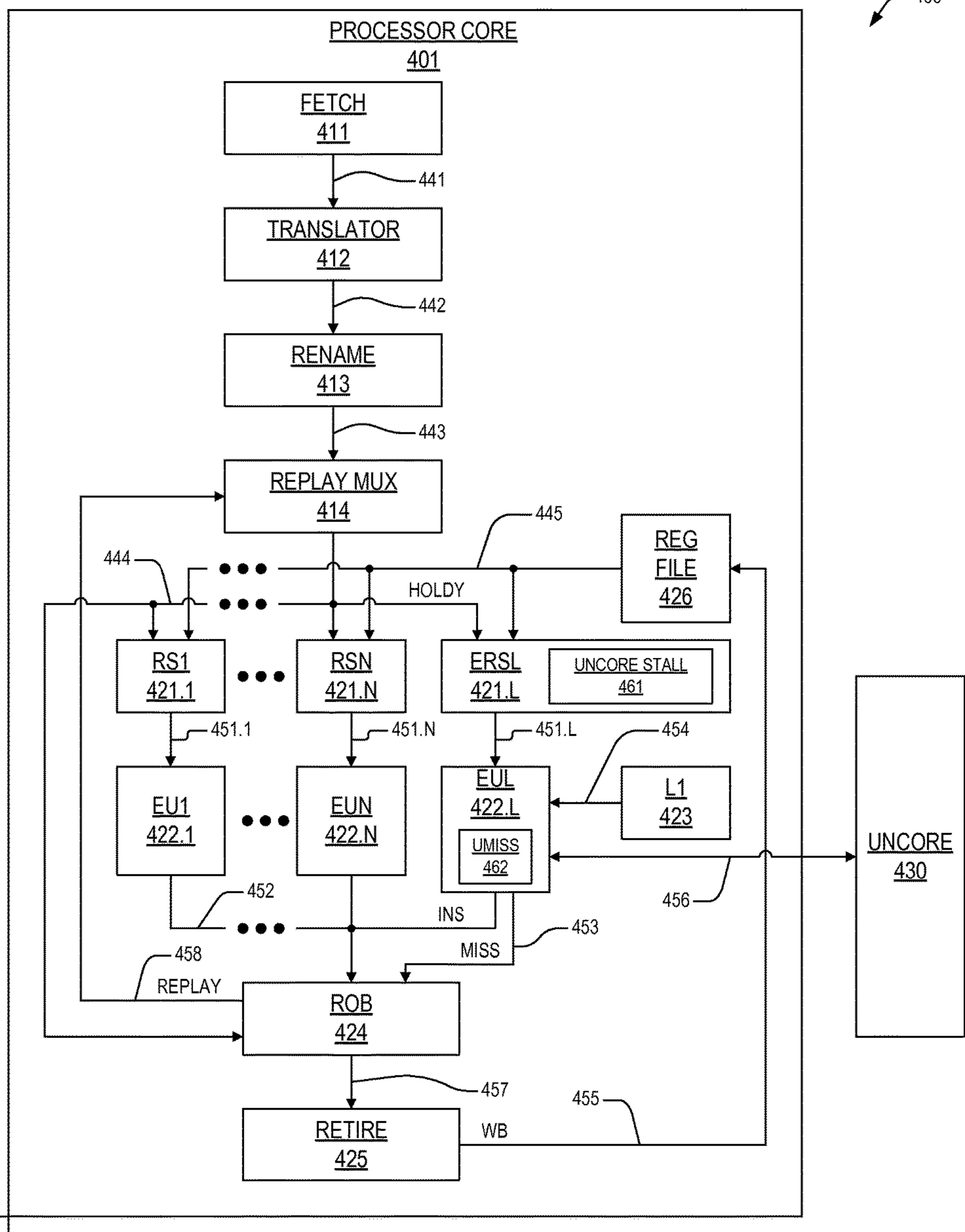
EXEMPLARY CORE STAGES FOR LOAD REPLAY REDUCTION
