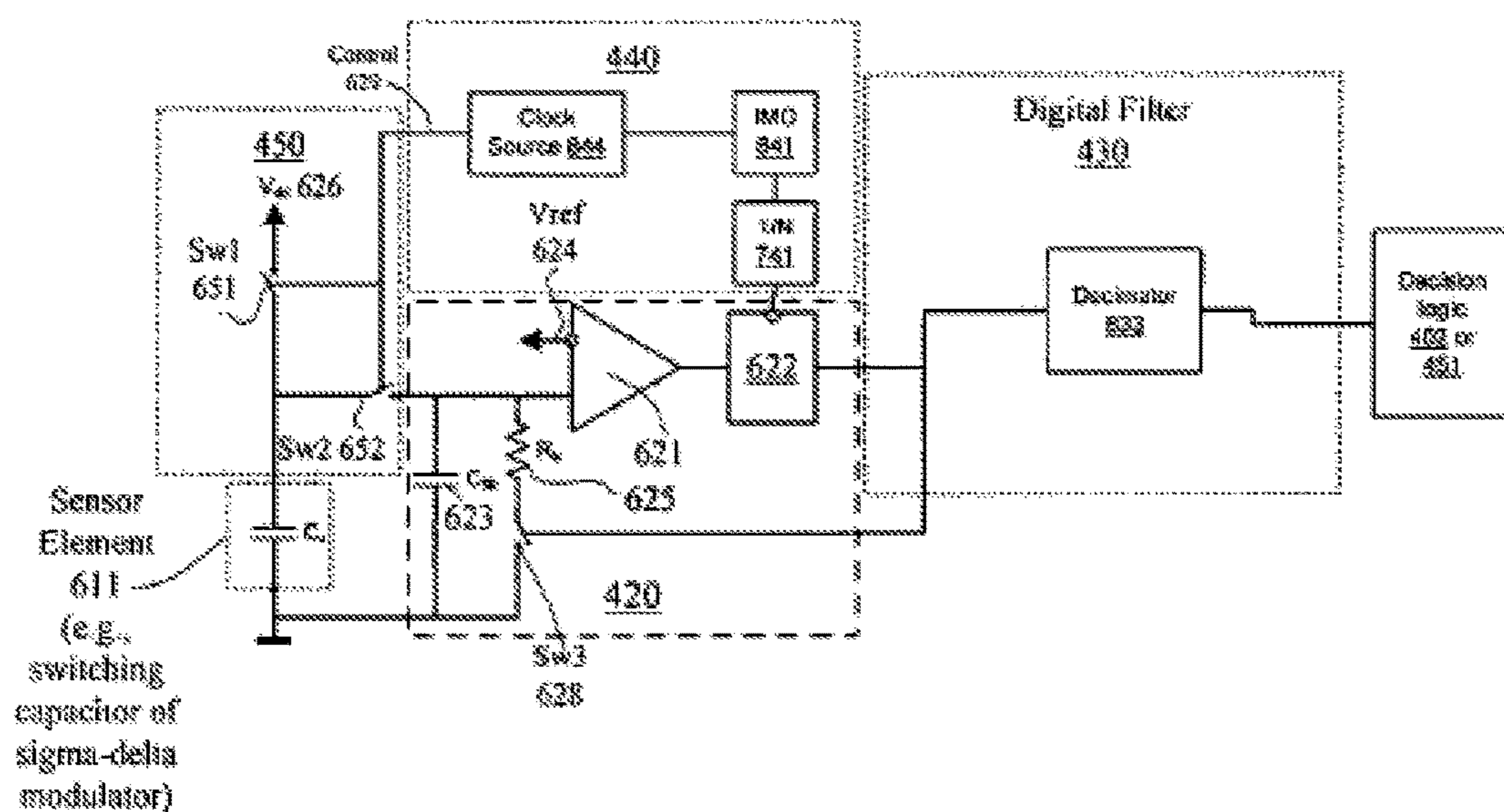
FIG. 22 (Prior Art)
