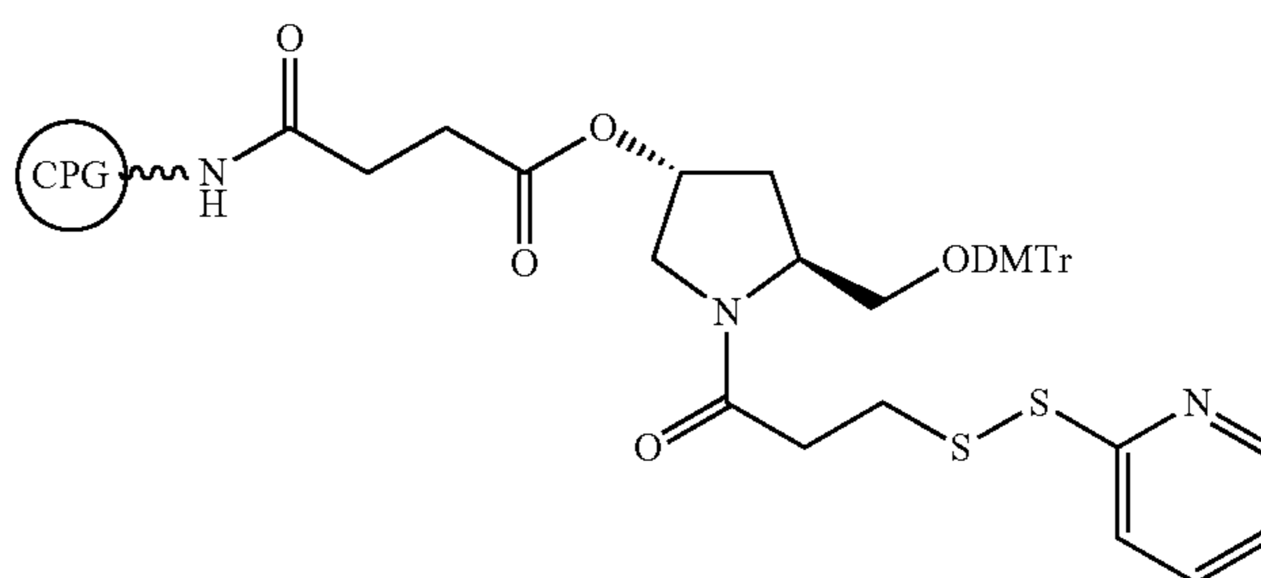
Scheme 9 a
