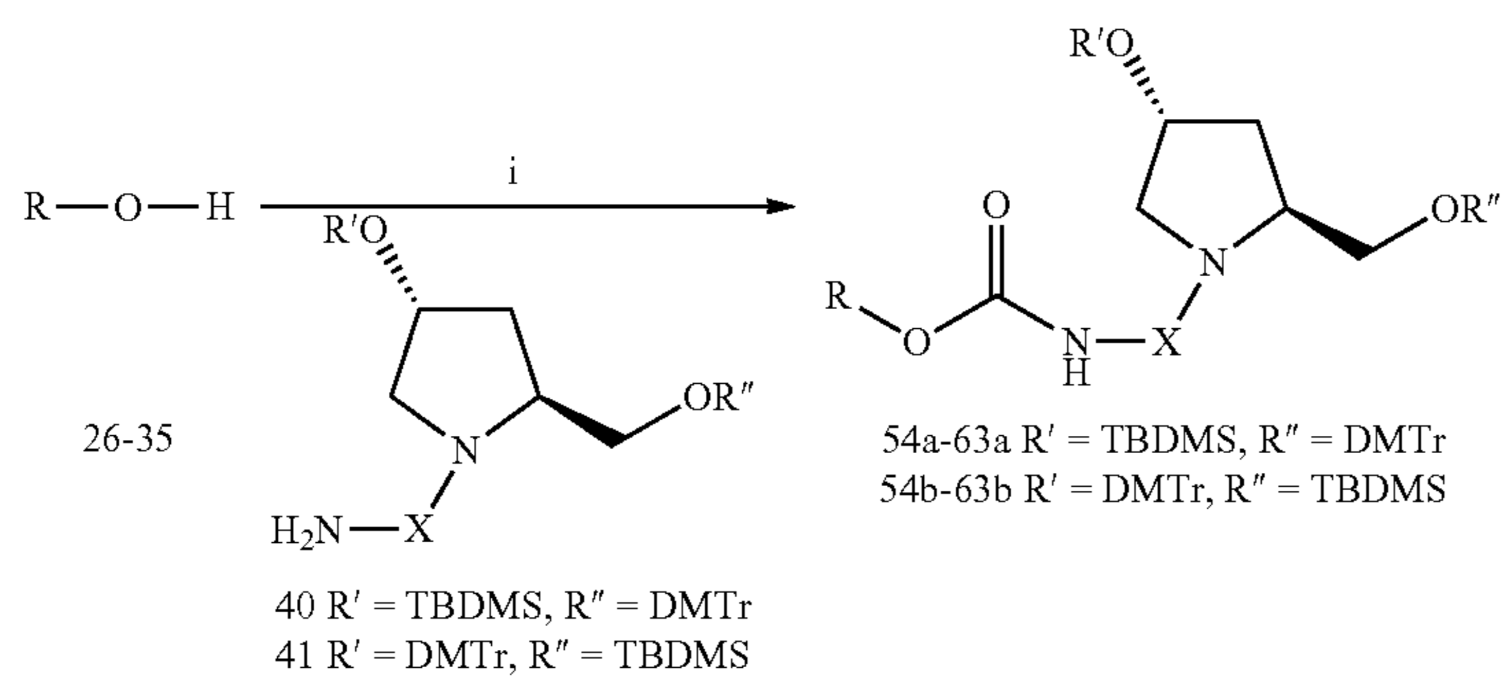
Scheme 7 a
