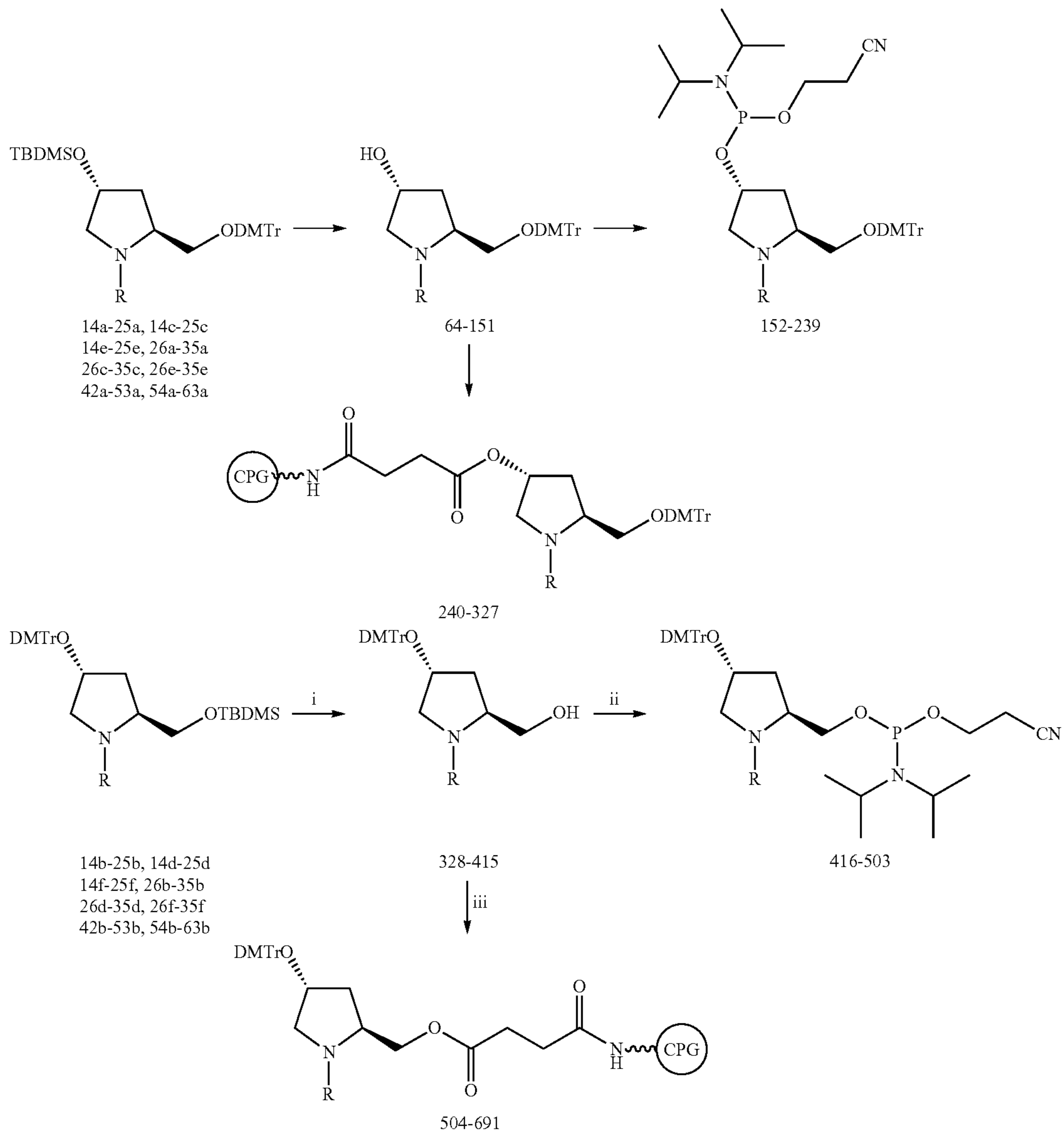
Scheme 8 a
