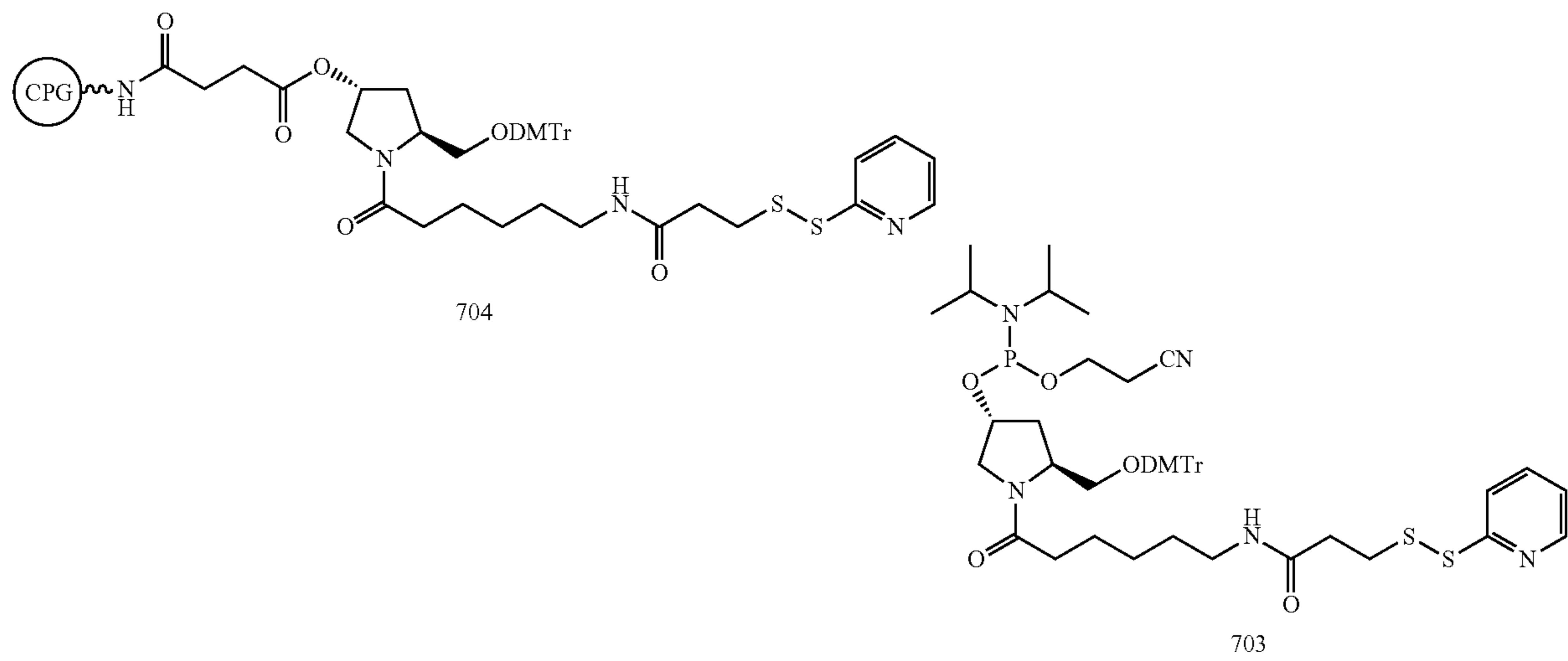
Scheme 10 a
