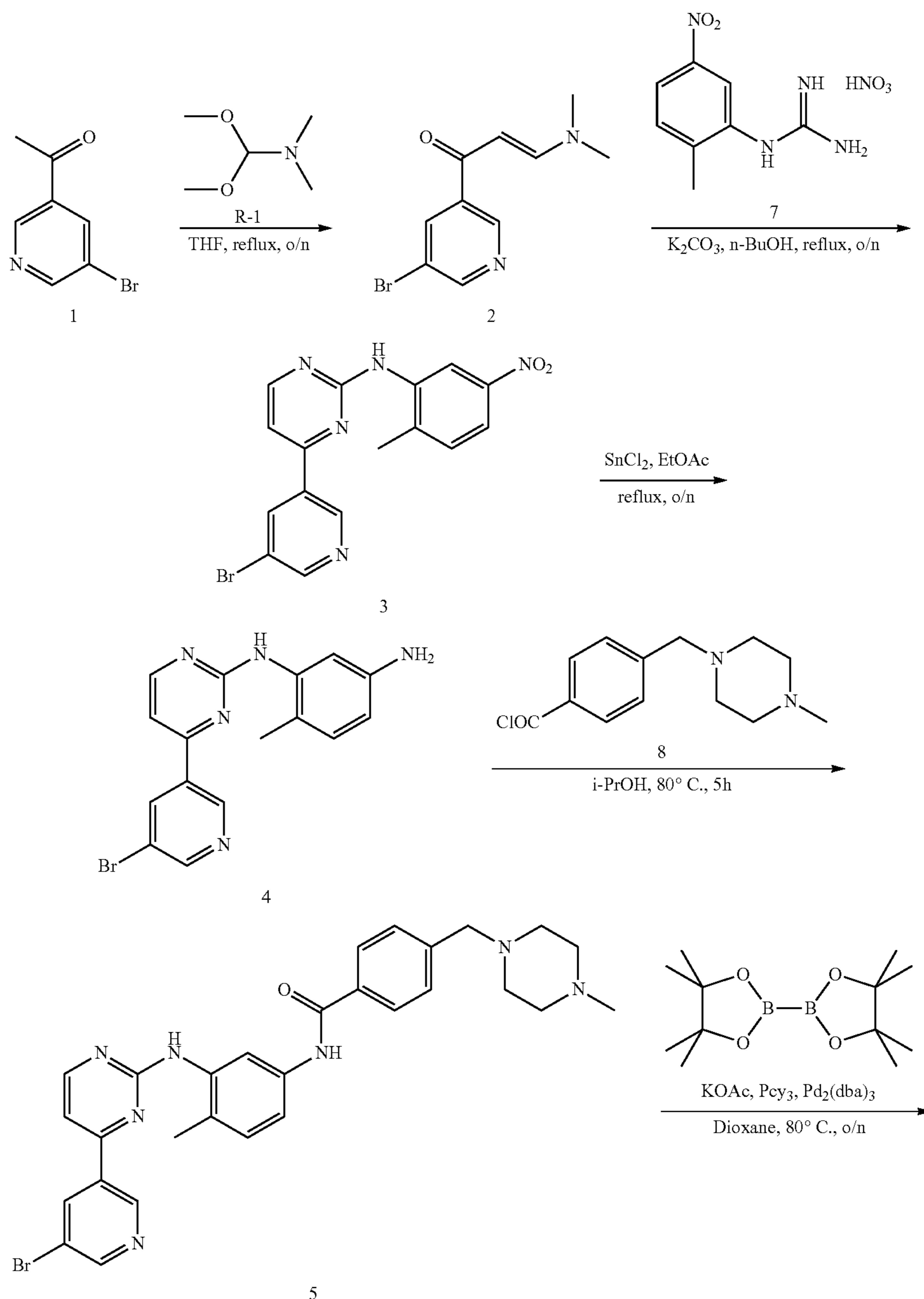
Scheme 1: Synthesis of Intermediates 5 and 6
