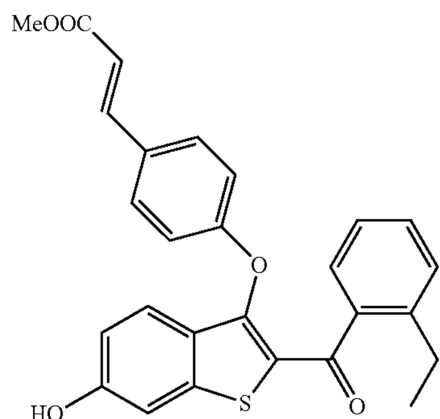
Methyl (E)-3-(4-((2-ethylbenzoyl)-6-hydroxybenzo[b]thiophen-3-yl)oxy)phenyl)acrylate
