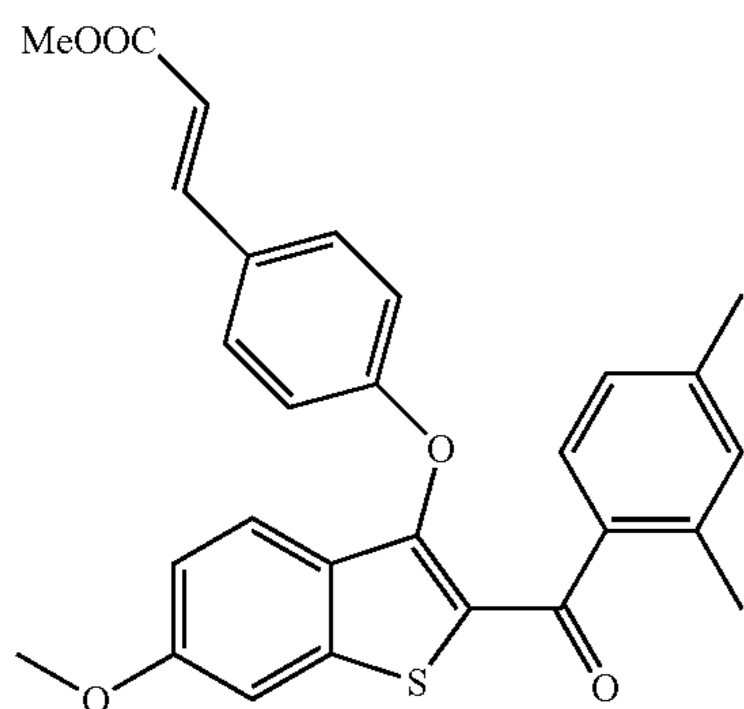
Methyl (E)-3-(4-((2-(2,4-dimethylbenzoyl)-6-methoxybenzo[b]thiophen-3-yl)oxy)phenyl)acrylate
