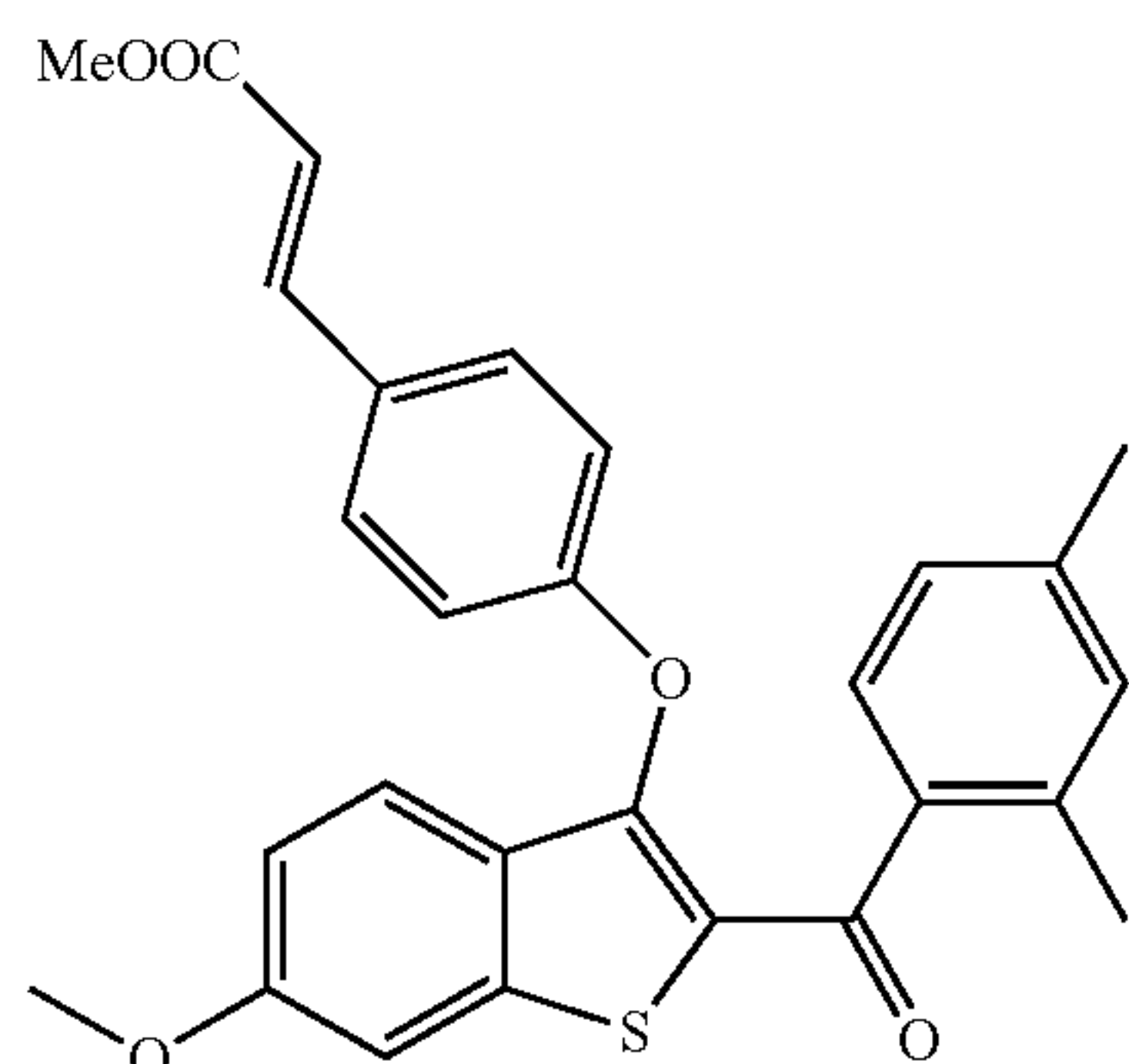
Methyl (E)-3-(4-((2-(2,4-dimethylbenzoyl)-6-methoxybenzo[b]thiophen-3-yl)oxy)phenyl)acrylate
