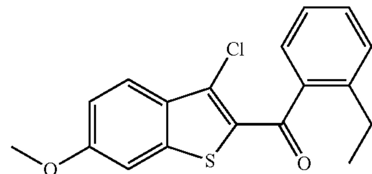
(3-Chloro-6-methoxybenzo[b]thiophen-2-yl)(2-ethylphenyl)methanone
