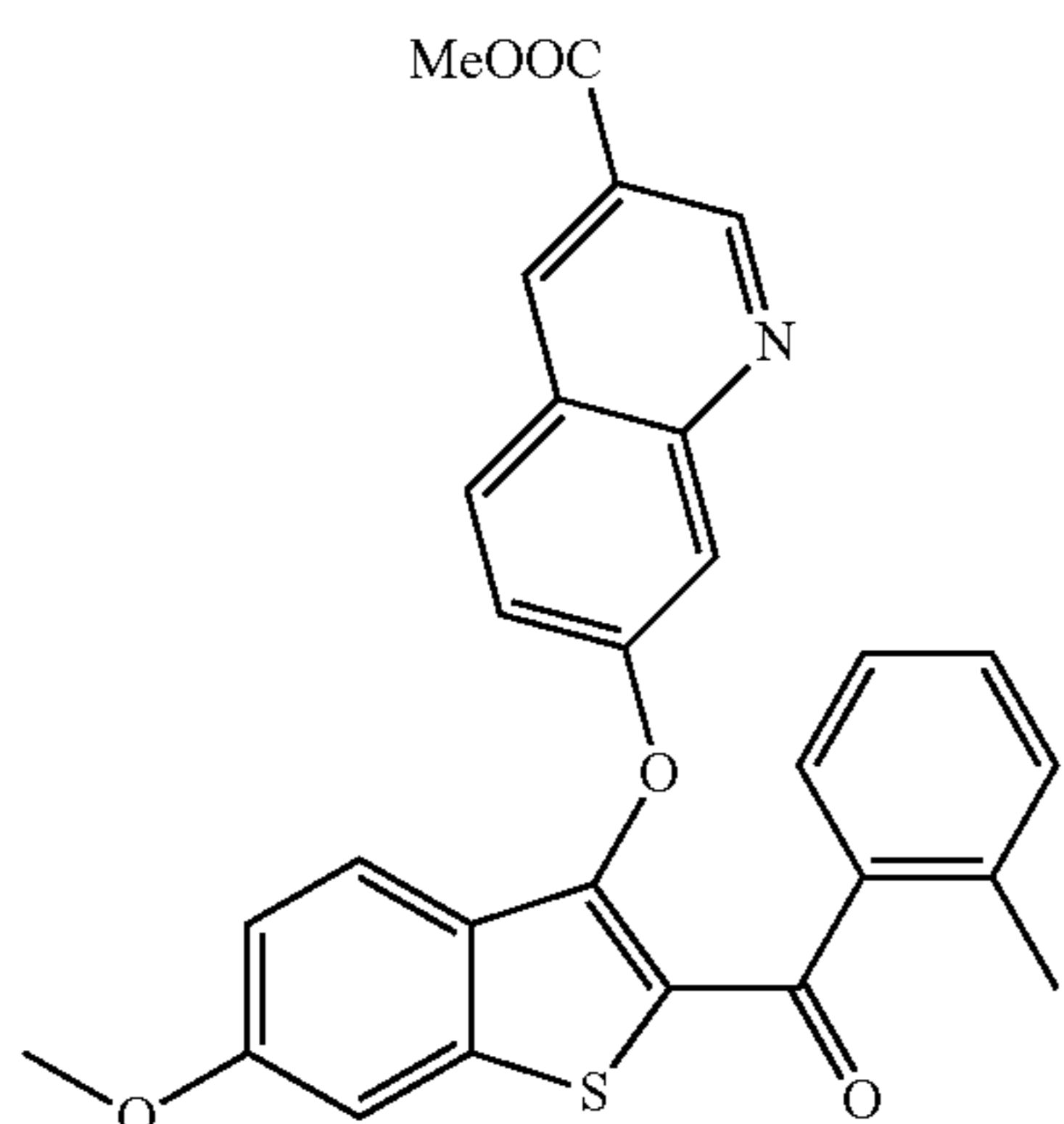
Methyl 7-((6-methoxy-2-(2-methylbenzoyl)benzo[b]thiophen-3-yl)oxy)quinoline-3-carboxylate
