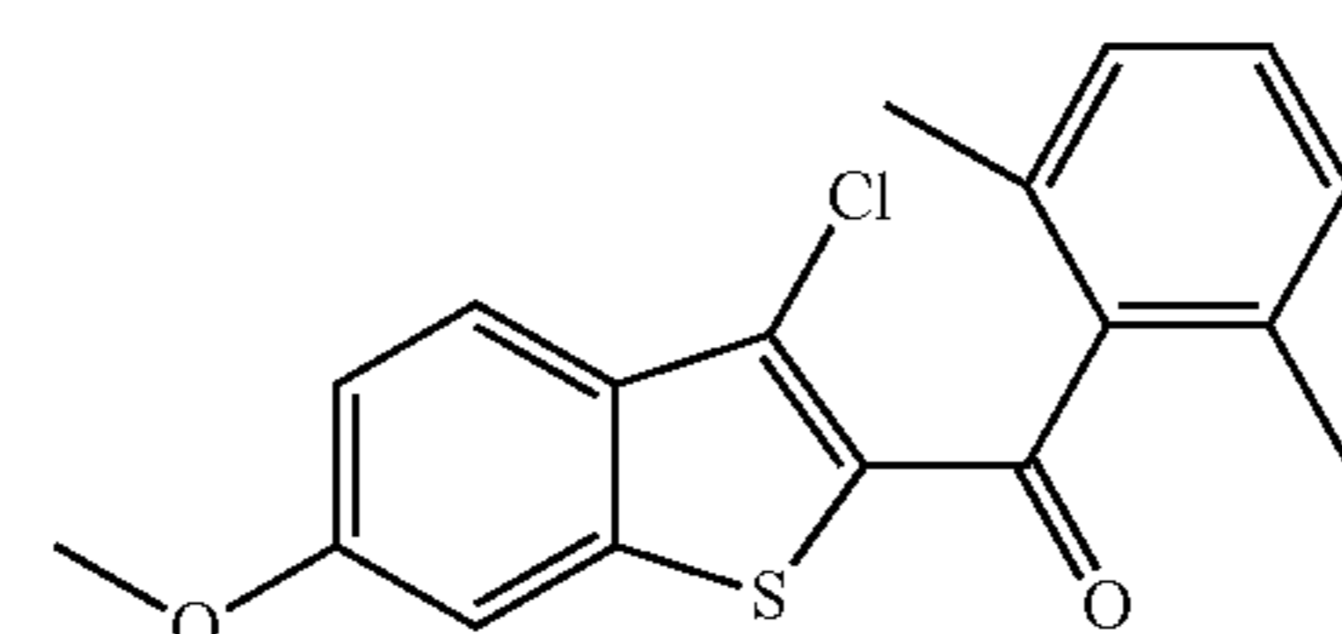
(3-Chloro-6-methoxybenzo[b]thiophen-2-yl)(2,6-dimethylphenyl)methanone
