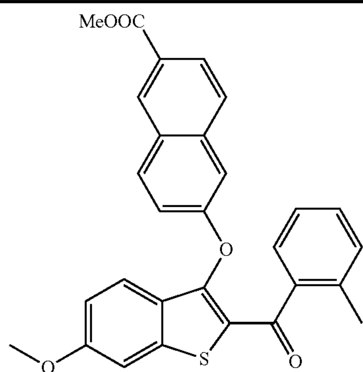
Methyl 6-((6-methoxy-2-(2-methylbenzoyl)benzo[b]thiophen-3-yl)oxy)-2-naphthoate
