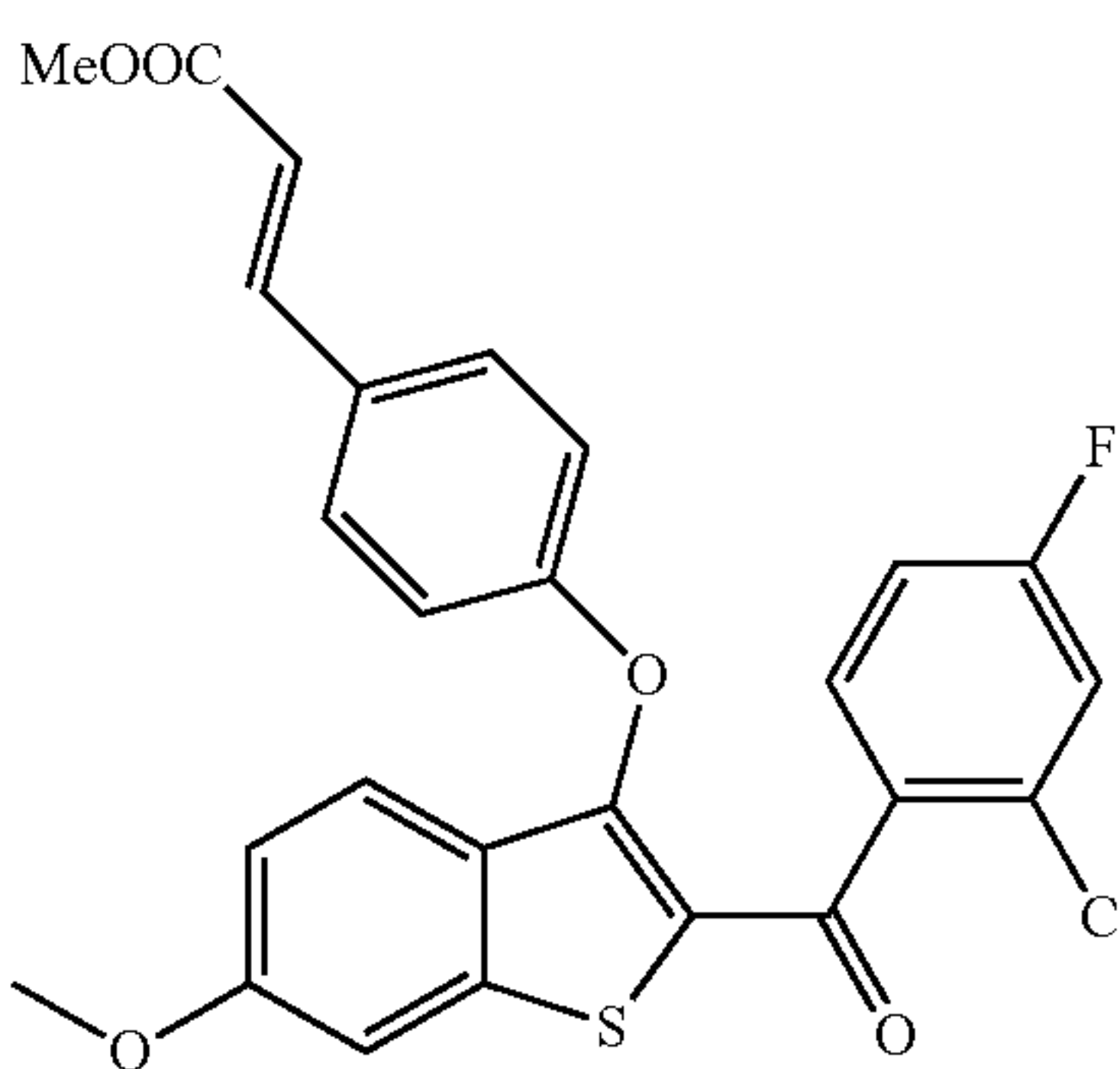
Methyl (E)-3-(4-((2-(2-chloro-4-fluorobenzoyl)-6-methoxybenzo[b]thiophen-3-yl)oxy)phenyl)acrylate
