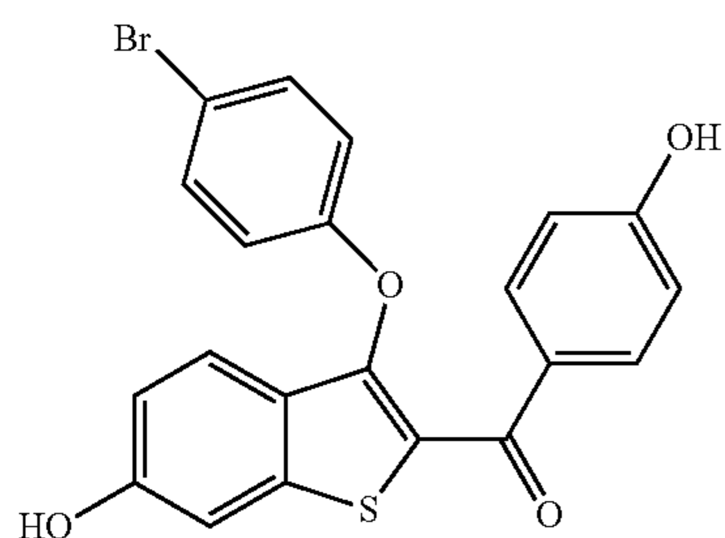
(3-(4-bromophenoxy)-6-hydroxybenzo[b]thiophen-2-yl)(4-hydroxyphenyl)methanone
