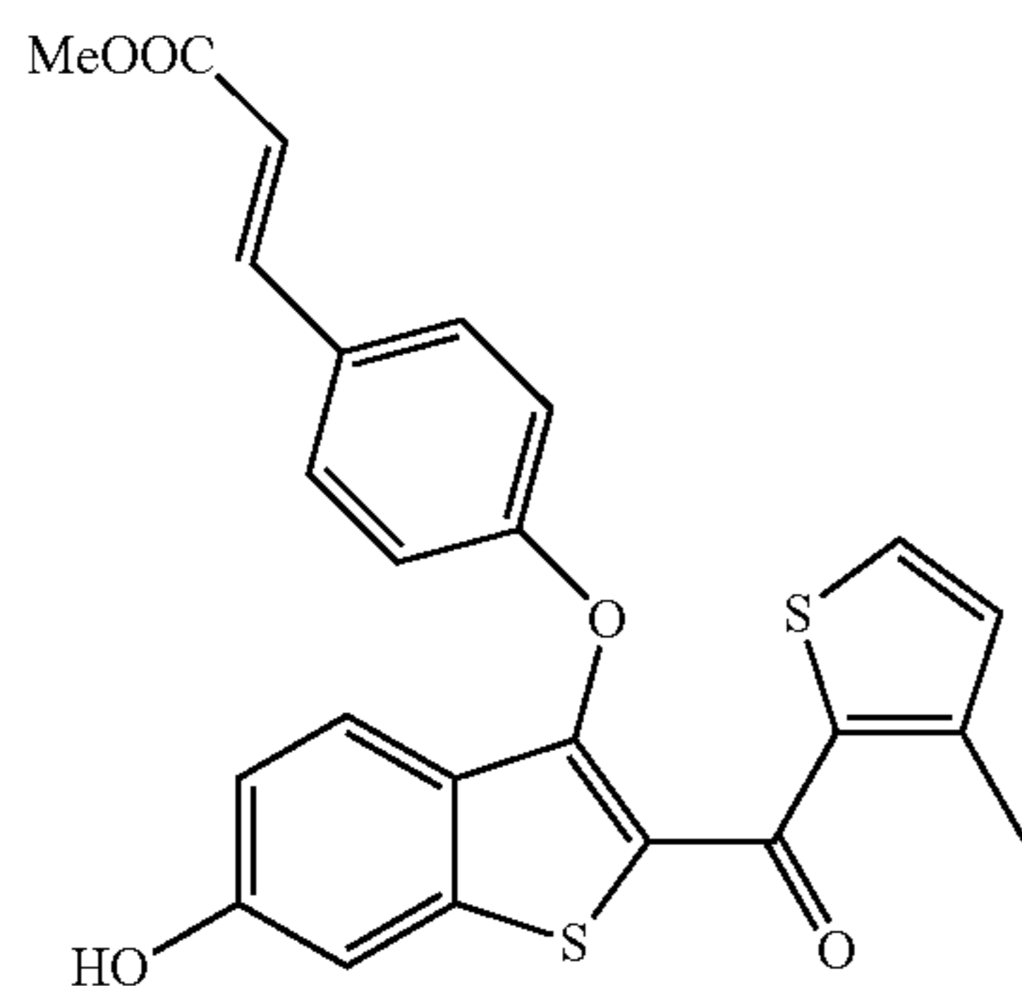
Methyl (E)-3-(4-((6-hydroxy-2-(3-methylthiophene-2-carbonyl)benzo[b]thiophen-3-yl)oxy)phenyl)acrylate
