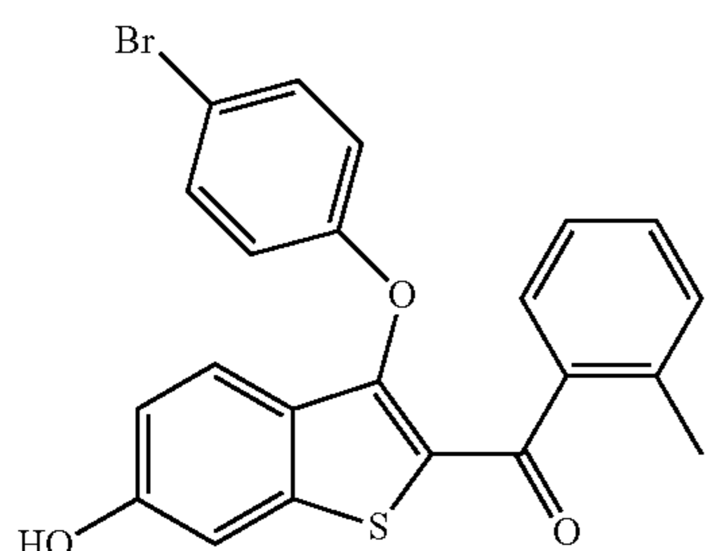
(3-(4-bromophenoxy)-6-hydroxybenzo[b]thiophen-2-yl)(o-tolyl)methanone
