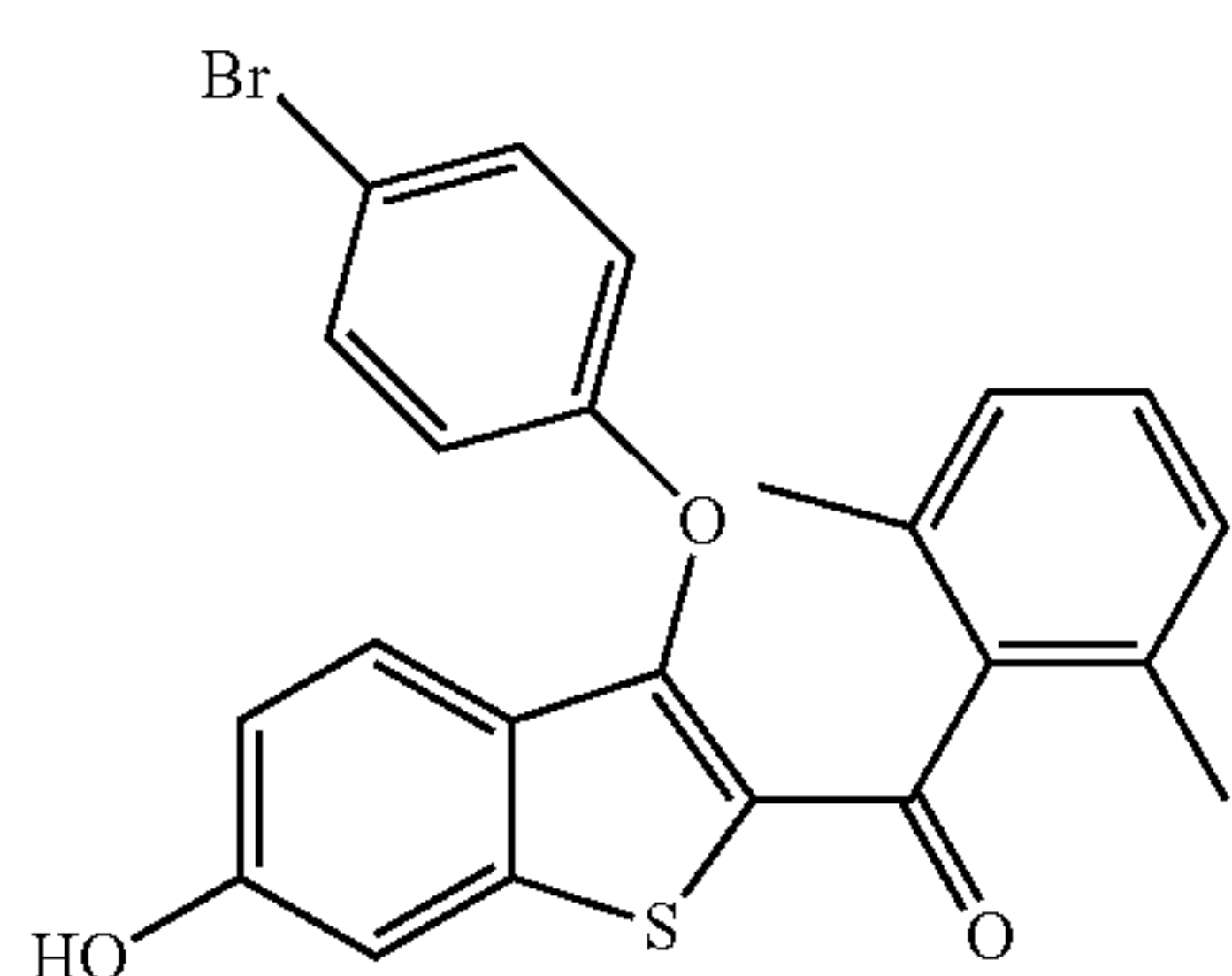
(3-(4-Bromophenoxy)-6-hydroxybenzo[b]thiophen-2-yl)(2,6-dimethylphenyl)methanone
