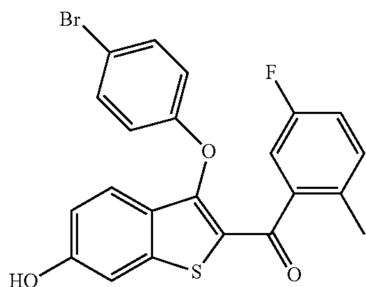
(3-(4-bromophenoxy)-6-hydroxybenzo[b]thiophen-2-yl)(5-fluoro-2-methylphenyl)methanone
