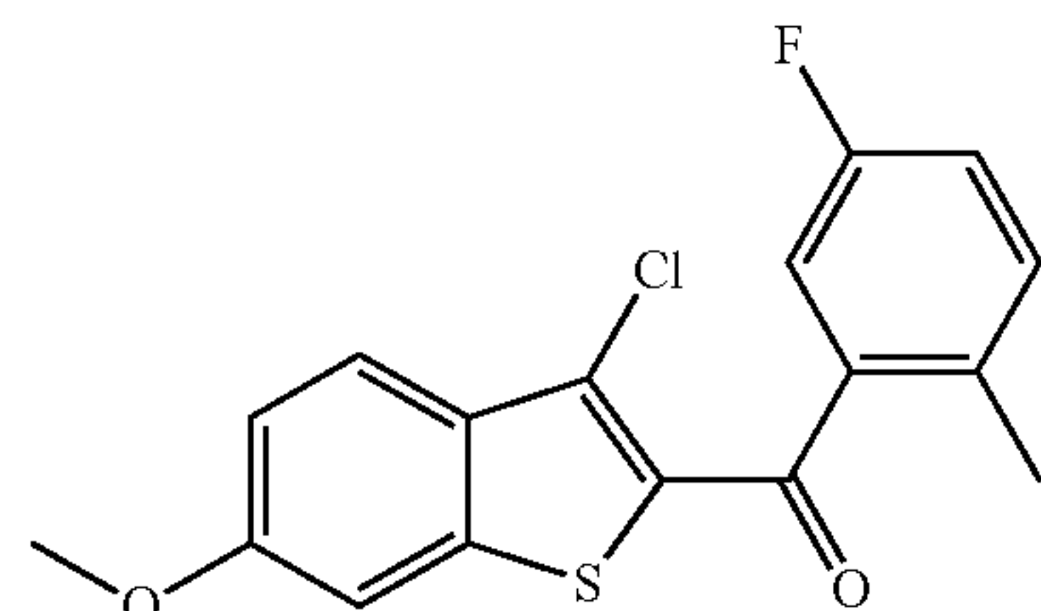
(3-chloro-6-methoxybenzo[b]thiophen-2-yl)(5-fluoro-2-methylphenyl)methanone
