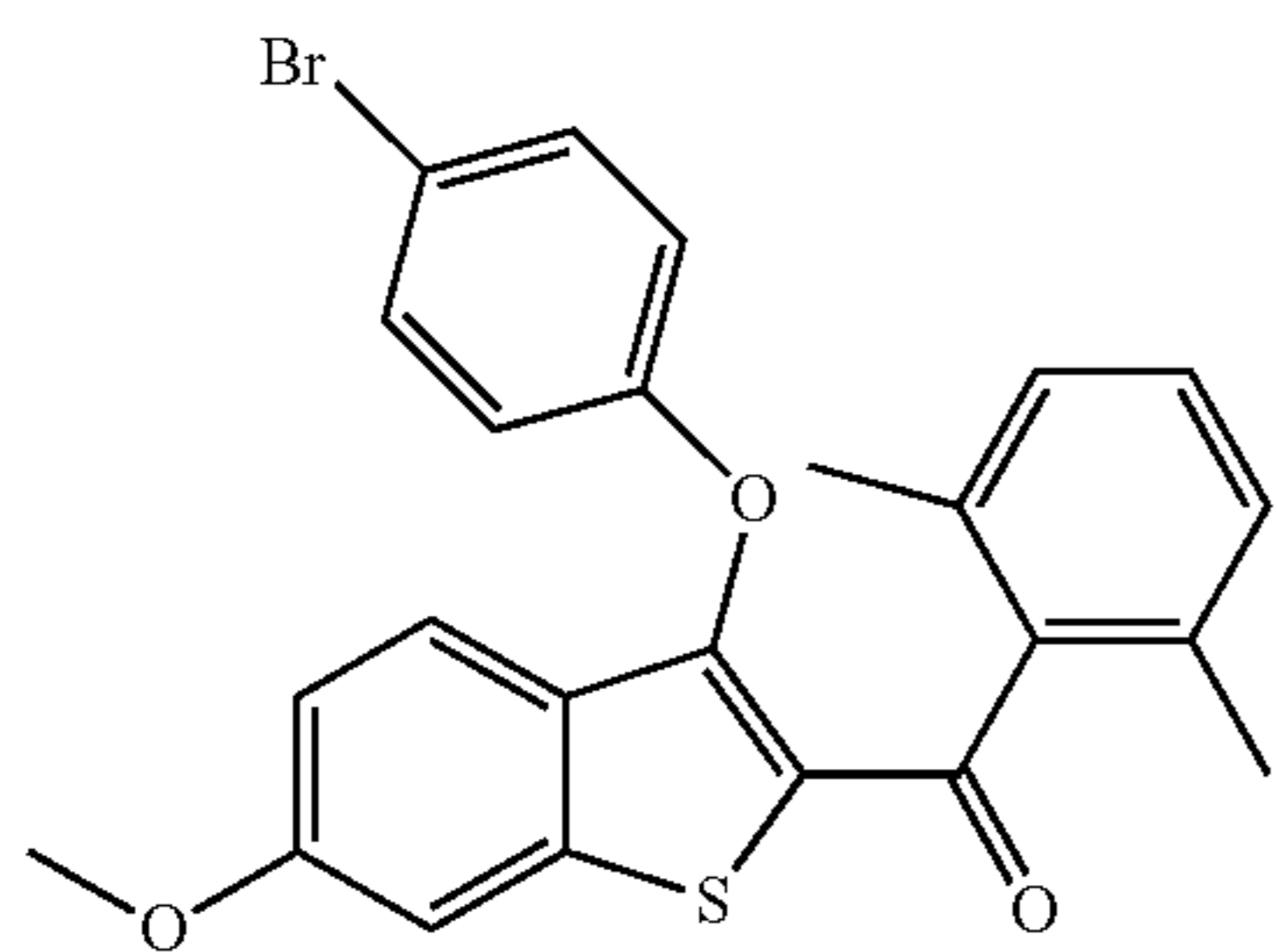
(3-(4-Bromophenoxy)-6-methoxybenzo[b]thiophen-2-yl)(2,6-dimethylphenyl)methanone
