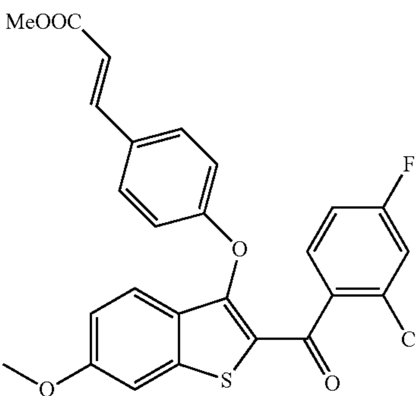
Methyl (E)-3-(4-((2-(2-chloro-4-fluorobenzoyl)-6-methoxybenzo[b]thiophen-3-yl)oxy)phenyl)acrylate
