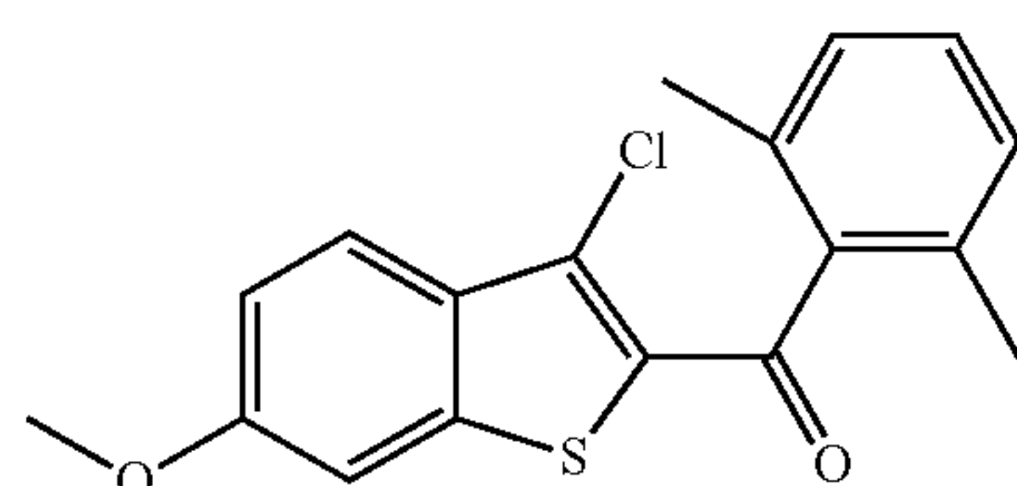
(3-Chloro-6-methoxybenzo[b]thiophen-2-yl)(2,6-dimethylphenyl)methanone
