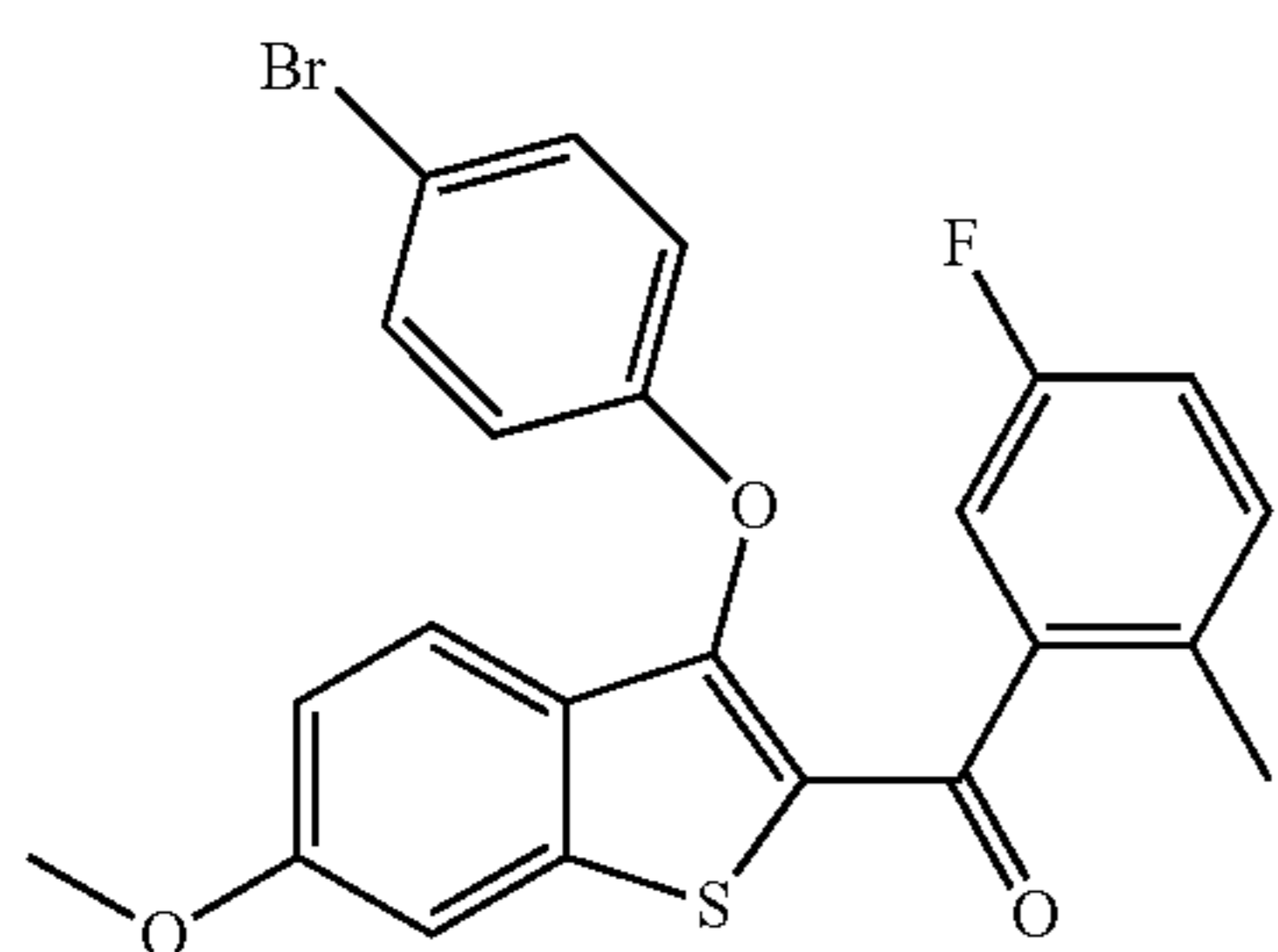
(3-(4-Bromophenoxy)-6-methoxybenzo[b]thiophen-2-yl)(5-fluoro-2-methylphenyl)methanone
