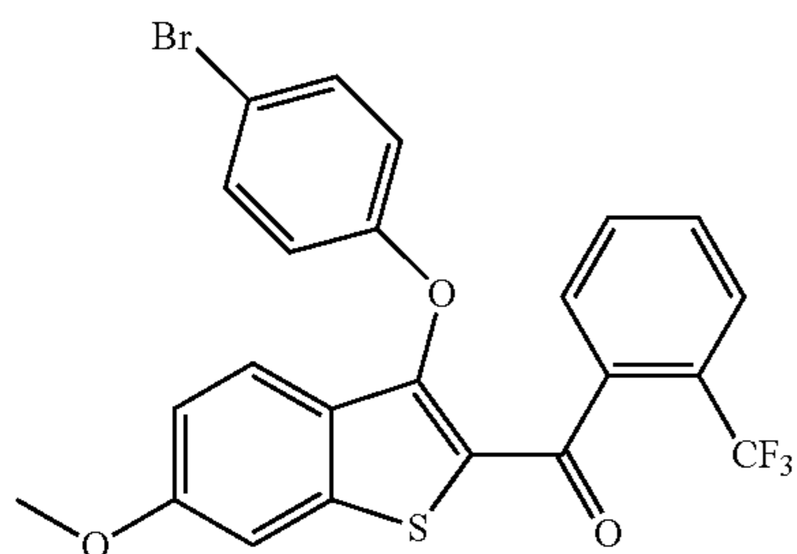
(3-(4-Bromophenoxy)-6-methoxybenzo[b]thiophen-2-yl)(2-(trifluoromethyl)phenyl)methanone
