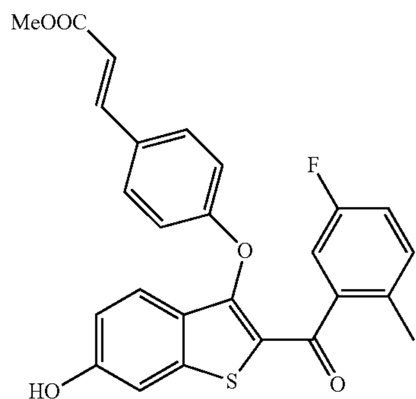
Methyl (E)-3-(4-((2-(5-fluoro-2-methylbenzoyl)-6-hydroxybenzo[b]thiophen-3-yl)oxy)phenyl)acrylate
