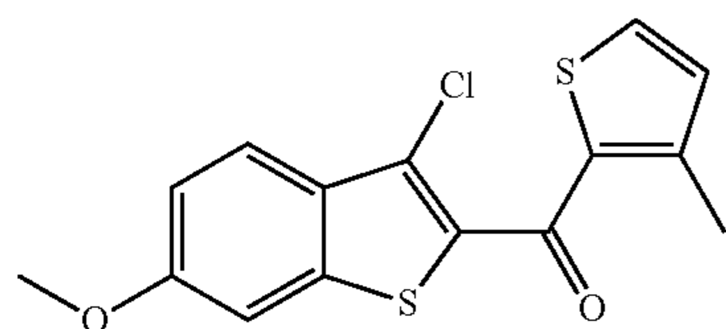
(3-chloro-6-methoxybenzo[b]thiophen-2-yl)(3-methylthiophen-2-yl)methanone
