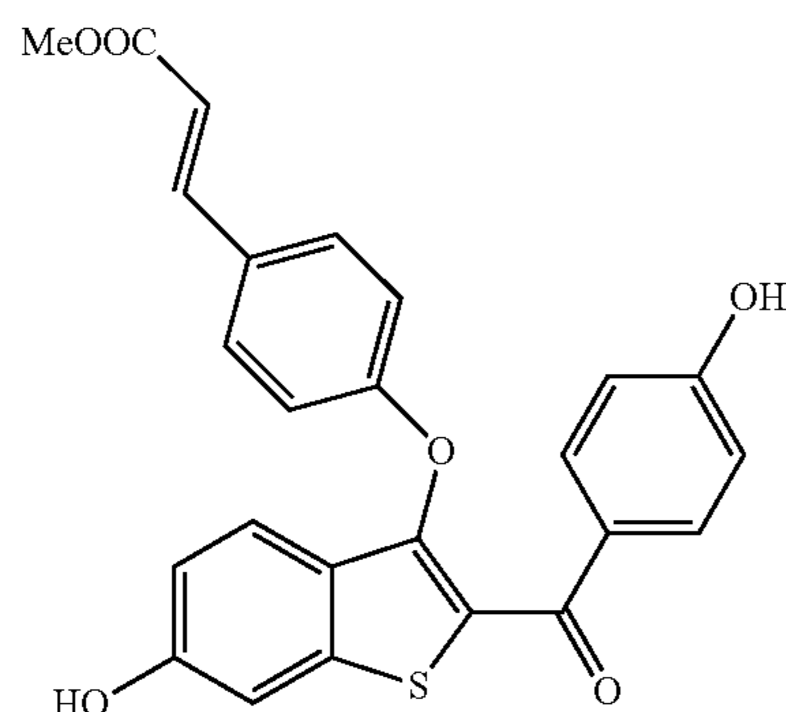
Methyl (E)-3-(4-((6-hydroxy-2-(4-hydroxybenzoyl)benzo[b]thiophen-3-yl)oxy)phenyl)acrylate
