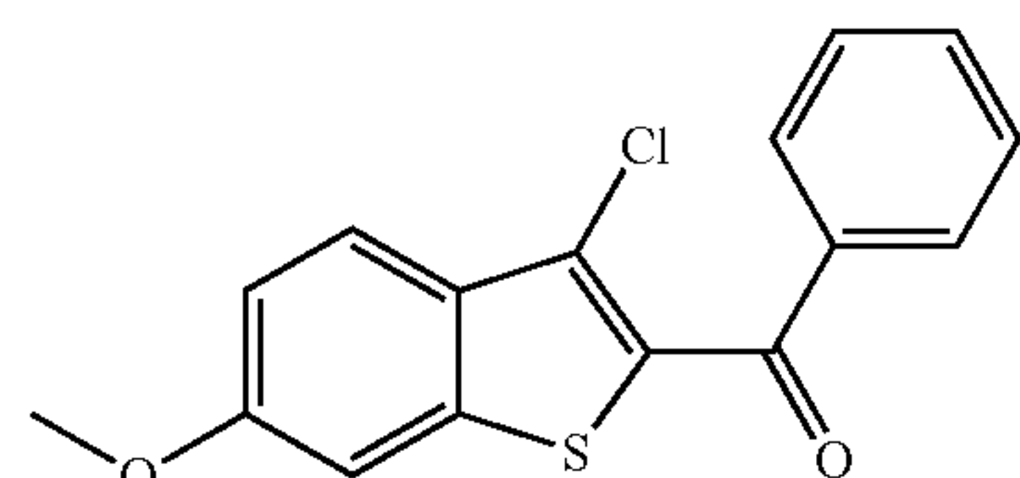
(3-Chloro-6-methoxybenzo[b]thiophen-2-yl)(phenyl)methanone
