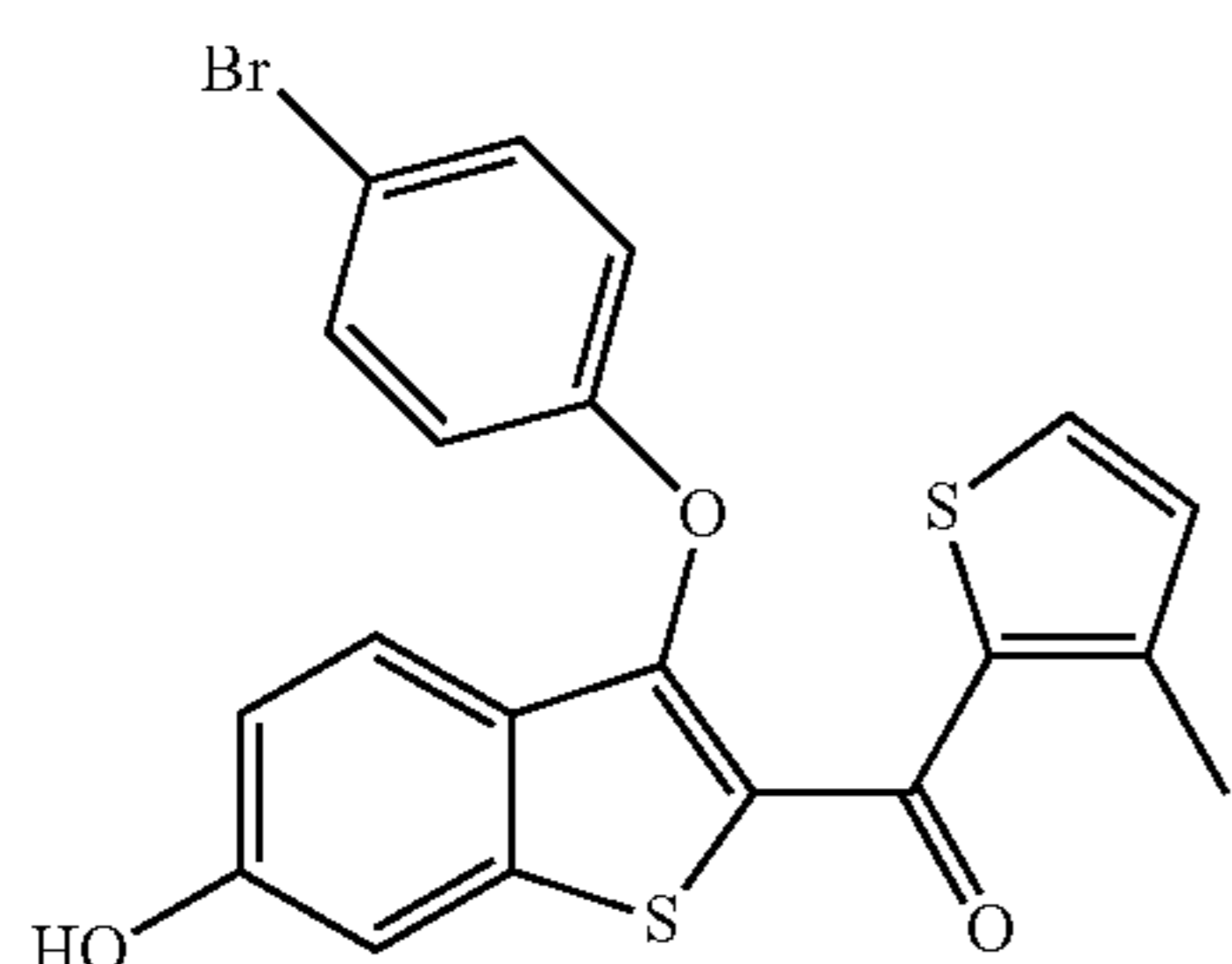
(3-(4-bromophenoxy)-6-hydroxybenzo[b]thiophen-2-yl)(3-methylthiophen-2-yl)methanone
