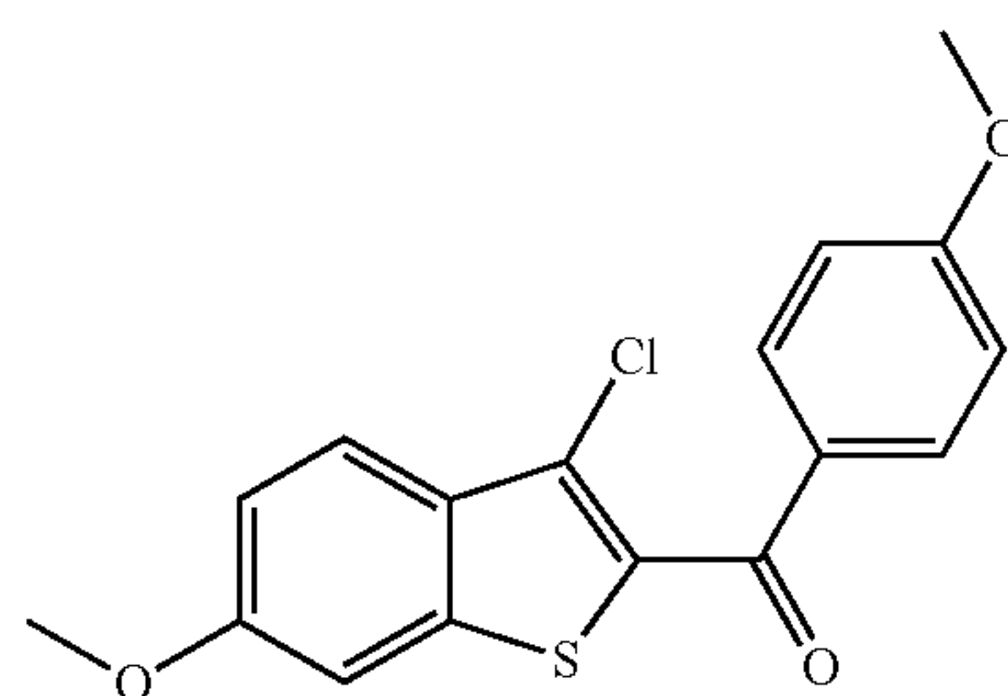
(3-Chloro-6-methoxybenzo[b]thiophen-2-yl)(4-methoxyphenyl)methanone
