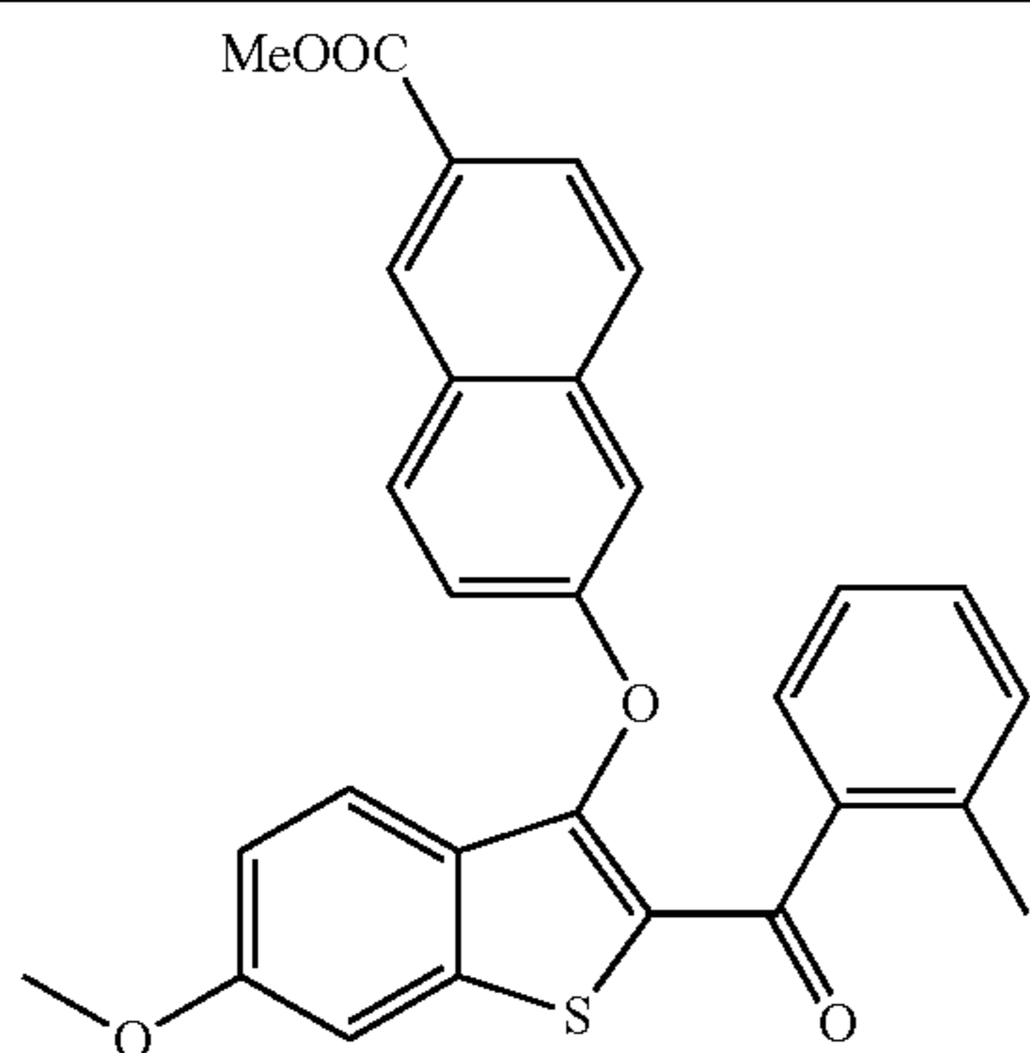
Methyl 6-((6-methoxy-2-(2-methylbenzoyl)benzo[b]thiophen-3-yl)oxy)-2-naphthoate
