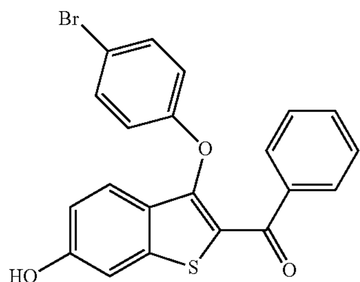
(3-(4-bromophenoxy)-6-hydroxybenzo[b]thiophen-2-yl)(phenyl)methanone
