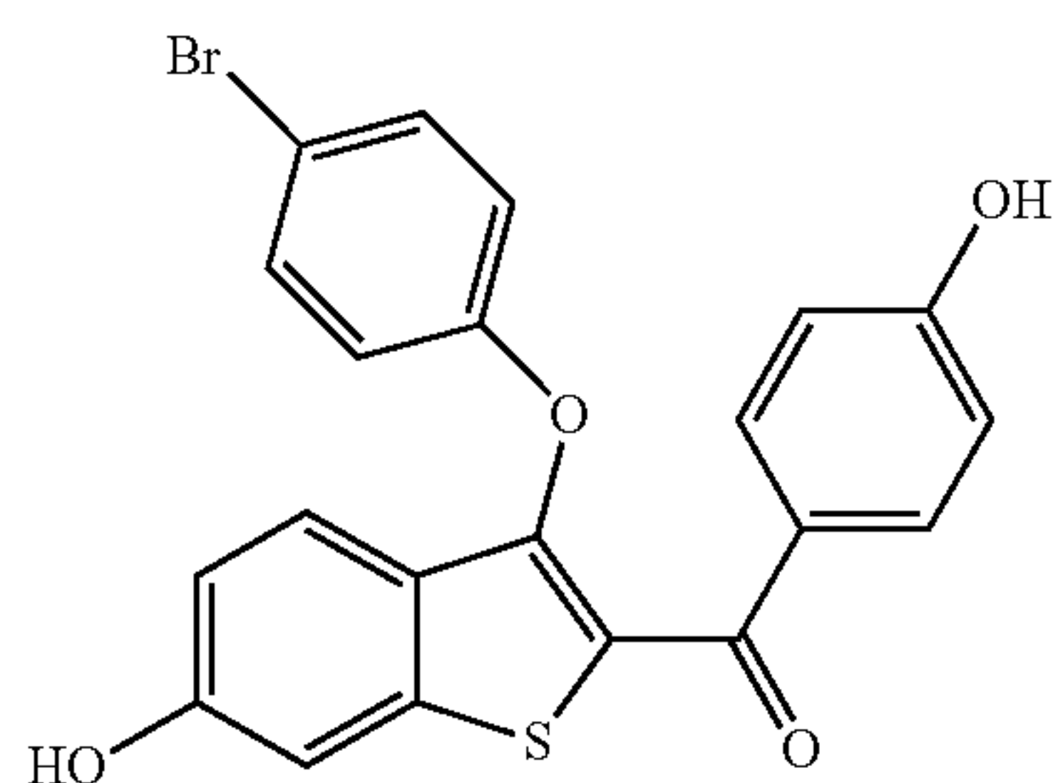
(3-(4-bromophenoxy)-6-hydroxybenzo[b]thiophen-2-yl)(4-hydroxyphenyl)methanone
