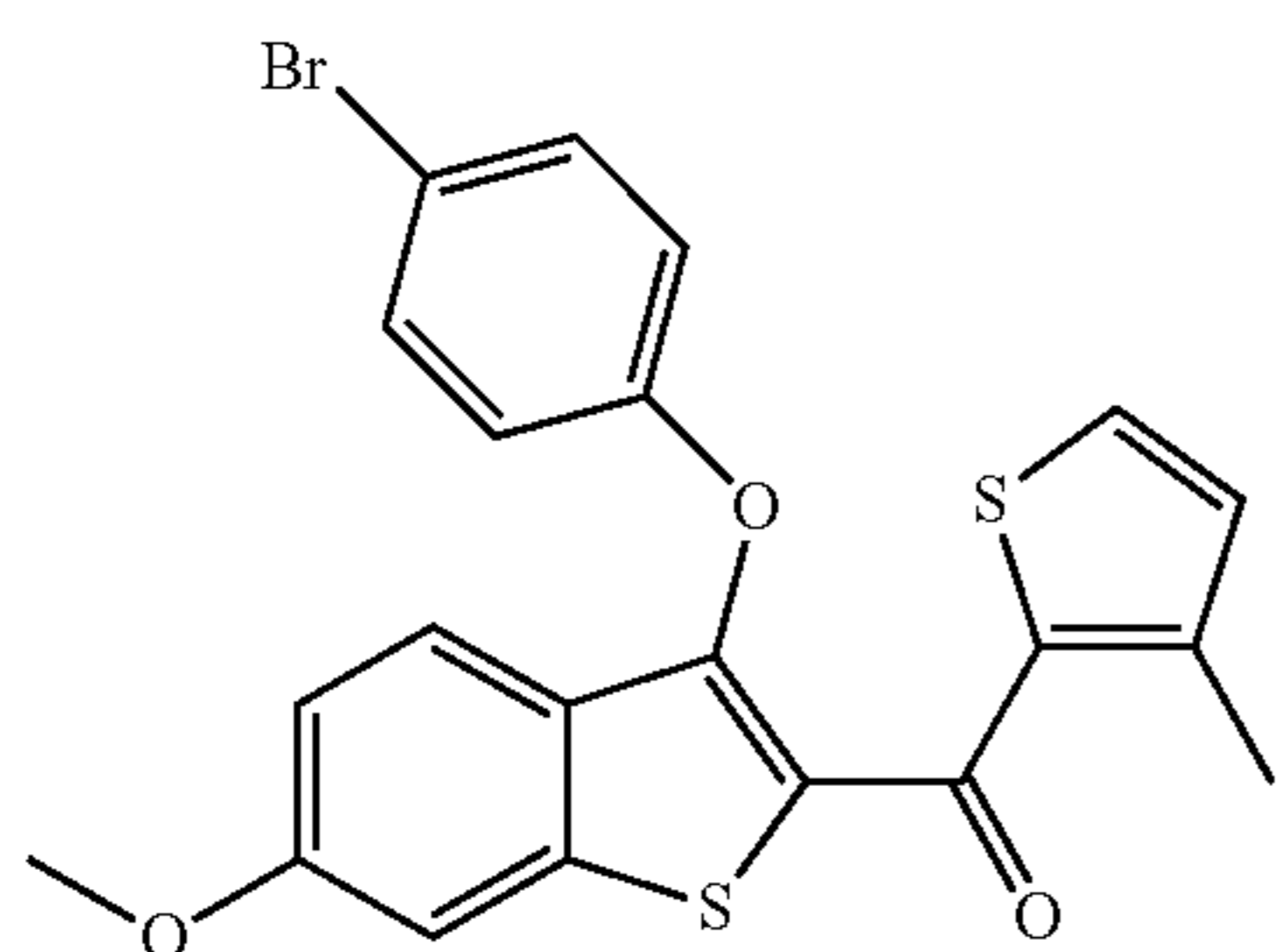
(3-(4-Bromophenoxy)-6-methoxybenzo[b]thiophen-2-yl)(3-methylthiophen-2-yl)methanone
