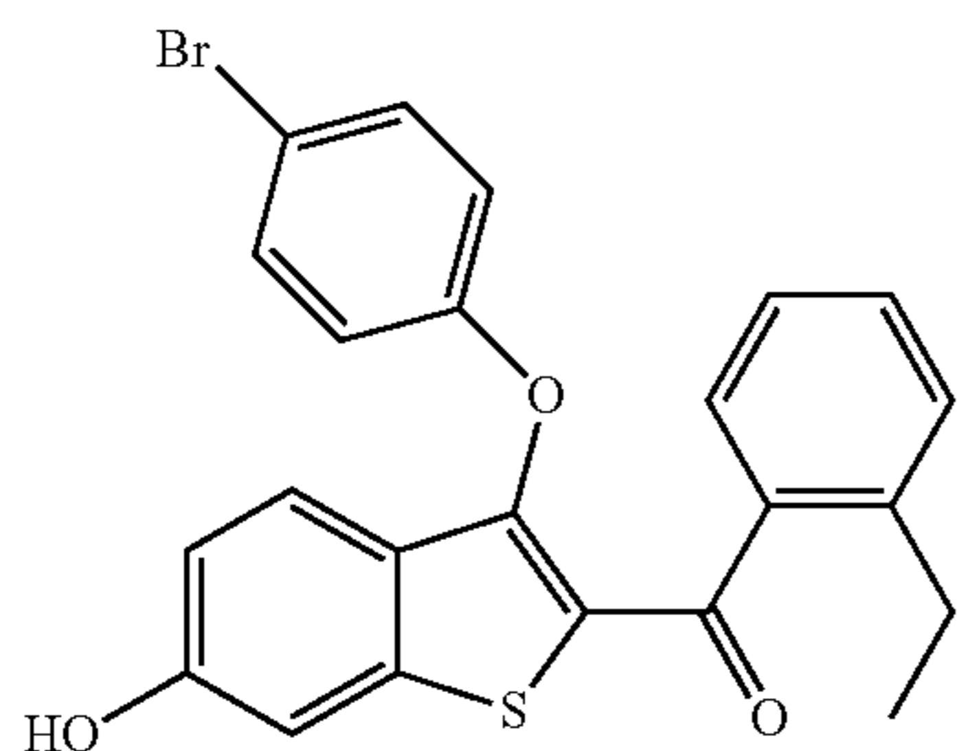
(3-(4-bromophenoxy)-6-hydroxybenzo[b]thiophen-2-yl)(2-ethylphenyl)methanone
