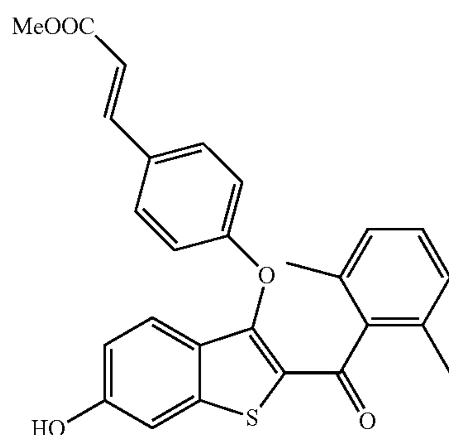
Methyl (E)-3-(4-((2-(2,6-dimethylbenzoyl)-6-hydroxybenzo[b]thiophen-3-yl)oxy)phenyl)acrylate
