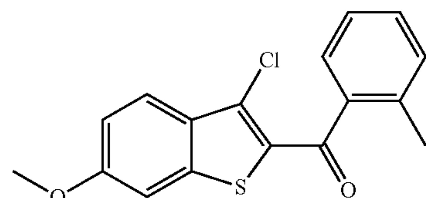
(3-Chloro-6-methoxybenzo[b]thiophen-2-yl)(o-tolyl)methanone
