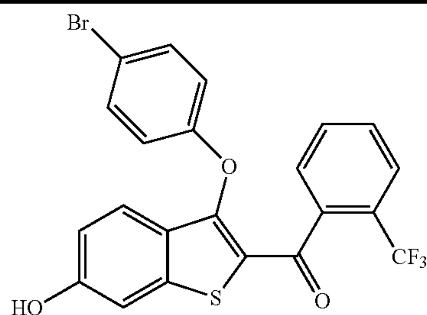
(3-(4-Bromophenoxy)-6-hydroxybenzo[b]thiophen-2-yl)(2-(trifluoromethyl)phenyl)methanone
