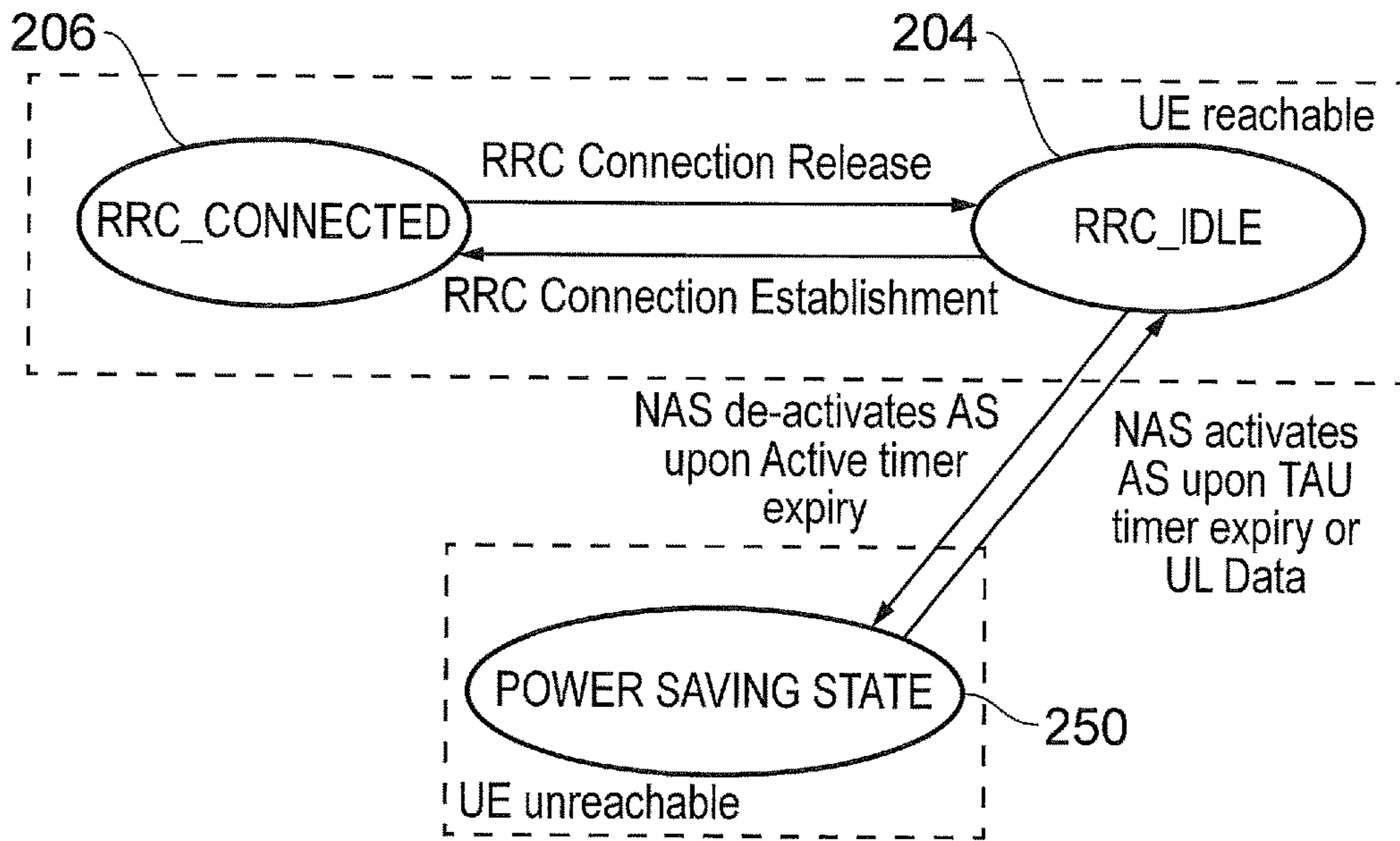
Power saving state in the UE from Idle state
