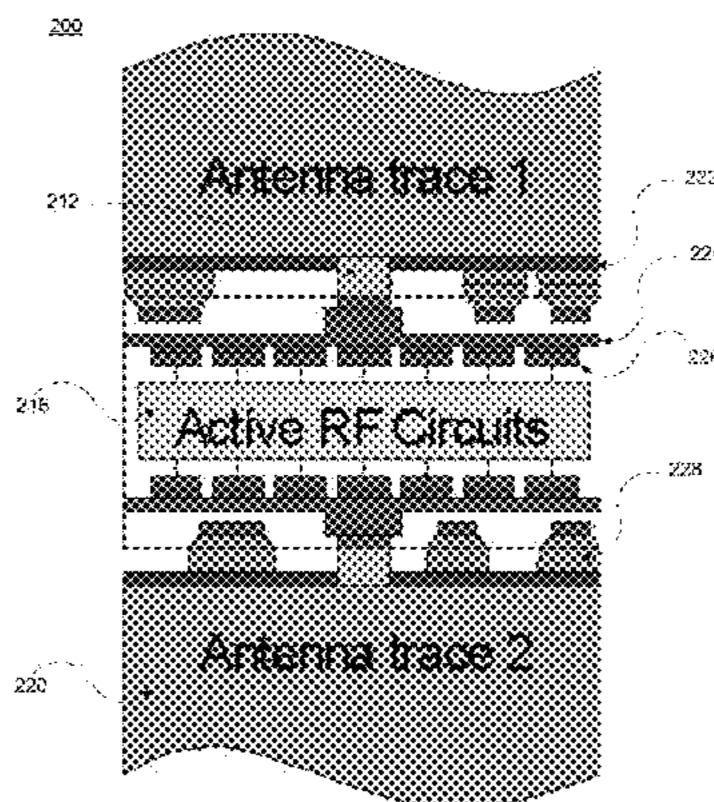
CONCEPTUAL DIAGRAM OF AN ASSEMBLED RFID TAG
