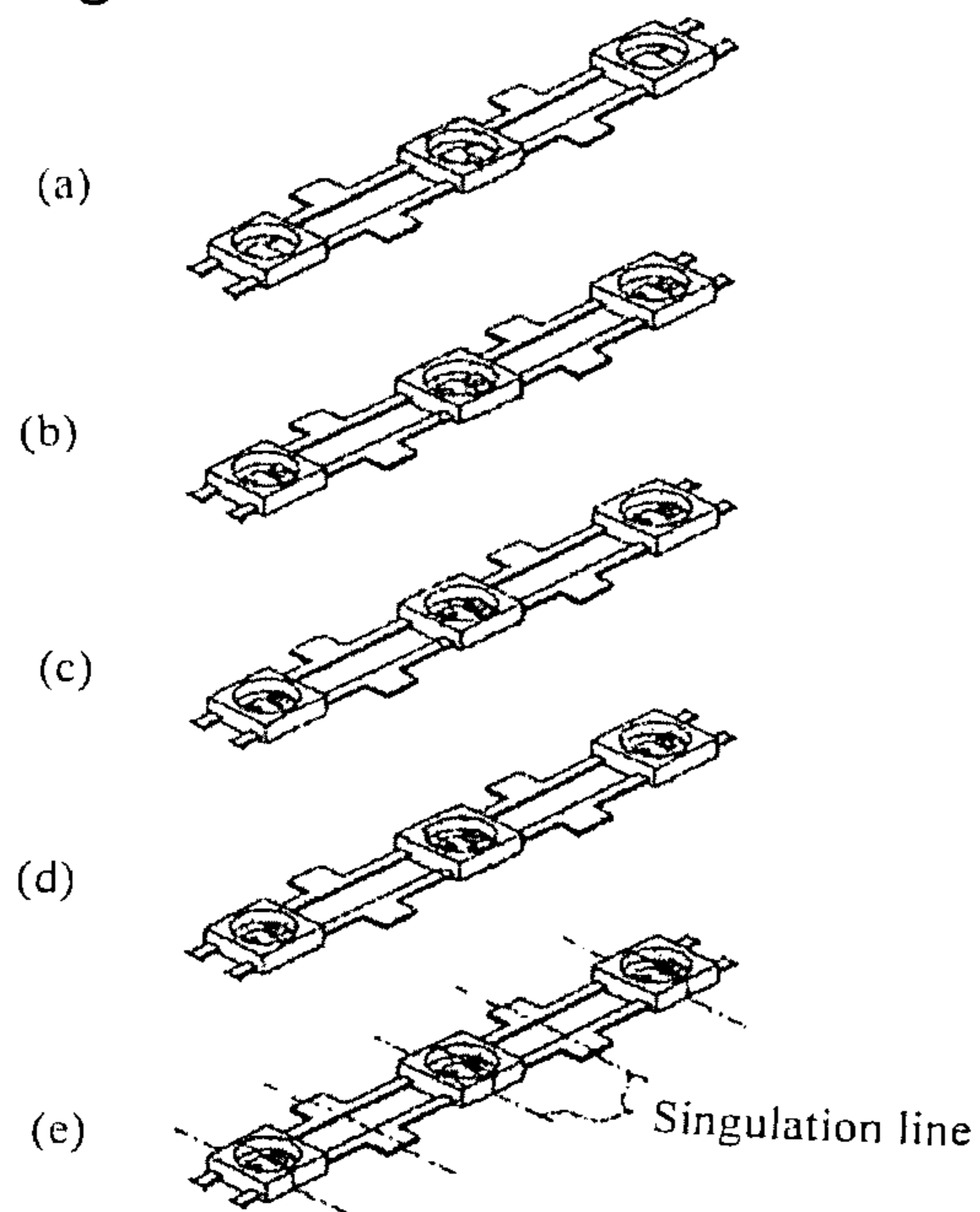
Fig. 14 (Prior Art)
