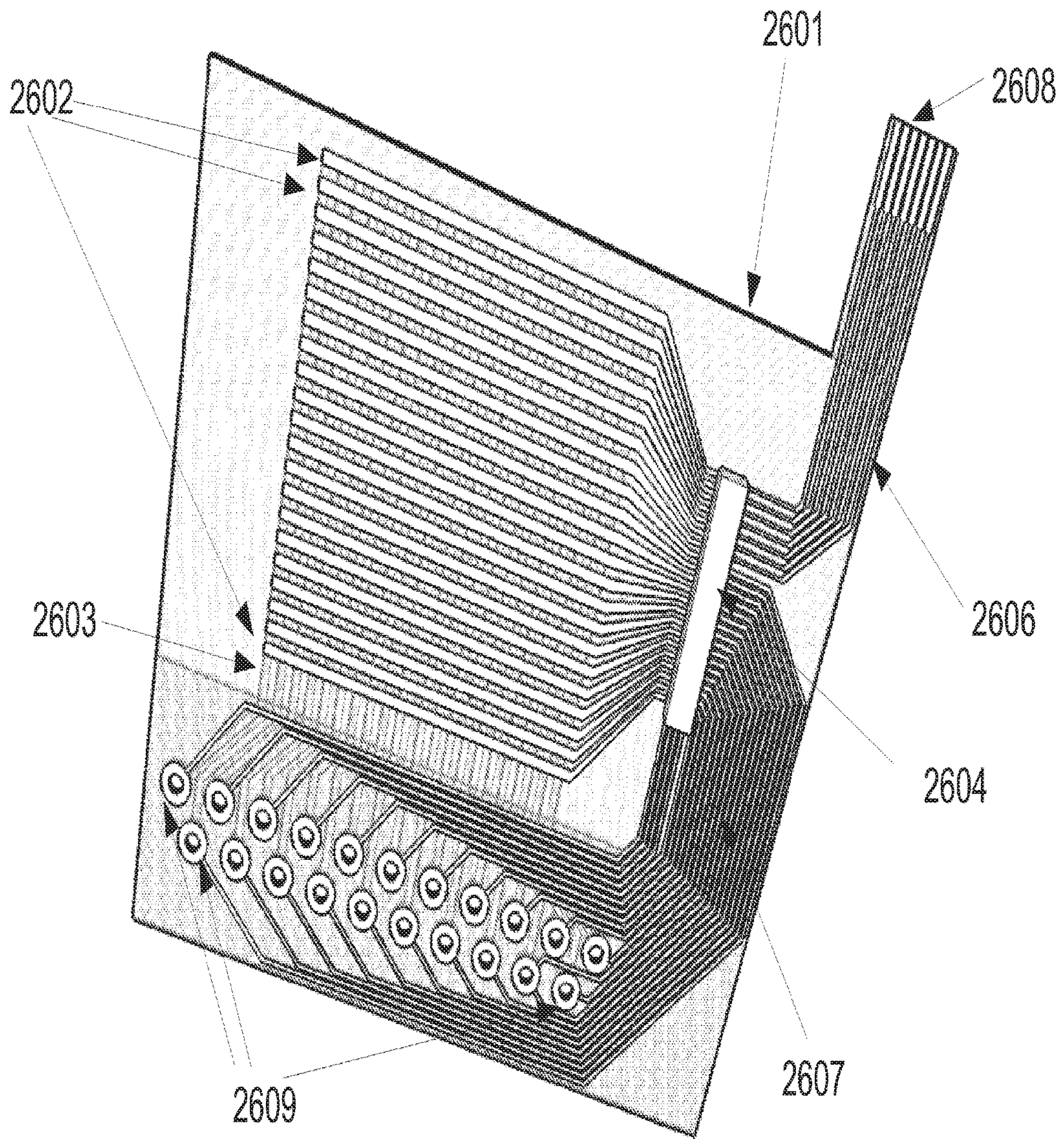
Figure 26b: Single Chip- Bottom View
