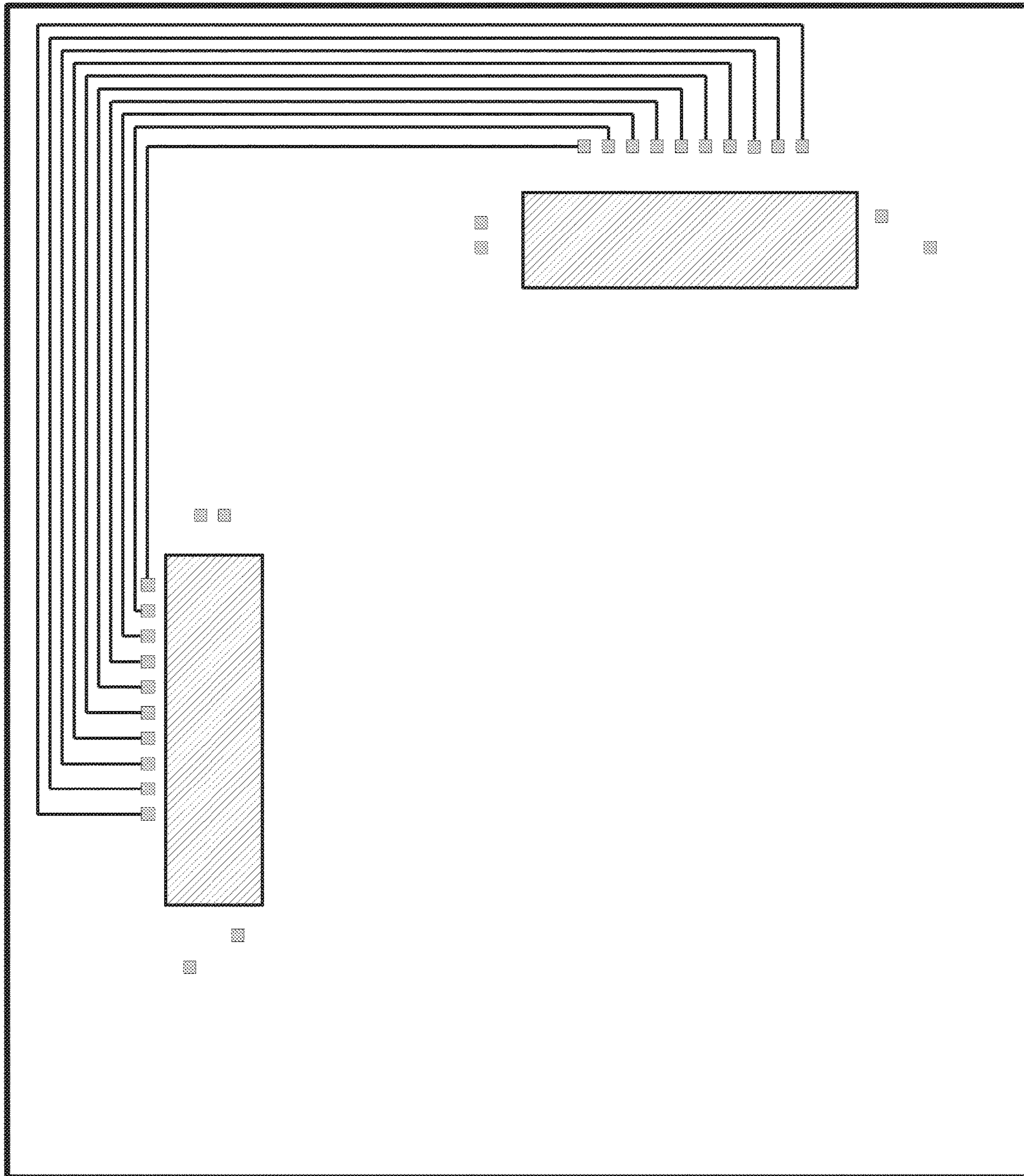
Fig 25C (Two Chip Sensor Substrate Top layer)
