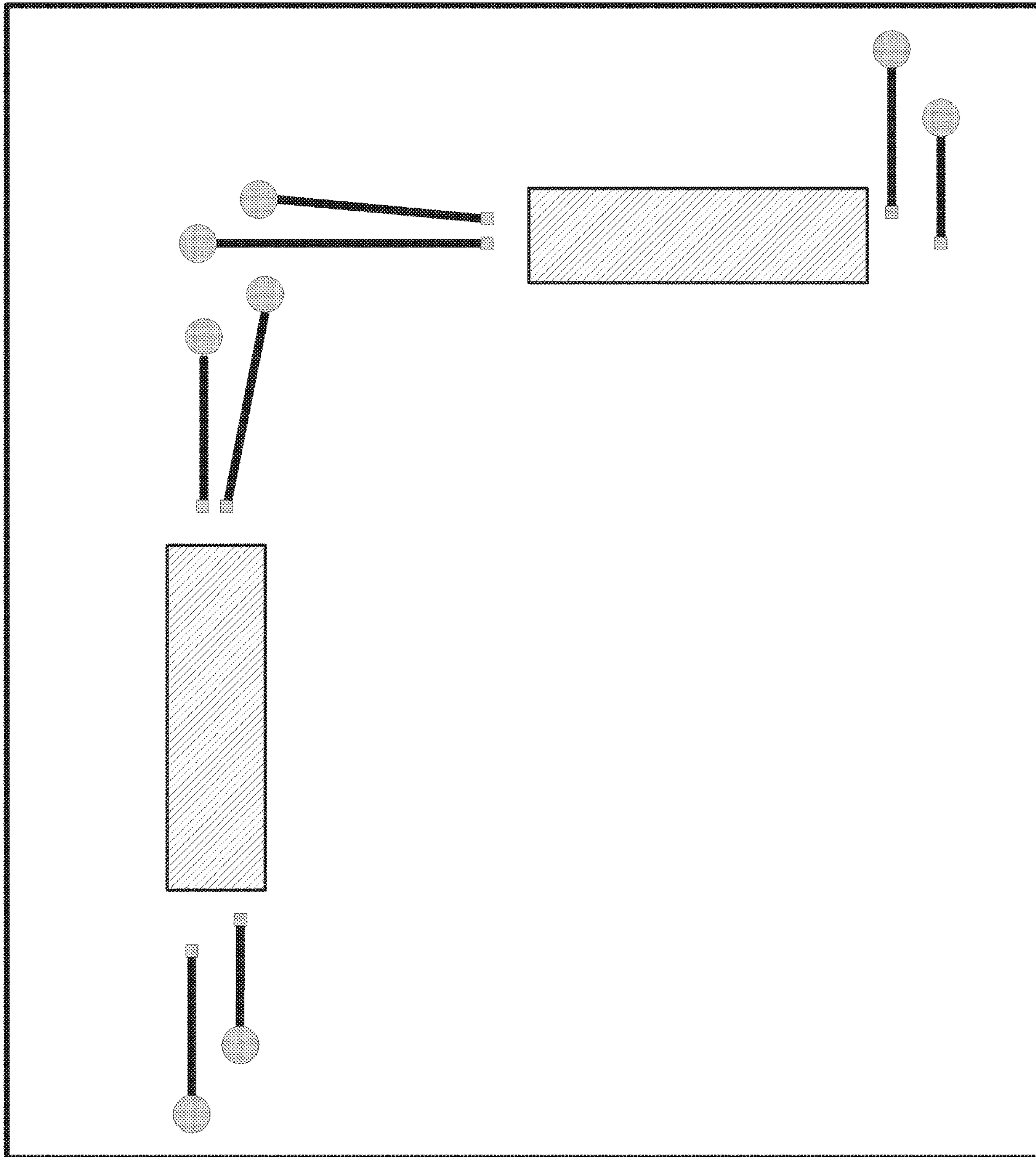
Fig 25B (Two Chip Sensor Substrate Bottom Layer)
