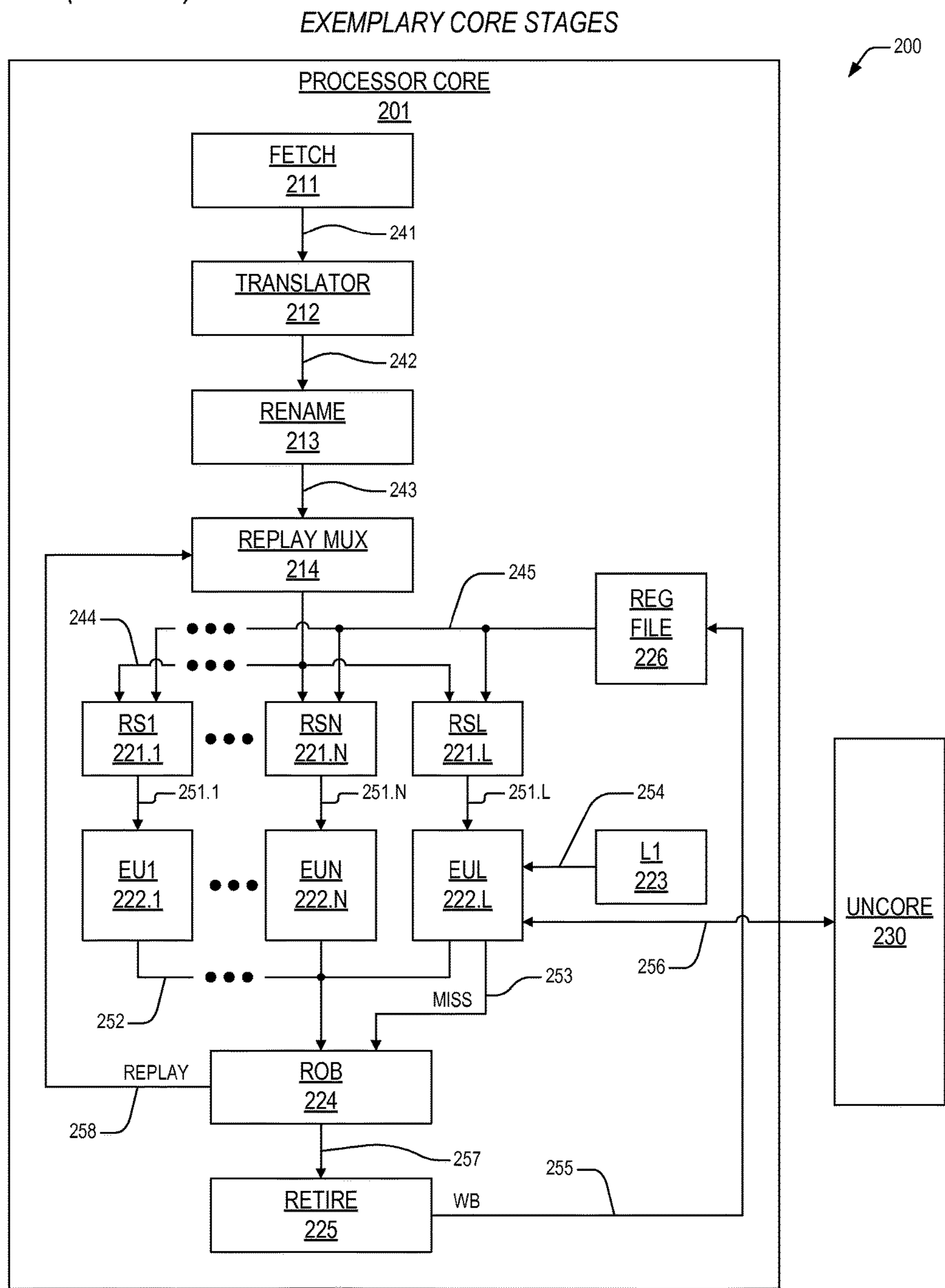
FIG. 2 (Prior Art)
