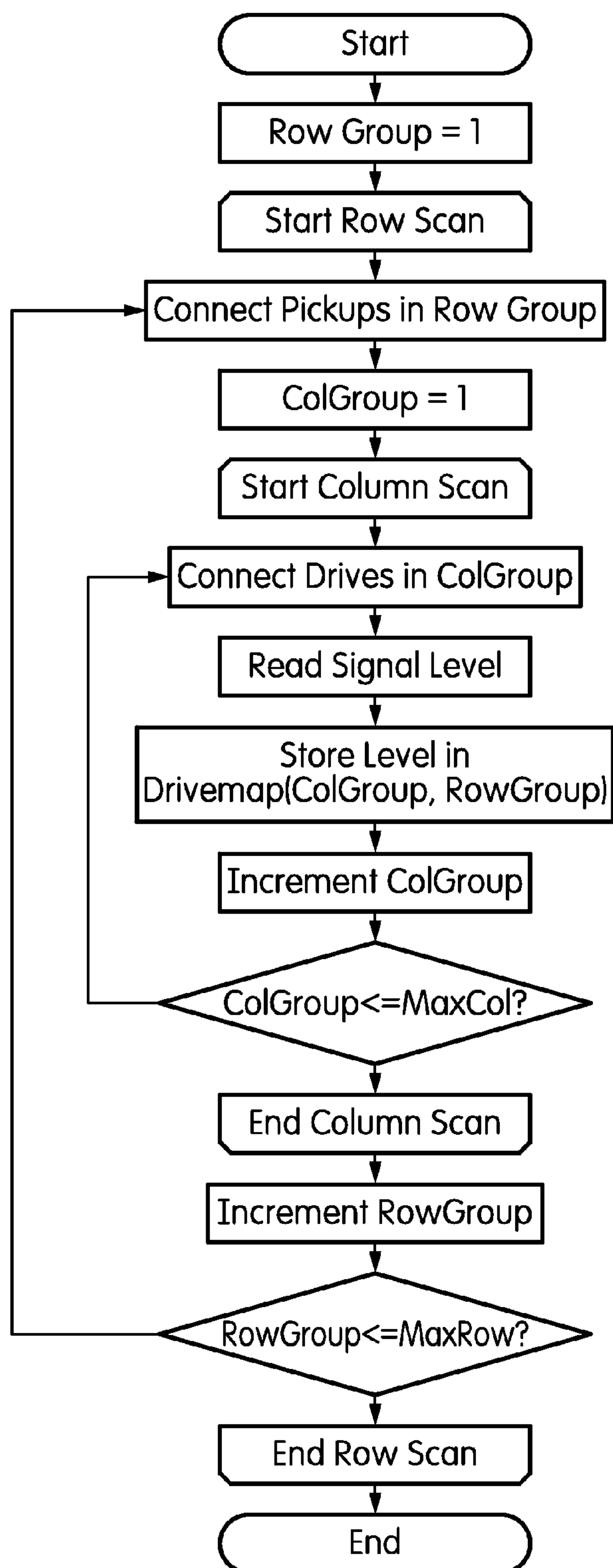
Dual Grid Coarse Position Determination - Scan Process
