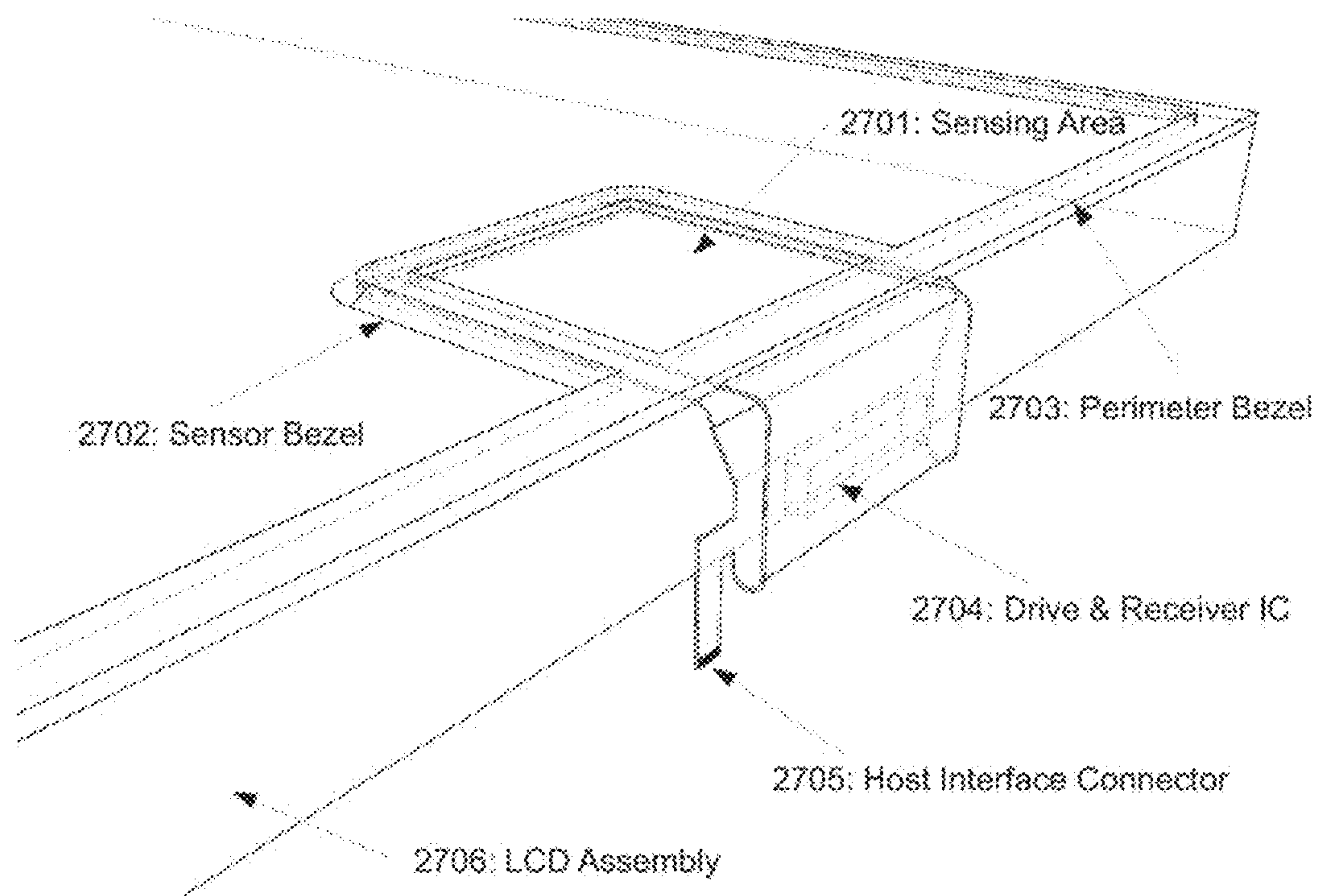
Fig 27: Screen with Fingerprint Sensor Overlay
