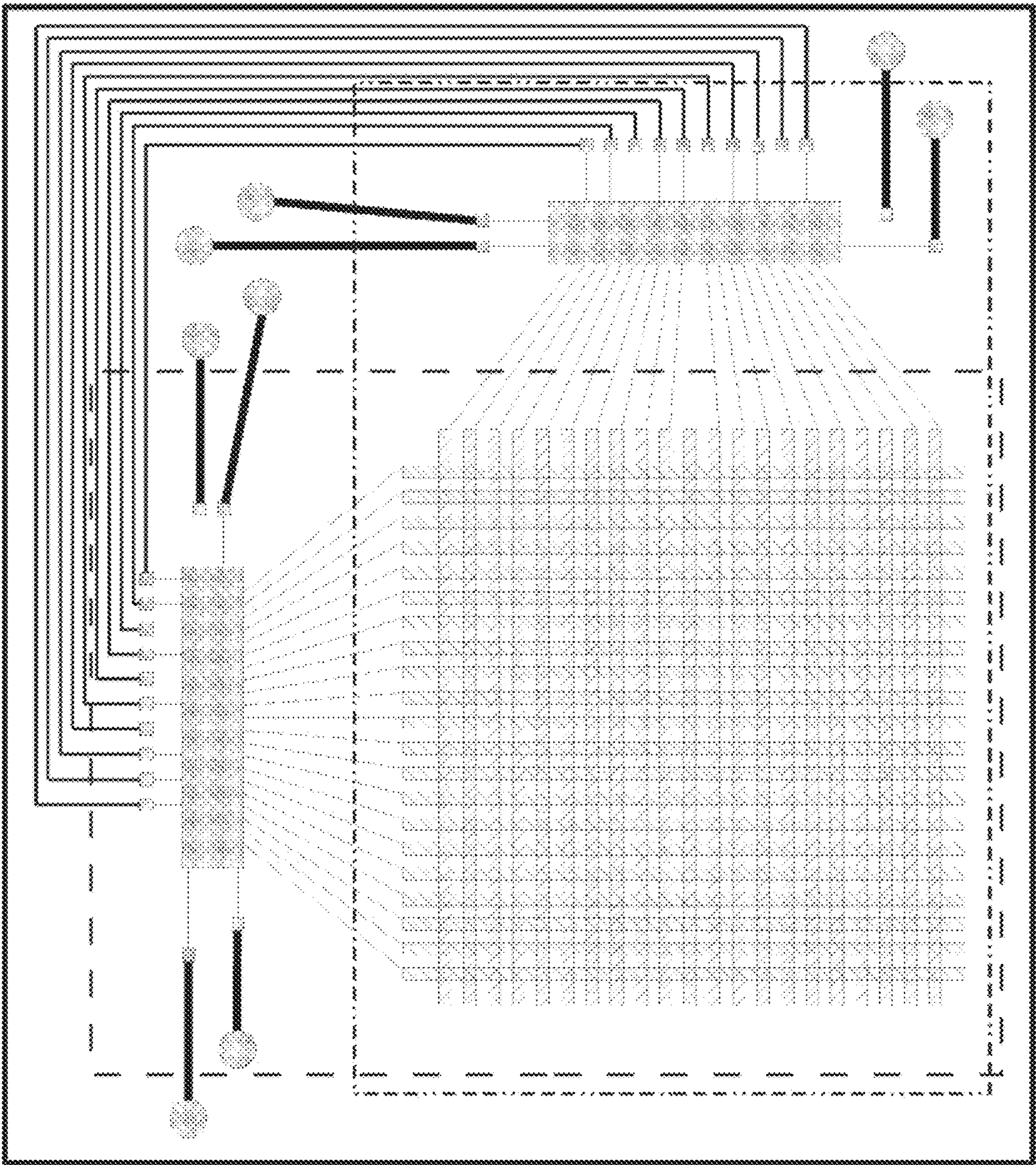
Fig 25A (Two Chip Sensor Stack-up)
