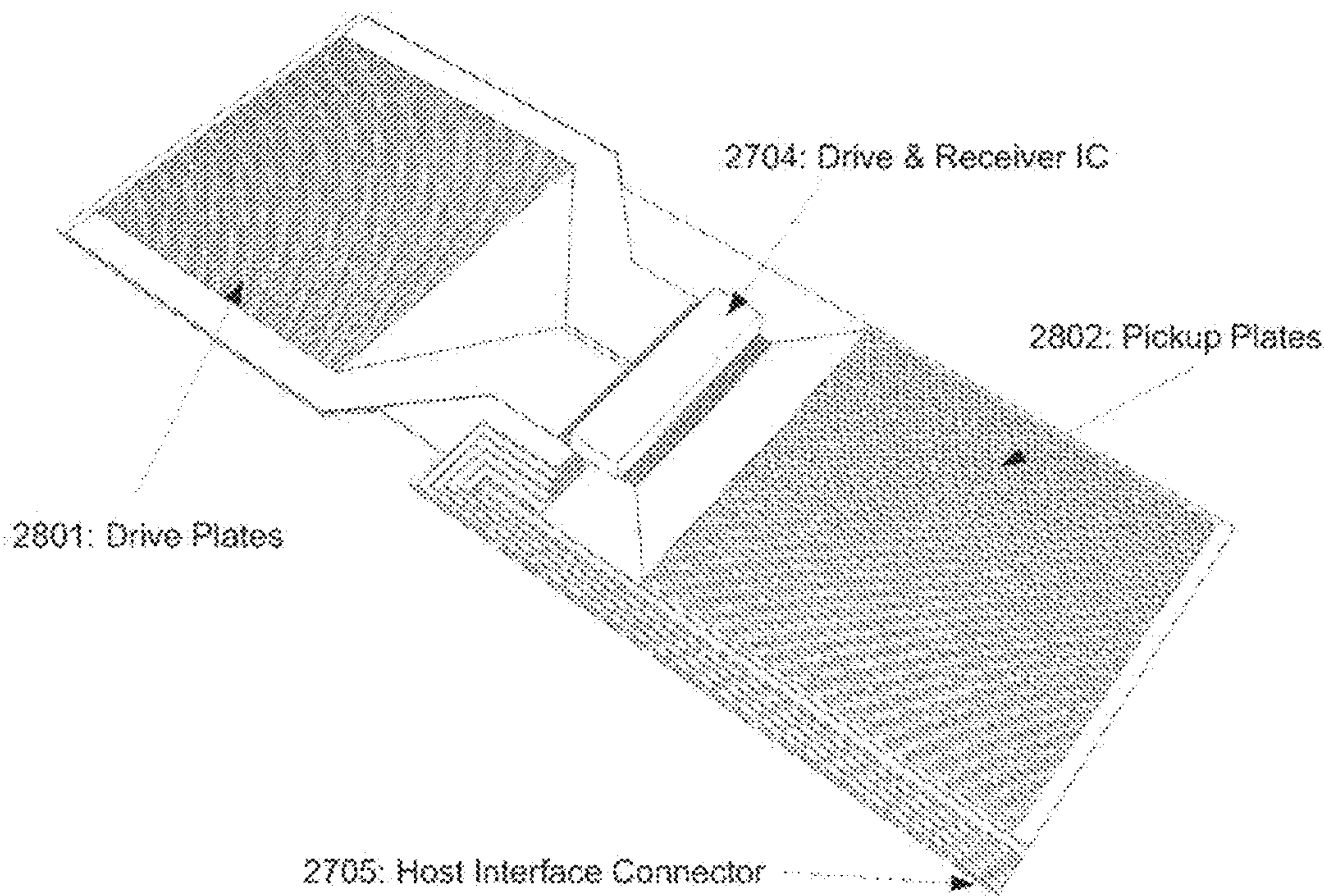
Fig 28: Unfolded Sensor
