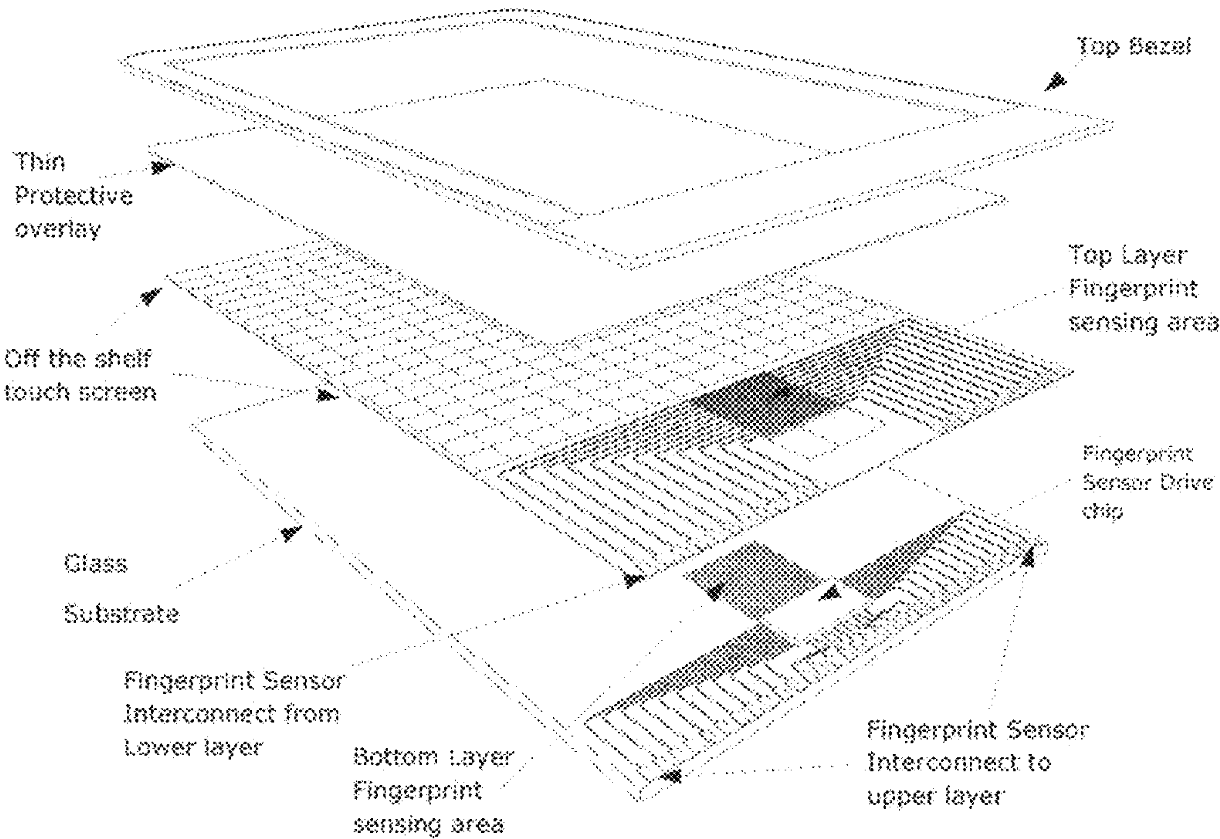
Fig 30: Exploded view of Fingerprint Sensor Sharing Substrate with Touchscreen
