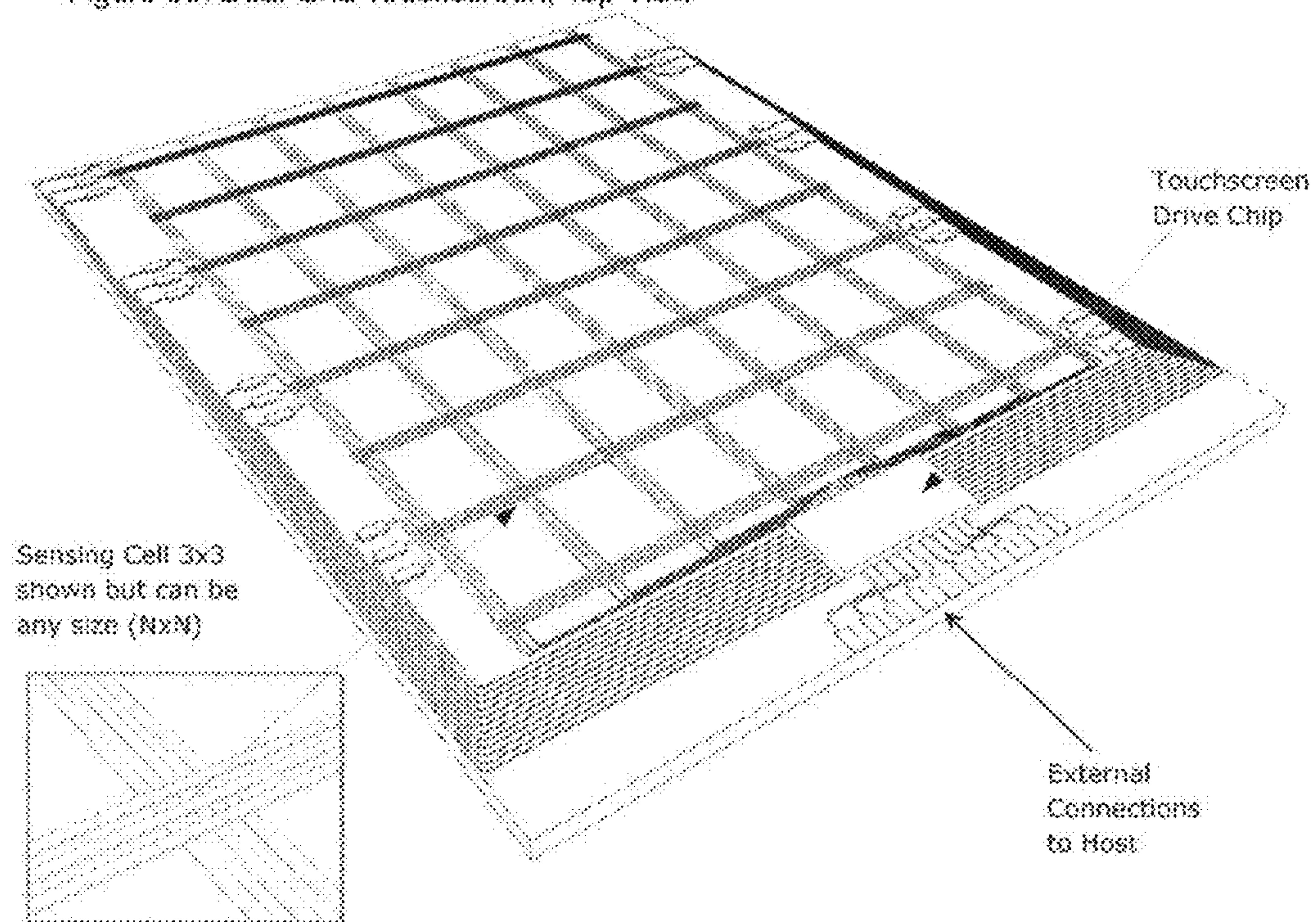
Figure 33: Dual Grid Touchscreen, Top View
