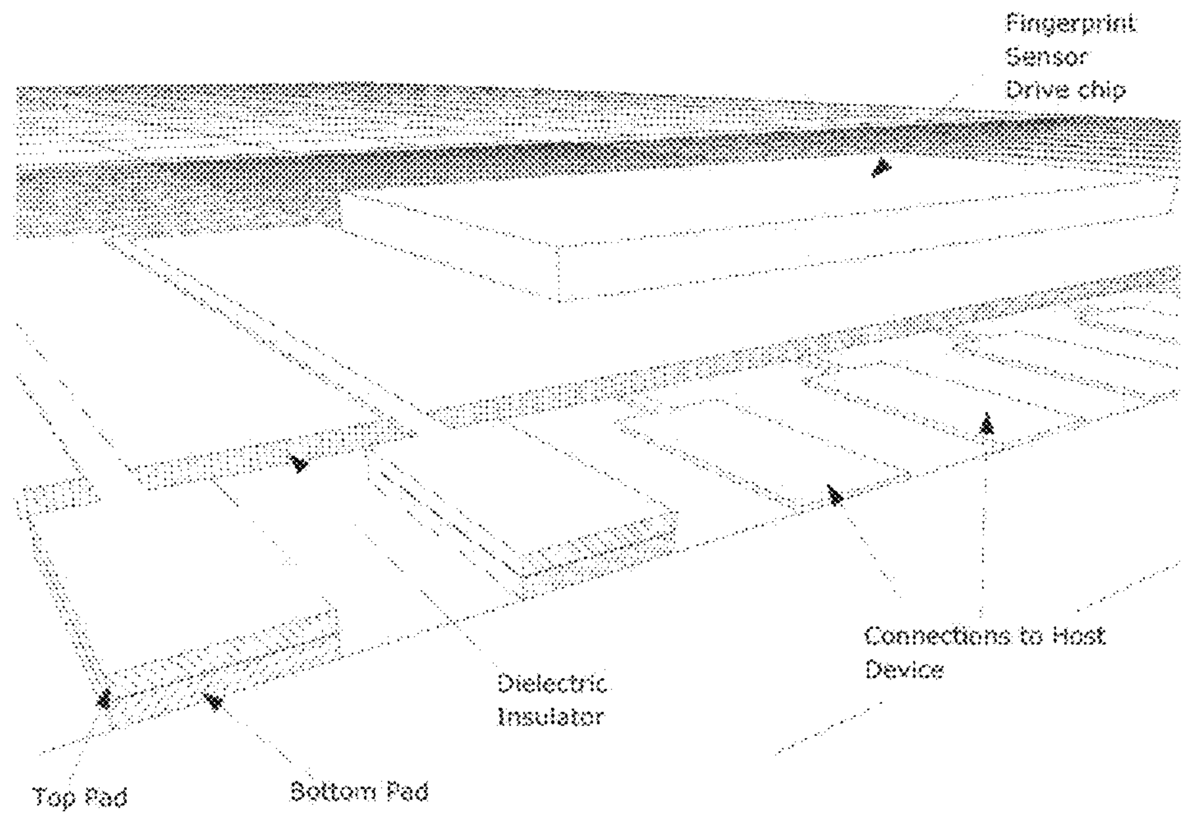
Fig 32: Detail Interconnect of Fingerprint Sensor Sharing Substrate with Touchscreen
