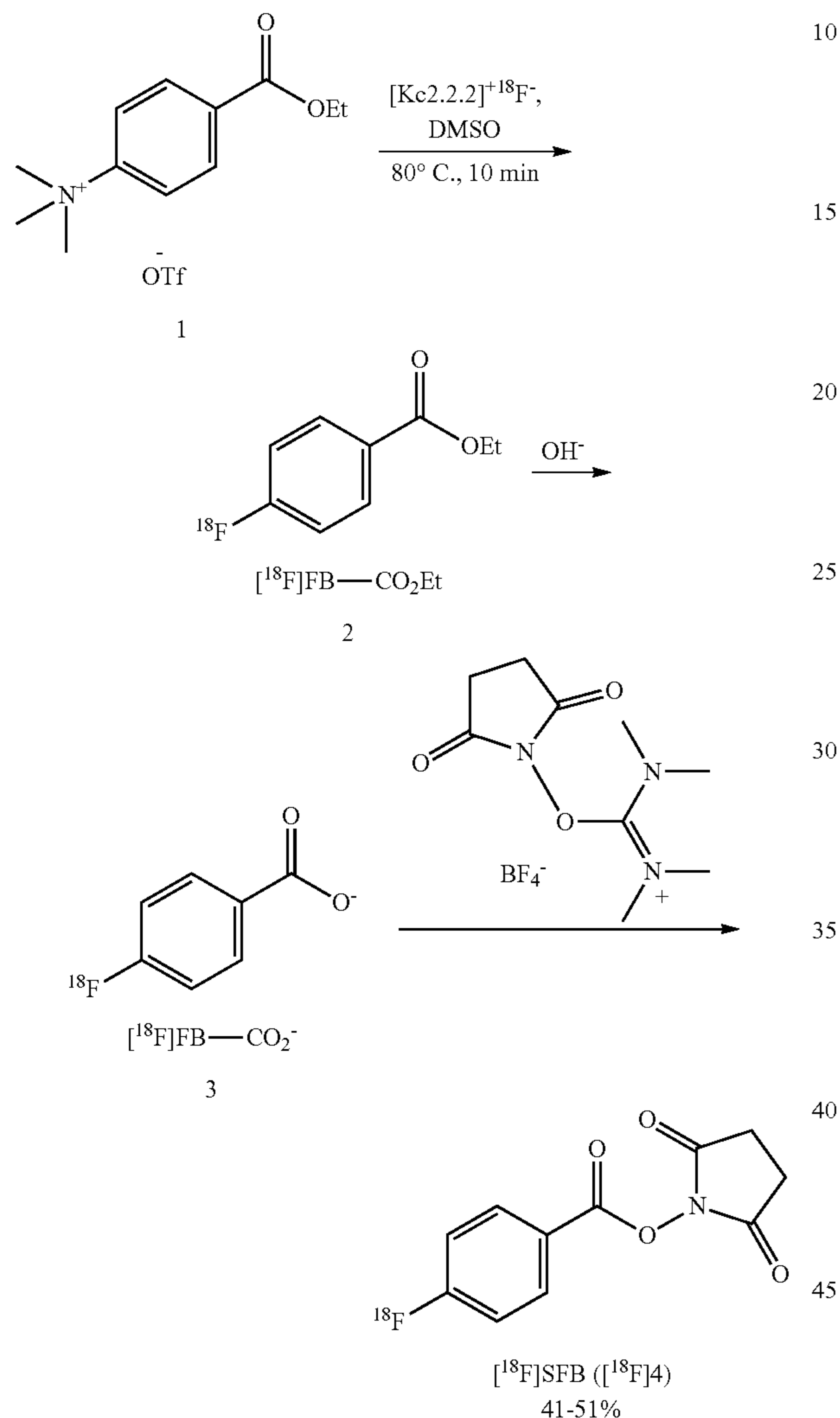
Scheme 1: Radiosynthesis of [ ^{18}\text{F} ]SFB according to Wester et al.
