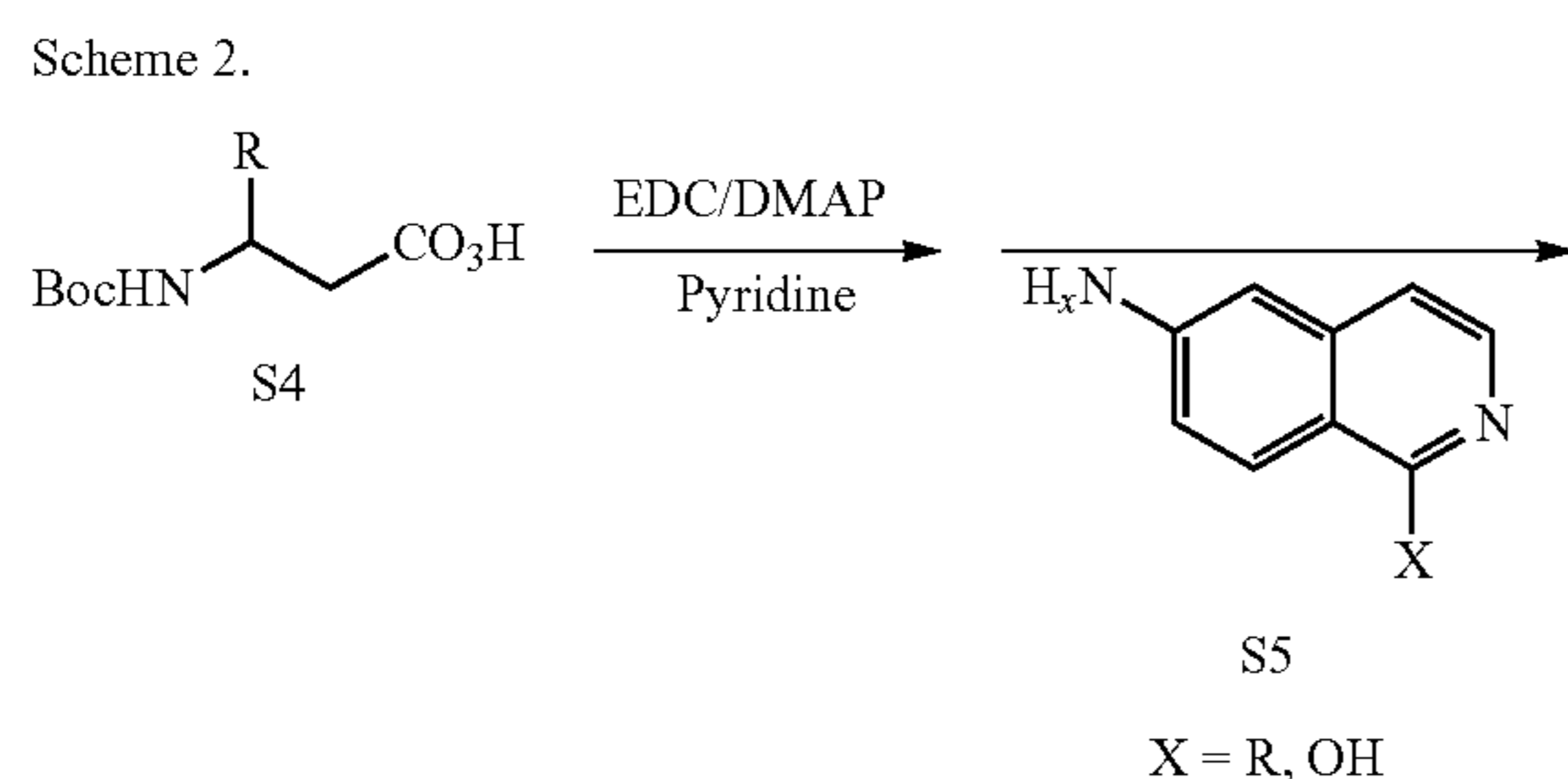
Scheme 2
