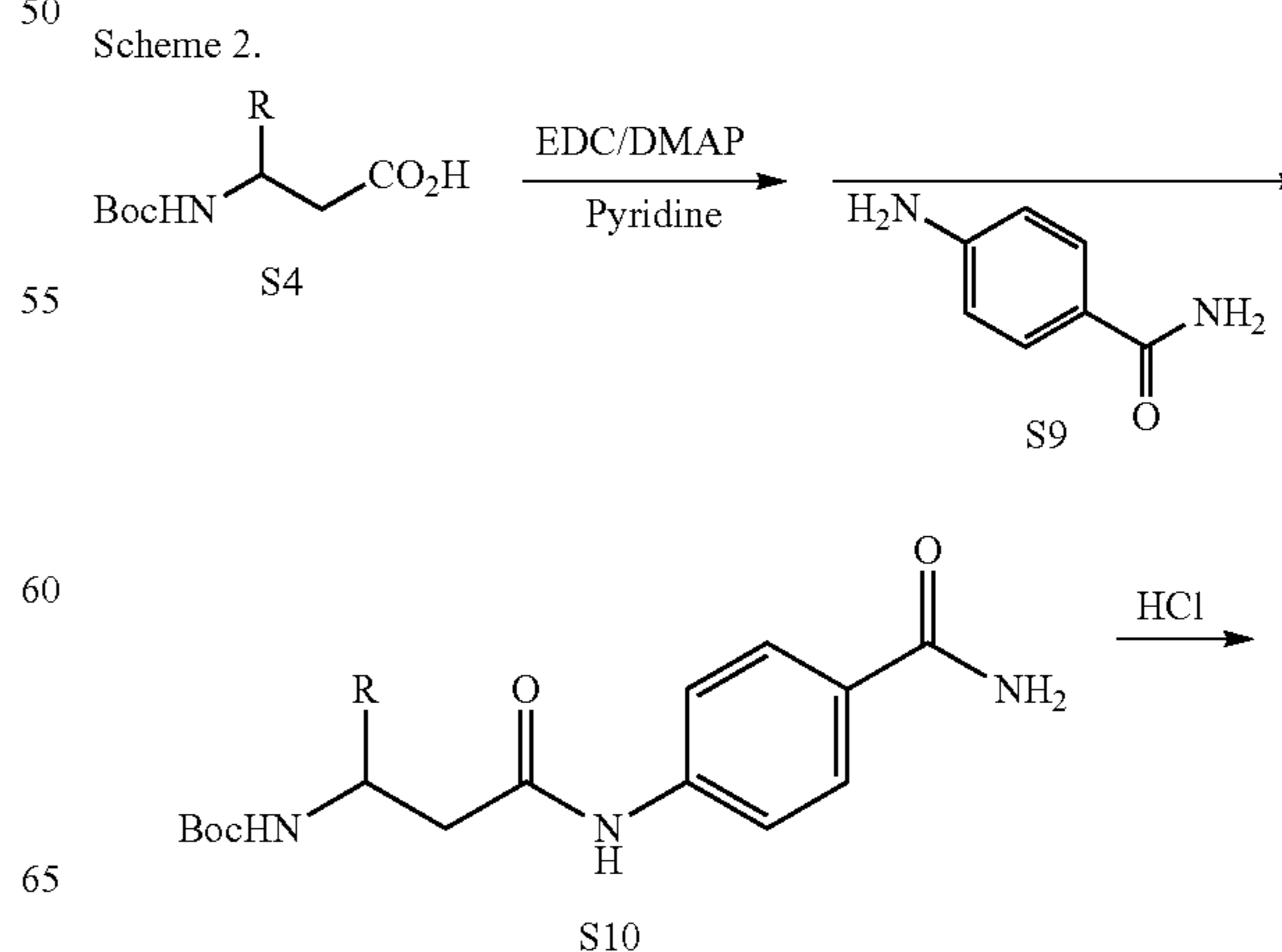
Scheme 3
