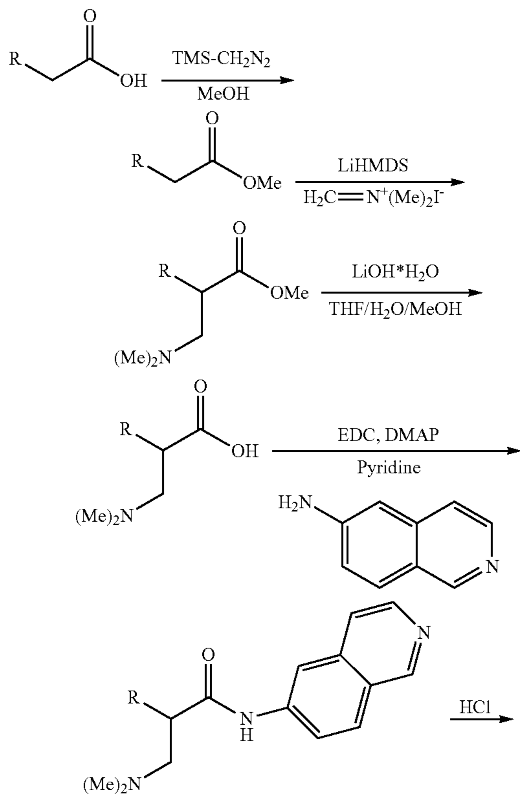
Scheme 4
