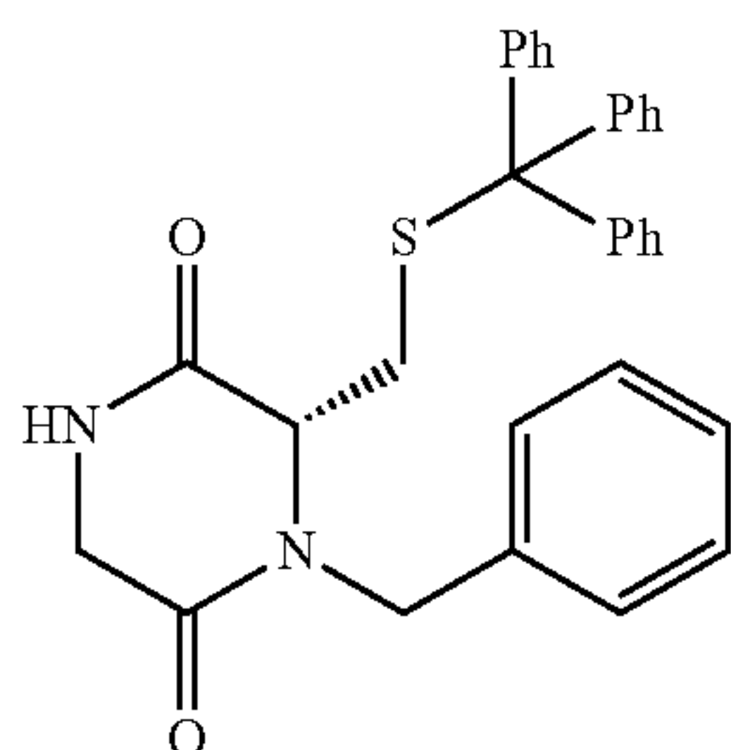
(6R)-1-benzyl-6-[(triphenylmethyl)sulfanyl]methyl}piperazine-2,5-dione
