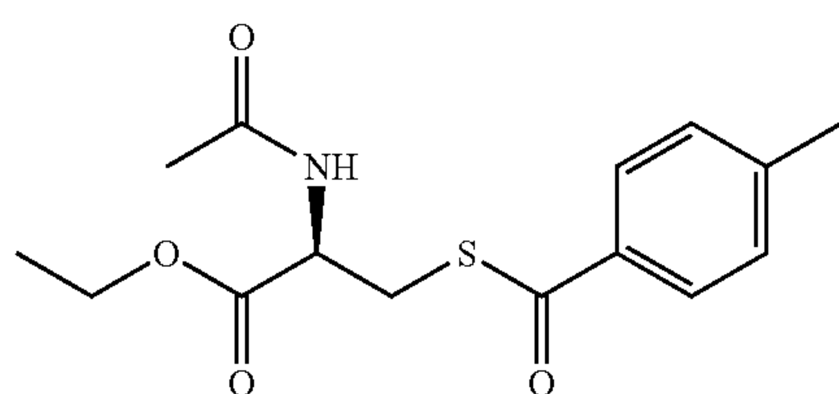
Ethyl (2R)-2-acetamido-3-(4-methylbenzoylsulfanyl)propanoate
