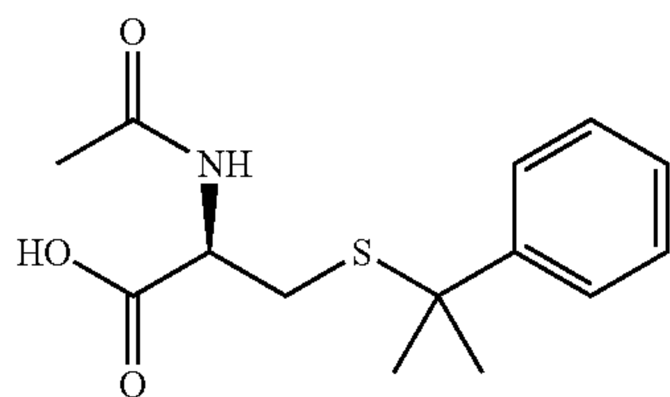
(2R)-2-Acetylamino-3-(1-methyl-1-phenyl-ethylsulfanyl)-propionic acid
