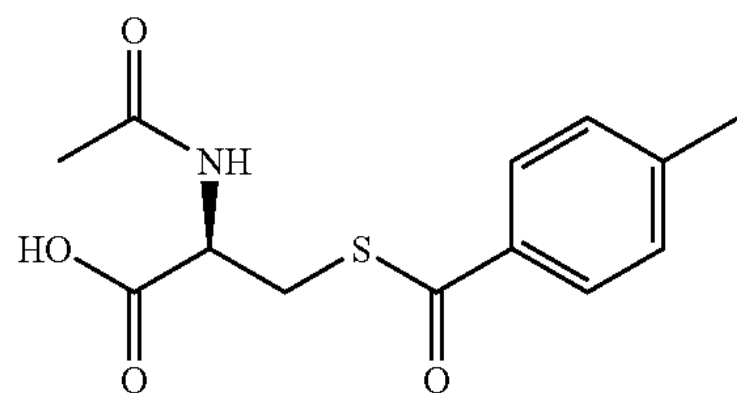
2-Acetylamino-3-(4-methylbenzoylsulfanyl)propionic acid
